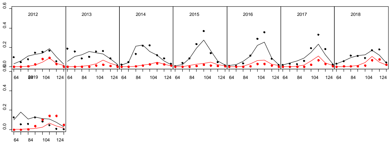
Summer Commercial total length New Shell & Old Shell: observed vs predictor
