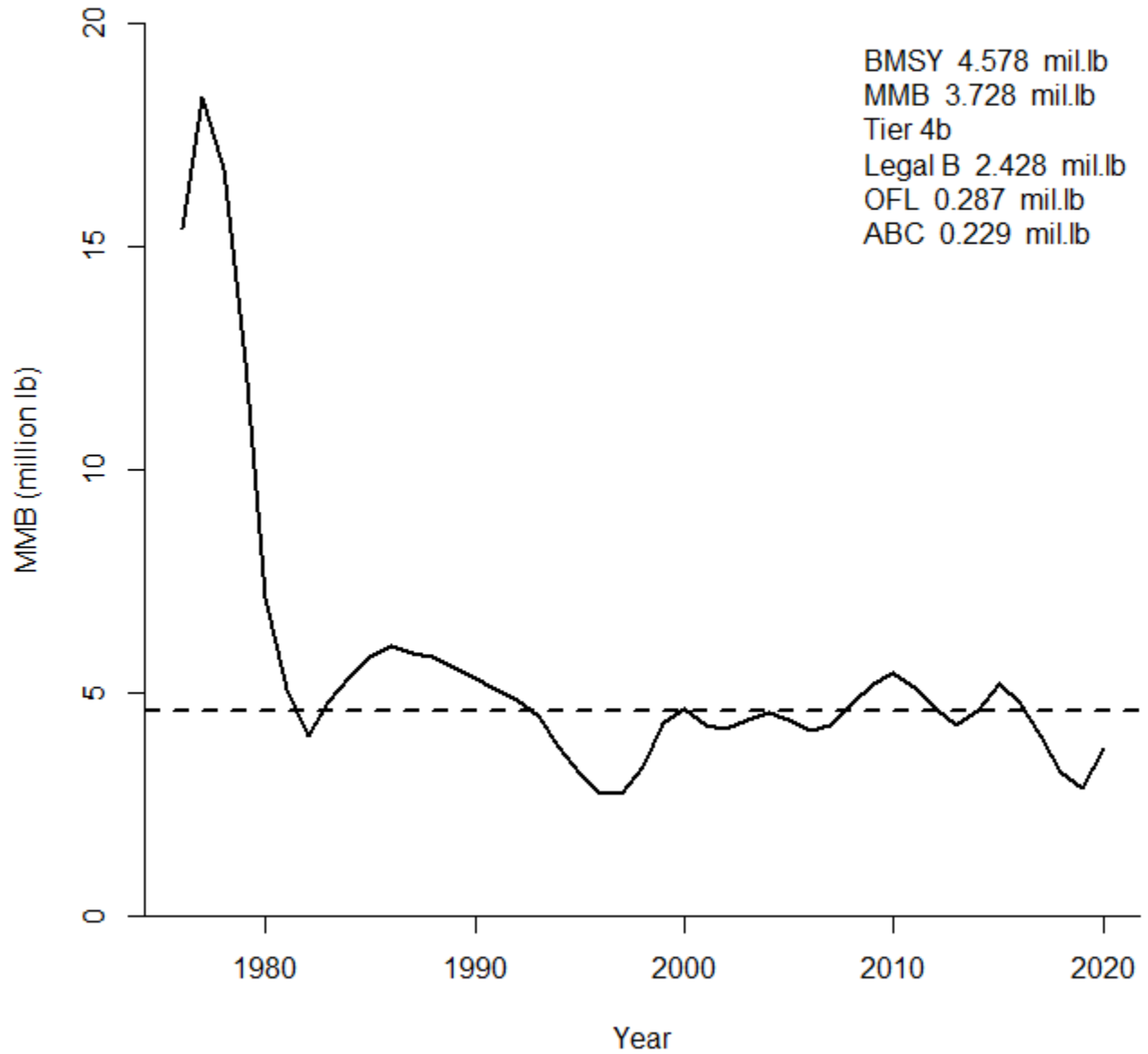
Figure 5. Estimated MMB during 1976-2019. Dash line shows Bmsy (Average MMB of 1980-2020). Dot indicate projected MMB of 2020.
