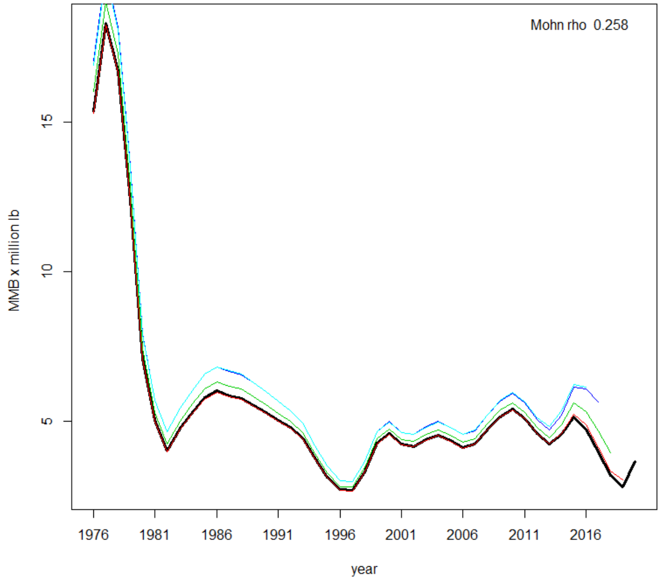
Figure 18. Retrospective Analyses of Norton Sound Red King Crab MMB from 2016 to 2019.
