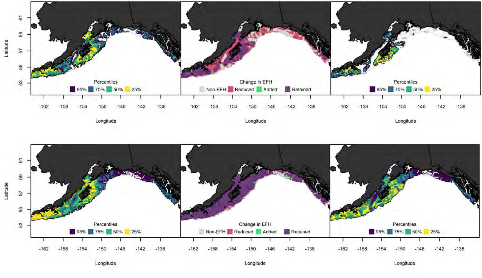
Fig. 1.12. Gulf of Alaska Pacific cod 2017 EFH percentiles ( left ) from RACE-GAP summer bottom trawl surveys (1993-2013; Rooney et al. 2018), changes in EFH area between the 2017 EFH map and the new EFH map ( center ), and new EFH percentiles ( right ) (1993-2019), where 25% = “hot spots”, 50% = “core habitat”, and all colored areas (25-95%) = EFH for subadults ( a ) and adults ( b ); contours are the 100, 200, and 500 m isobaths.
