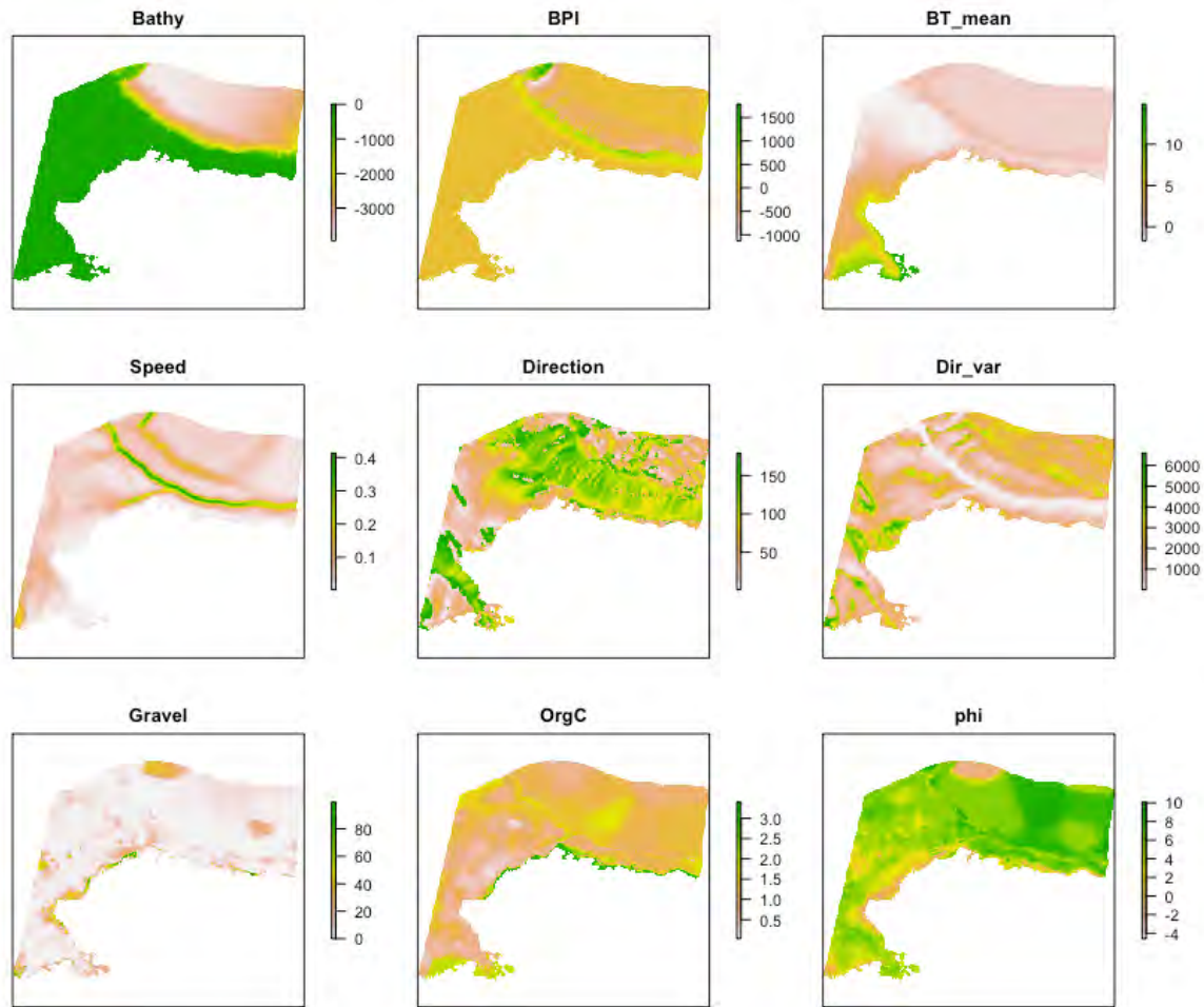
Fig. 2.2. Selected habitat covariates to be considered in the species distribution models for the demersal life stages of Arctic cod, saffron cod, and snow crab: bathymetry (m), bathymetric position index (bpi), mean summer bottom temperature (C), mean bottom current speed (m/s), mean bottom current direction (angle), mean bottom current direction variability, % gravel, % Organic Carbon and sediment size (phi).
