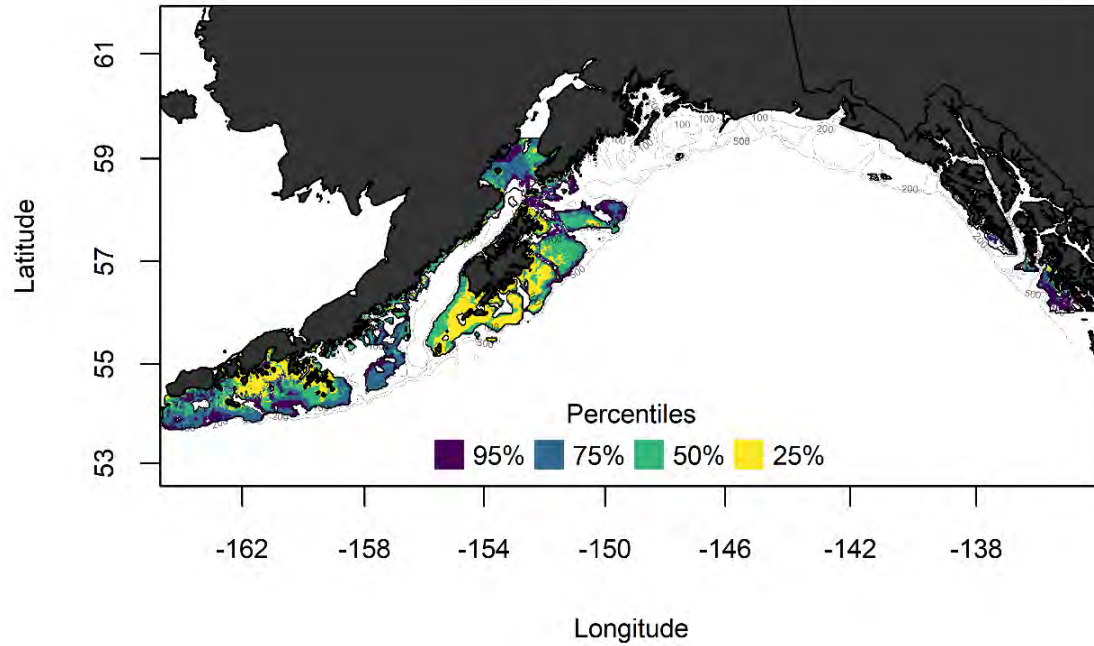
Fig. S.17. Composite of Gulf of Alaska subadult Pacific cod EFH percentiles (25% = “hot spots”, 50% = “core habitat”, all colored areas (25-95%) = EFH) constructed from species distribution model (SDM) predicted, habitat-linked abundance using RACE-GAP summer bottom trawl surveys (1993-2019); contours are 100, 200, and 500 m isobaths.
