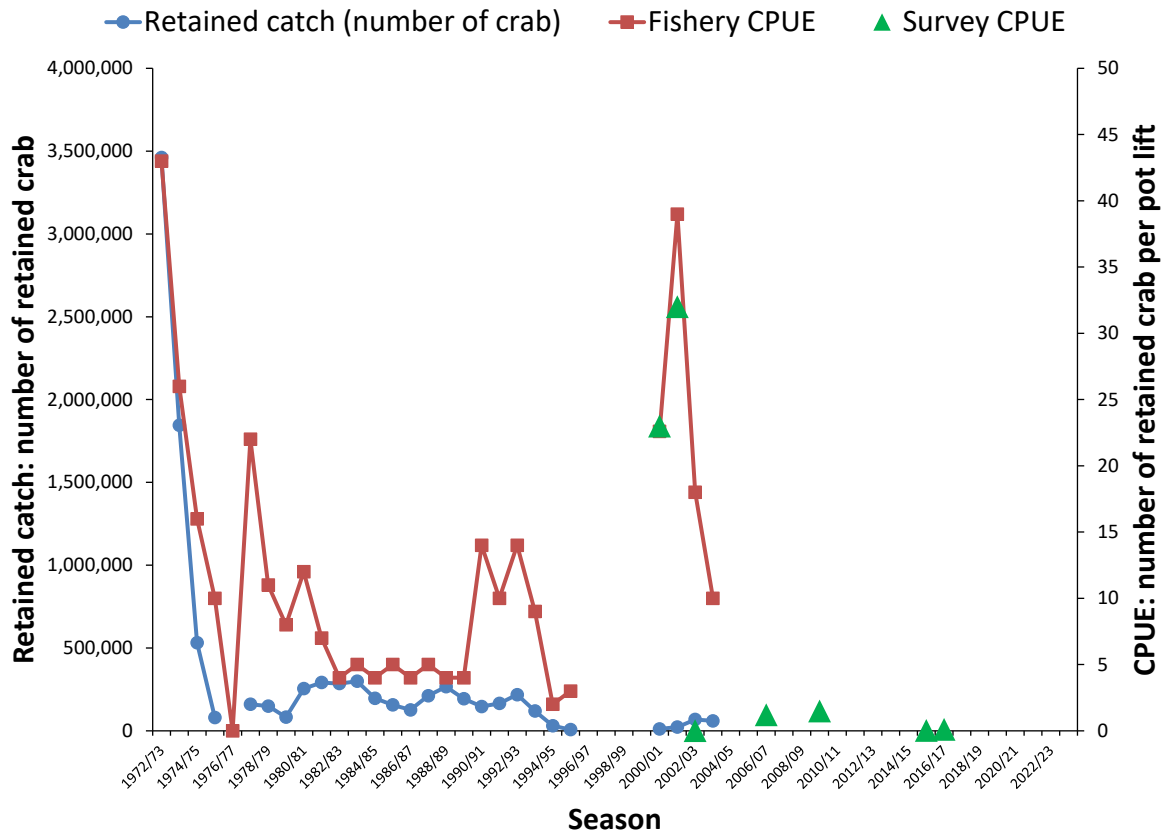
Figure 7. Retained catch (number of crab) and CPUE (number of retained crab per pot lift) in the western Aleutian Islands red king crab fishery, 1972/73–2022/23 (from Table 1a). Data for 1972/73–1983/84 are for the area west of 172° W longitude; data for 1984/85–1997/98, 1999/00, and 2004/05–2022/23 are for the area west of 171° W longitude; data for 1998/99 are for the area west of 174° W longitude; and data for 2000/01–2003/04 are for the area between 179° W longitude and 179° E longitude. ADF&G survey legal male CPUE values are shown by green triangles.
