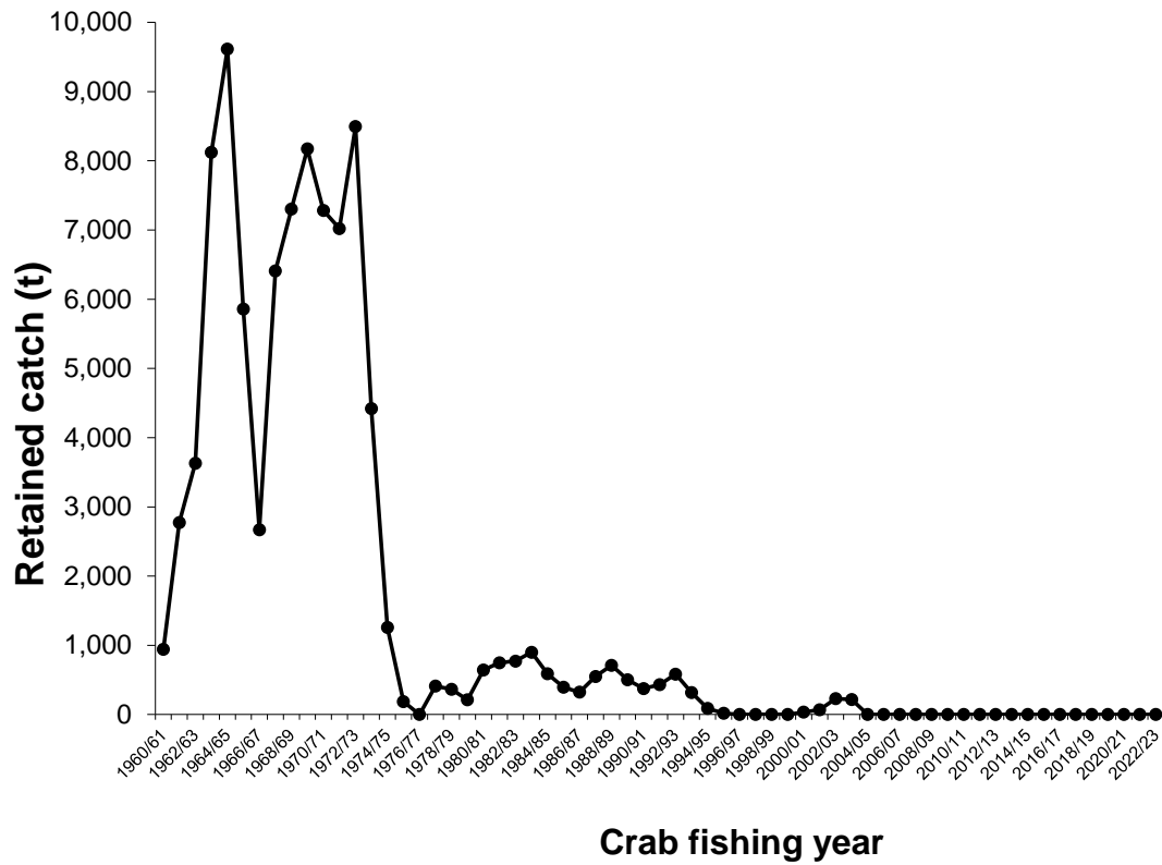
Figure 3. Retained catch (t) in the Western Aleutian Islands red king crab fishery, 1960/61–2022/23 (catch is for the area west of 172° W longitude during 1960/61–1983/84 and for the area west of 171° W longitude during 1984/85–2021/22; see Table 1a).
