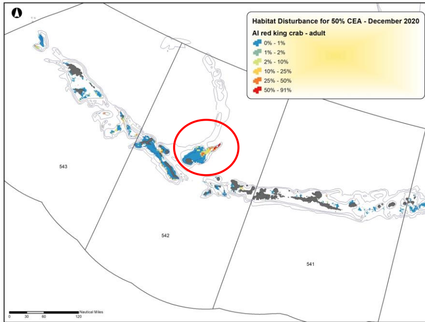
Figure C: Estimated habitat disturbance via NOAA fishing effect model.
