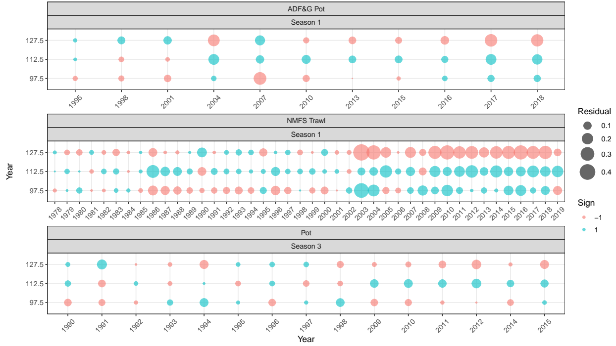
Figure 23: Bubble plots of residuals by stage and year for the all the size composition data sets (ADF&G pot survey, NMFS trawl survey, and the directed pot fishery) for SMBKC in the fit surveys model (19.1).
