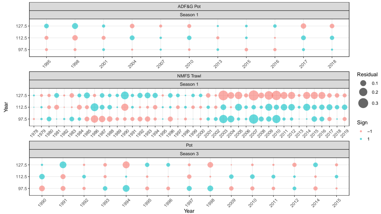
Figure 22: Bubble plots of residuals by stage and year for the all the size composition data sets (ADFG pot survey, NMFS trawl survey, and the directed pot fishery) for SMBKC in the reference model (19.0).
