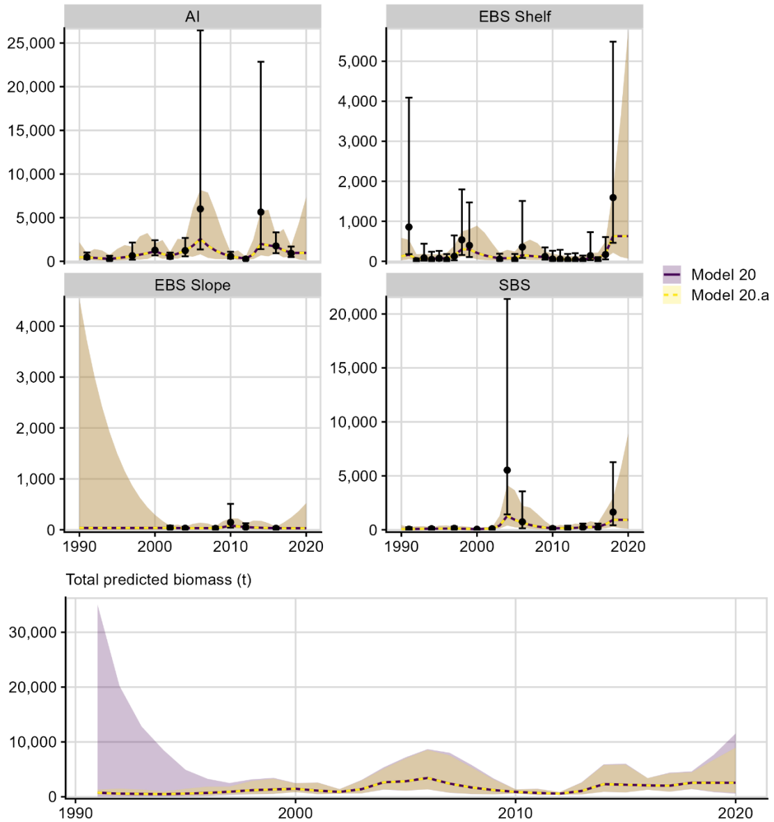
Figure C-2. Model fits by survey region (top) and total predicted biomass for all species in the other rockfish complex except shortspine thornyhead (SST). Results are shown for Model 20, the status quo multivariate random effects (REM) model fit in AD Model Builder, and Model 20.a, the same REM model but fit in Template Model Builder.
