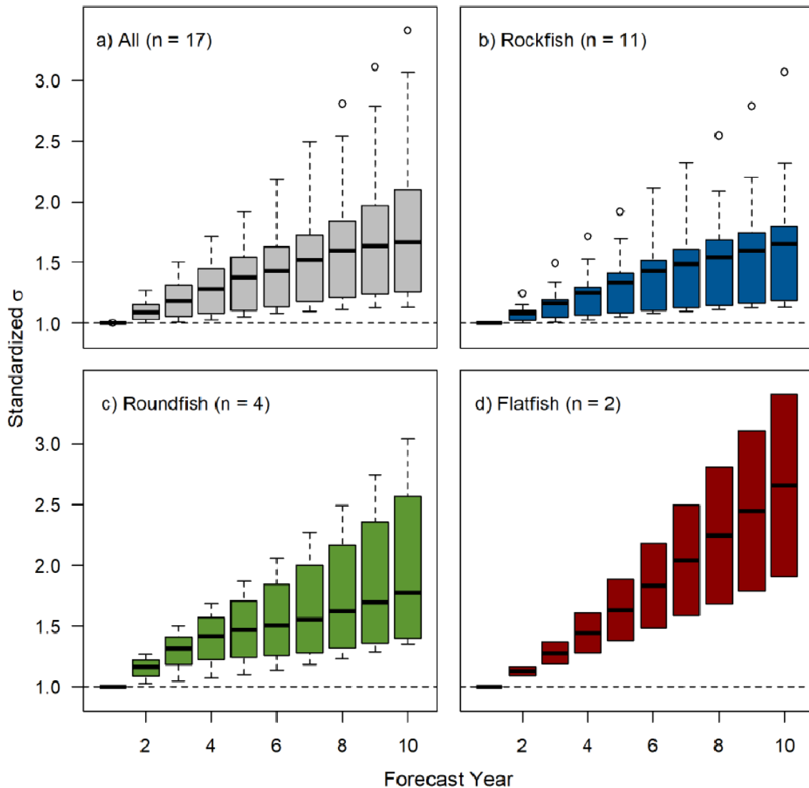
Figure 4. Change in sigma reflecting increased uncertainty during the projection period grouped by life history for assessed West Coast stocks. The number of species in each life history grouping is shown in each figure. (From Wetzel and Hamel 2019).
