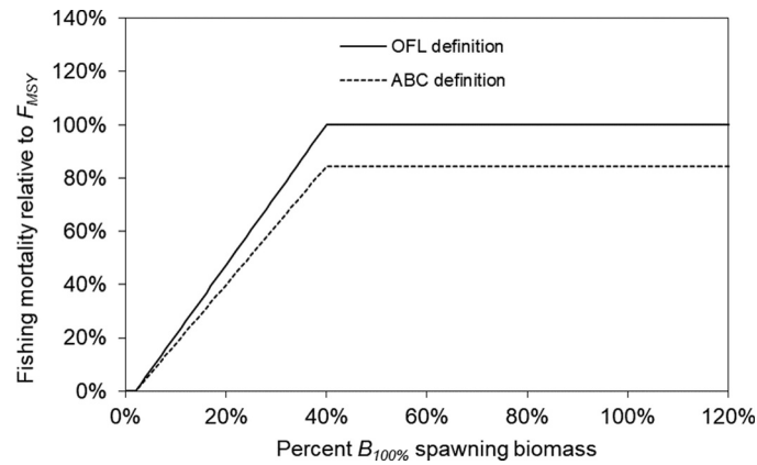
Figure 1. Harvest control rule for NPFMC Tier 3 stocks where F35% is considered a proxy for FMSY showing the buffer between the ABC and OFL, and how fishing mortality is ramped downwards as stock size declines.
