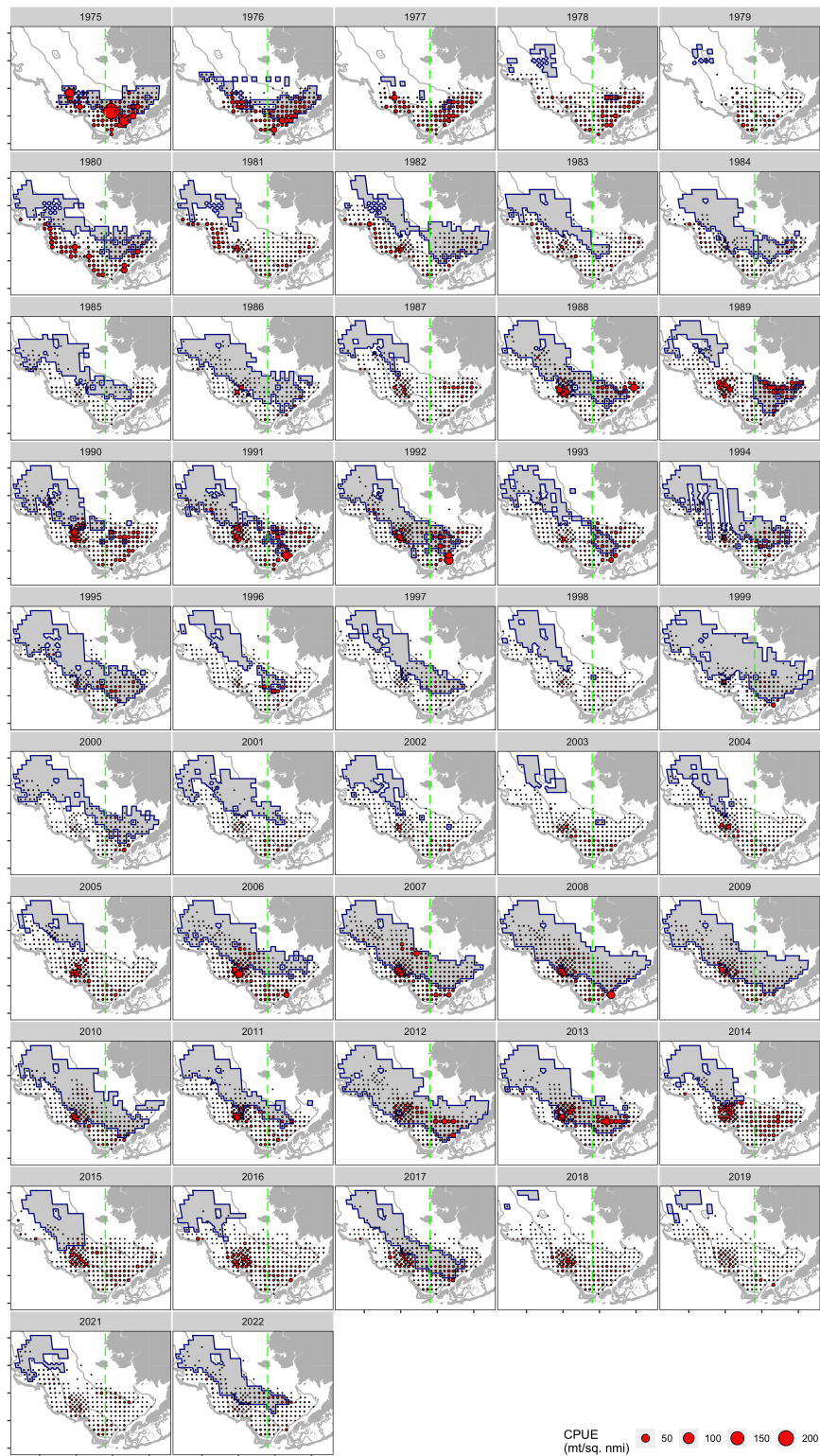
Figure 2: CPUE of large males (> 60 mm CW) in the NMFS EBS survey.
