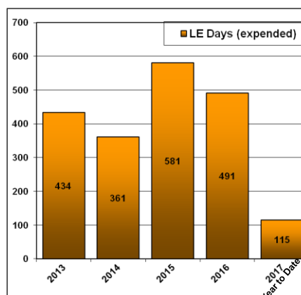
Annual Major Cutter Days
