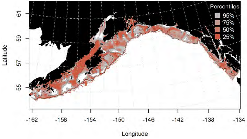
Figure 125. -- Predicted summer essential fish habitat for G. chalcogrammus juveniles and adults (top and bottom panel, respectively) from summer bottom trawl surveys.
