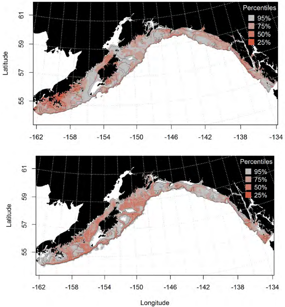
Figure 180. -- Predicted summer essential fish habitat for H. bolini juveniles and adults (top and bottom panel, respectively) from summer bottom trawl surveys.
