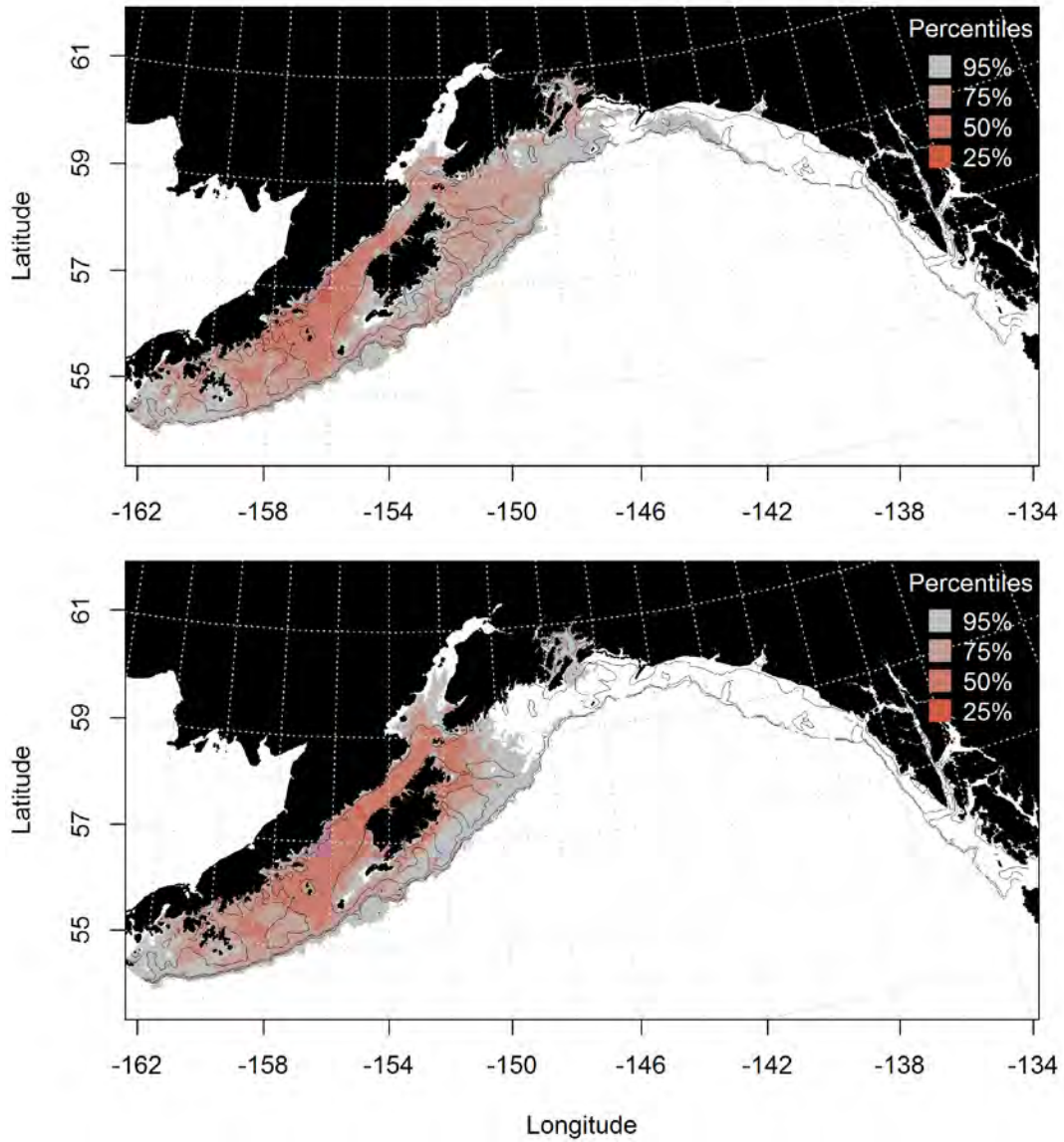
Figure 109. -- Spring, and summer essential fish habitat predicted for larval R. hippoglossoides (top and bottom panel, respectively) from the EcoFOCI database.
