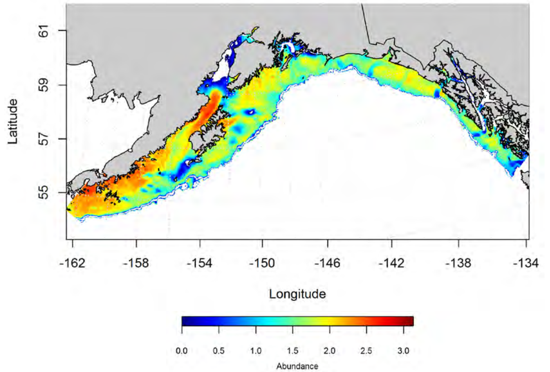
Figure 10. -- Best-fitting generalized additive model (GAM) effects of retained habitat variables on abundance ( \text{kg} \cdot \text{ha}^{-1} ) of juvenile A. stomias from summer bottom trawl surveys of the Gulf of Alaska slope and shelf (left panel) alongside GAM-predicted juvenile A. stomias abundance (right panel).
