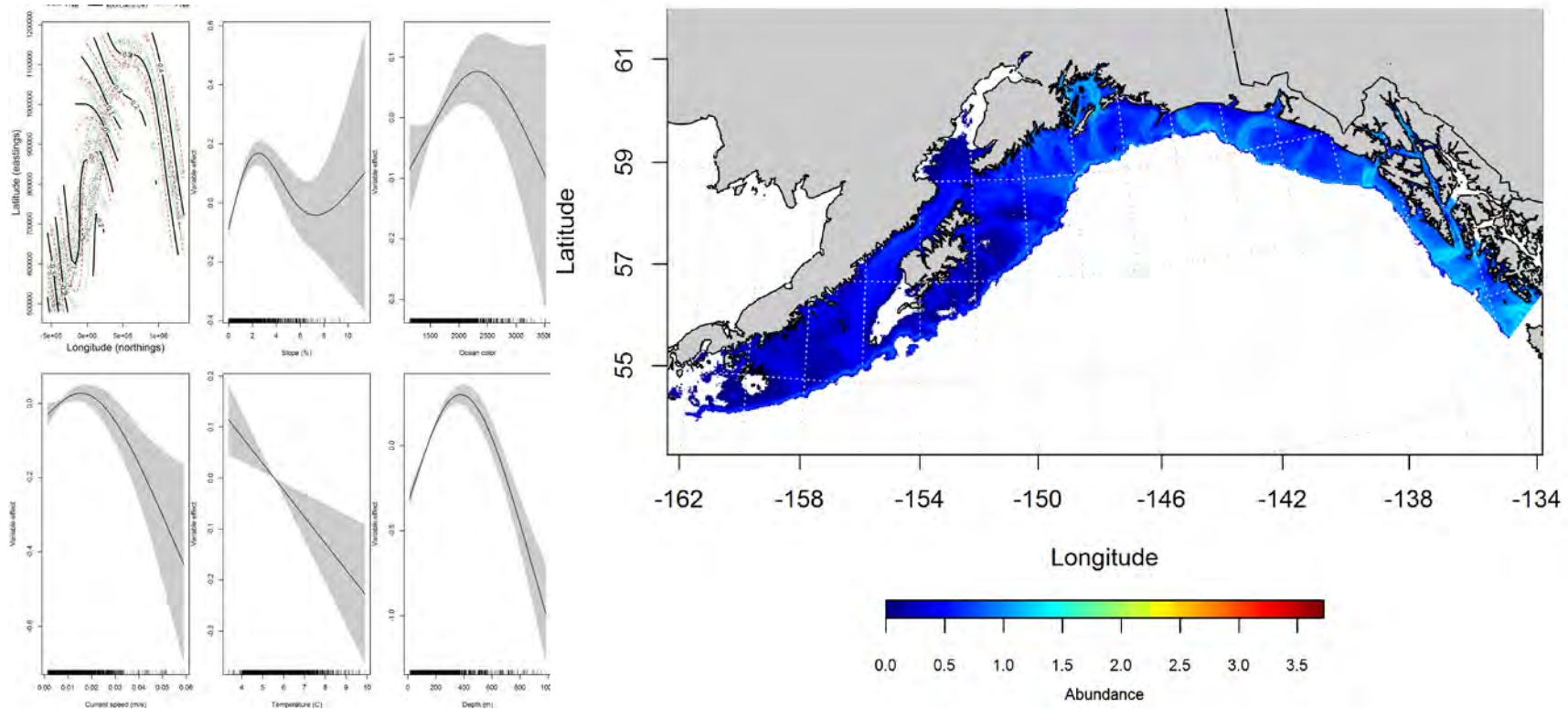
Figure 40. -- Best-fitting generalized additive model (GAM) effects of retained habitat variables on abundance ( \text{kg}\cdot\text{ha}^{-1} ) of juvenile M. pacificus from summer bottom trawl surveys of the Gulf of Alaska slope and shelf (left panel) alongside GAM-predicted juvenile M. pacificus abundance (right panel).
