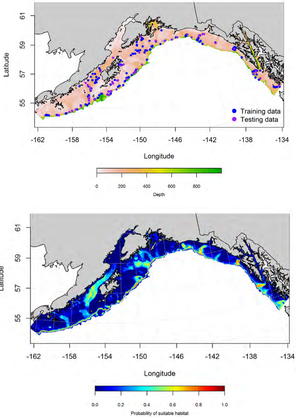
Figure 201. -- Locations of trawl survey catches of adult S. aleutianus (top panel). Blue points were used to train the maximum entropy model predicting the probability of the distribution of adult S. aleutianus based on trawl survey catches (bottom panel) and the purple points were used to test the model.
