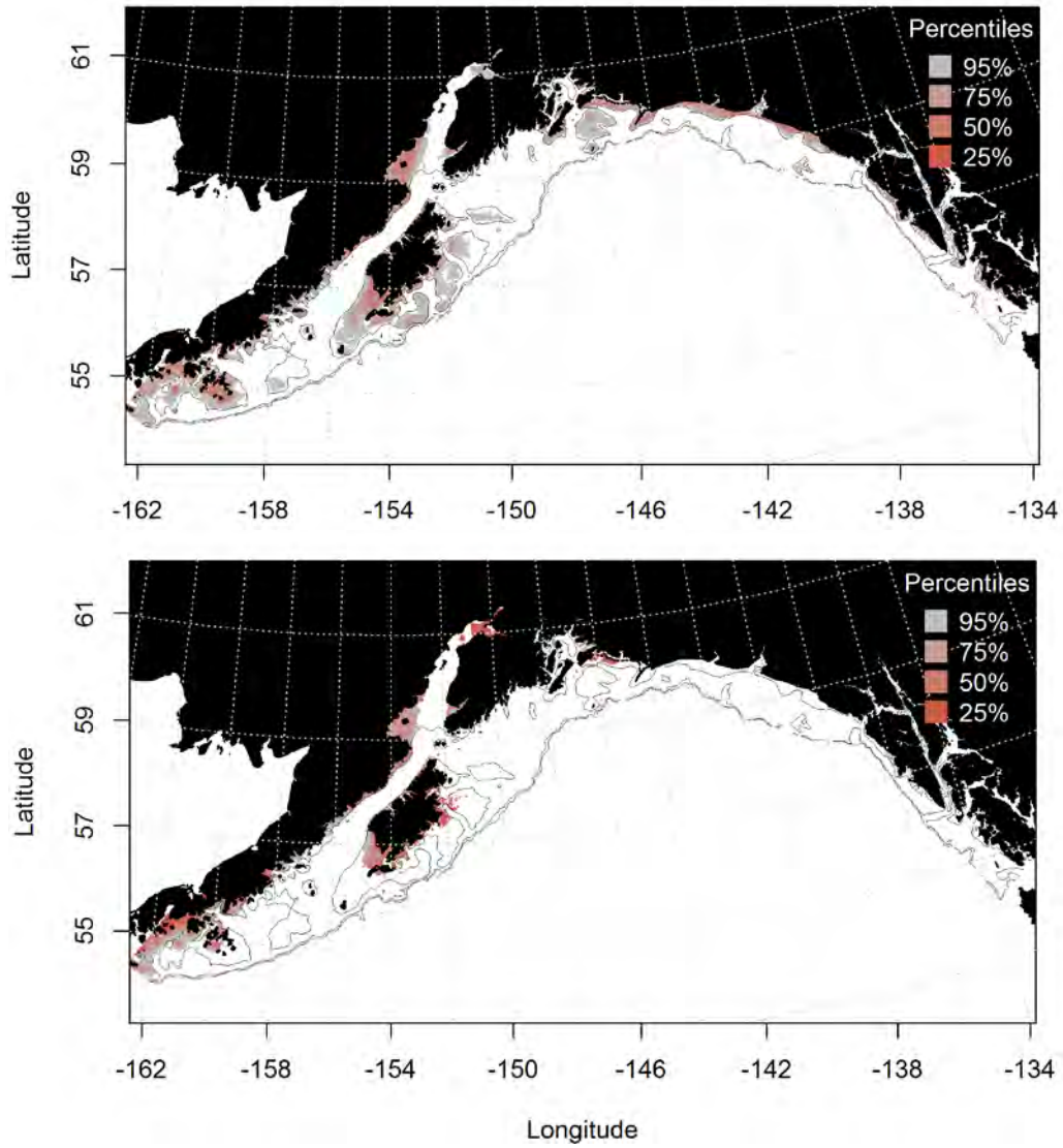
Figure 72. -- Predicted summer essential fish habitat for L. aspera juveniles and adults (top and bottom panel, respectively) from summer bottom trawl surveys.
