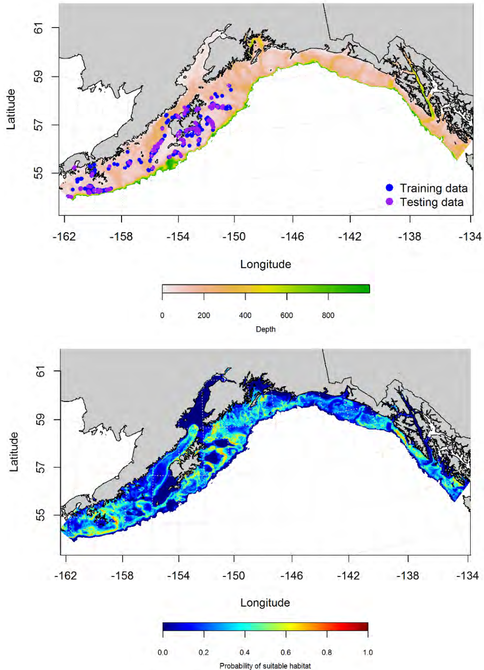
Figure 120. -- Locations of fall (September-November) commercial fisheries catches of G. chalcogrammus (top panel). Blue points were used to train the maximum entropy model predicting the probability of the fall distribution of G. chalcogrammus commercial catches (bottom panel) and the purple points were used to test the model.
