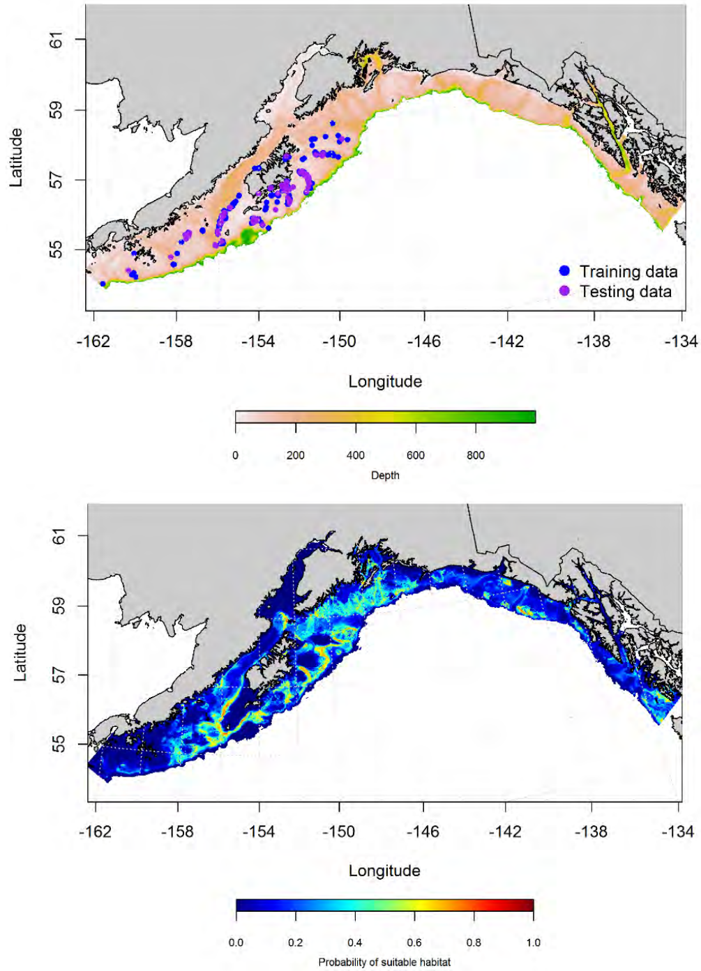
Figure 28. -- Locations of fall (September-November) commercial fisheries catches of G. zachirus (top panel). Blue points were used to train the maximum entropy model predicting the probability of the fall distribution of G. zachirus commercial catches (bottom panel) and the purple points were used to test the model.
