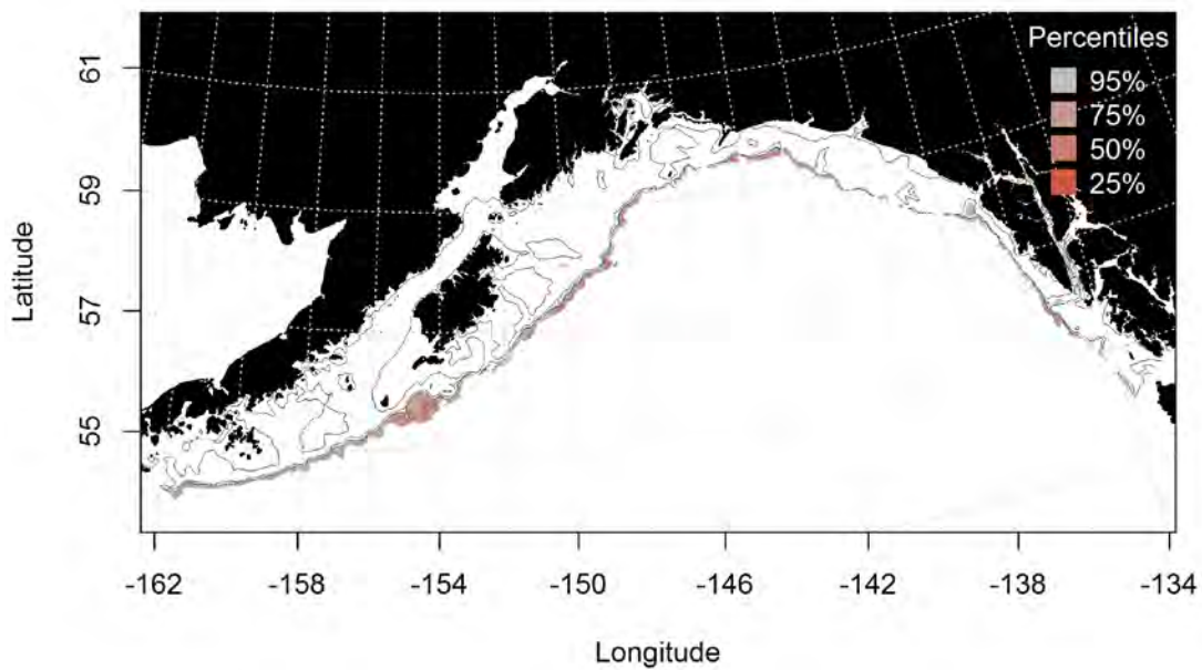
Figure 194. -- Predicted summer essential fish habitat for S. altivelis all life stages combined from summer bottom trawl surveys.
