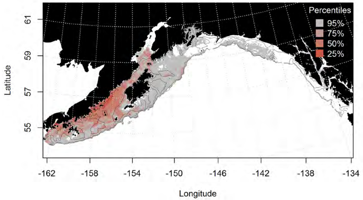
Figure 179. -- Spring essential fish habitat predicted for larval Hemitripteridae from the EcoFOCI database.
