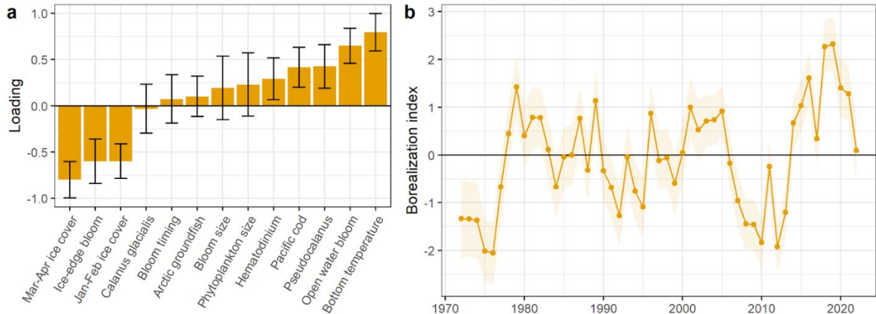
Figure 3-7 An index of borealization (the transition from Arctic to subarctic conditions) in the southeast BS, 1972-2022. a) Loadings for thirteen physical and biological time series onto a shared trend identified using Dynamic Factor Analysis (DFA). Time series with negative loadings are associated with more Arctic conditions, time series with positive loadings are associated with more subarctic conditions, and time series with 95% confidence intervals that include 0 cannot be assigned to either state. b) Borealization index, defined as the shared trend from the DFA model (estimate with 95% confidence interval). Negative values indicate more Arctic conditions, positive values indicate more subarctic conditions.
