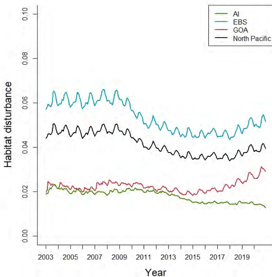
Figure 4. A time-series output of the Fishing Effects Model showing habitat disturbance aggregated for all areas less than 1000 m depth for the Aleutian Islands, Eastern Bering Sea, Gulf of Alaska, and the North Pacific at large.
