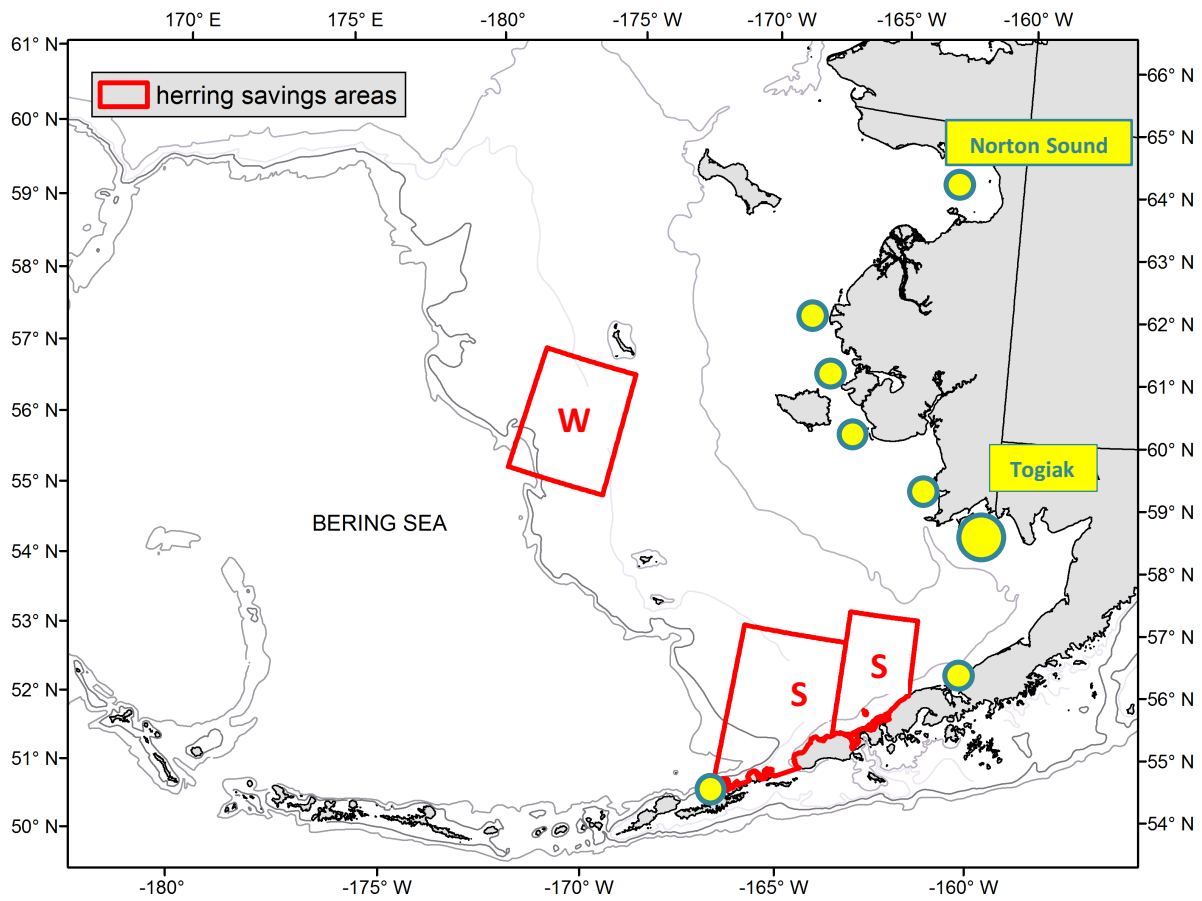
Figure 1. Locations of Pacific herring fisheries in the BSAI (yellow dots) and Herring Savings Areas (red-outlined polygons). Red letting indicates seasonality of Savings Areas: W = winter, S = summer. The two largest herring fisheries are labeled by name; the larger dot at Togiak indicates that this is the largest herring fishery in the BSAI.
