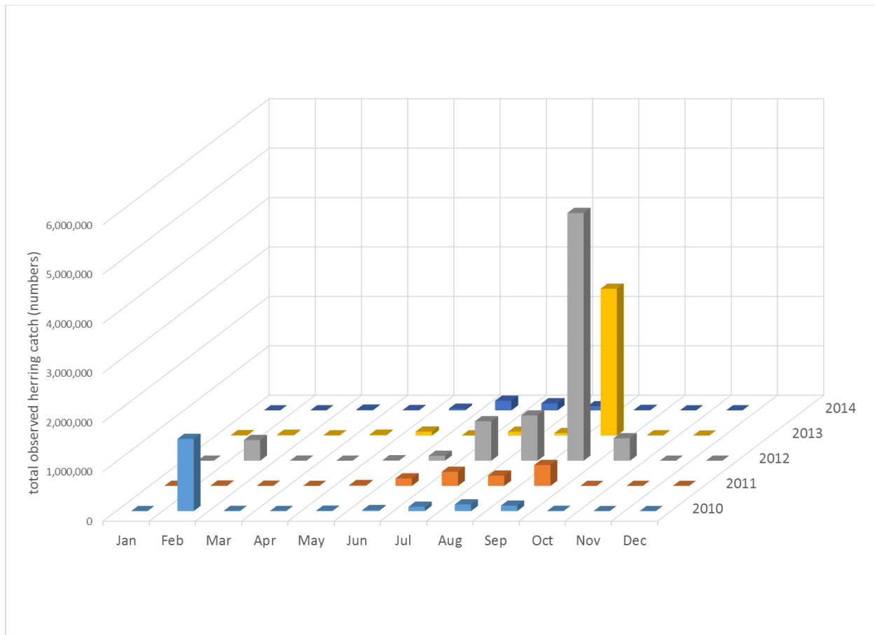
Figure 31. Seasonal patterns of observed Pacific herring catches in federal fisheries in the BSAI, 2010-2014.
