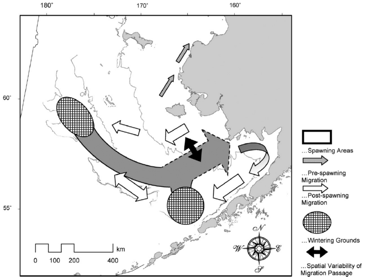
Figure 2. Hypothesized migration routes and seasonal distributions of Pacific herring in the EBS. Figure is from Tojo et al. 2007.
