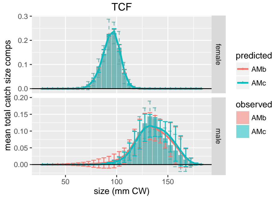
Figure 148. Comparison of observed and predicted &times mean total catch size comps for TCF.
