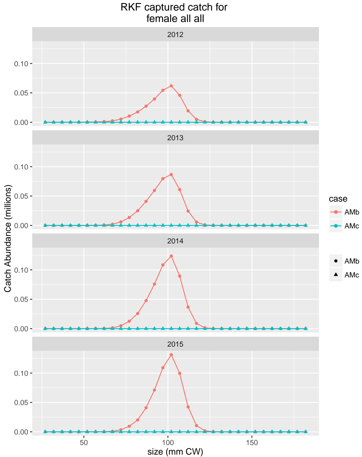
Figure 94. Predicted RKF captured catch abundance for female all all, (5 of 5).
