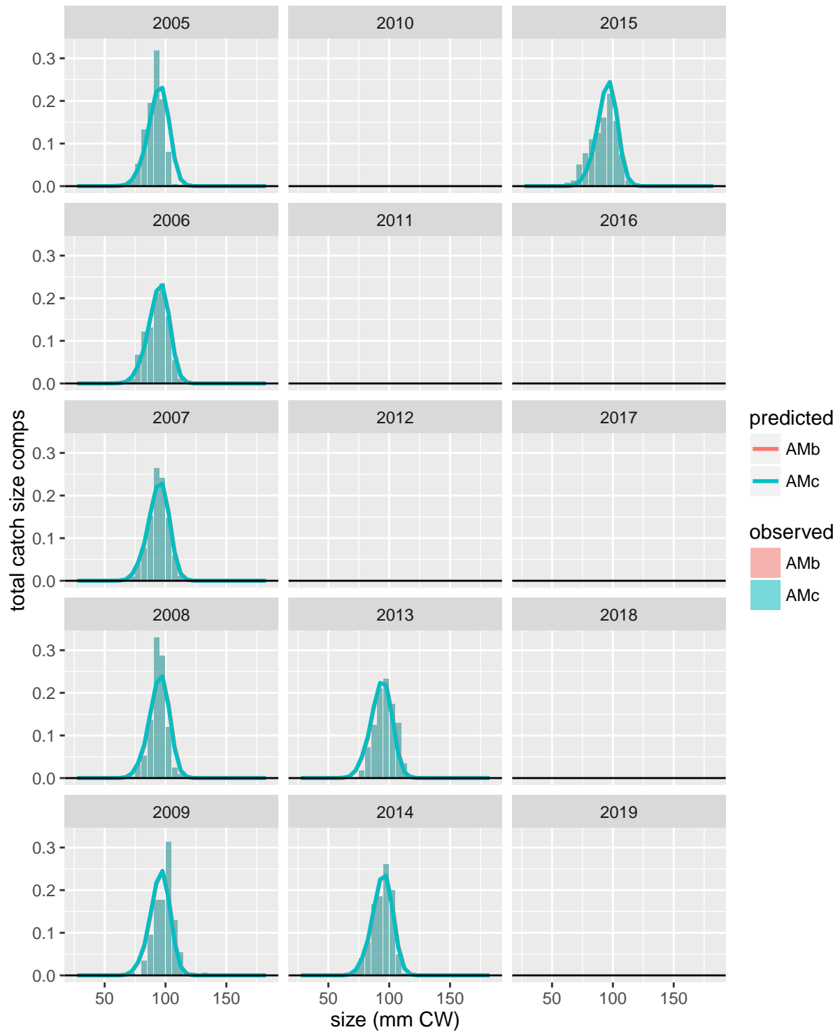
Figure 152. Comparison of observed and predicted female, all maturity, all shell total catch size comps for TCF. Page 2 of 2.
