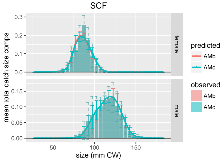
Figure 147. Comparison of observed and predicted &times mean total catch size comps for SCF.
