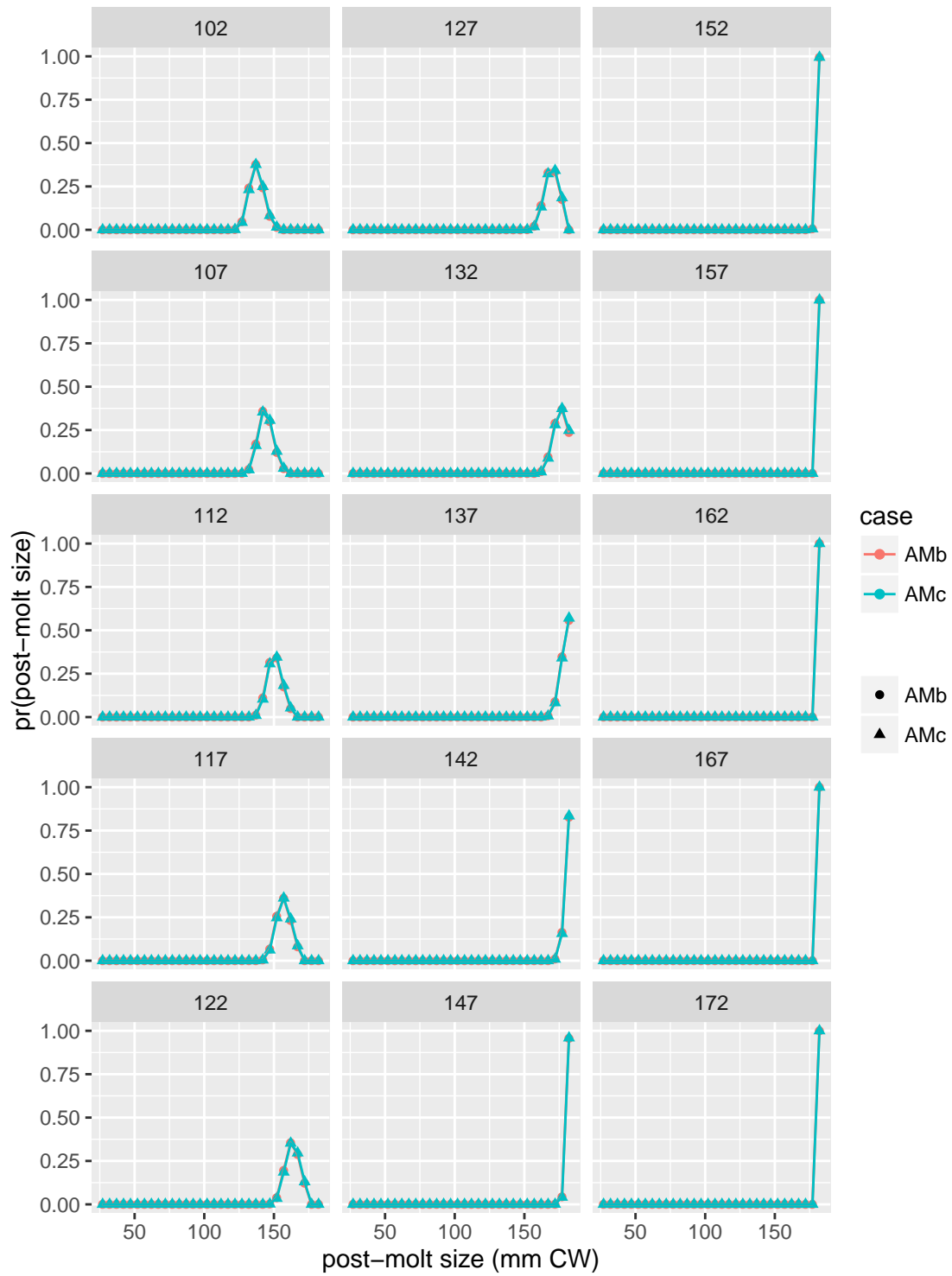
Figure 5. Growth matrices for males during 1949-2016, page 2.
