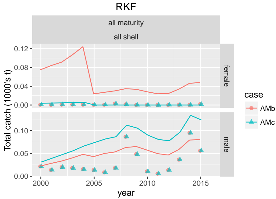
Figure 142. Comparison of observed and predicted total catch for RKF. Recent time period.
