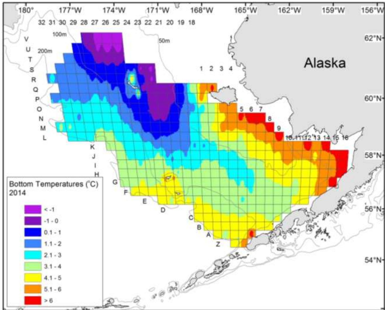
Figure 5. Bottom temperatures (°C) measured at stations from the National Marine Fisheries Service eastern Bering Sea bottom trawl survey, beginning 8 June 2014 in Bristol Bay and ending on 2 August 2014 at the western edge of the survey.
