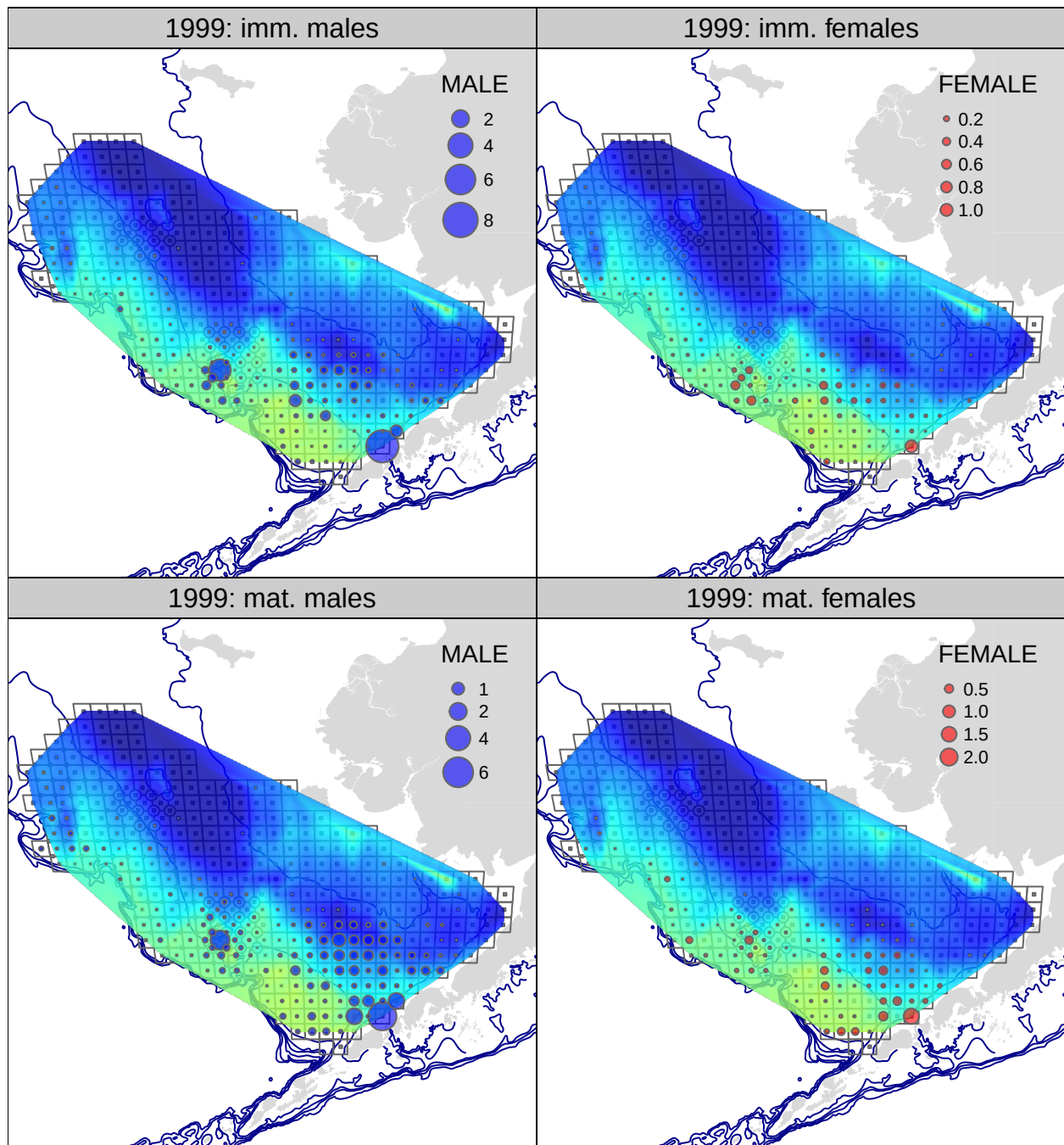
Figure 26: Tanner crab CPUE (biomass) from the 1999 NMFS EBS bottom trawl survey. upper row: immature crab; lower row: mature crab; lefthand column: males; righthand column: females.
