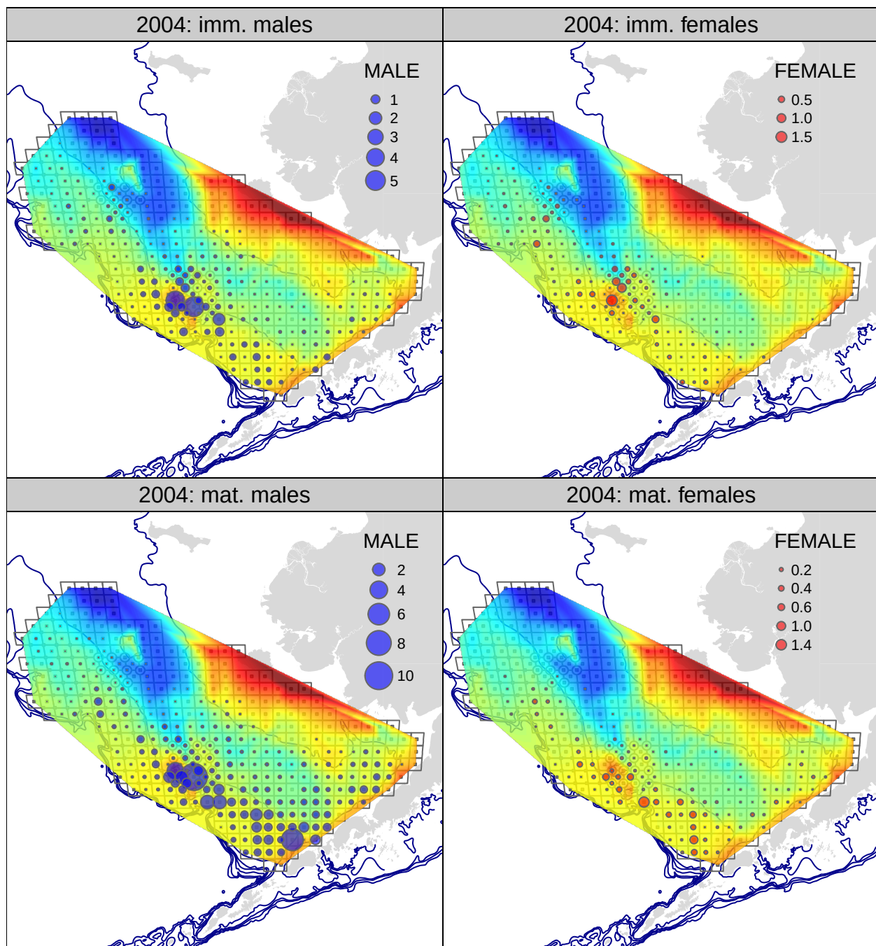
Figure 31: Tanner crab CPUE (biomass) from the 2004 NMFS EBS bottom trawl survey. upper row: immature crab; lower row: mature crab; lefthand column: males; righthand column: females.
