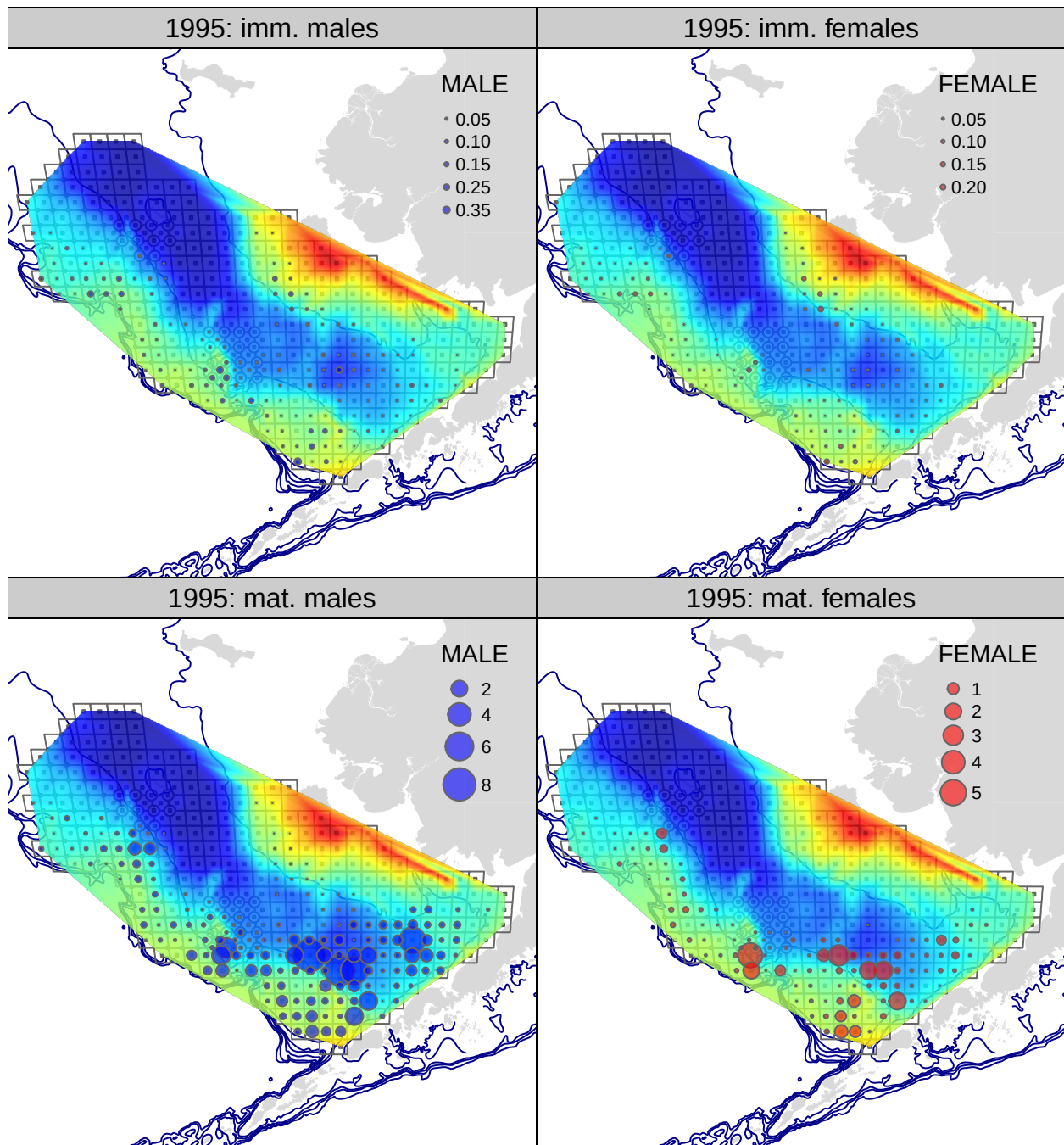
Figure 22: Tanner crab CPUE (biomass) from the 1995 NMFS EBS bottom trawl survey. upper row: immature crab; lower row: mature crab; lefthand column: males; righthand column: females.
