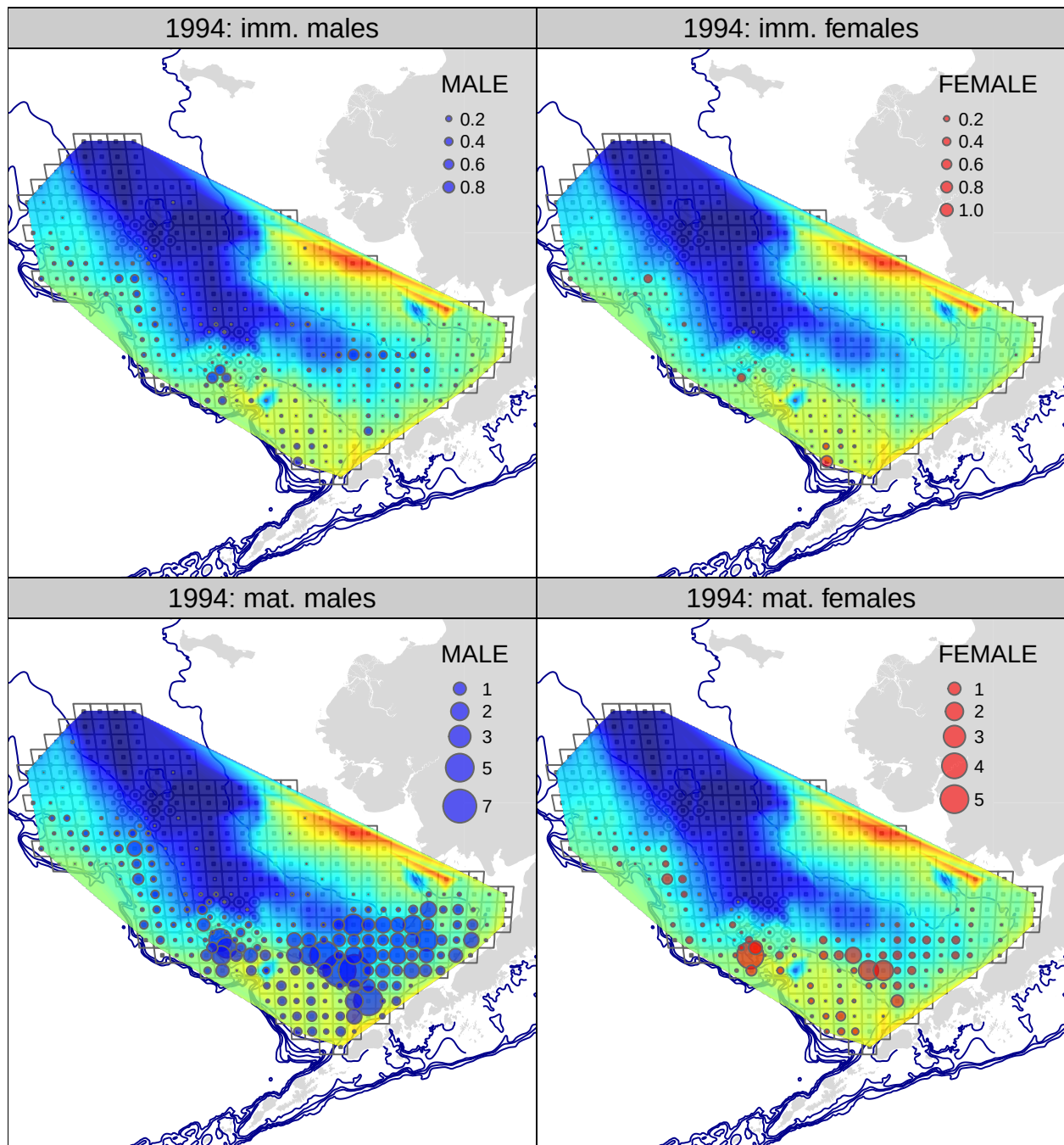
Figure 21: Tanner crab CPUE (biomass) from the 1994 NMFS EBS bottom trawl survey. upper row: immature crab; lower row: mature crab; lefthand column: males; righthand column: females.
