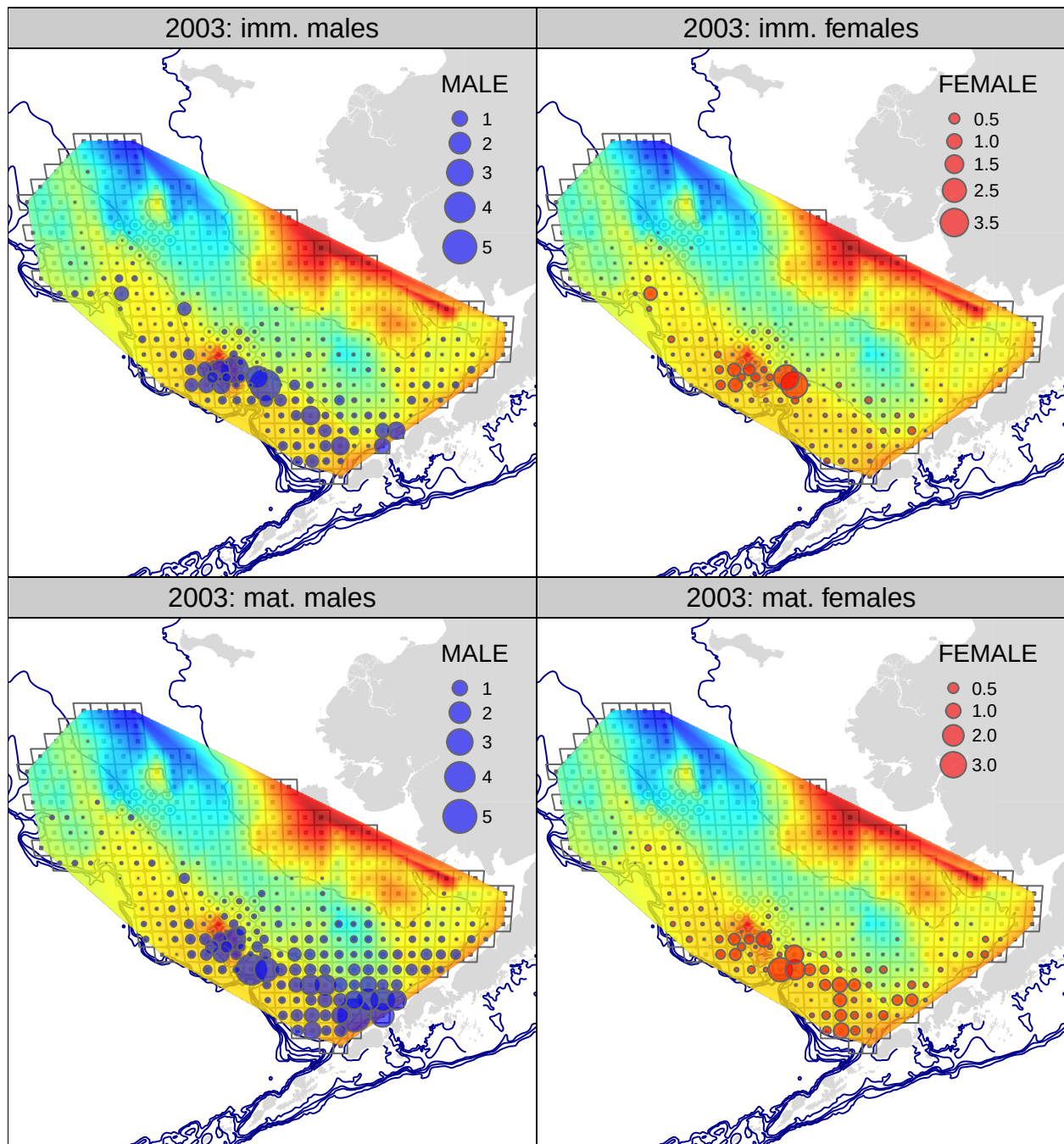
Figure 30: Tanner crab CPUE (biomass) from the 2003 NMFS EBS bottom trawl survey. upper row: immature crab; lower row: mature crab; lefthand column: males; righthand column: females.
