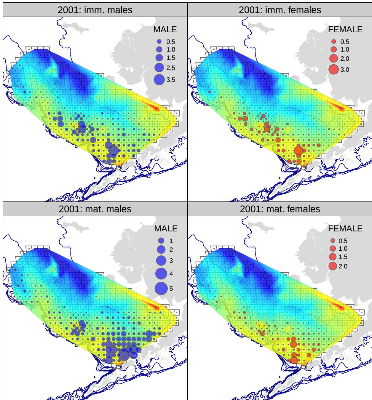
Figure 28: Tanner crab CPUE (biomass) from the 2001 NMFS EBS bottom trawl survey. upper row: immature crab; lower row: mature crab; lefthand column: males; righthand column: females.
