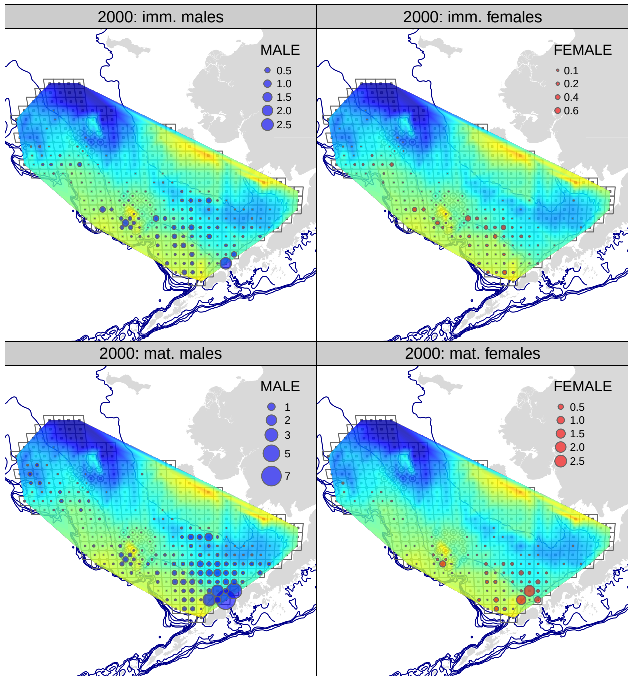
Figure 27: Tanner crab CPUE (biomass) from the 2000 NMFS EBS bottom trawl survey. upper row: immature crab; lower row: mature crab; lefthand column: males; righthand column: females.
