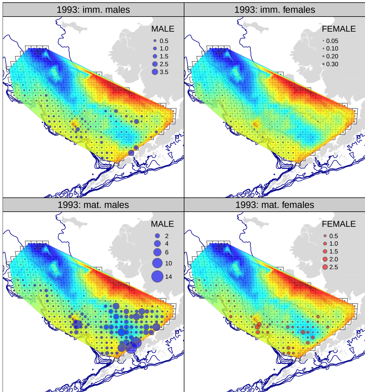
Figure 20: Tanner crab CPUE (biomass) from the 1993 NMFS EBS bottom trawl survey. upper row: immature crab; lower row: mature crab; lefthand column: males; righthand column: females.
