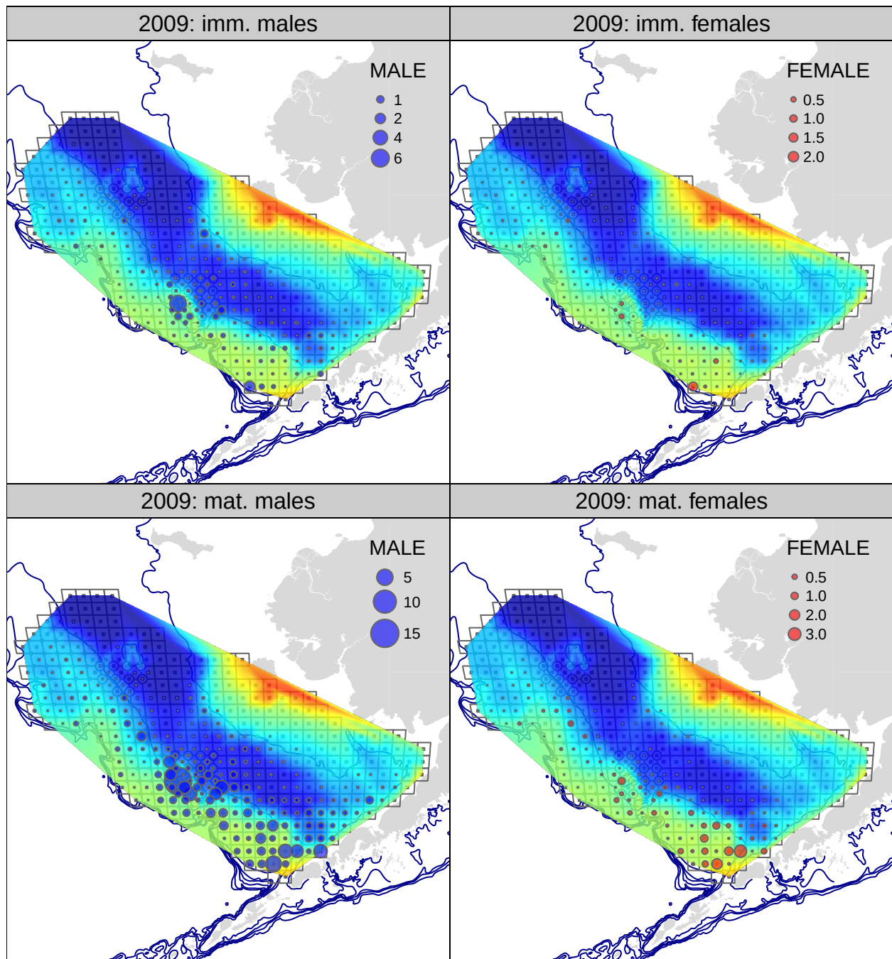
Figure 36: Tanner crab CPUE (biomass) from the 2009 NMFS EBS bottom trawl survey. upper row: immature crab; lower row: mature crab; lefthand column: males; righthand column: females.
