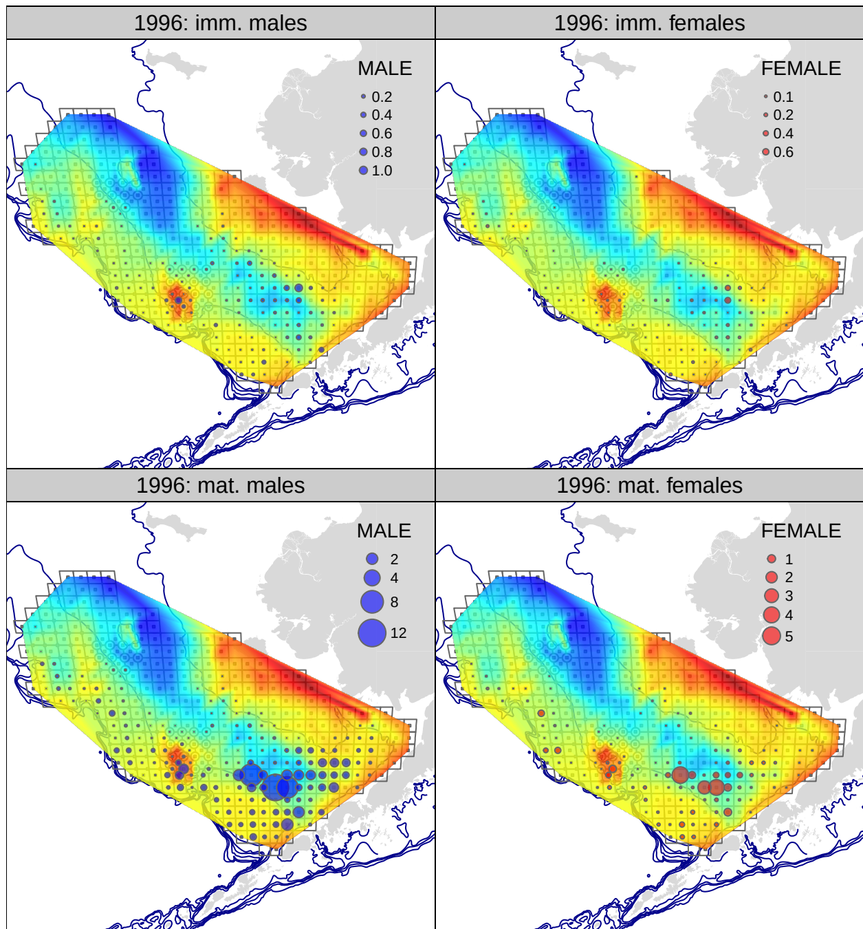
Figure 23: Tanner crab CPUE (biomass) from the 1996 NMFS EBS bottom trawl survey. upper row: immature crab; lower row: mature crab; lefthand column: males; righthand column: females.
