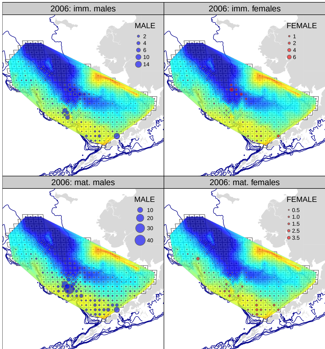
Figure 33: Tanner crab CPUE (biomass) from the 2006 NMFS EBS bottom trawl survey. upper row: immature crab; lower row: mature crab; lefthand column: males; righthand column: females.
