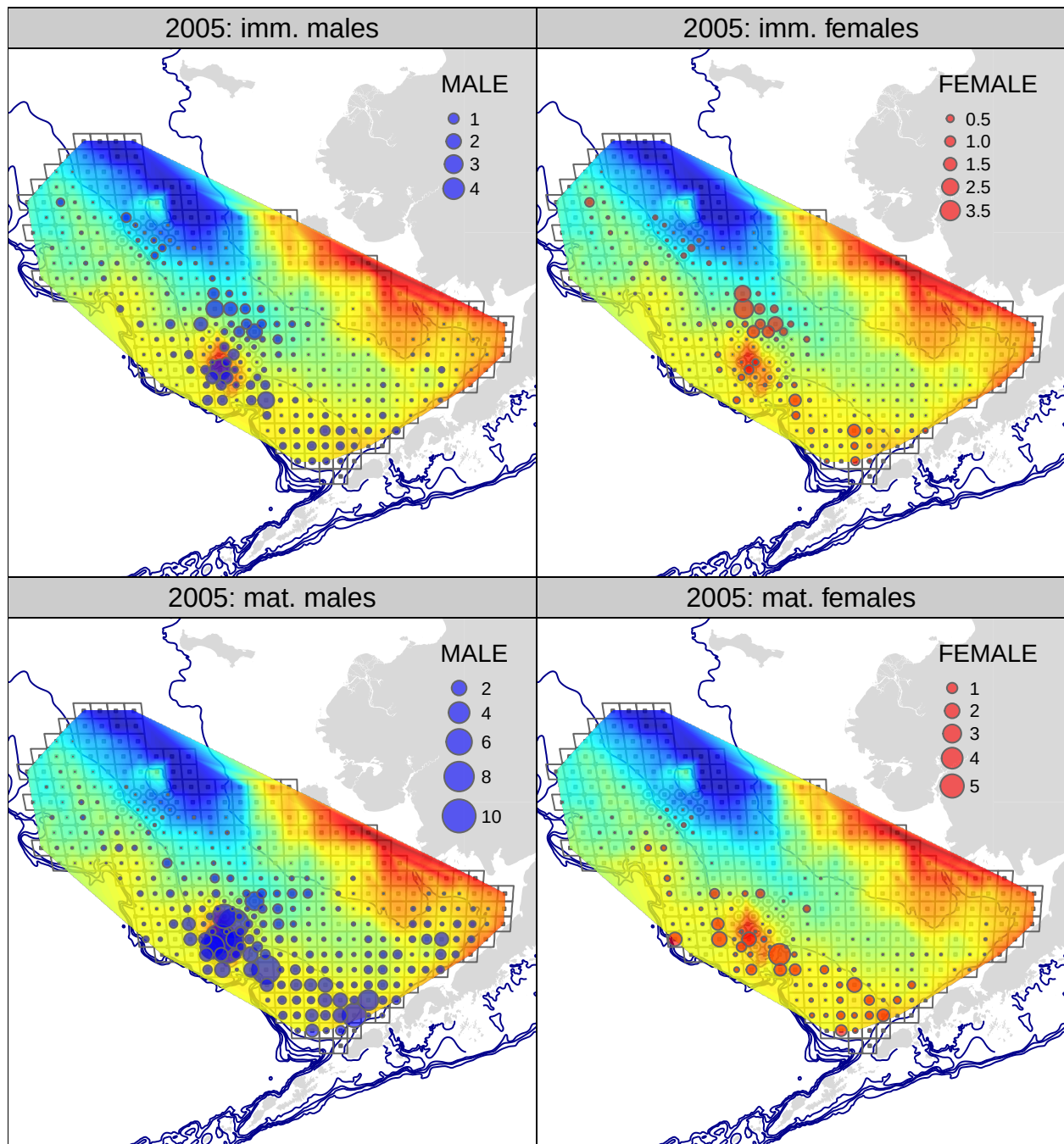
Figure 32: Tanner crab CPUE (biomass) from the 2005 NMFS EBS bottom trawl survey. upper row: immature crab; lower row: mature crab; lefthand column: males; righthand column: females.
