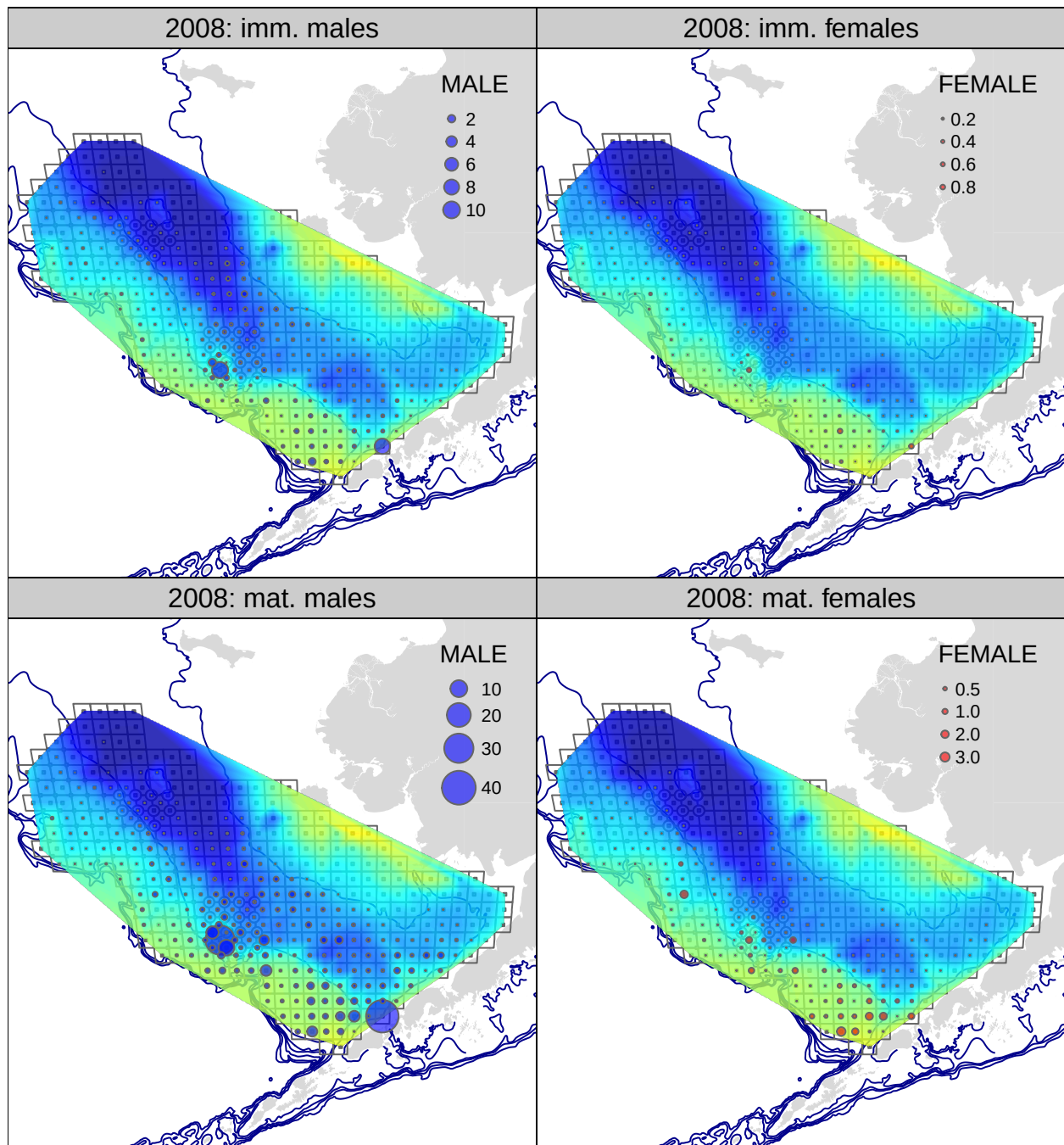
Figure 35: Tanner crab CPUE (biomass) from the 2008 NMFS EBS bottom trawl survey. upper row: immature crab; lower row: mature crab; lefthand column: males; righthand column: females.
