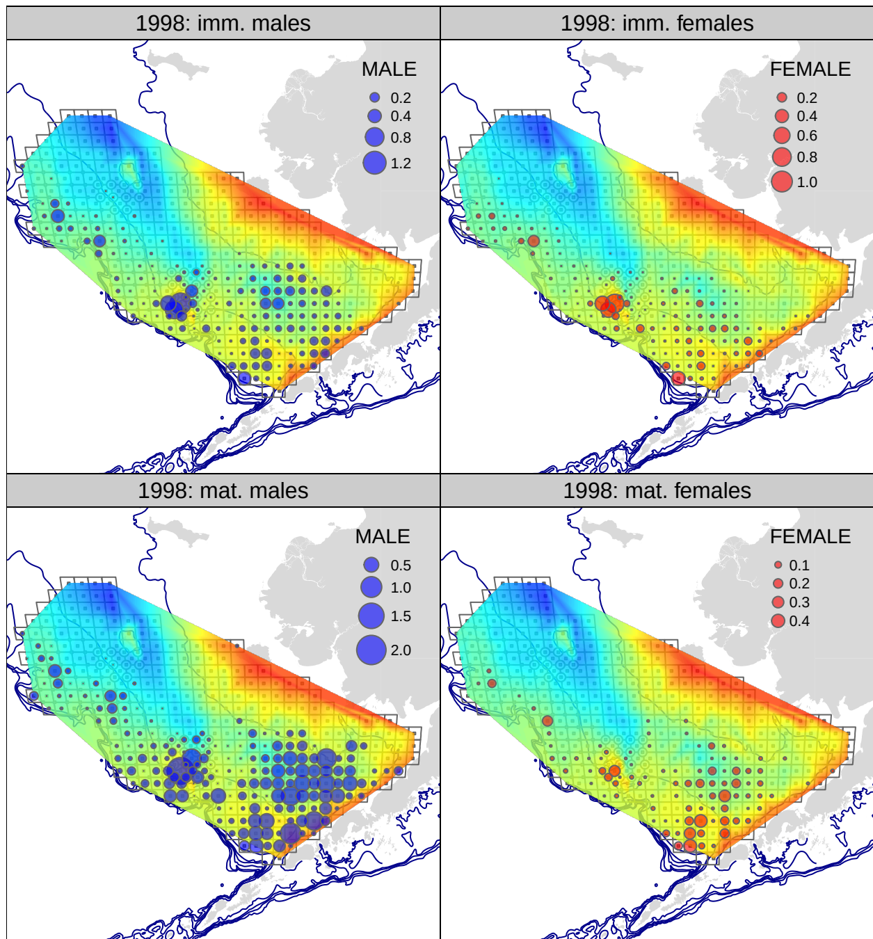
Figure 25: Tanner crab CPUE (biomass) from the 1998 NMFS EBS bottom trawl survey. upper row: immature crab; lower row: mature crab; lefthand column: males; righthand column: females.
