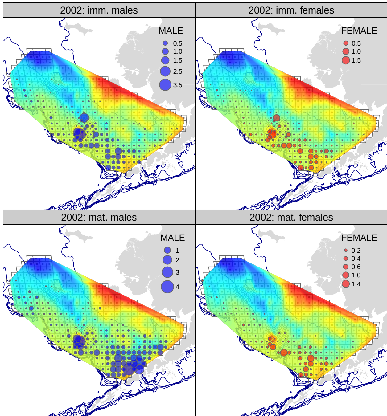
Figure 29: Tanner crab CPUE (biomass) from the 2002 NMFS EBS bottom trawl survey. upper row: immature crab; lower row: mature crab; lefthand column: males; righthand column: females.
