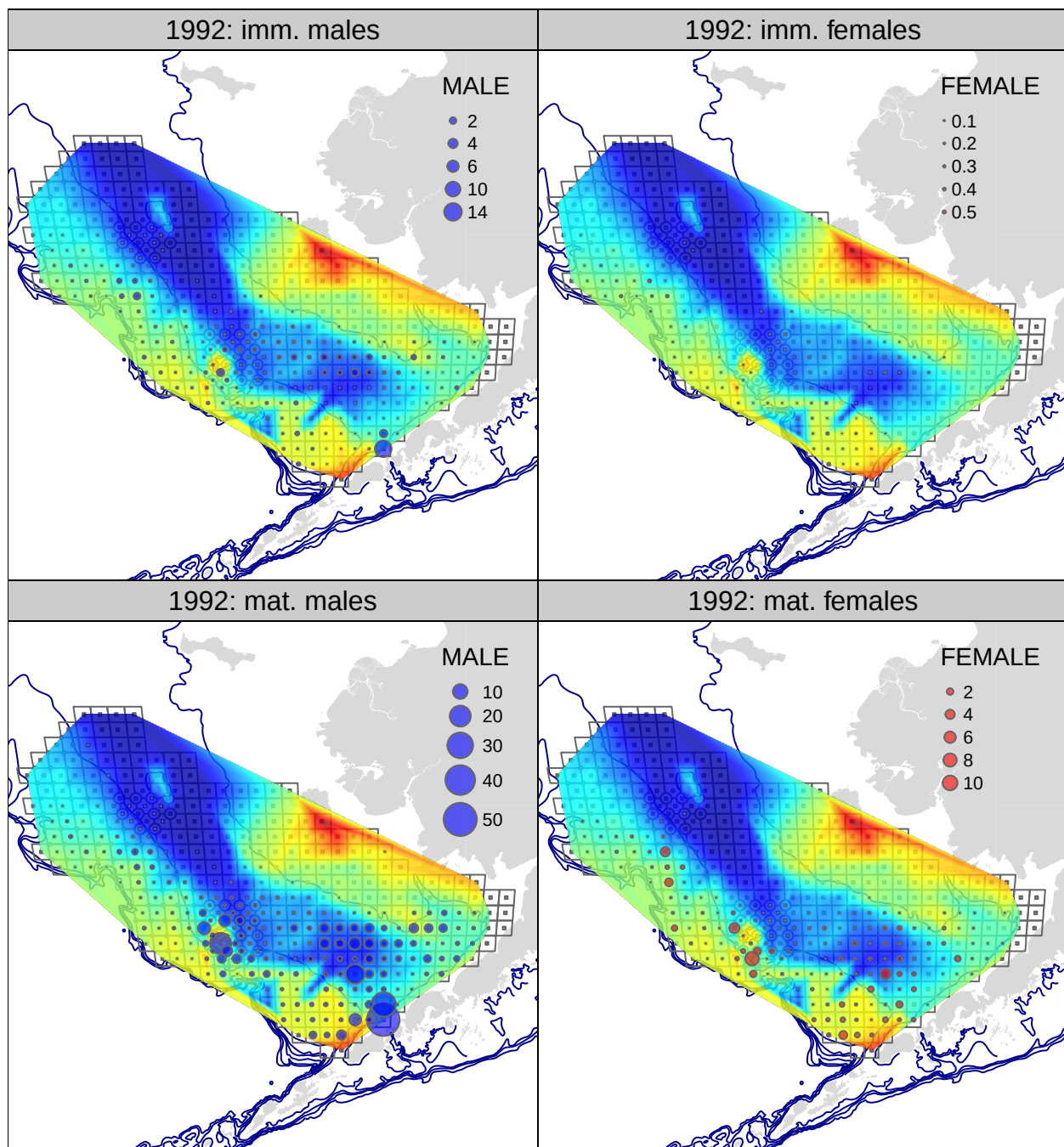
Figure 19: Tanner crab CPUE (biomass) from the 1992 NMFS EBS bottom trawl survey. upper row: immature crab; lower row: mature crab; lefthand column: males; righthand column: females.
