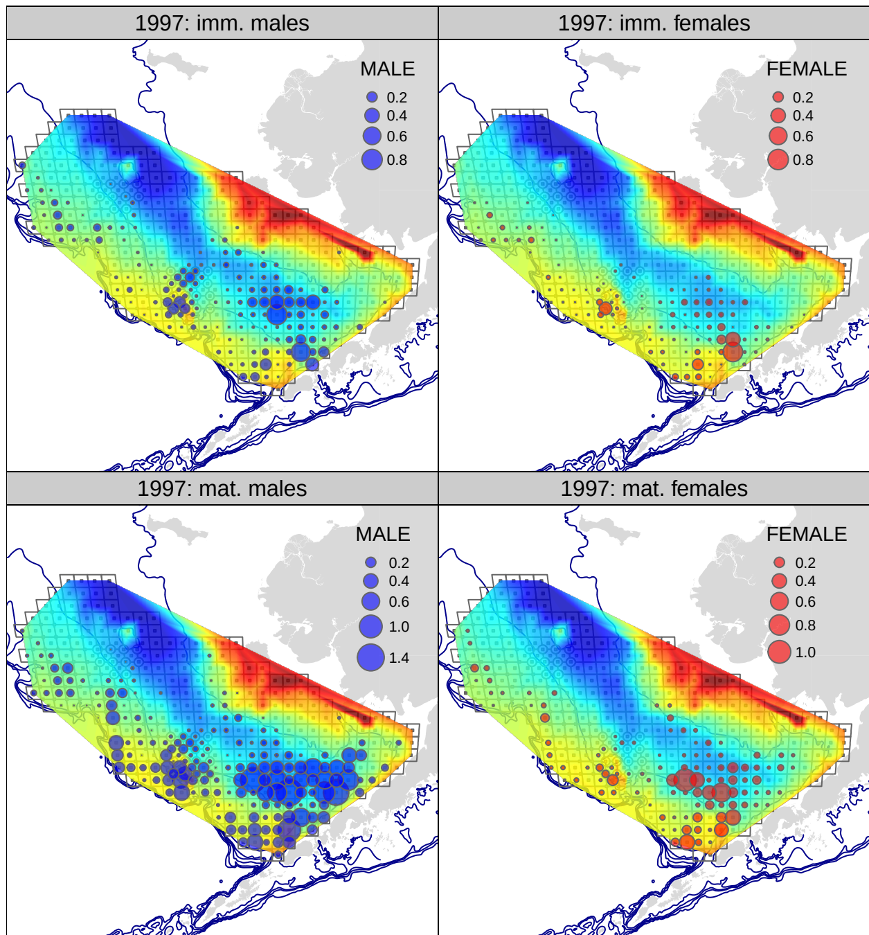
Figure 24: Tanner crab CPUE (biomass) from the 1997 NMFS EBS bottom trawl survey. upper row: immature crab; lower row: mature crab; lefthand column: males; righthand column: females.
