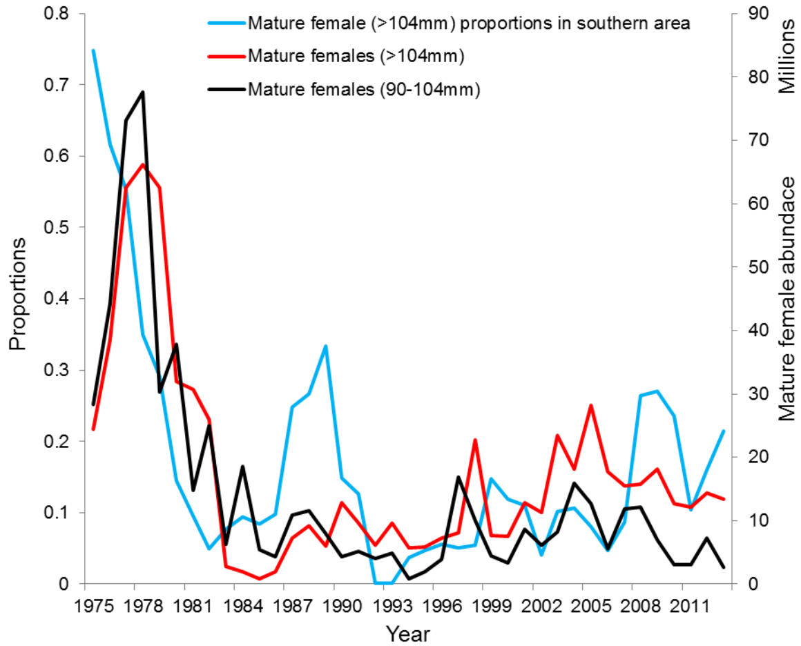
Fig. C8. Proportions (3-point-moving average) in southern Bristol Bay (<math>56^{\circ}\text{N}</math>) for mature females (>104 mm carapace length) and mature female red king crab abundances during 1975-2013 from the summer trawl surveys.
