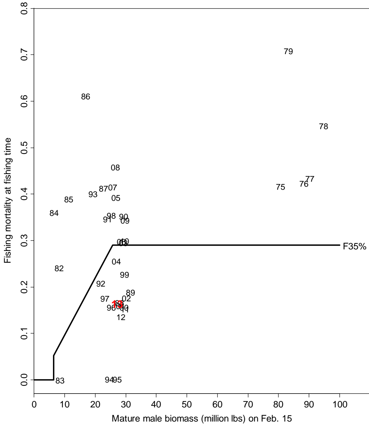
Figure 12(4na). Relationships between full fishing mortalities for the directed pot fishery and mature male biomass on Feb. 15 during 1975-2013 under scenario 4na. Average of recruitment from 1984 to 2014 was used to estimate B_{MSY} . Pot and trawl handling mortality rates were assumed to be 0.2 and 0.8, respectively.
