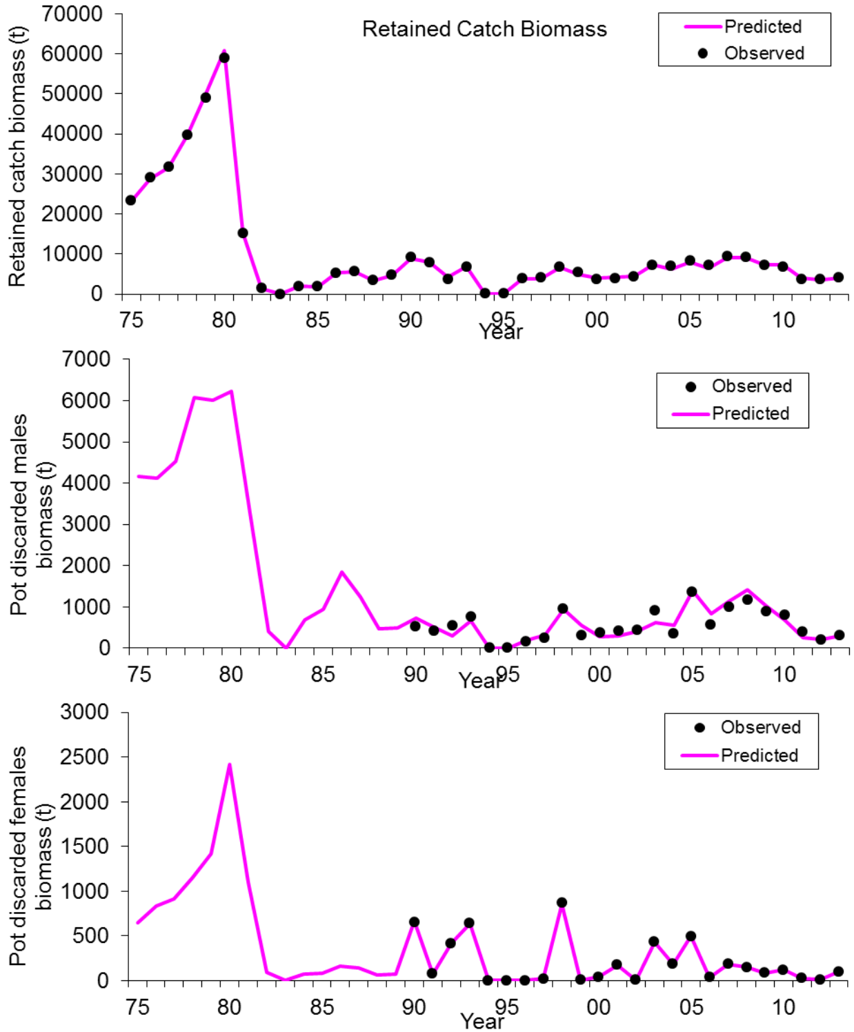
Figure 15a(4nb). Observed and predicted catch mortality biomass under scenario 4nb. Mortality biomass is equal to caught biomass times a handling mortality rate. Pot handling mortality rate is 0.2.
