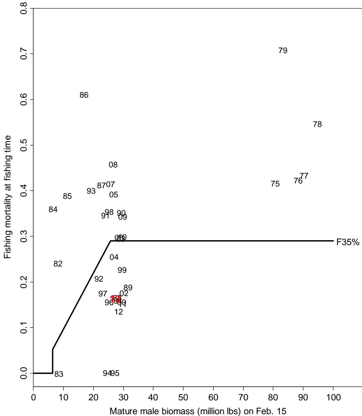
Figure 12(4nb). Relationships between full fishing mortalities for the directed pot fishery and mature male biomass on Feb. 15 during 1975-2013 under scenario 4nb. Average of recruitment from 1984 to 2014 was used to estimate B_{MSY} . Pot and trawl handling mortality rates were assumed to be 0.2 and 0.8, respectively.
