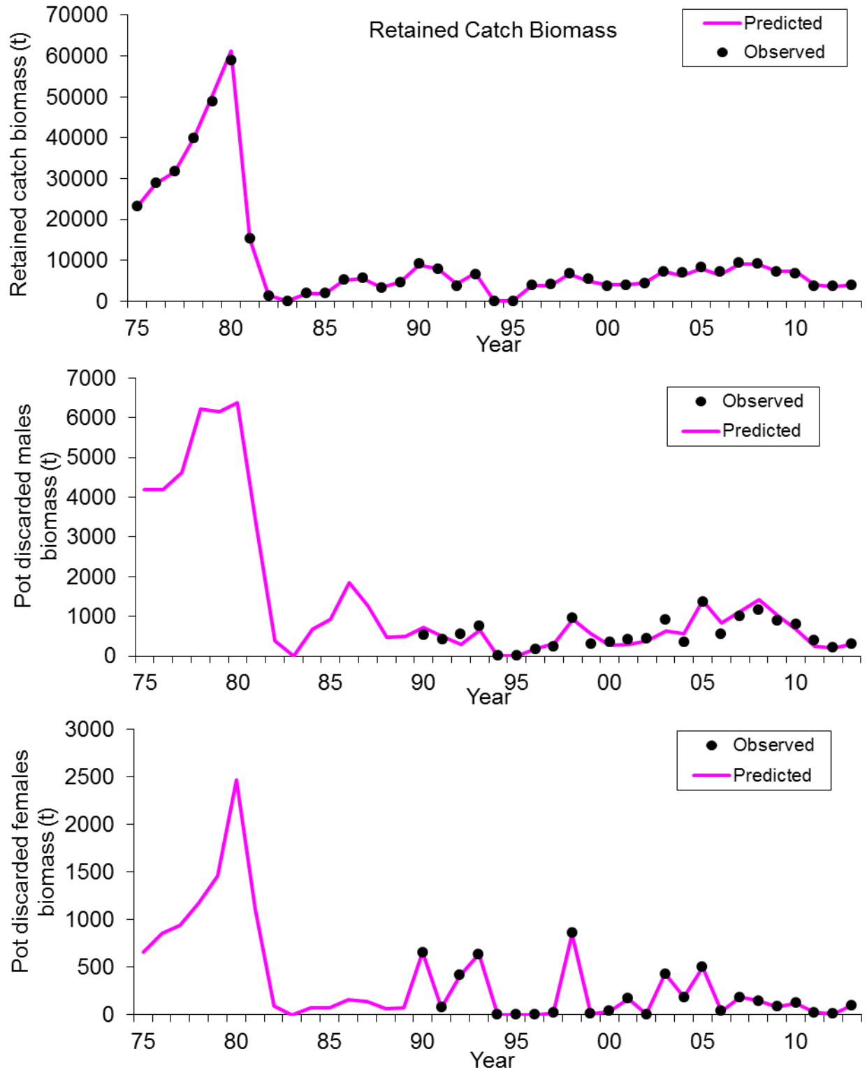
Figure 15a(4na). Observed and predicted catch mortality biomass under scenario 4na. Mortality biomass is equal to caught biomass times a handling mortality rate. Pot handling mortality rate is 0.2.
