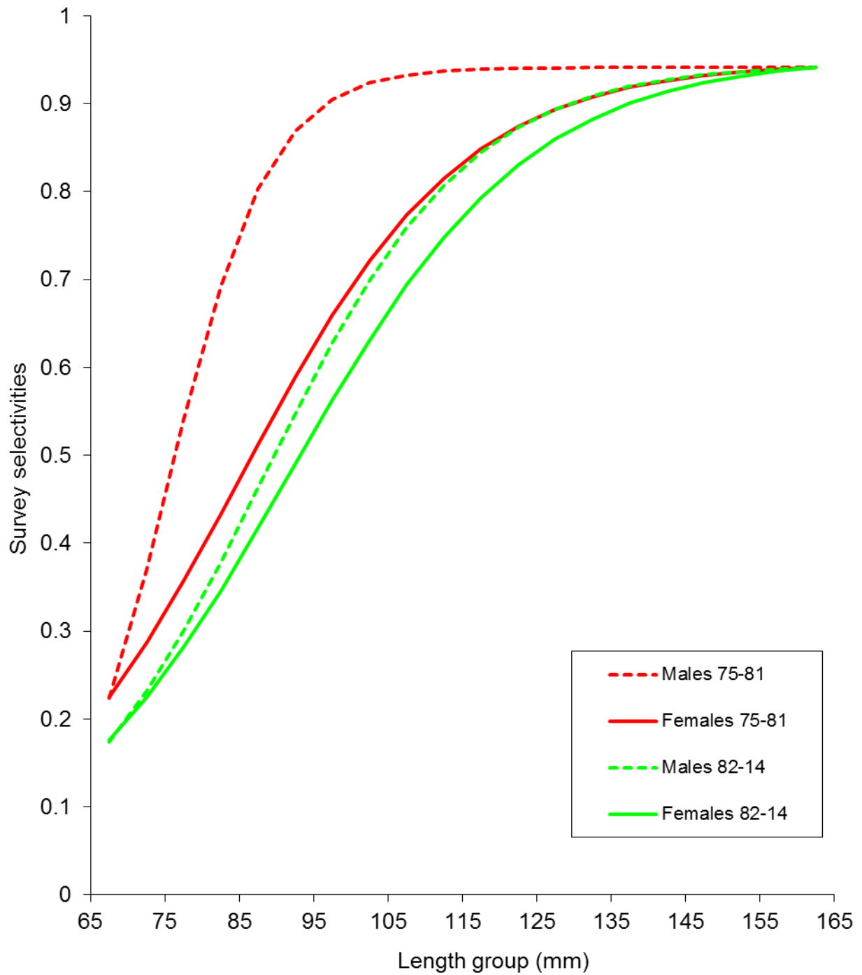
Figure 8a(4nb). Estimated trawl survey selectivities under scenario 4nb. Pot and trawl handling mortality rates were assumed to be 0.2 and 0.8, respectively.
