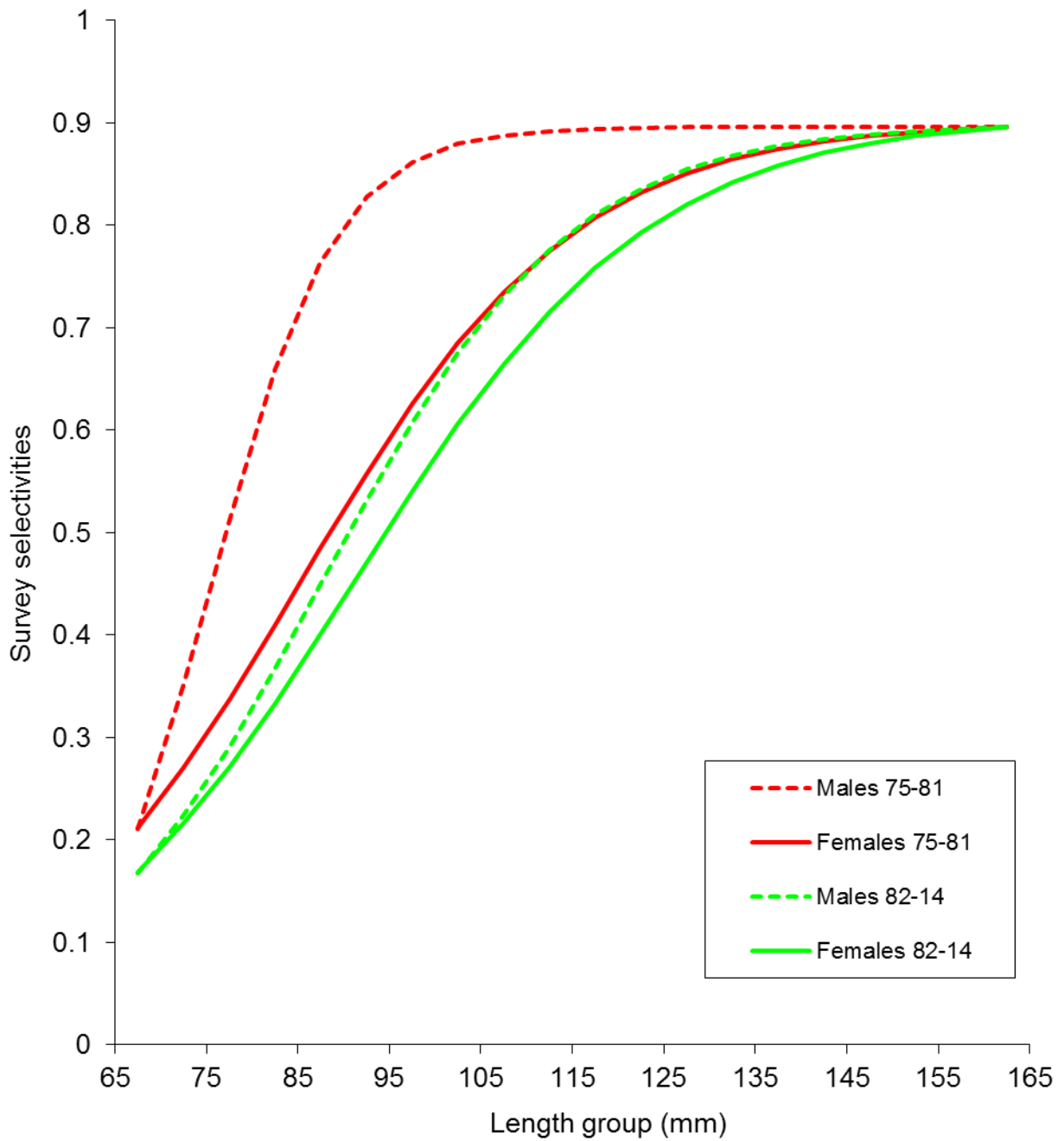
Figure 8a(4na). Estimated trawl survey selectivities under scenario 4na. Pot and trawl handling mortality rates were assumed to be 0.2 and 0.8, respectively.
