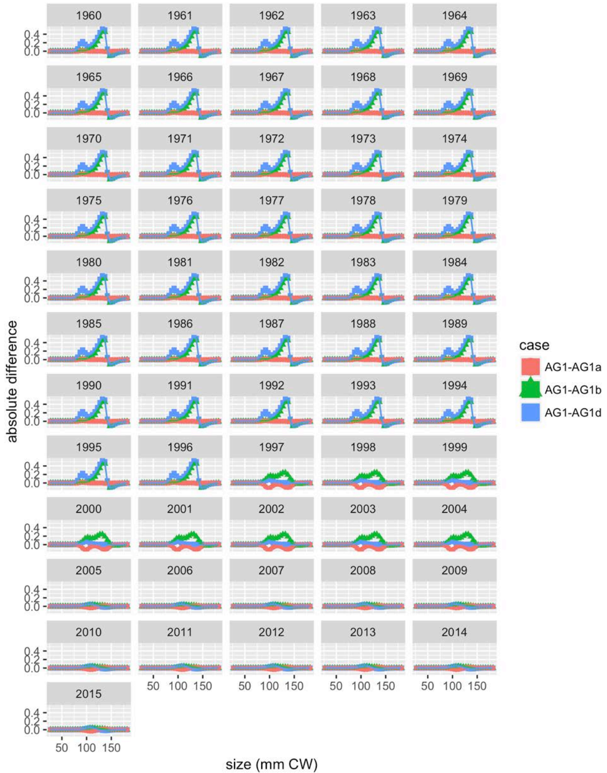
Figure 68. Differences for SCF males: fishery selectivity.
