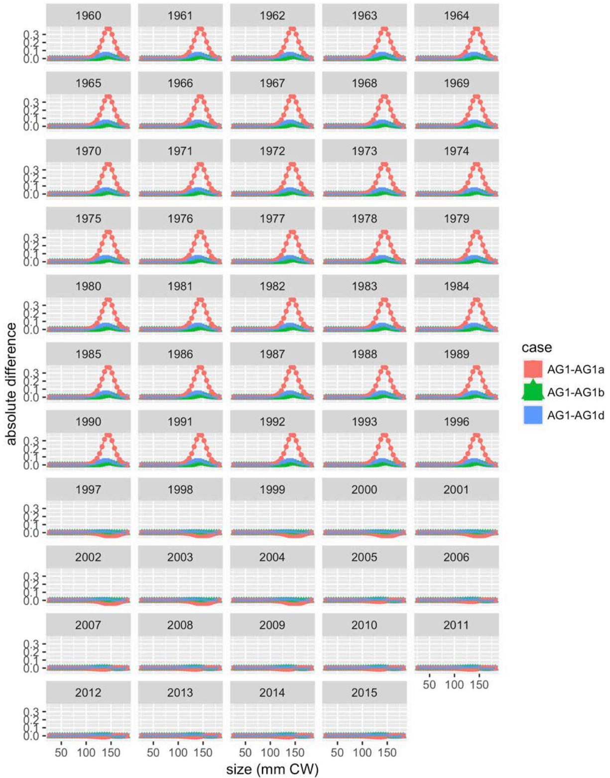
Figure 76. Differences for RKF males: fishery selectivity.
