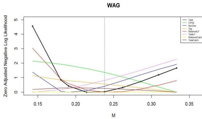
Figure 2. Total and components negative log-likelihoods vs. M for scenario 1c model fit without M penalty for WAG . Top left: WAG data with a minimum (vertical bar) at M = 0.2232 \text{ yr}^{-1} ; top right: M profiles for the WAG portion of the EAG and WAG combined likelihood including the fish ticket CPUE likelihood with a minimum at M = 0.2472 \text{ yr}^{-1} ; bottom left: M profiles for the WAG portion of the EAG and WAG combined likelihood without fish ticket CPUE likelihood with a minimum at M = 0.2379 \text{ yr}^{-1} ; bottom right: WAG data with the dome shaped selectivity with a minimum at M = 0.2970 \text{ yr}^{-1} . The negative log likelihood values were zero adjusted.
