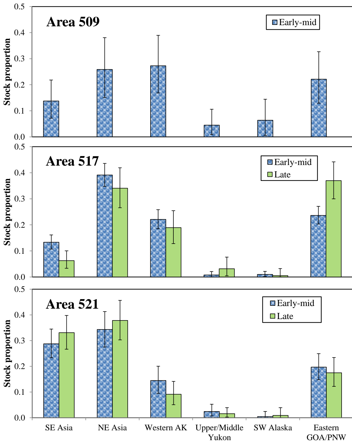
Figure 14. -- Stock composition estimates and 95% BAYES credible intervals for the 2014 chum salmon genetic samples from the NMFS reporting area 509 for the Early-Middle time period, and areas 517 and 521 for the Early-Middle and Late time periods (Table 8).
