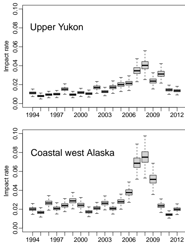
Figure 31. Estimated impact of the EBS pollock fishery on the Upper Yukon stock (top) and coastal west Alaska (which includes the “middle Yukon”; bottom), 1994-2012. Vertical axis is the ratio of AEQ over the point estimates of total run sizes.
