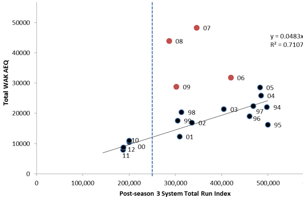
Figure 11. Relationship between post-season inriver run abundance of the 3 System Index and the bycatch AEQ attributed to all Western Alaska stocks (combined AEQ of CWAK, Upper Yukon and Middle Yukon). The 250,000 Chinook salmon reference point is indicated by the vertical line.
