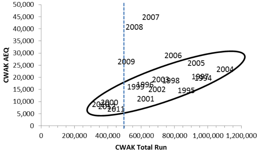
Figure 5. Relationship between the CWAK total run index estimate and bycatch AEQ for the CWAK reporting group. Those years showing a linear trend and not considered outliers are included in the ellipse ( Y=0.0227x , R^2 = 0.6739 ). The proposed threshold identified by the natural break in the data is shown by the vertical dotted line.
