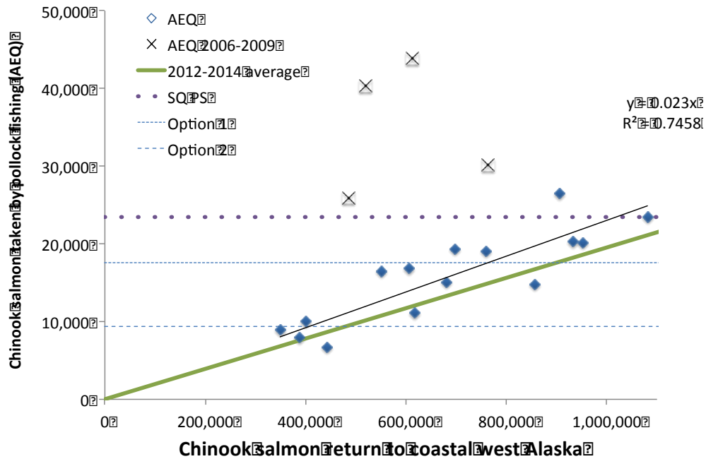
Figure 35. Relationship between in-river run abundance for coastal west Alaska and the bycatch AEQ values. Horizontal dotted lines represent the AEQ mapping of PSC for status quo performance standard (23,448 Chinook salmon in AEQ terms) and Alternative 5, options 1 and 2 (17,586 and 9,379 Chinook salmon in AEQ terms, respectively). The thick diagonal green line is the estimated impact post Amendment 91 (~2%) and the thin line is the estimate based on all years from 1994-2012 except 2006-2009.
