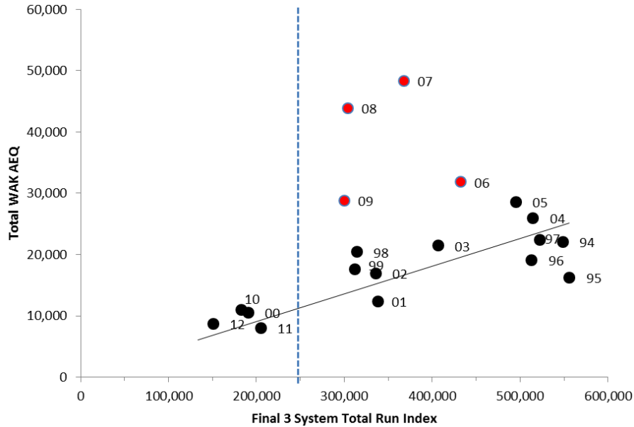
Figure 8. Relationship between final inriver run abundance of the 3 System Inriver Run Index and the bycatch AEQ attributed to all Western Alaska stocks (combined AEQ of CWAK, Upper Yukon and Middle Yukon) ( Y=0.0451x , R^2 = 0.570 ). The 250,000 Chinook salmon reference point is indicated by the vertical line.
