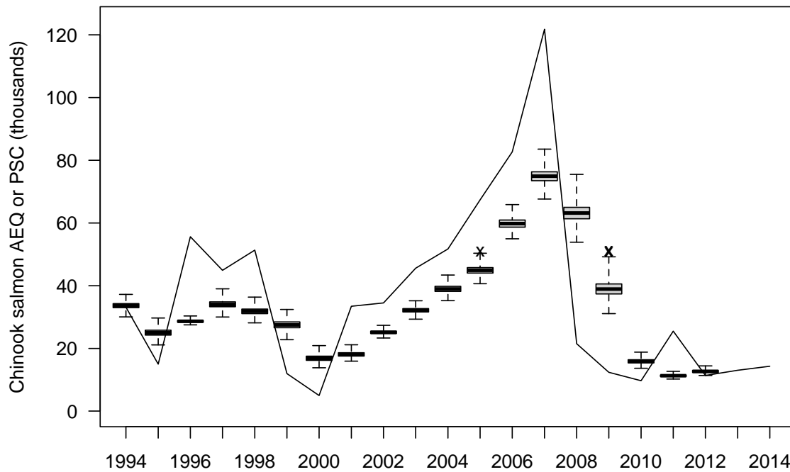
Figure 30. Estimated annual total adult equivalent (AEQ) mortality of Chinook salmon from the EBS pollock fishery, 1994-2012 (boxplots) and PSC (1994-2014). Units are numbers of salmon and height of boxes represent the uncertainty (inter-quartile ranges) due to oceanic survival and other factors that vary within the model. Horizontal lines within the boxes represent the medians of the posterior distribution. (From Ianelli and Stram 2014).
