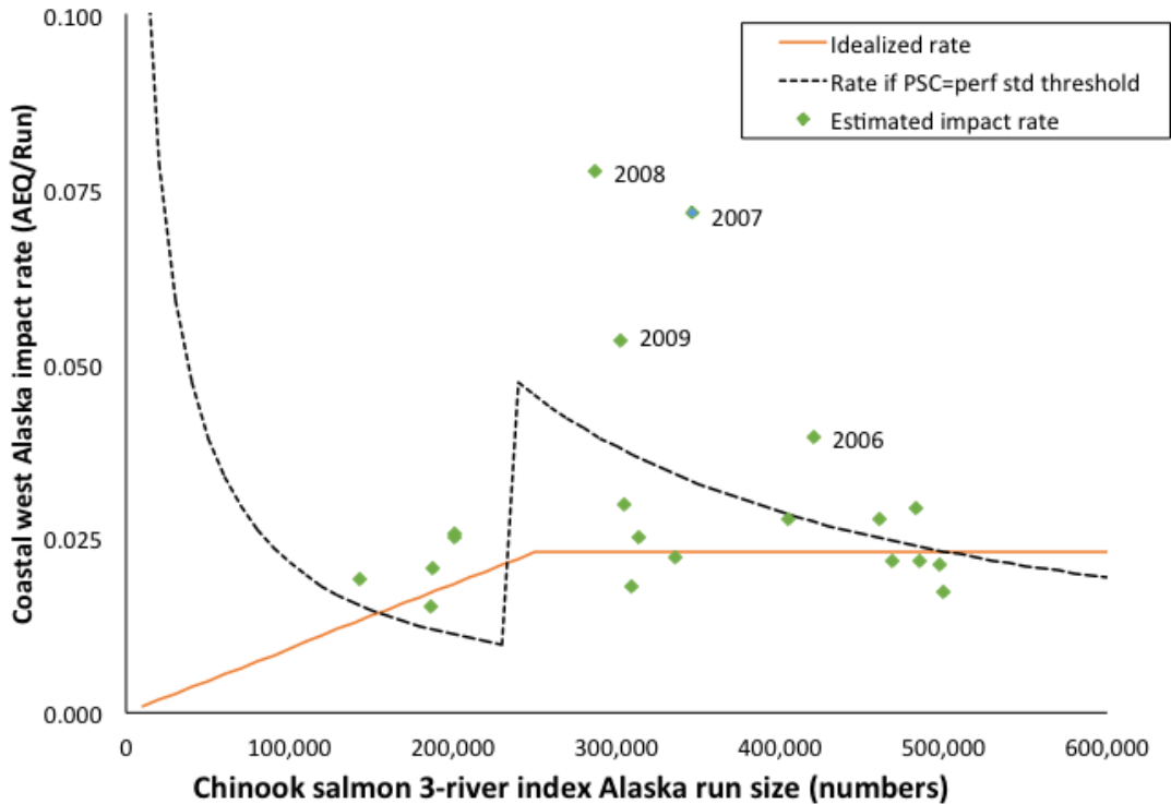
Figure 37. Estimated impact rate to coastal west Alaska stocks versus historical 3-river run index (points) compared with an “idealized” rate which decreased at low stock sizes (solid line) and an example of what the rate would look like if the performance standard threshold was reached (dashed line).
