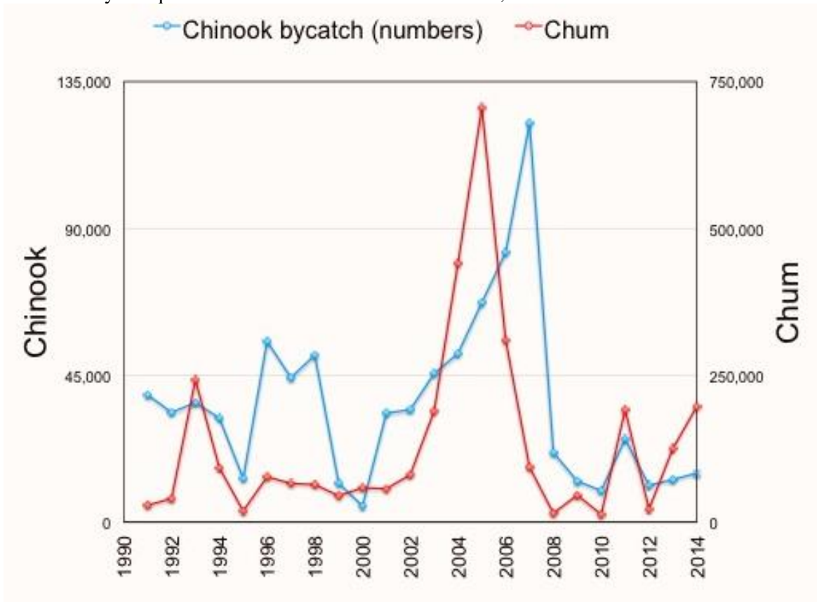
Figure 1. Time series of Chinook and chum salmon bycatch in the pollock fishery, 1991-2014.
