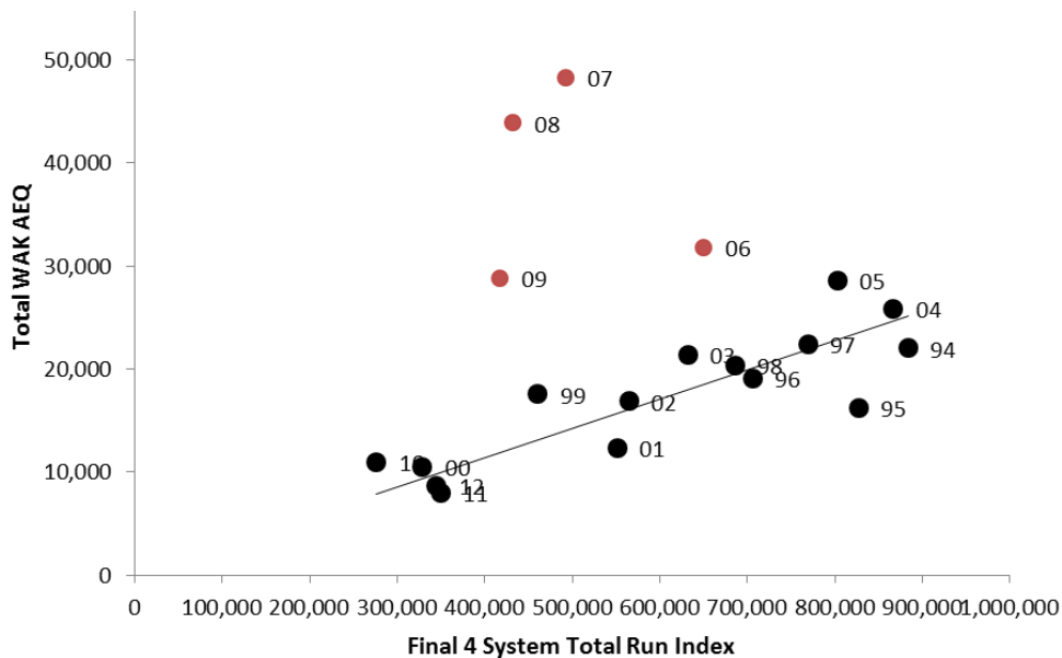
Figure 9. Relationship between final inriver run abundance of the 4 System Inriver Run Index (Kuskokwim, Upper Yukon, Unalakleet and Nushagak river systems) and the bycatch of AEQ attributed to Western Alaska stocks ( Y=0.0285x , R^2 = 0.712 ).
