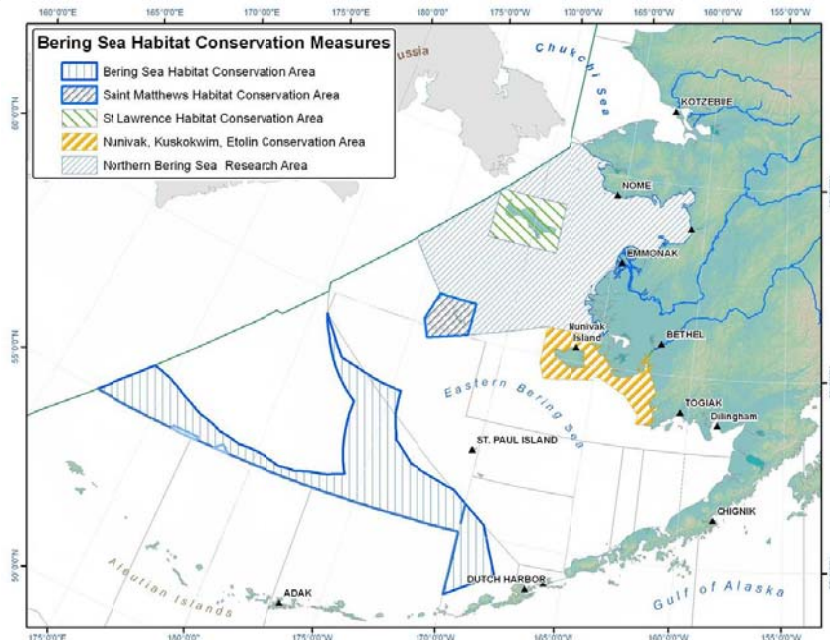
Figure 9. Bering Sea Habitat Conservation measures closure areas.
