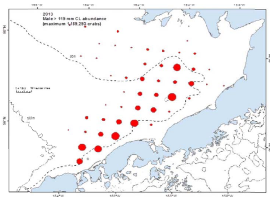
Figure 2 Distribution of mature male red king crab abundance from the NMFS trawl survey 2013
