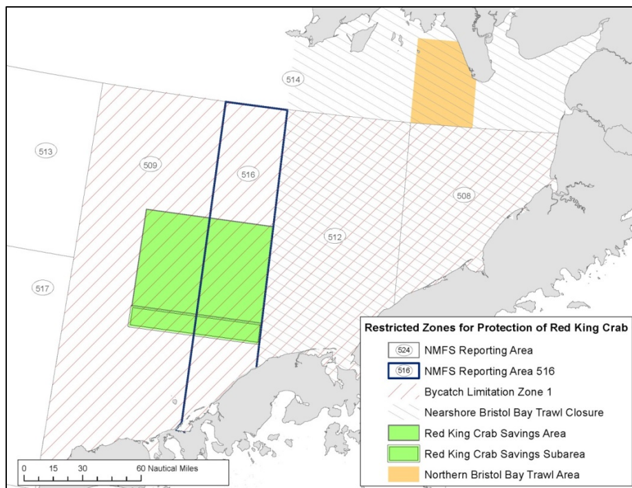
Figure 3 Restricted trawling areas for protection of red king crab in the eastern Bering Sea.
