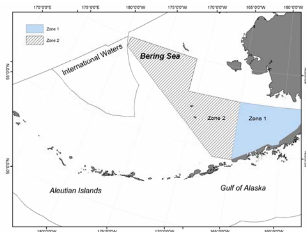
Figure 4. Zones 1 and 2 area for closures (Bristol Bay red king crab and EBS Tanner crab).
