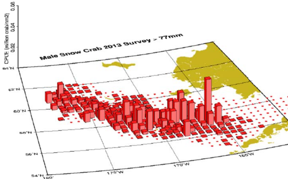
Figure 6 2013 Survey CPUE (million crab per nm 2 ) of males >77mm by tow. Filled circles are tows with 0 CPUE.
