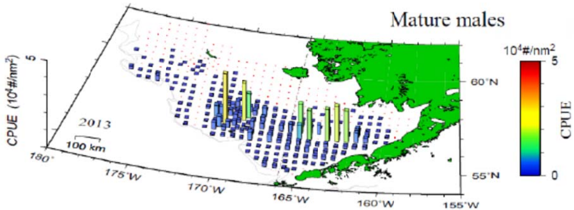
Figure 5 Distribution of mature males (number/sq. nm) in the summer trawl survey 2013
