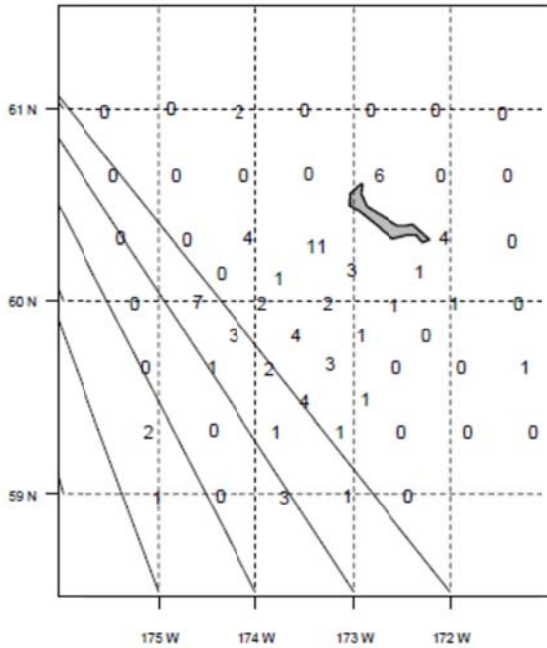
Figure 8 Catches of male blue king crab measuring at least 90 mm CL from the 2013 NMFS trawl-survey
