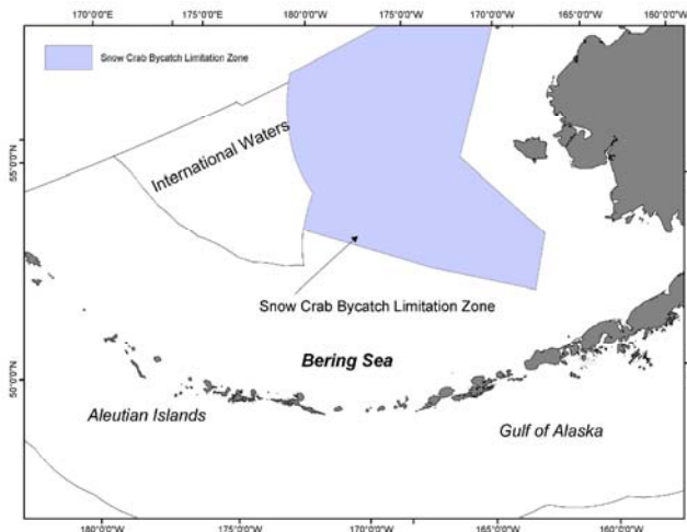
Figure 7. C. opilio Bycatch Limitation Zone (COBLZ)
