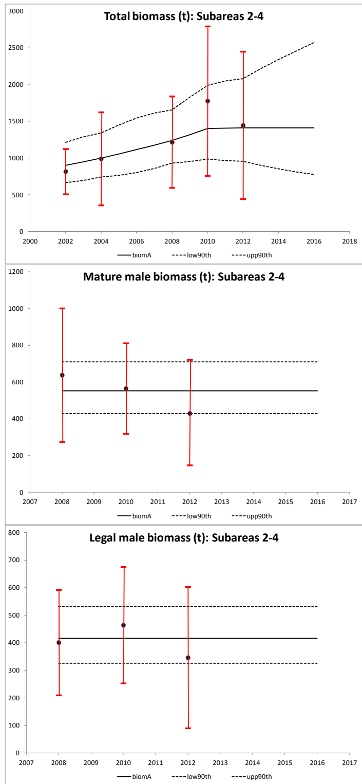
Figure 13. Plots of estimated and projected-into-2016 biomass of total, mature male, and legal male golden king crab in NMFS slope survey Subareas 2–4 with 90% confidence intervals and survey area-swept estimates; red bars are survey estimate plus/minus 2 standard errors.
