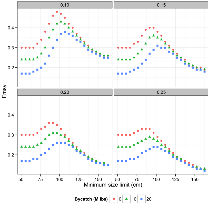
Figure 2. Estimates of F_{MSY} versus alternative minimum size limits and three levels of bycatch. Each panel represents an alternative discard mortality rate (indicated on the top of the panel).
