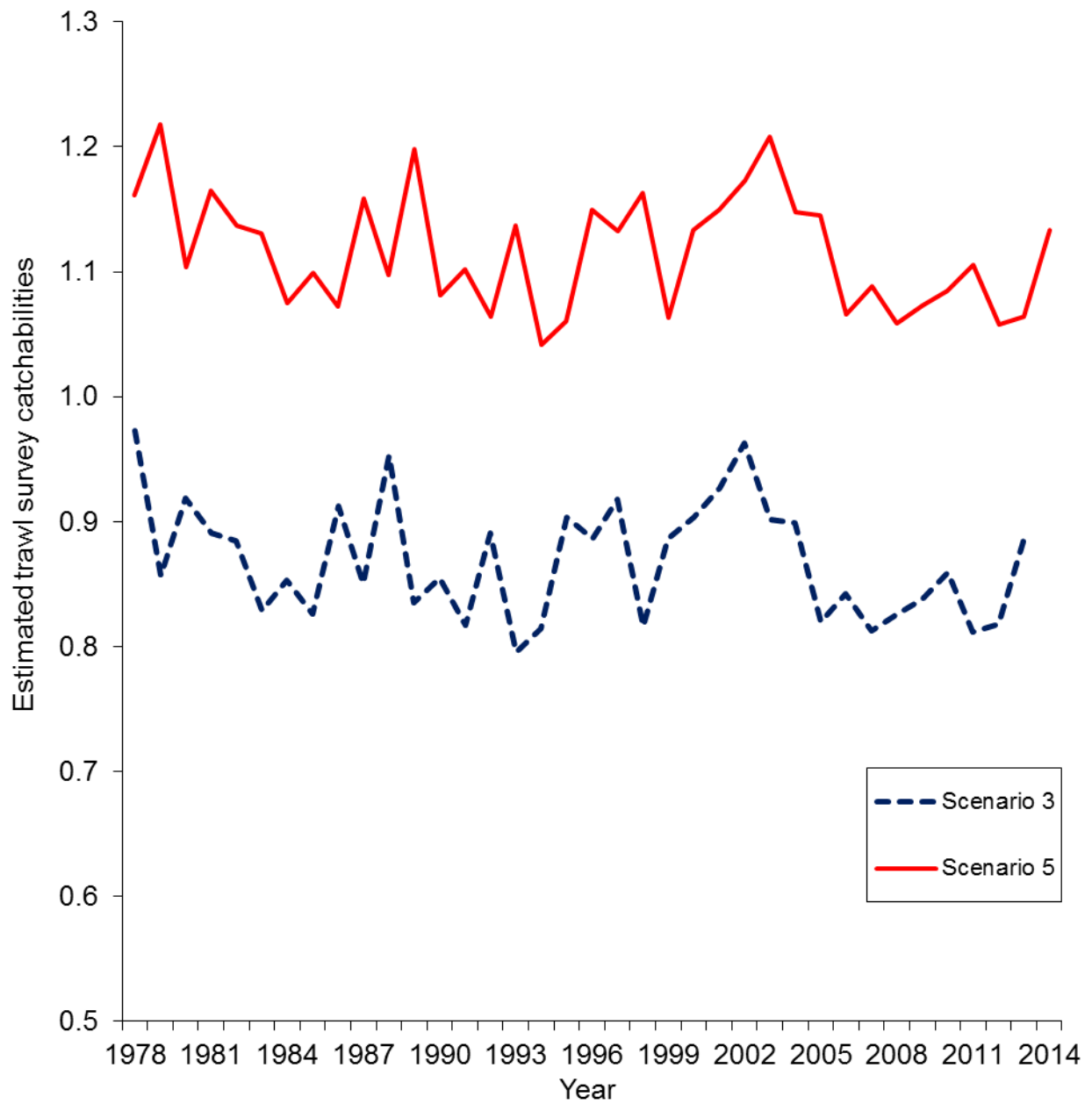
Figure 17. Estimated trawl survey catchabilities for scenarios 3 and 5.
