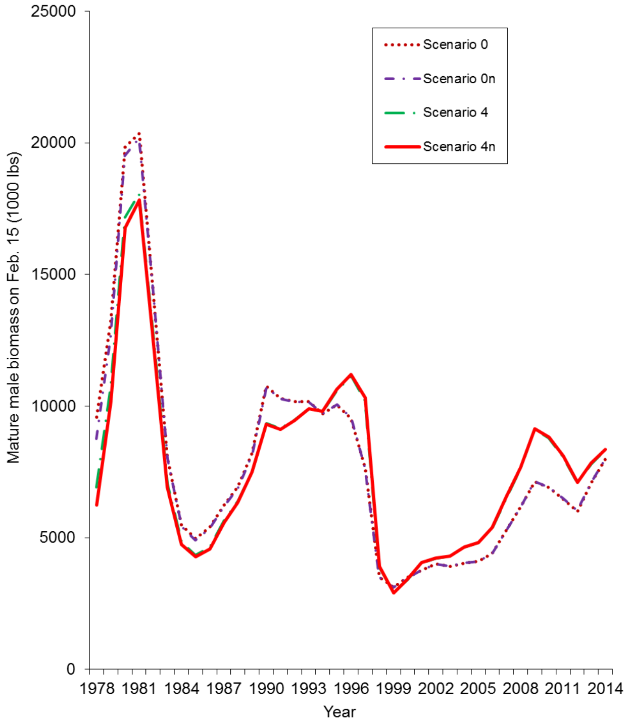
Figure 22. Estimated mature male biomass time series on Feb. 15 during 1978-2014 with scenarios 0, 0n, 4 and 4n.
