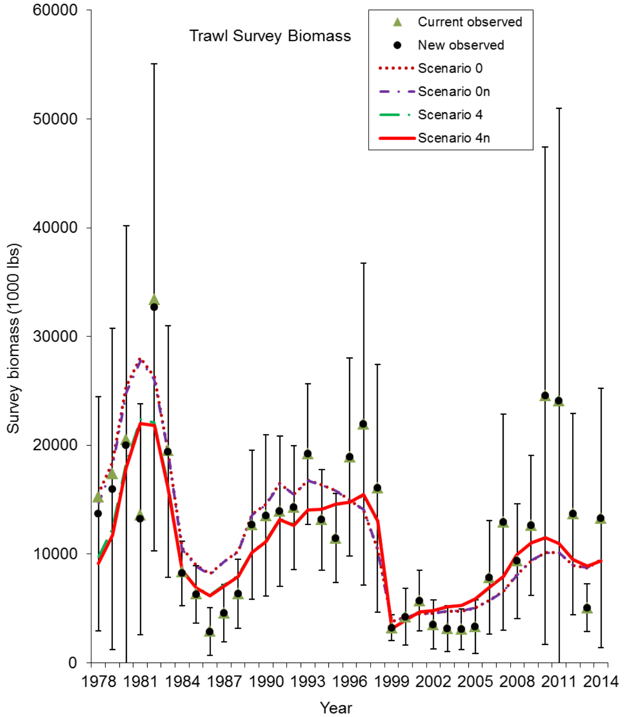
Figure 19. Comparisons of area-swept estimates of total male survey biomass and model prediction for model estimates in 2014 under scenarios 0, 0n, 4 and 4n. The error bars are plus and minus 2 standard deviations of new time series area-swept estimates.
