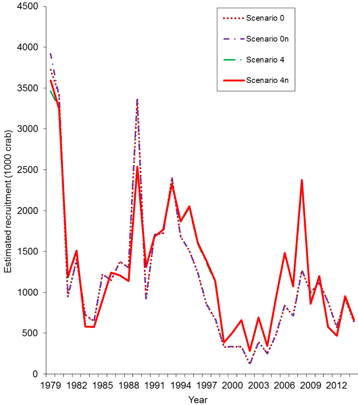
Figure 21. Estimated recruitment time series during 1979-2014 with scenarios 0, 0n, 4 and 4n.
