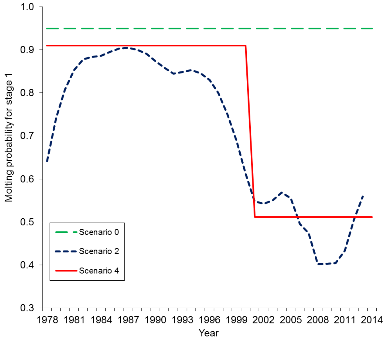
Figure 16. Estimated molting probabilities for stage 1 for scenarios 0, 2 and 4.
