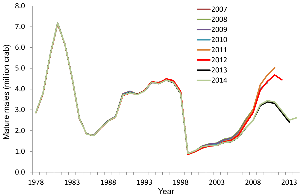
Figure 19. Retrospective plot of model-estimated legal and mature male abundance at time of survey for 2014 model scenario 4n with terminal years 2007-2014. Estimates are based on all available data up to and including terminal-year trawl and pot surveys.
