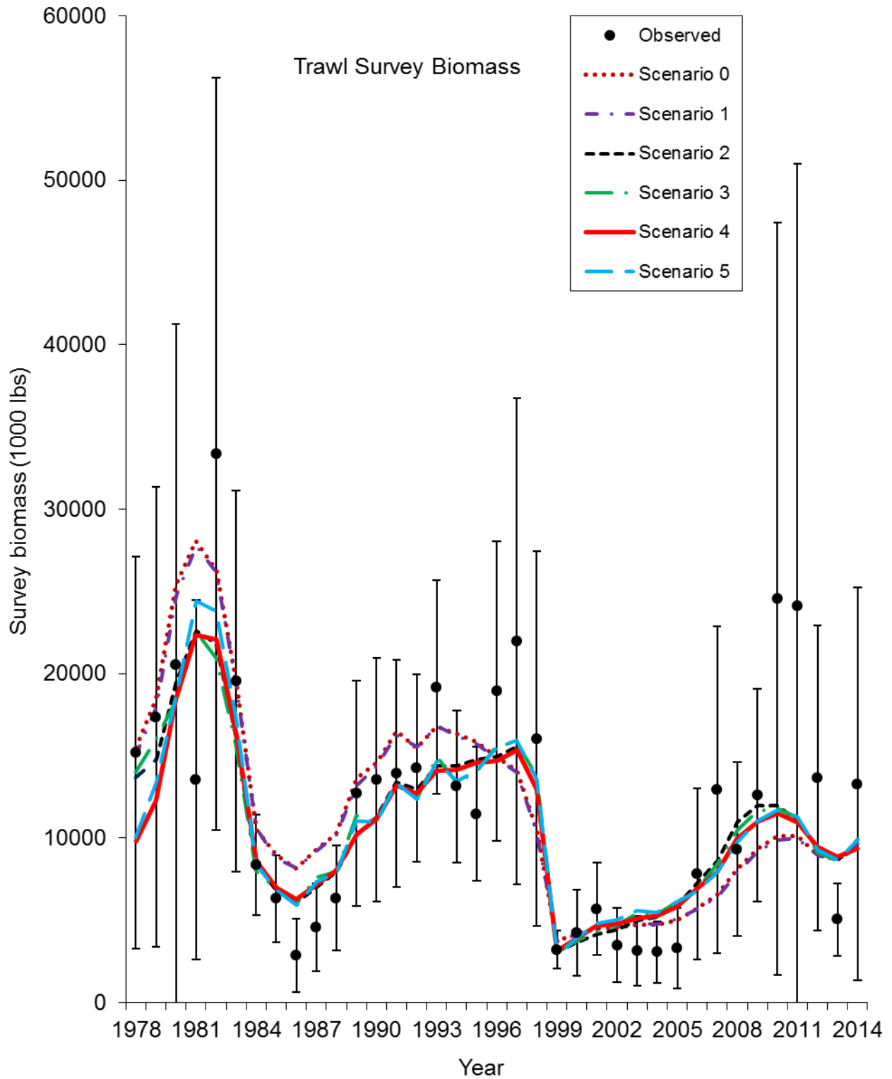
Figure 7. Comparisons of area-swept estimates of total male survey biomass and model prediction for model estimates in 2014 under scenarios 0-5. The error bars are plus and minus 2 standard deviations.
