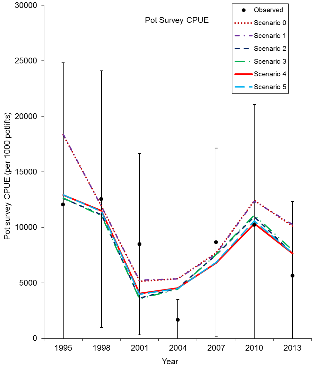
Figure 8. Comparisons of total male pot survey CPUEs and model prediction for model estimates in 2014 under scenarios 0-5. The error bars are plus and minus 2 standard deviations of scenario 4.
