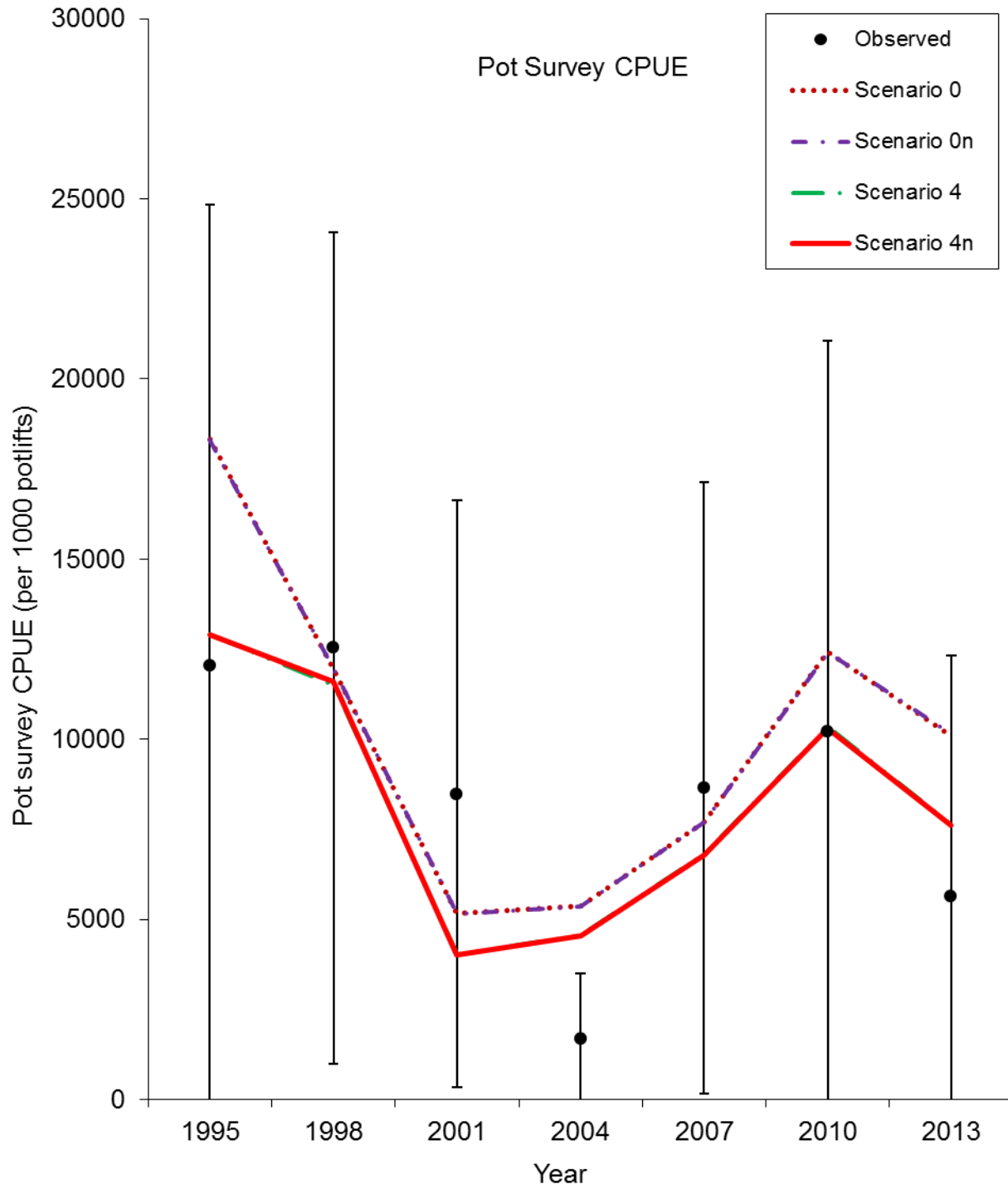
Figure 20. Comparisons of total male pot survey CPUEs and model prediction for model estimates in 2014 under scenarios 0, 0n, 4 and 4n. The error bars are plus and minus 2 standard deviations of scenario 4n.
