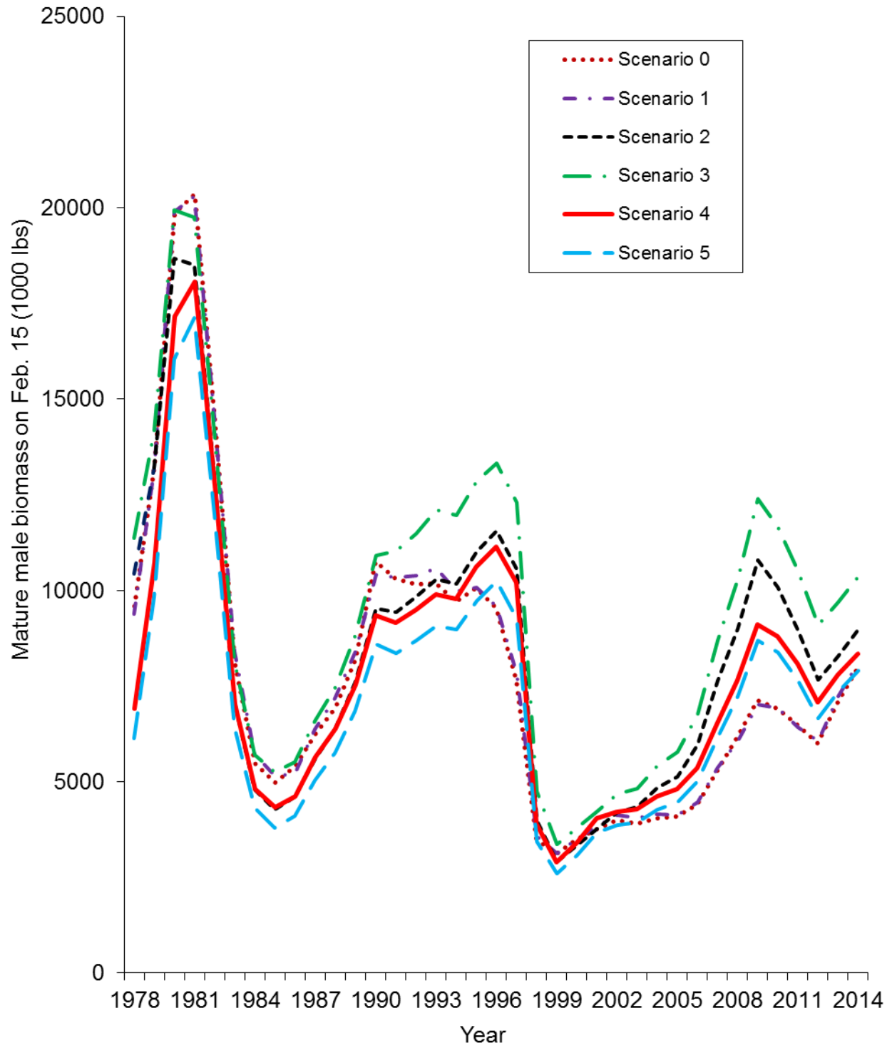
Figure 14. Estimated mature male biomass time series on Feb. 15 during 1978-2014 with scenarios 0-5.
