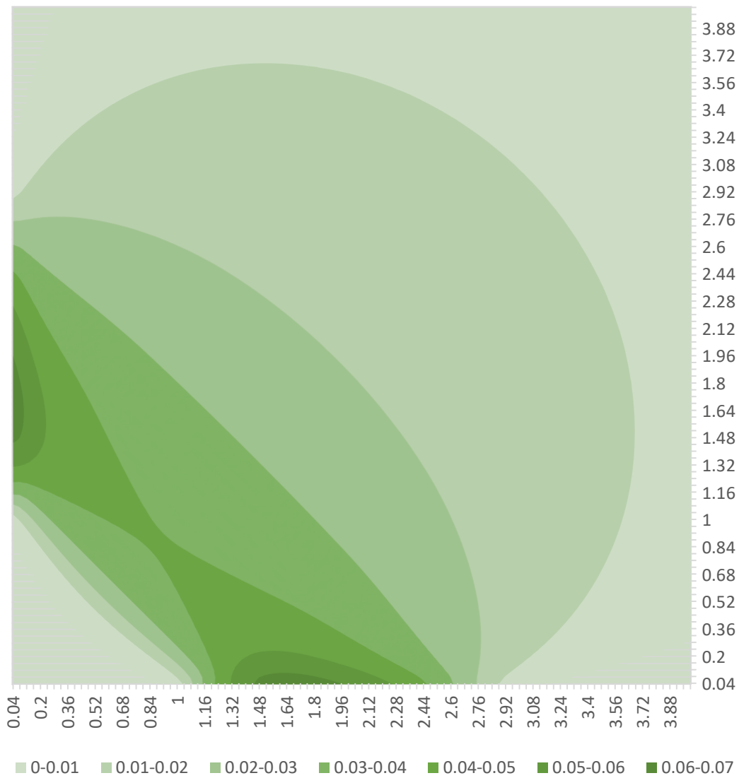
Figure 2.1.3.6. Contour plot showing the proportion of the 3-dimensional correlation volume under which the CV_{ABC} ratio exceeds unity, as a function of the ratios \sigma_1/\sigma_3 and \sigma_2/\sigma_3 (axes are interchangeable), where \sigma_1 is the log-scale standard deviation of F_{40\%} , \sigma_2 is the log-scale standard deviation of B_{40\%} , and \sigma_3 is the log-scale standard deviation of female spawning biomass.
