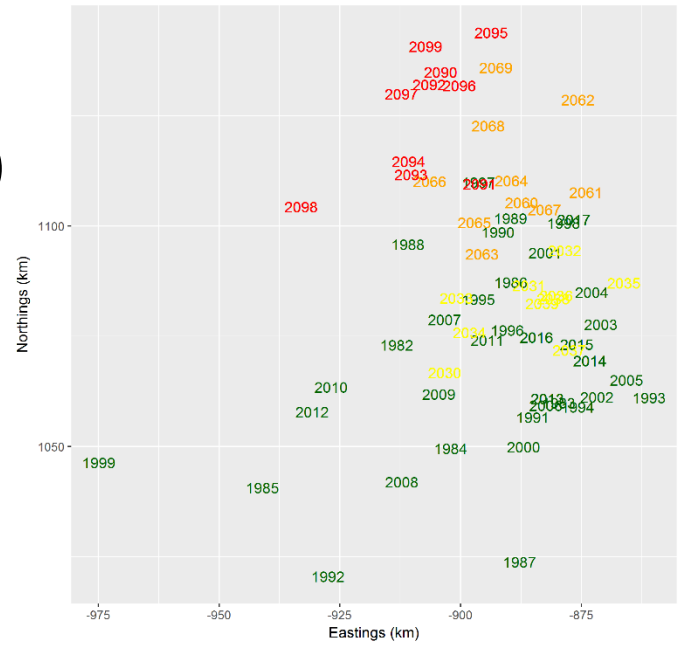
Average Center of Gravity - Adult_Arrowtooth_Flounder
