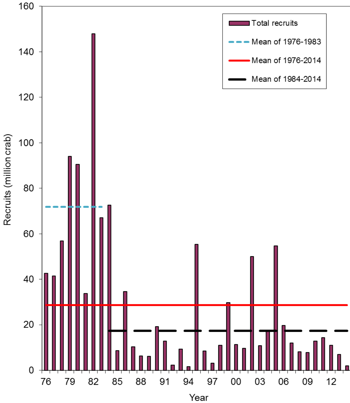
Figure 11(2n). Estimated recruitment time series during 1976-2014 (occurred year) with scenario 2n. Mean male recruits during 1984-2014 was used to estimate B35%.
