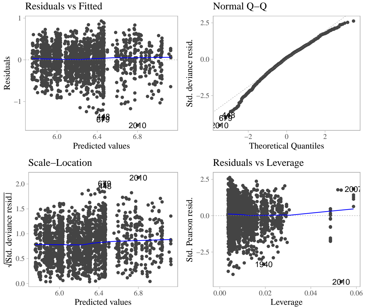
Figure 4: Linear model diagnostics for the final model fit to total catch CPUE with a lognormal distributed error.
