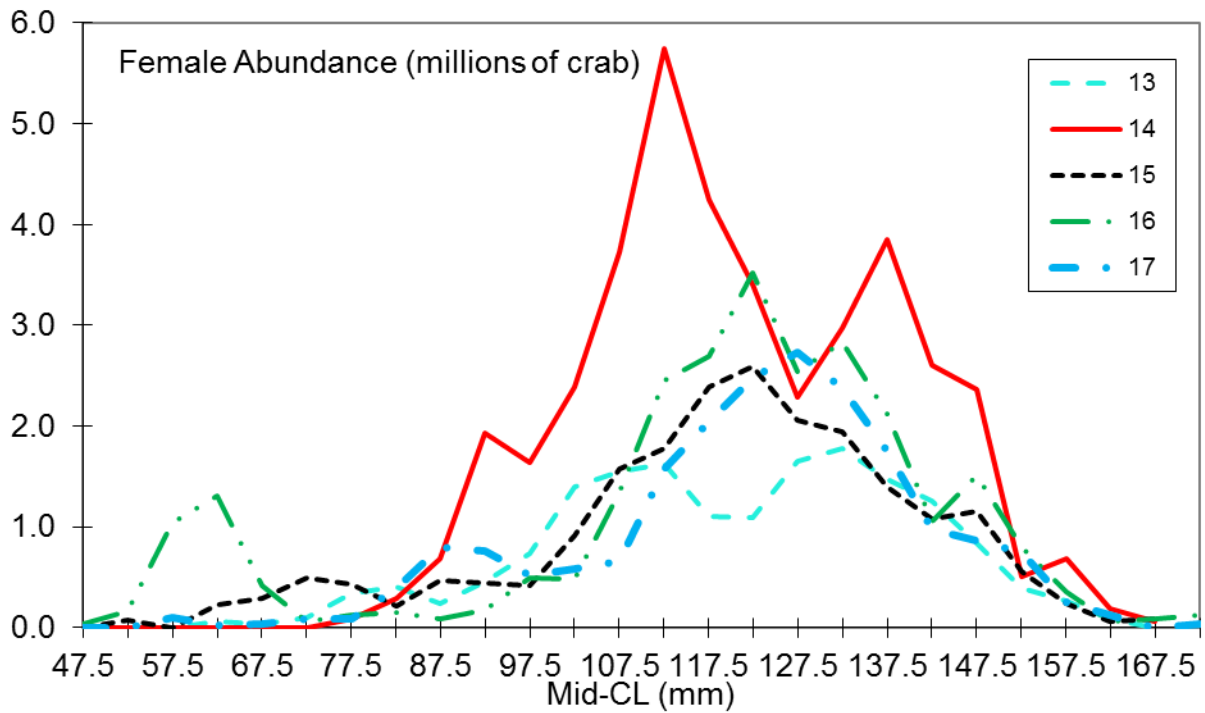
Figure 34. Length frequency distributions of male (top panel) and female (bottom panel) red king crab in Bristol Bay from NMFS trawl surveys during 2013-2017. For purposes of these graphs, abundance estimates are based on area-swept methods.
