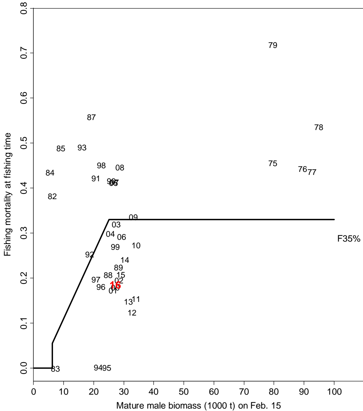
Figure 13(2bn2). Relationships between full fishing mortalities for the directed pot fishery and mature male biomass on Feb. 15 during 1975-2016 under scenario 2bn2. Average of recruitment from 1984 to 2017 was used to estimate BMSY. Pot, fixed gear and trawl handling mortality rates were assumed to be 0.2, 0.5 and 0.8, respectively.
