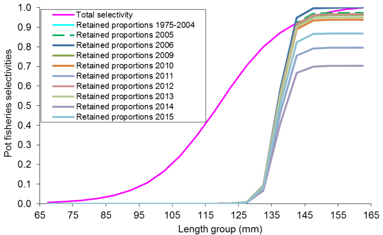
Figure 8d. Estimated pot fishery selectivities and retained proportions under scenarios 2bn1 (upper panel) and 2bn2 (lower panel). Estimated retained proportions for years not shown are within the range of estimated retained proportions in the figure. Pot, fixed gear and trawl handling mortality rates were assumed to be 0.2, 0.5 and 0.8, respectively.
