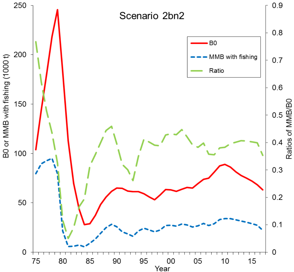
Figure D1. Estimated B0, MMB with fishing, and ratios of MMB/B0 from 1975 to 2017 for scenario 2bn2 for Bristol Bay red king crab.
