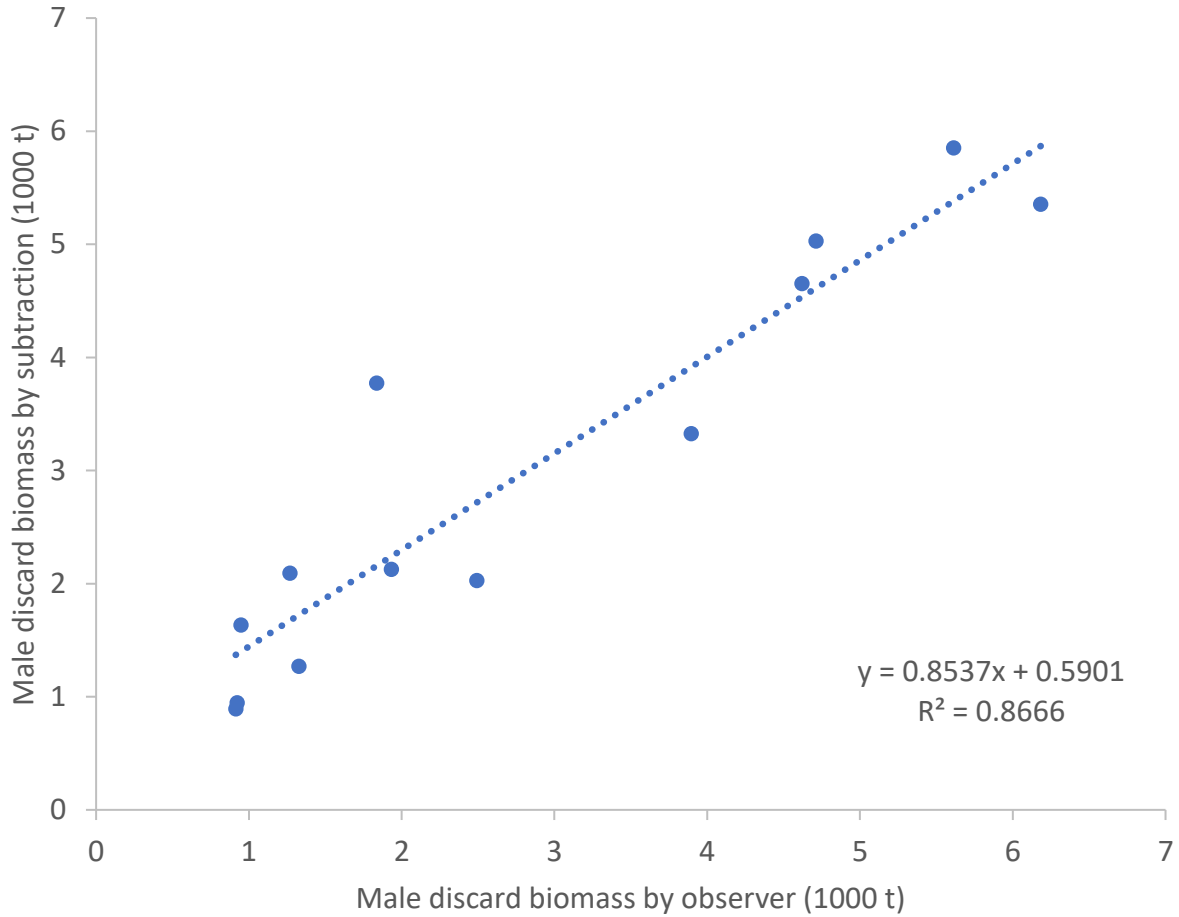
Figure C1. Relationship between male discard biomasses estimated by Subtraction approach and observer's determination of retained status in the Bristol Bay red king crab directed pot fishery.
