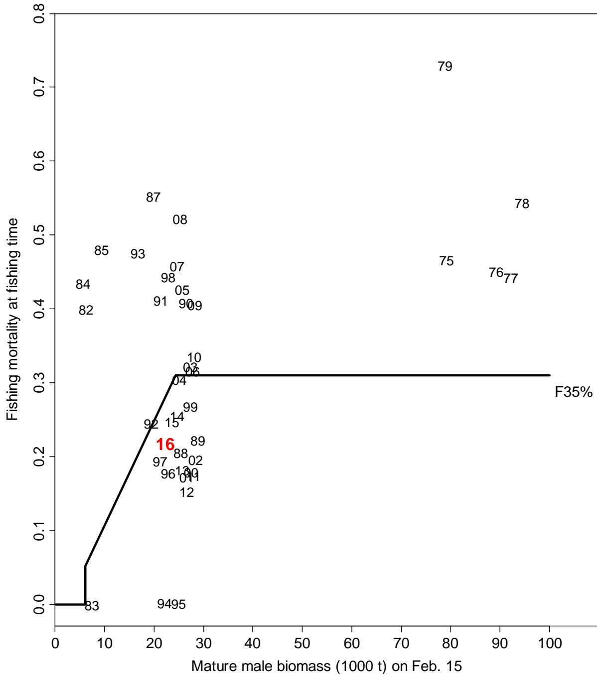
Figure 13(2bn1). Relationships between full fishing mortalities for the directed pot fishery and mature male biomass on Feb. 15 during 1975-2016 under scenario 2bn1. Average of recruitment from 1984 to 2017 was used to estimate BMSY. Pot, fixed gear and trawl handling mortality rates were assumed to be 0.2, 0.5 and 0.8, respectively.
