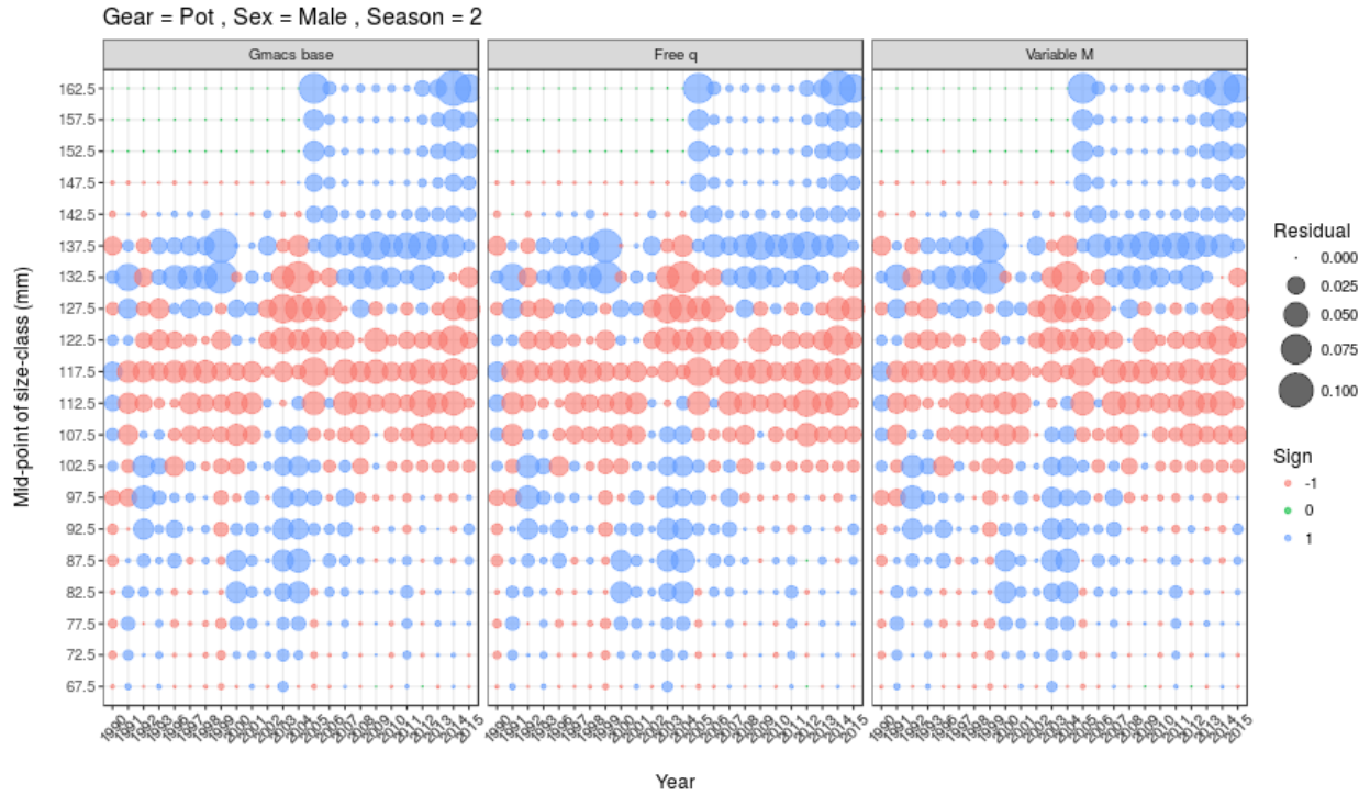
Figure 32: Size-frequency residuals of discarded male BBRKC by year in the directed pot fishery for the 2017 model and each of the Gmacs model scenarios.
