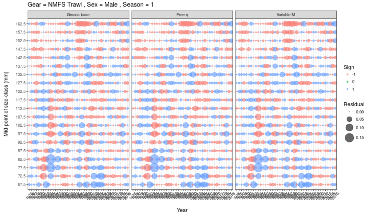
Figure 40: Size-frequency residuals of discarded male BBRKC by year in the NMFS trawl survey for the 2017 model and each of the Gmacs model scenarios.
