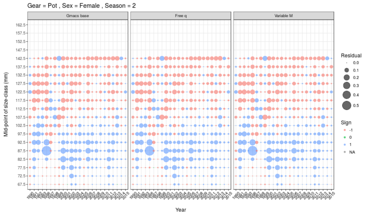
Figure 33: Size-frequency residuals of discarded female BBRKC by year in the directed pot fishery for the 2017 model and each of the Gmacs model scenarios.
