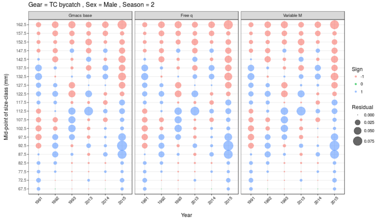
Figure 36: Size-frequency residuals of discarded male BBRKC by year in the tanner crab bycatch fishery for the 2017 model and each of the Gmacs model scenarios.
