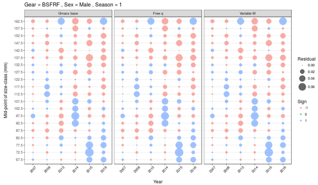
Figure 42: Size-frequency residuals of discarded male BBRKC by year in the BSFRF survey for the 2017 model and each of the Gmacs model scenarios.
