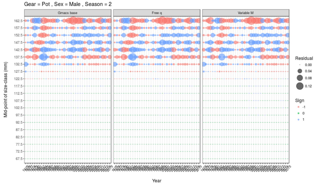
Figure 31: Size-frequency residuals of male BBRKC by year retained in the directed pot fishery for the 2017 model and each of the Gmacs model scenarios.
