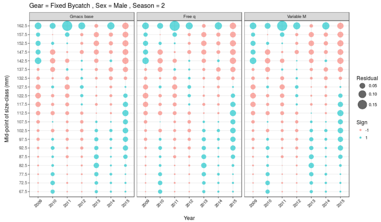
Figure 38: Size-frequency residuals of discarded male BBRKC by year in the fixed bycatch fishery for the 2017 model and each of the Gmacs model scenarios.
