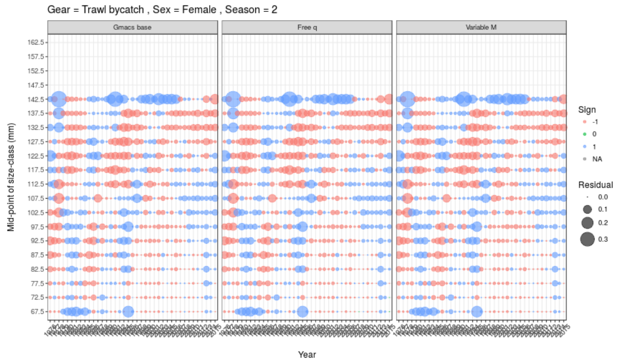
Figure 35: Size-frequency residuals of discarded female BBRKC by year in the trawl bycatch fishery for the 2017 model and each of the Gmacs model scenarios.
