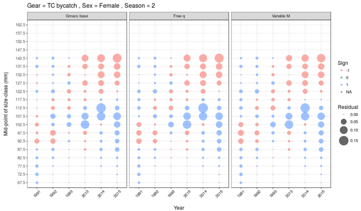
Figure 37: Size-frequency residuals of discarded female BBRKC by year in the tanner crab bycatch fishery for the 2017 model and each of the Gmacs model scenarios.
