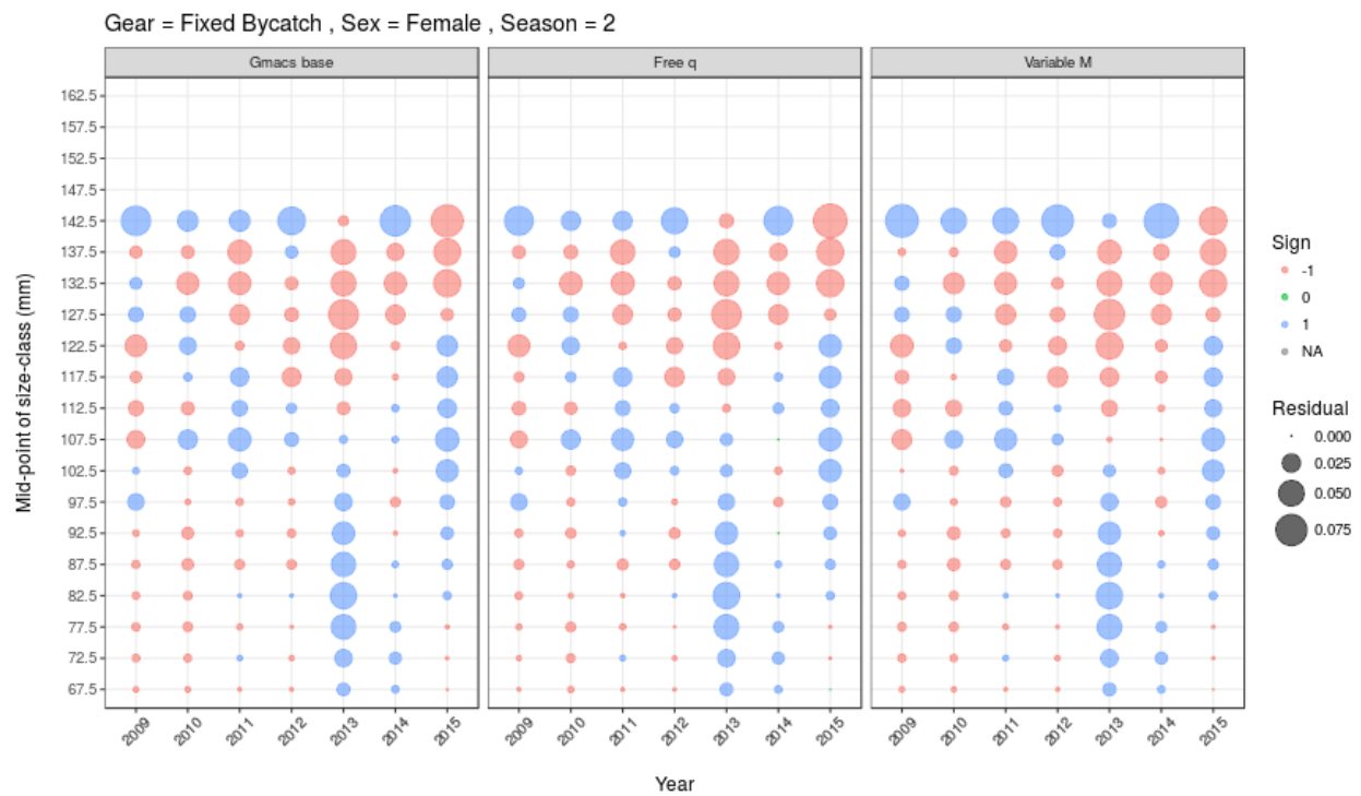
Figure 39: Size-frequency residuals of discarded female BBRKC by year in the fixed bycatch fishery for the 2017 model and each of the Gmacs model scenarios.
