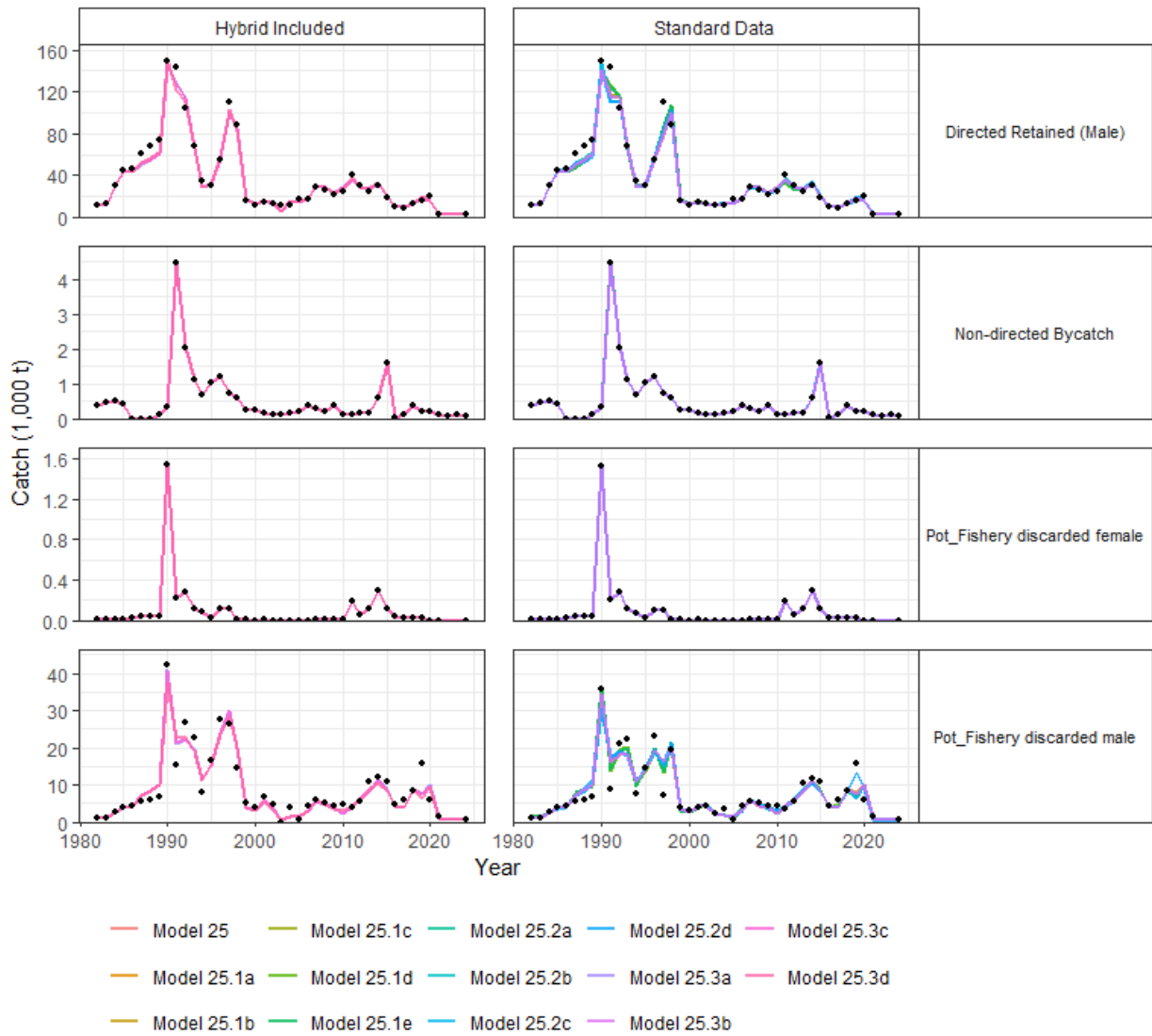
Figure 10: Model fits to catch data.
