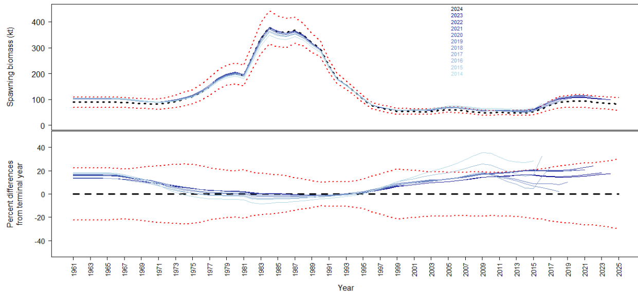
Figure 1A. 24 Retrospective analysis for Authors' preferred Model 15.1 with data for the previous 10 years being systematically removed from the model. Black dashed line is the 2024 Model 15.1 estimate, the red dotted lines are the 95% confidence intervals calculated as \pm 1.96 \times standard deviation.
