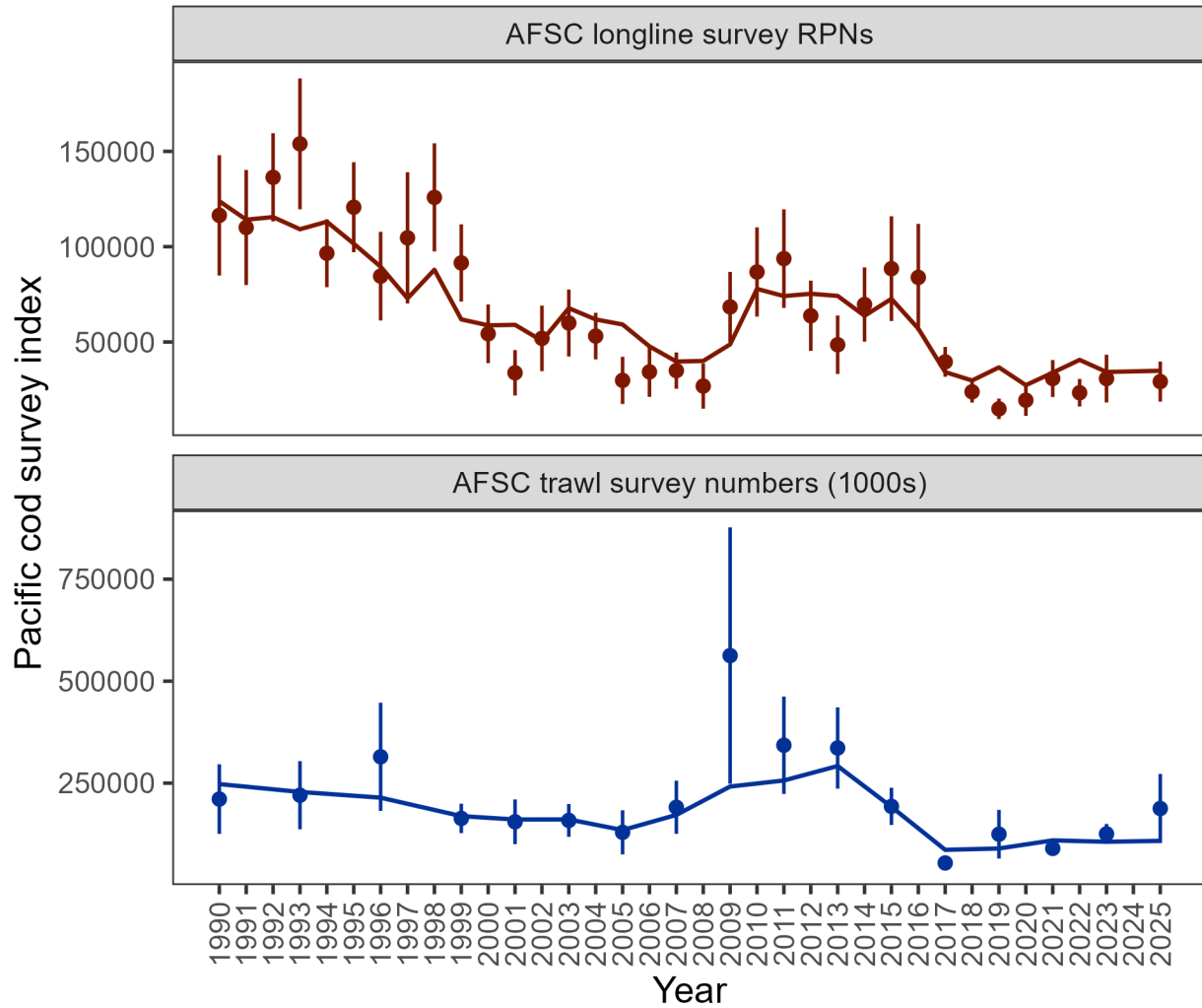
Figure 2.10. Population indices fit by the assessment model, including AFSC longline survey relative population numbers (RPN – top panel) and AFSC bottom trawl survey abundance (numbers – bottom panel). Model fit is shown as a solid line and observed data is shown as points (with error bars indicating the 95% confidence intervals).
