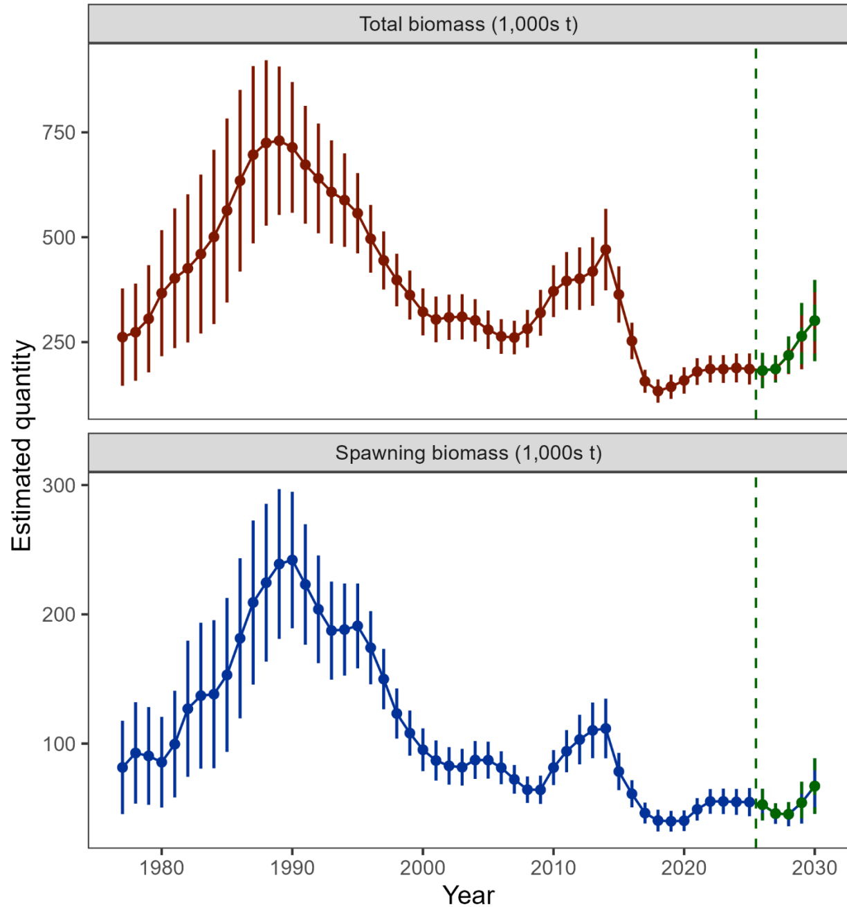
Figure 2.13. Estimated total biomass (top panel) and spawning biomass (bottom panel) from the author's recommended model with 95% confidence intervals. The five-year forecasted biomass values are denoted in green shading and with the vertical dashed line in each plot.
