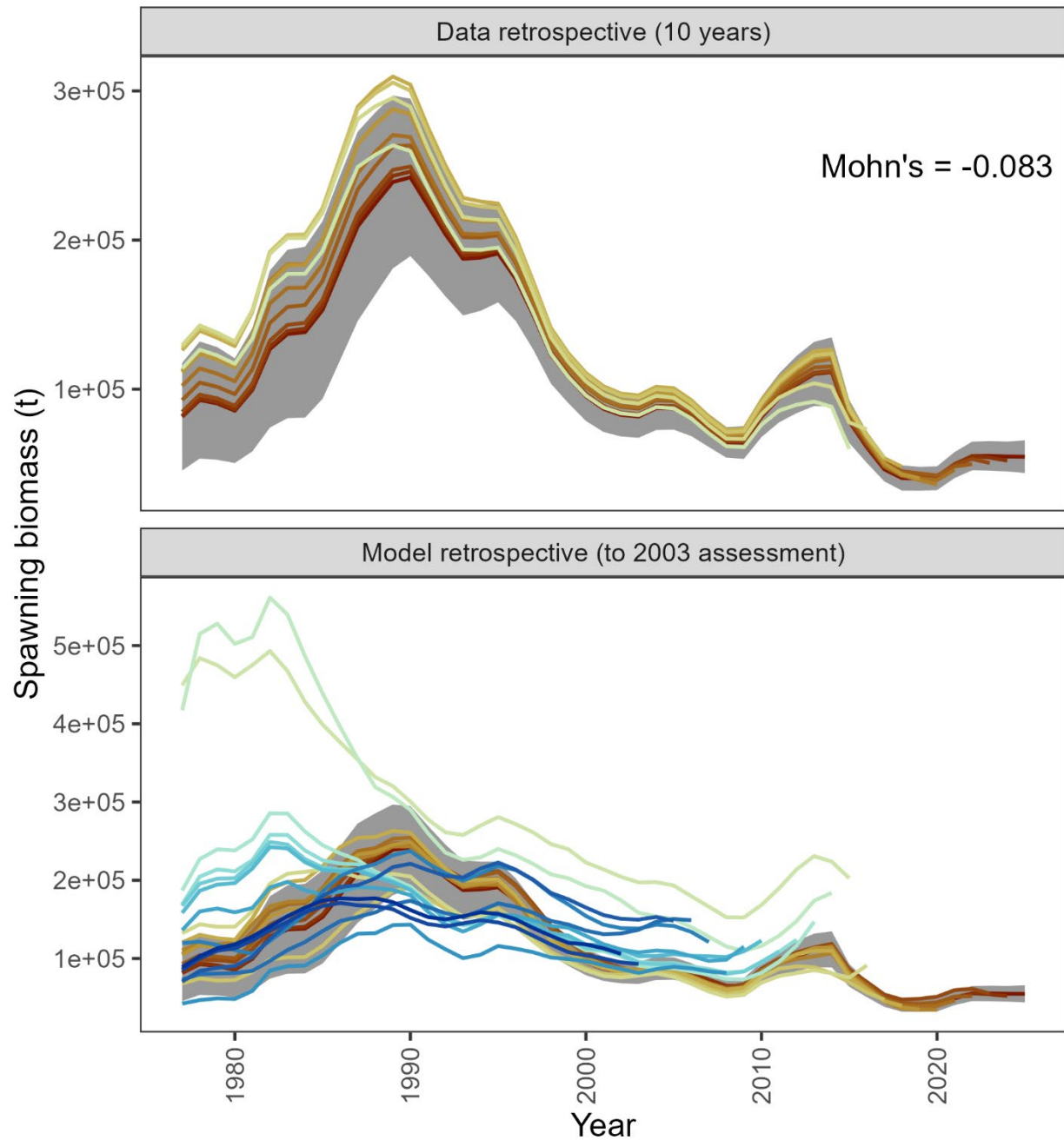
Figure 2.9. Retrospective analysis of spawning biomass upon removing data from Model 24.0 as applied in 2025 (top panel) and in comparison to previously accepted models (bottom panel). The shaded region is the 95% confidence intervals from Model 24.0.
