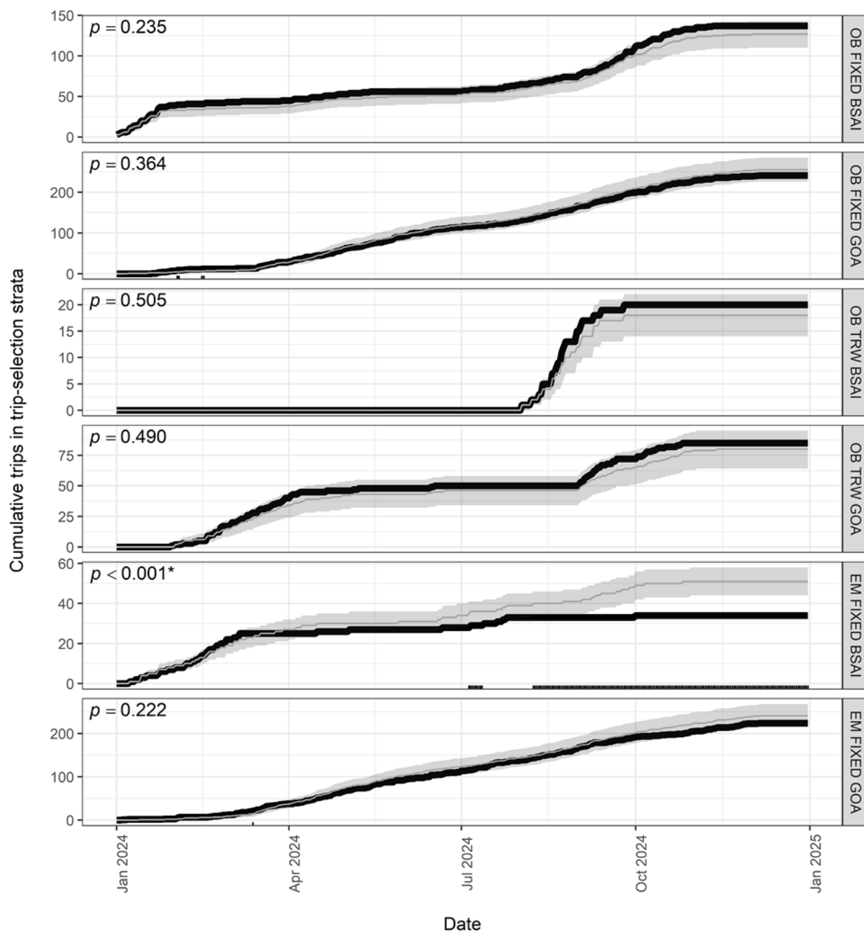
Figure 3-5-- Cumulative number of trips monitored during 2024 (black line) compared to the expected range of observed trips (shaded ribbon) given fishing effort and sampling rates. Dates where the monitored number of trips is outside of expected (less or more than the range) are depicted as tick marks on the x-axis. Test results (using a binomial distribution) determining if the observed rate was sampled at the selection rate are denoted as p -values.---
