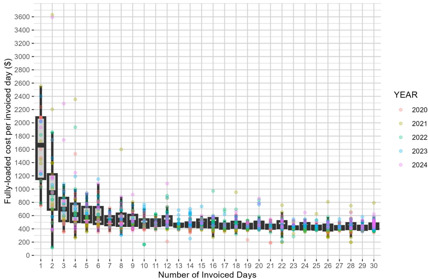
Figure 2-1-- Relationship between the fully loaded cost per invoiced day for full observer coverage as a function of the number of days invoiced, which is a proxy for the duration of the deployment. The fully-loaded cost per day is calculated as the invoice total divided by the number of days on the invoice. Includes all vessel/gear types.
