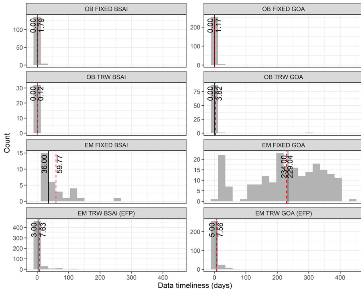
Figure 3-3-- Distributions of data timeliness (the time between a trip or delivery ending and those monitoring data being available for catch accounting) by stratum. Solid black lines and annotations to the left show median data timeliness. Dashed red lines and annotations to the right show mean data timeliness.
