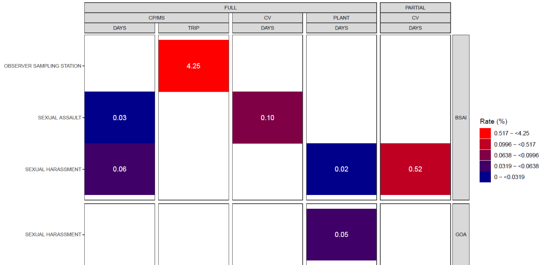
Figure 5-2-- Occurrence rates by FMP (rows, right), and coverage type, vessel type, and unit type (columns) for the highest-rate subcategory of all the OLE high-priority statement subcategories ("Observer Sampling Station") in Figure 5.1 and the OLE priority statement categories of sexual assault and sexual harassment.
