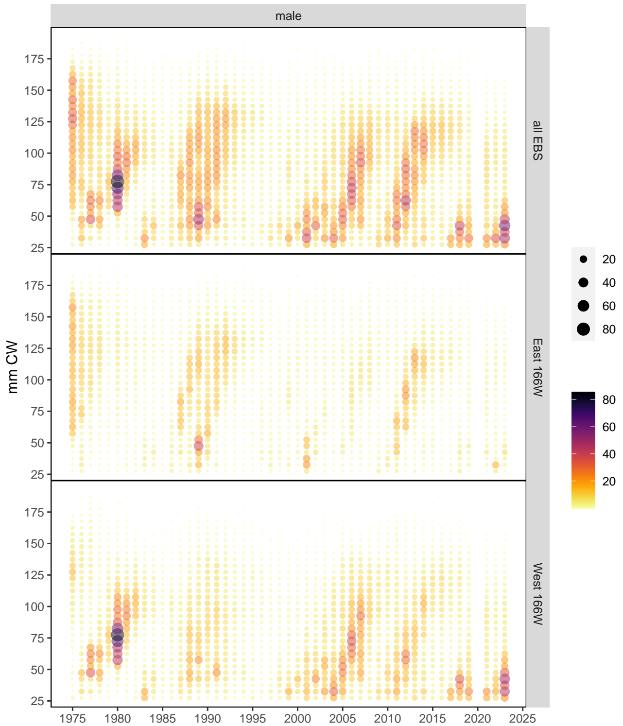
Figure 34. Annual size compositions, by 5-mm CW bin, from the NMFS EBS shelf bottom trawl survey for males by ADF&G management area for 1975-2023 as a bubble plot. The size compositions are truncated for crab < 25 mm CW.
