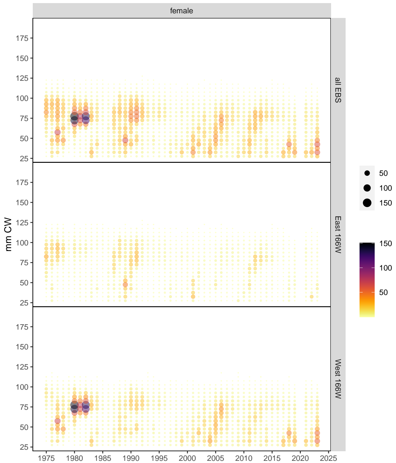
Figure 35. Annual size compositions, by 5-mm CW bin, from the NMFS EBS shelf bottom trawl survey for females by ADF&G management area for 1975-2023 as a bubble plot. The size compositions are truncated for crab < 25 mm CW.
