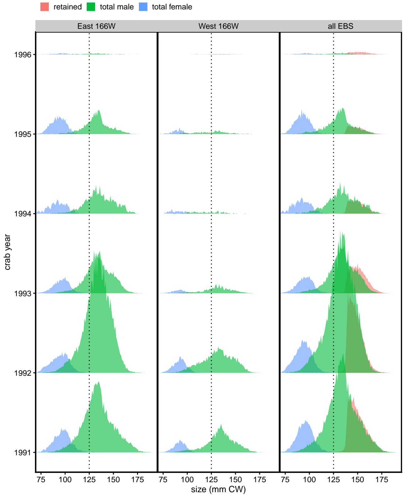
Figure 14. Comparison of expanded size compositions for retained and total catch in the directed fishery prior to 1997/98. Retained catch has already been aggregated across ADF&G management areas. Dotted line indicates recent industry-preferred size.
