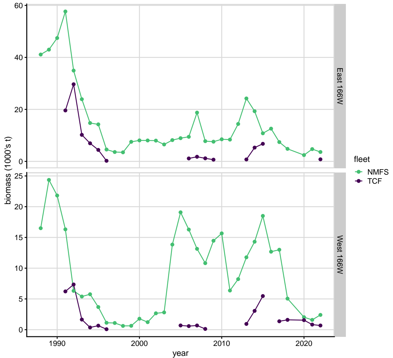
Figure 31. Comparison of the biomass of industry-preferred size males estimated from the NMFS EBS shelf survey and caught in the directed fishery ('TCF'), by ADF&G management area. The survey values have been lagged a year to align visually with the fishery values.
