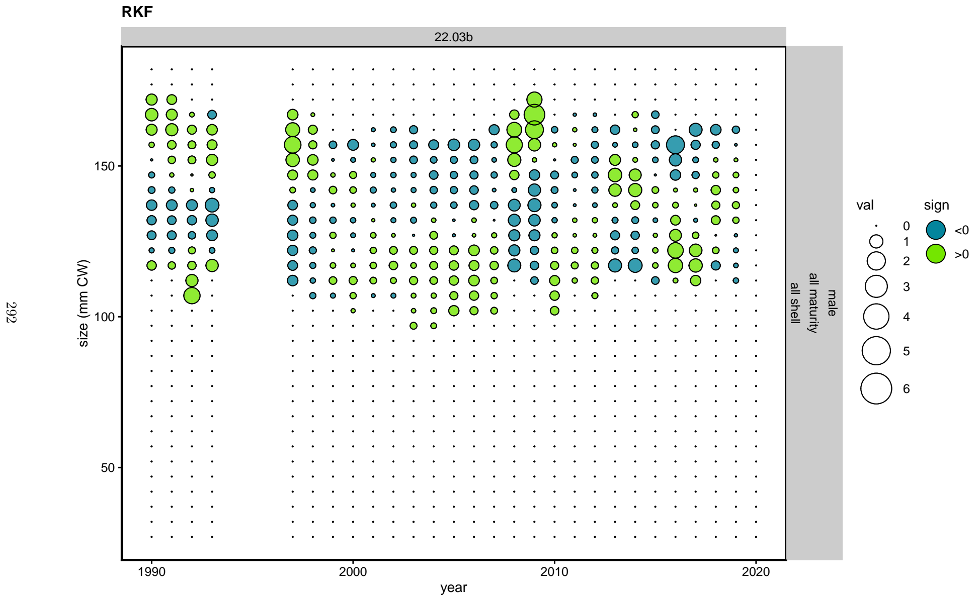
Figure 104. Pearson's residuals for fits to total catch size composition data. Symbol areas reflect the size of each residual, extreme values (residuals larger than 4 in scale) are indicated with a red 'X' to facilitate identification. Preferred model is 22.03b.
