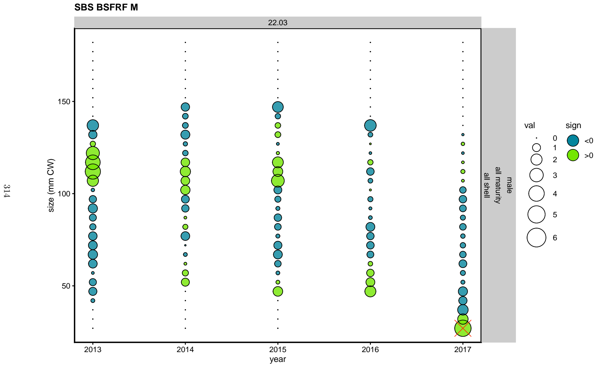
Figure 126. Pearson's residuals for fits to survey size composition data. Symbol areas reflect the size of each residual, extreme values (residuals larger than 4 in scale) are indicated with a red 'X' to facilitate identification. Preferred model is 22.03b.
