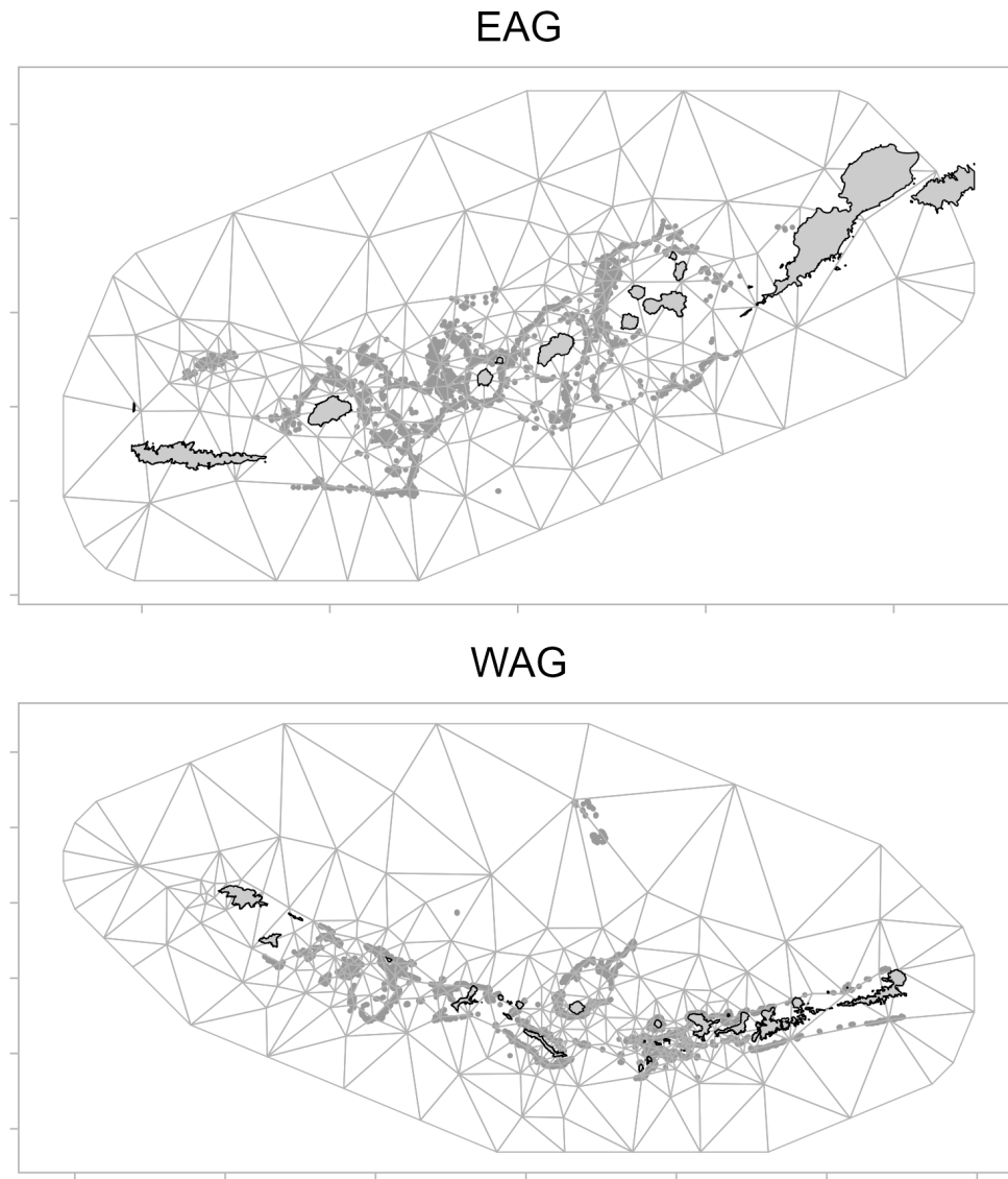
Figure 8: Triangular mesh based on k-means clustering with 150 knots used in spatiotemporal GAMMs for EAG and WAG. Grey points are observer pot locations for which confidentiality waivers have been obtained.
