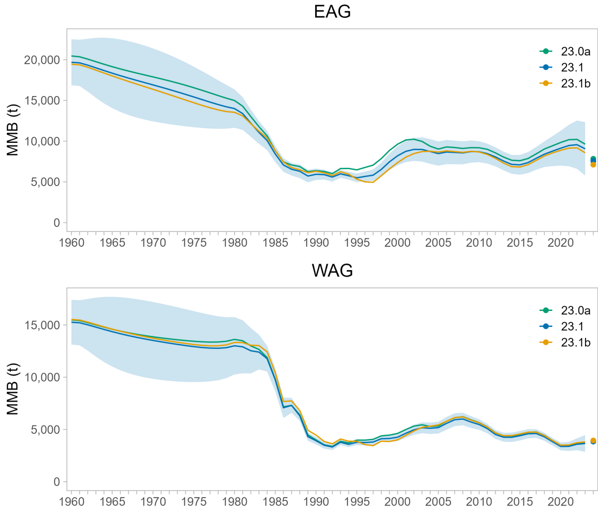
Figure 25: Comparison of model estimated MMB (lines) and terminal year MMB projected to mating (Feb 15, 2025) (dots). Shaded area represents the 95% confidence interval for model 23.1. Model 23.0a is the base model with updated data, 23.1 truncates the size composition, 23.0a uses alternative size composition weights, and 23.1b uses an additional selectivity period.
