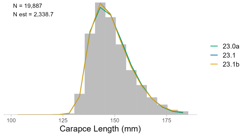
Figure 14: Comparison of model fit to aggregated retained catch size composition in the WAG. Estimated effective sample sizes are for model 23.1.
