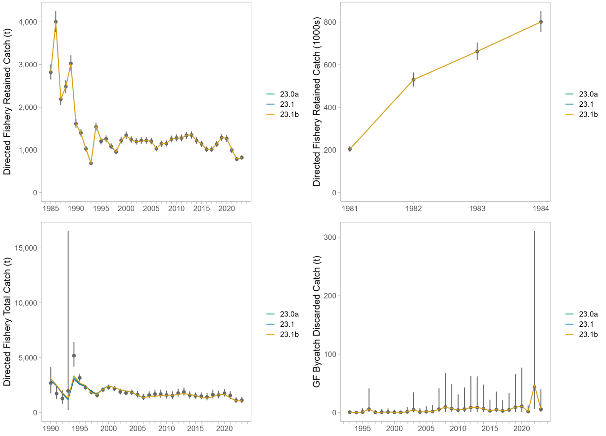
Figure 8: Comparison of model fit to retained catch, total catch, and groundfish bycatch mortality for the WAG. Error bars on observed values represent 95% confidence intervals.
