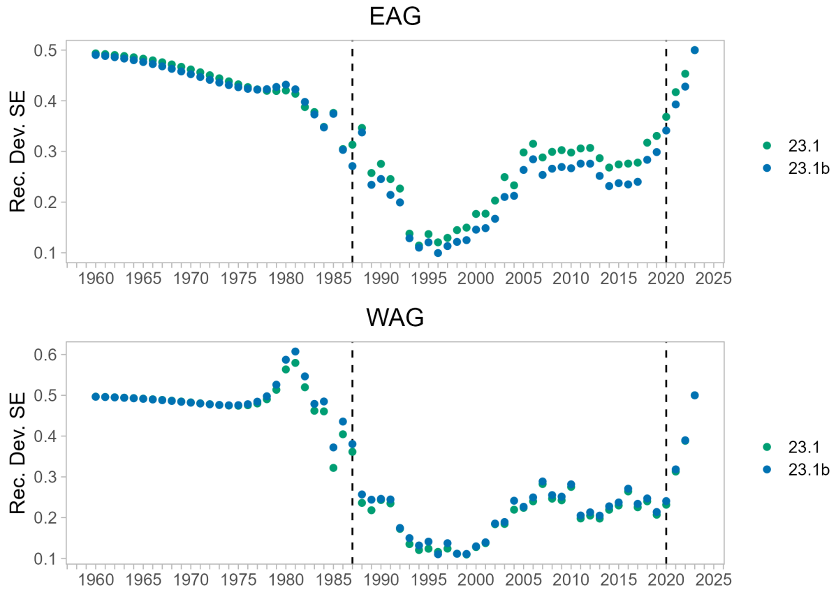
Figure 24: Standard errors of recruitment deviations for models 23.1 and 23.1b. Dotted lines indicate the reference time series for mean recruitment used in reference point calculation, 1987 - 2020.
