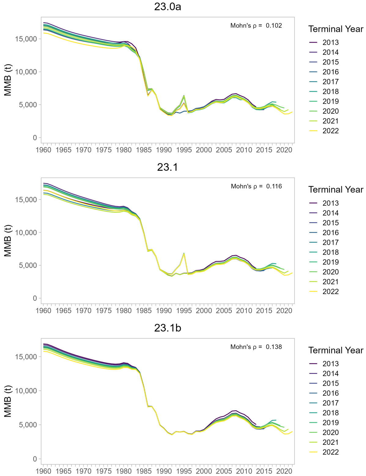
Figure 31: Estimated MMB and associated Mohn's \rho from retrospective analysis of WAG models 23.0a, 23.1, and 23.1b.
