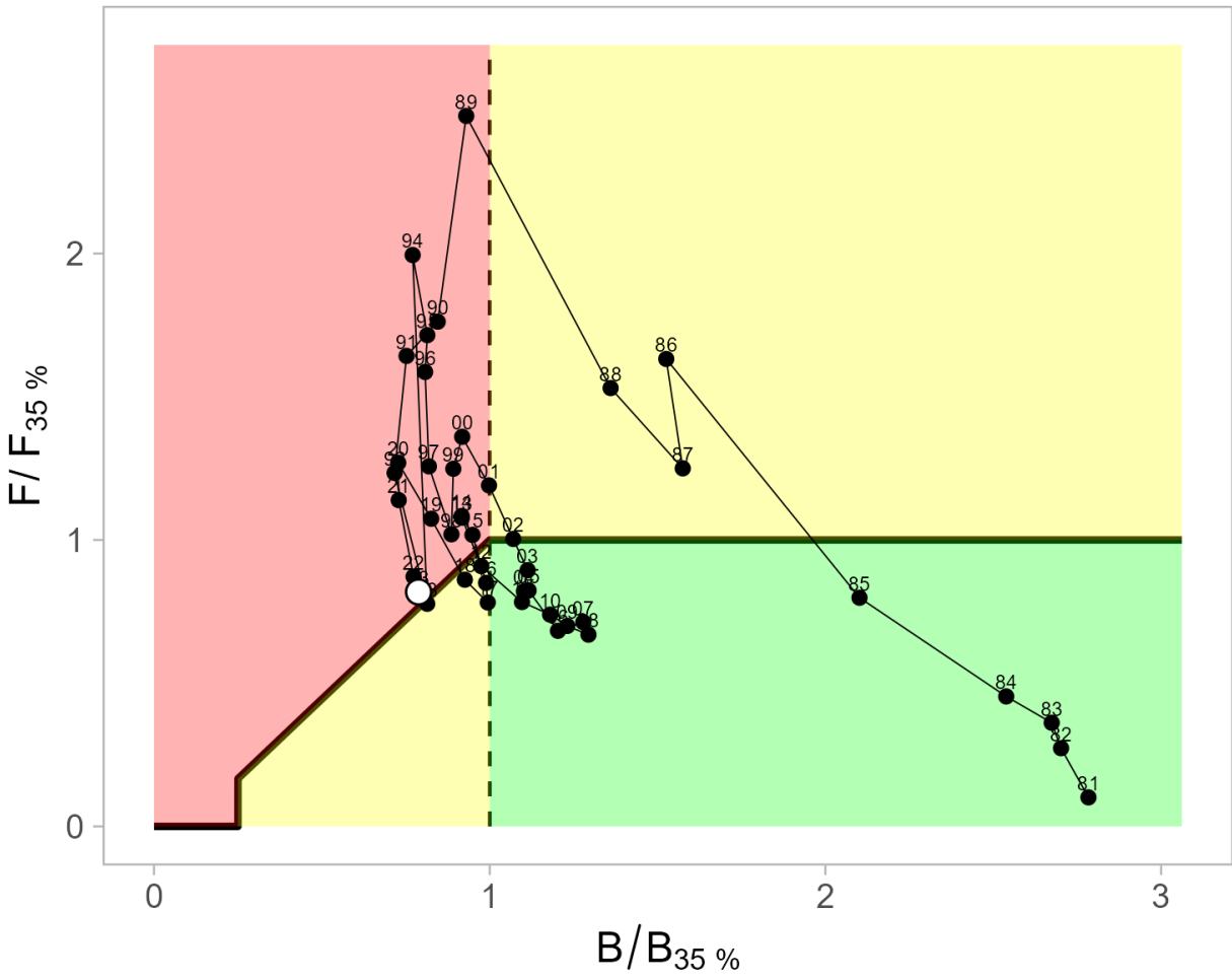
Figure 29: Kobe plot for model WAG 23.1. Bolded line indicates the tier 3 F_{OFL} control rule.
