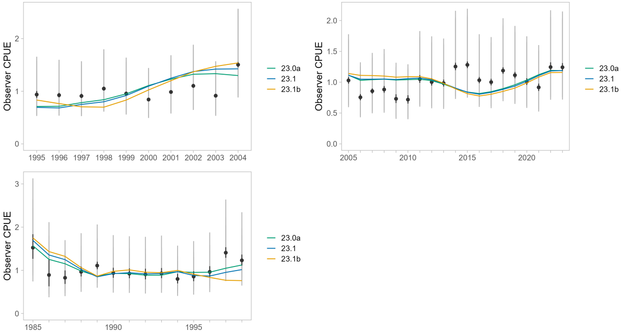
Figure 9: Comparison of model fit to CPUE indices for the EAG. Error bars on observed values represent 95% confidence intervals (black) and estimated additional error (grey).
