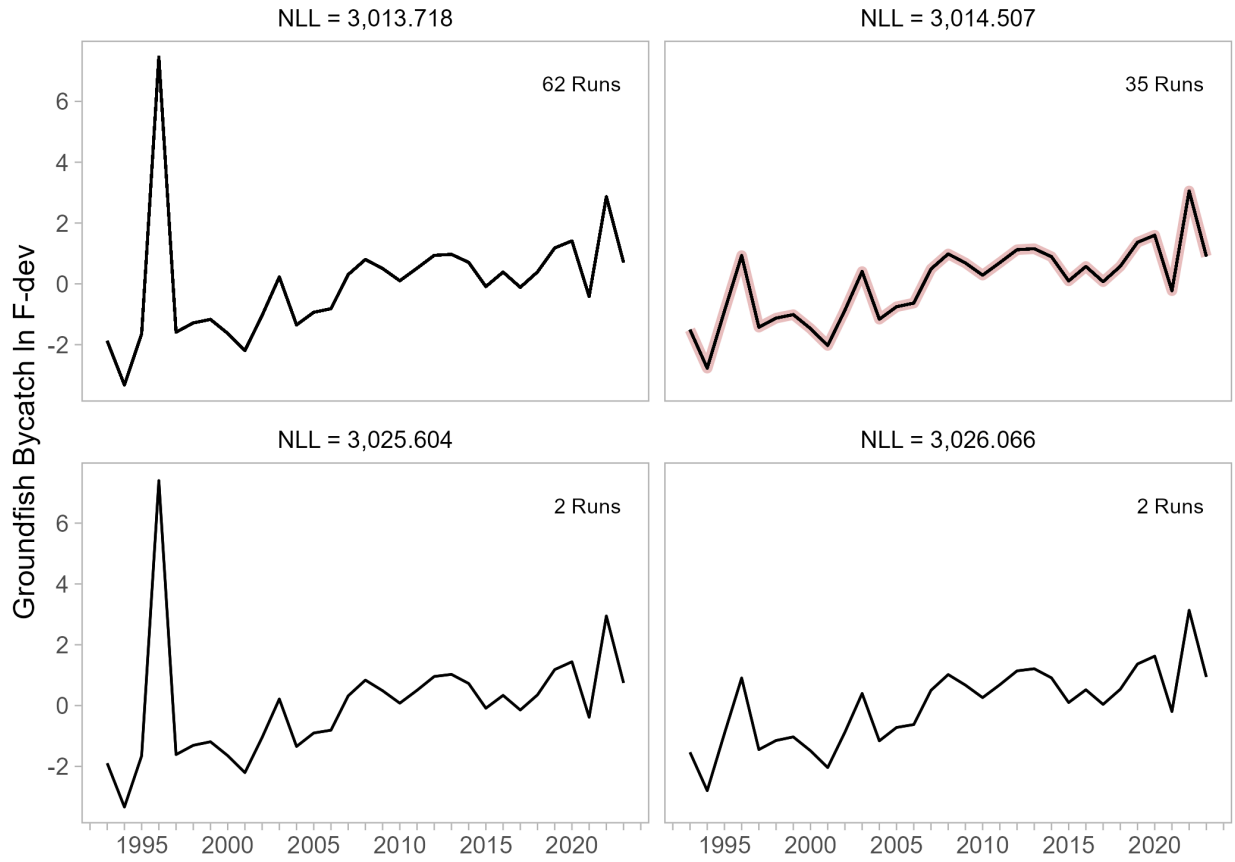
Figure 37: Log deviations for annual fishing mortality in the groundfish bycatch fleet for model WAG 23.1, by NLL minima reached in jitter runs. The red line indicates log deviations estimated by the MLE model.
