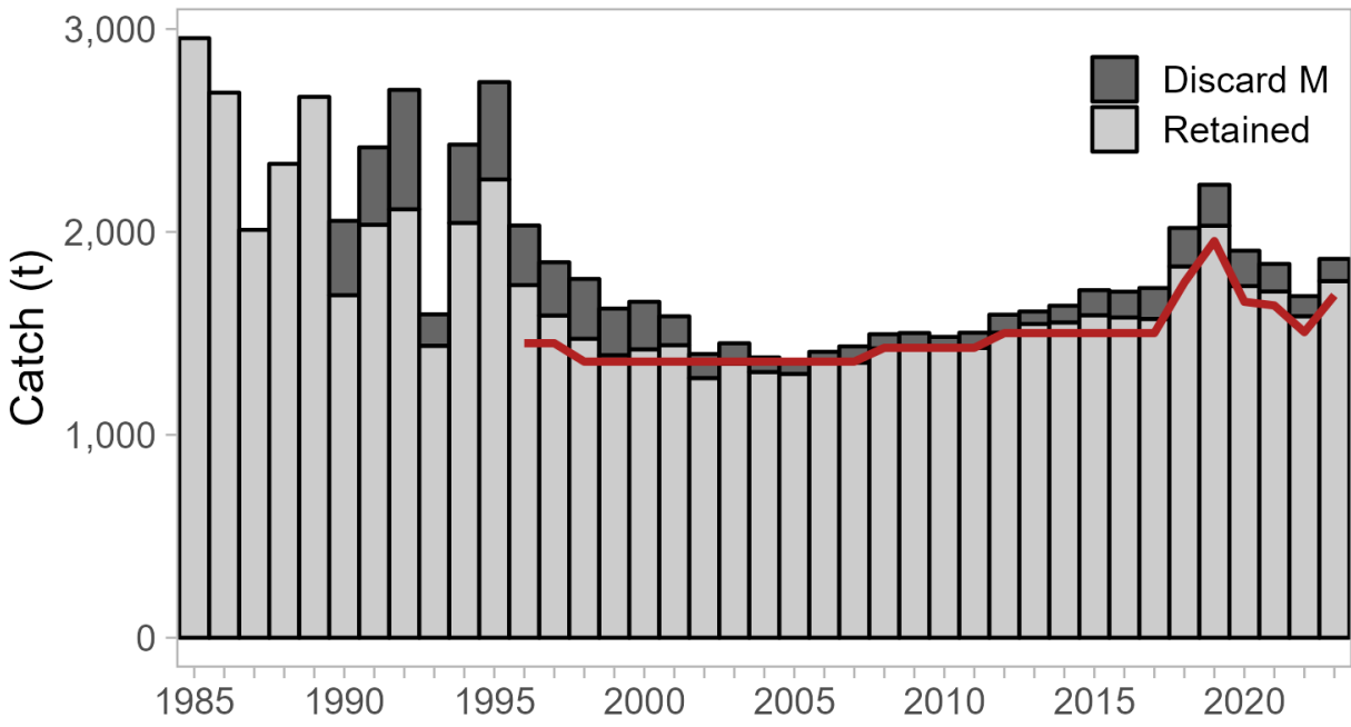
Figure 2: Time series of retained catch (t), directed fishery discard mortality (t), and the total allowable catch (t; red line) in the EAG.
