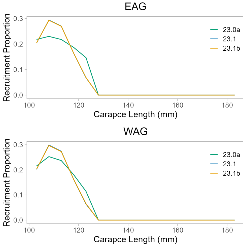
Figure 22: Comparison of model estimated recruitment size distribution.
