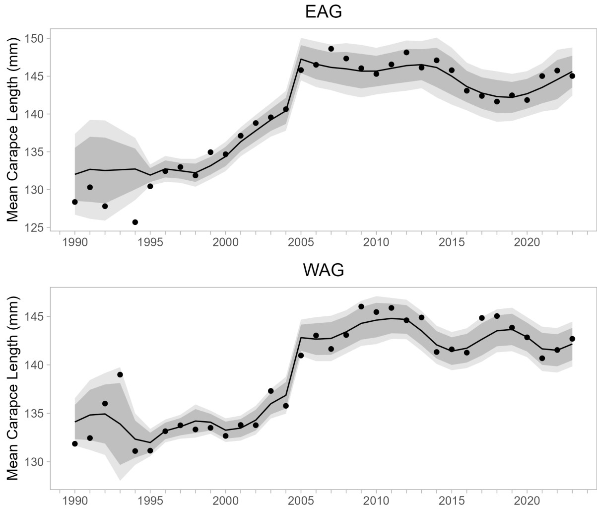
Figure 18: Fit to mean size of total catch crab and associated 95% CI based on observed (dark grey) and estimated (light grey) effective sample sizes for model 23.1.
