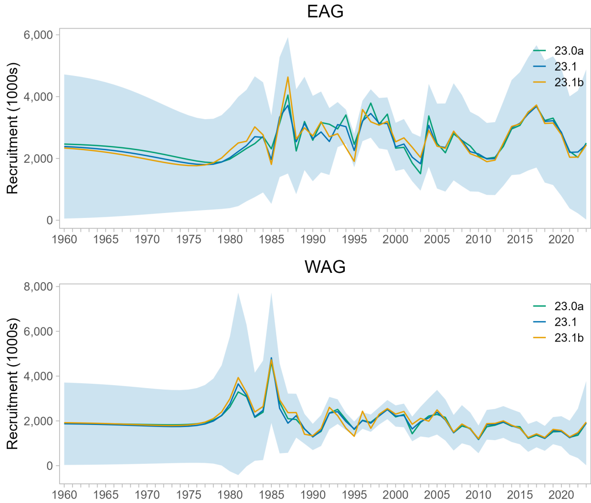
Figure 23: Comparison of model estimated recruitment. Shaded area represents the 95% confidence interval for model 23.1.
