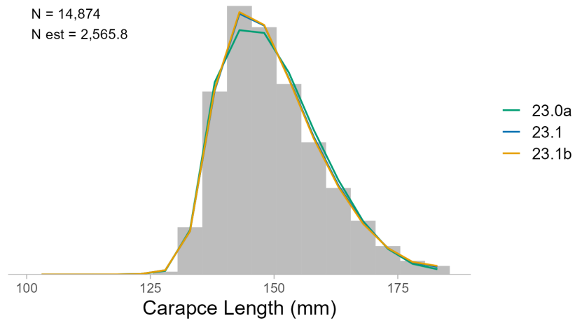
Figure 11: Comparison of model fit to aggregated retained catch size composition in the EAG. Estimated effective sample sizes are for model 23.1.
