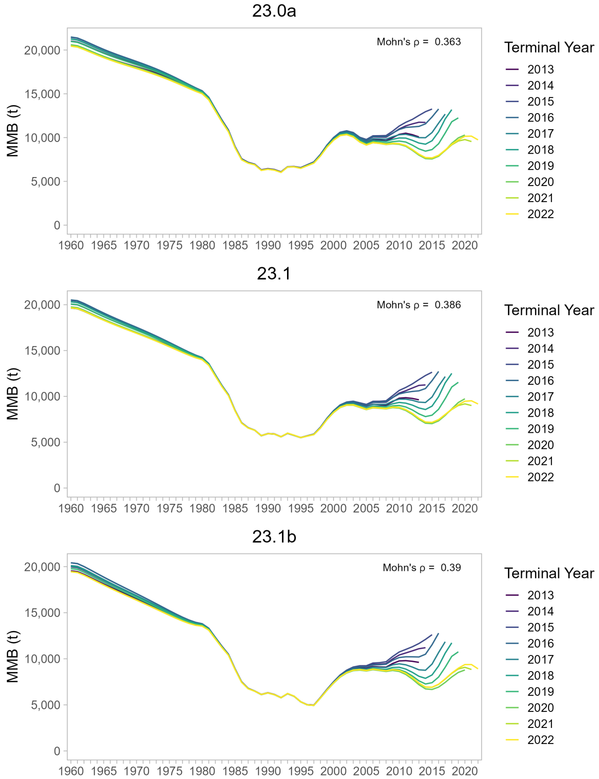
Figure 30: Estimated MMB and associated Mohn's \rho from retrospective analysis of EAG models 23.0a, 23.1, and 23.1b.
