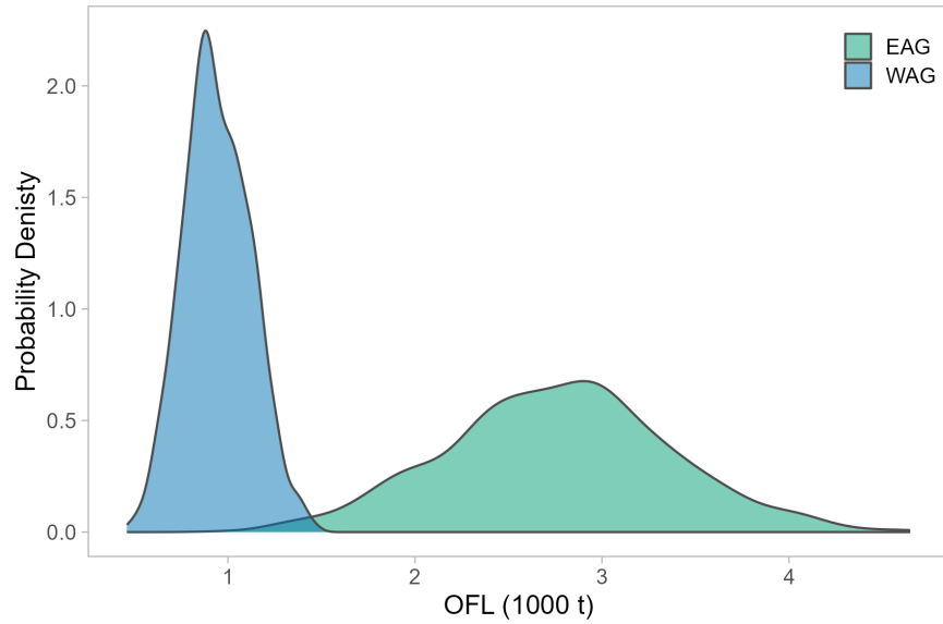
Figure 39: Distrubition of OFL (1000 t) based on MCMC for model 23.1.
