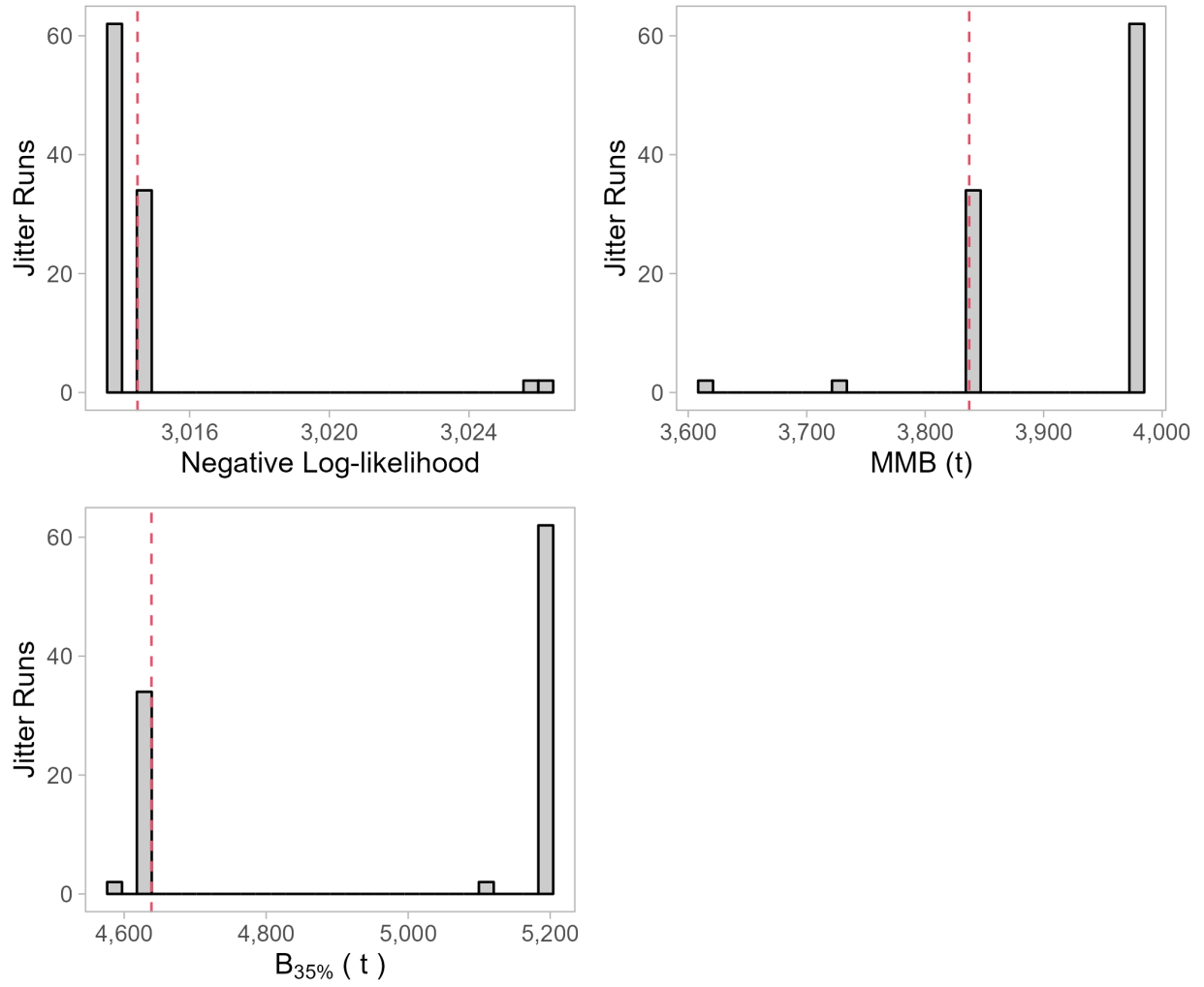
Figure 34: Distrubution of total NLL, mature male biomass, and B_{35\%} for 100 jitter runs of model WAG 23.1. The dotted line is the MLE model.
