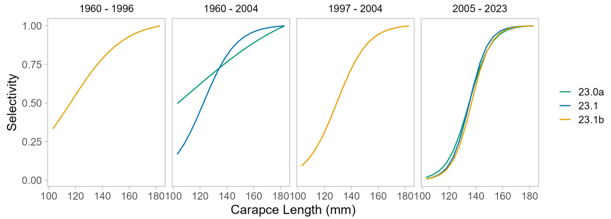
Figure 19: Comparison of estimated selectivity for the directed fishery in the EAG. Model 23.0a is the base model with updated data, 23.1 truncates the size composition, 23.0a uses alternative size composition weights, and 23.1b uses an additional selectivity period.
