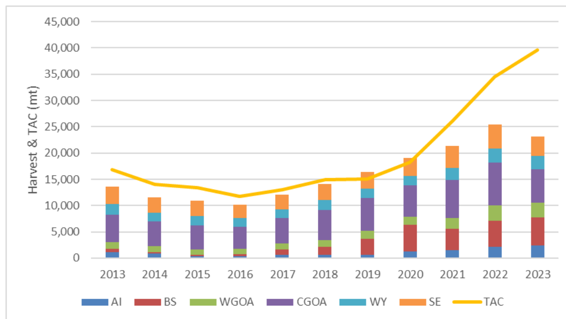
Figure 3-1 Sablefish harvest (mt) by FMP subarea and total allowable catch (mt) for all FMP subareas combined, 2013 through 2023
