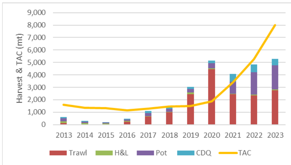
Figure 3-3 BS sablefish TACs and harvest (mt) by sector from 2013 through 2023
