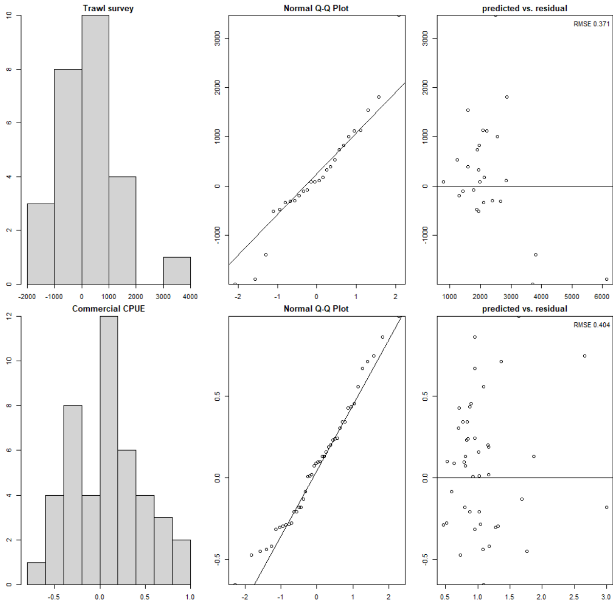
Residuals Histogram, Q-Q Plot, Predicted vs. Residual: Gmacs
