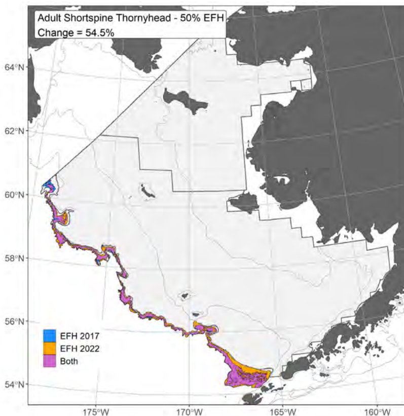
Figure 51. Change in 50% CEA, 2017 compared to 2022 - EBS Shortspine thornyhead rockfish.
