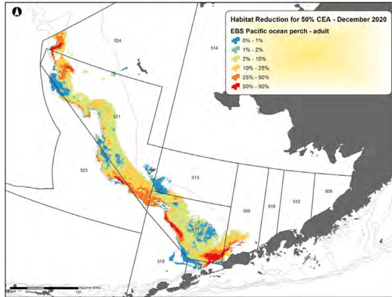
Figure 37. Proportion of habitat disturbance, December 2020 - EBS Pacific ocean perch.
