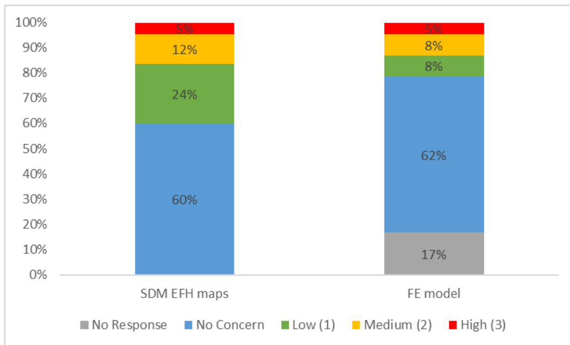
Figure 8: Ranked concerns by qualitative score ( low (1), medium (2), high (3) ) reported by stock authors in the 2022 FE Assessment Questionnaire for the SDM ensemble EFH maps representing the summer distribution for their species or species complexes (left), and the FE model results representing the effects of fishing on their species' or species complex's CEA (right).
