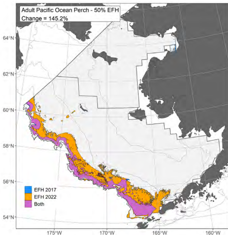
Figure 39. Change in 50% CEA, 2017 compared to 2022 - EBS Pacific ocean perch.
