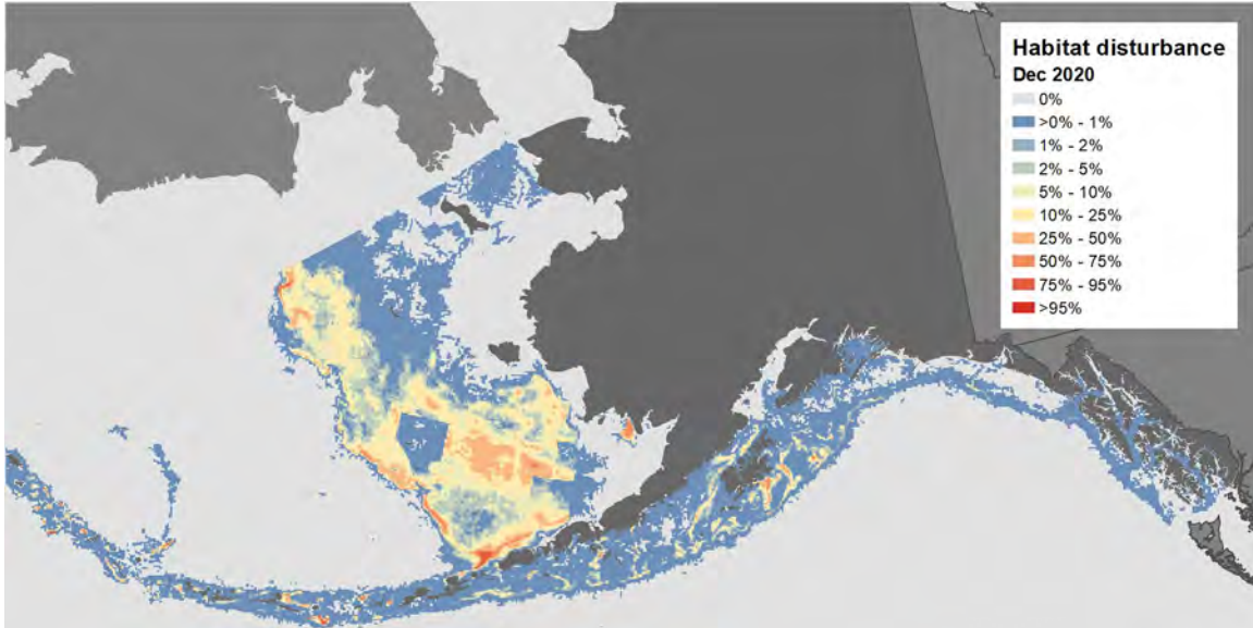
Figure 2. Eastern Bering Sea cumulative percentage habitat disturbed. All gears combined.
