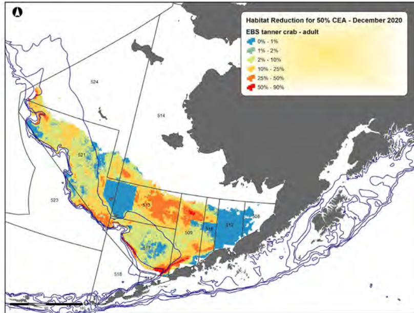
Figure 65. Proportion of habitat disturbance, December 2020 - EBS Tanner Crab.
