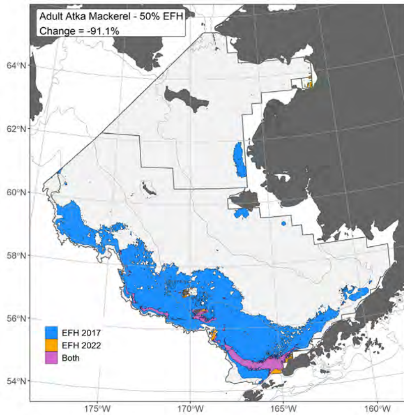
Figure 16. Change in 50% CEA, 2017 compared to 2022 - EBS Atka mackerel.
