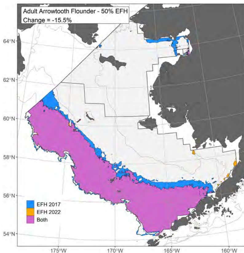
Figure 11. Change in 50% CEA, 2017 compared to 2022 - EBS adult arrowtooth flounder.
