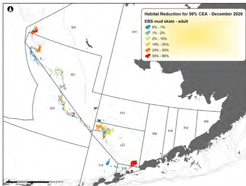
Figure 60. Proportion of habitat disturbance, December 2020 - EBS Mud Skate.
