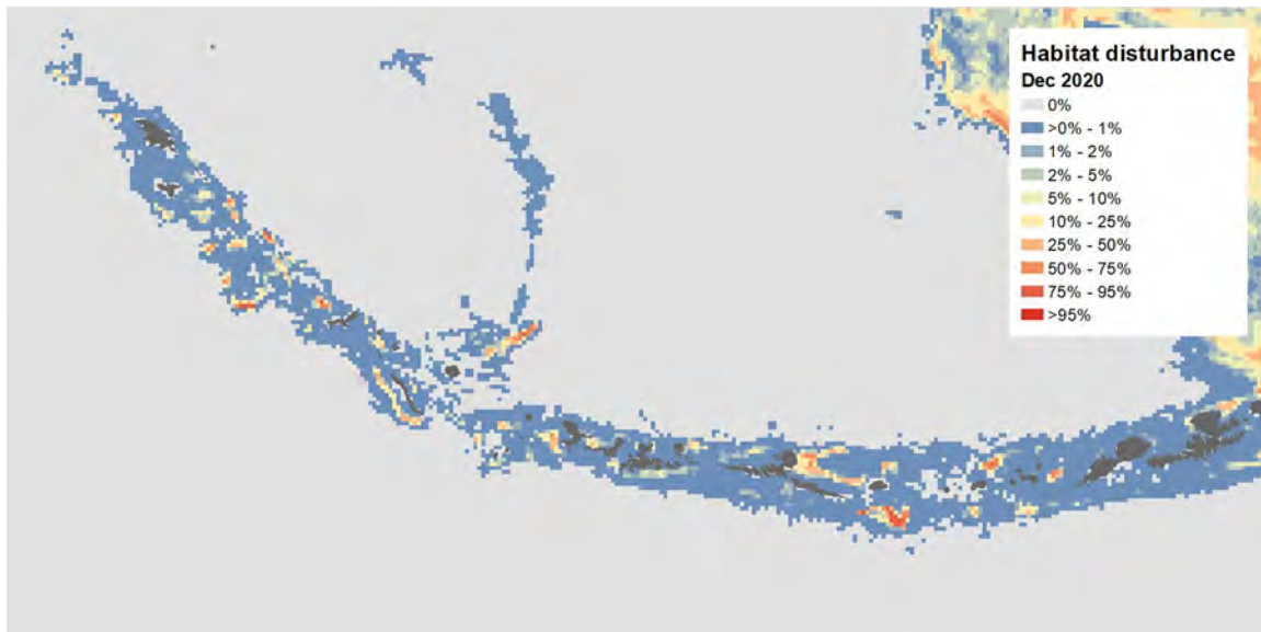
Figure 1. Aleutian Islands cumulative percentage habitat disturbed. All gears combined.
