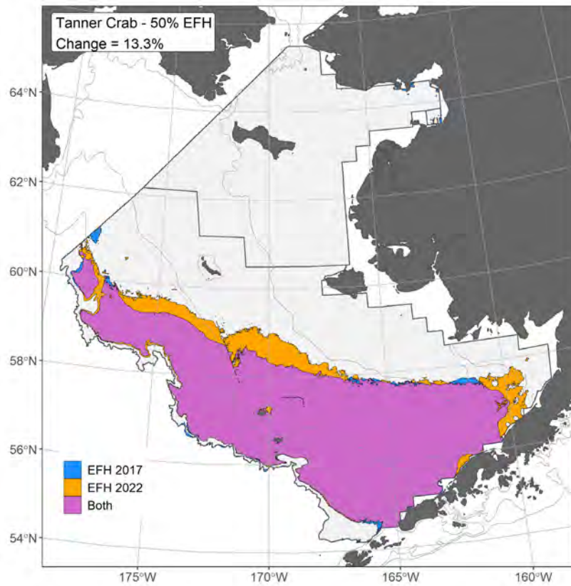
Figure 67. Change in 50% CEA, 2017 compared to 2022 - EBS Tanner Crab.
