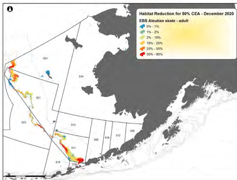
Figure 54. Proportion of habitat disturbance, December 2020 - EBS Aleutian skate.
