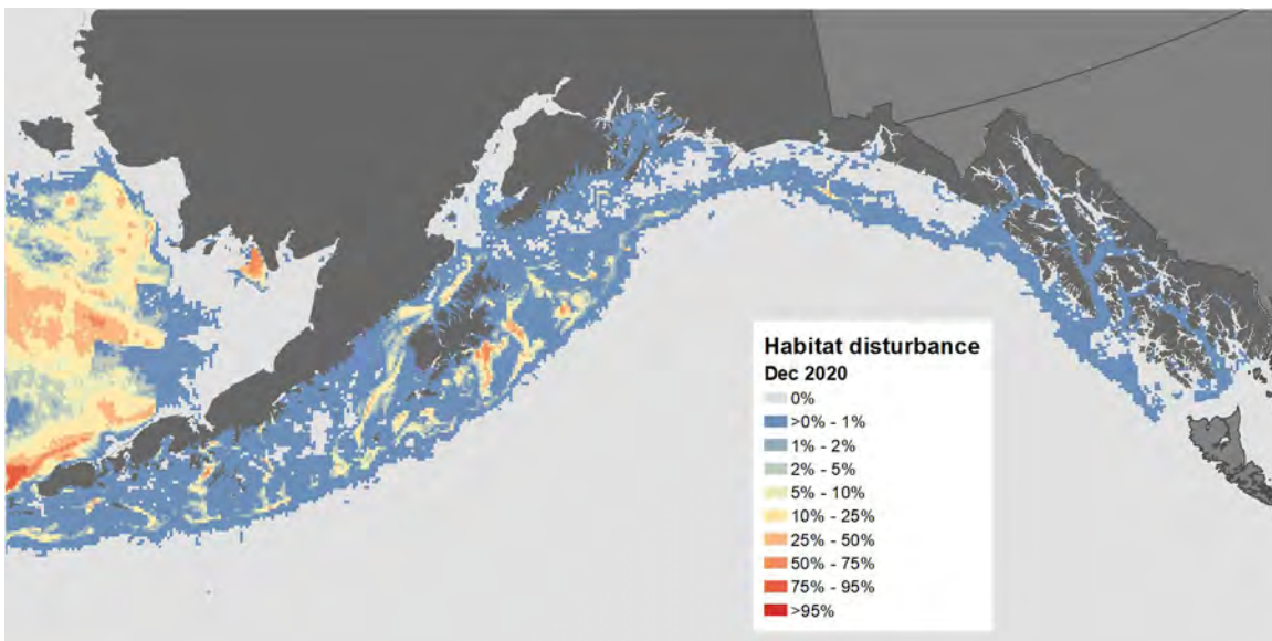
Figure 3. Gulf of Alaska cumulative percentage habitat disturbed. All gears combined.
