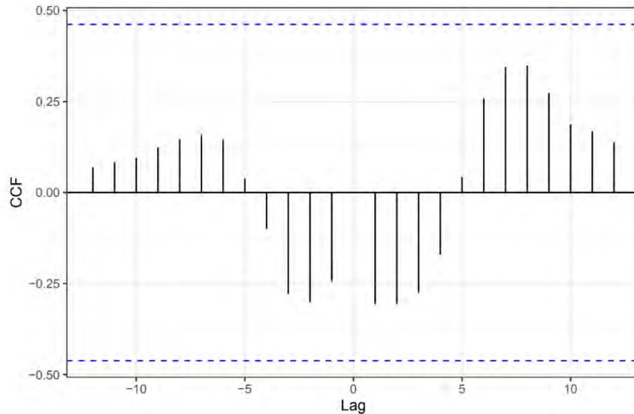
Figure A5.17. Cross-correlation between the observed probability of having undergone terminal molt at 75 mm carapace width and the mean fishing disturbance.
