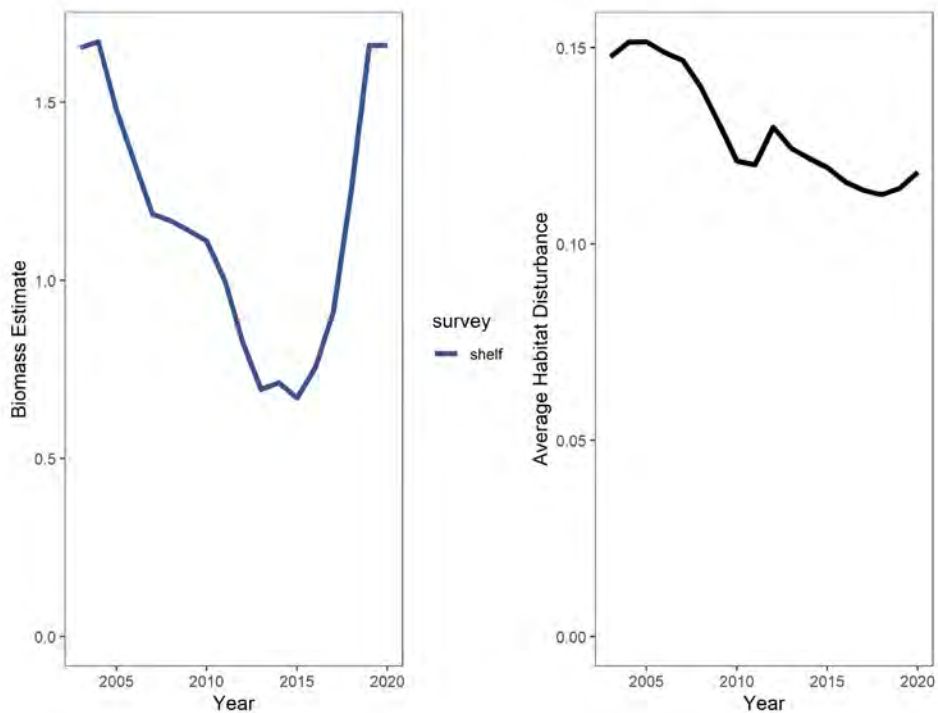
Figure 30. EBS rex sole biomass over time (as estimated in the 2020 Tier 5 assessment; left panel) and habitat disturbance over time (averaged over months within each year; right panel).
