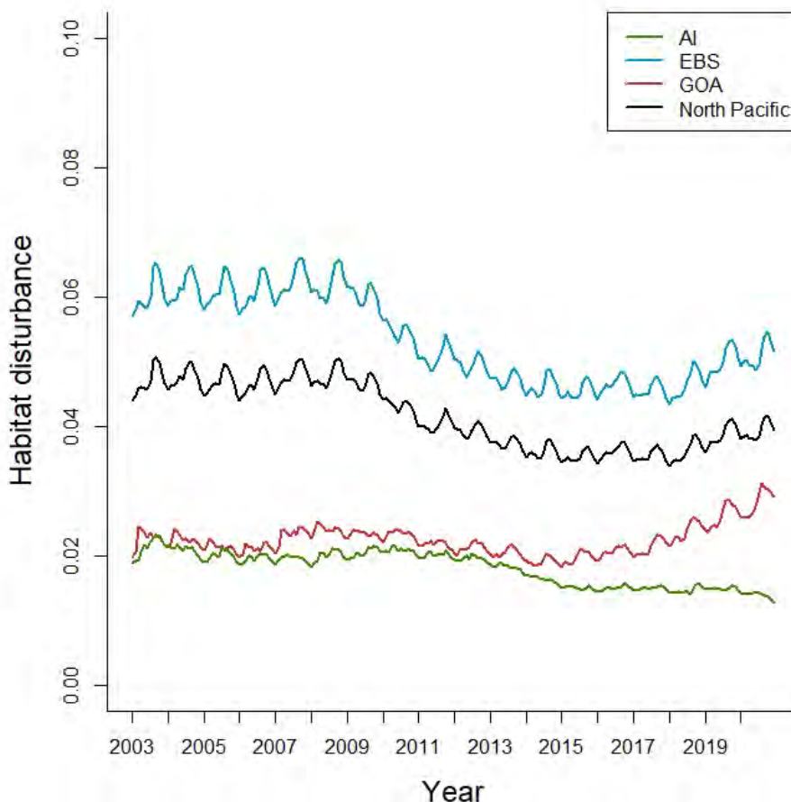
Figure 4. A time-series output of the Fishing Effects Model showing habitat disturbance aggregated for all areas less than 1000 m depth for the Aleutian Islands (AI), Eastern Bering Sea (EBS), Gulf of Alaska (GOA), and the North Pacific at large.
