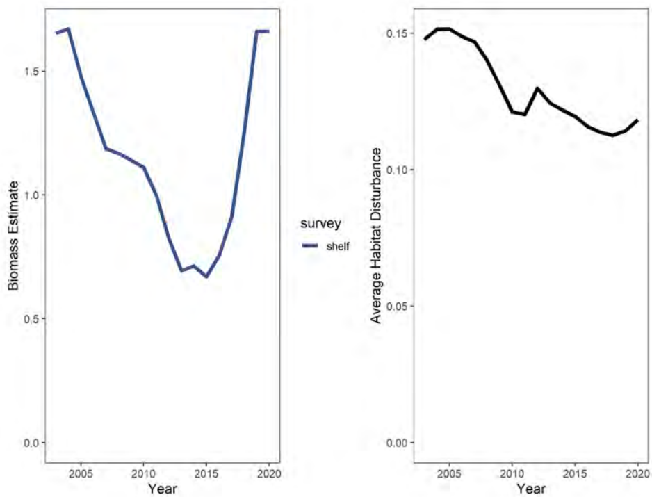
Figure A5.7. EBS rex sole biomass over time (as estimated in the 2020 Tier 5 assessment; left panel) and habitat disturbance over time (averaged over months within each year; right panel).
