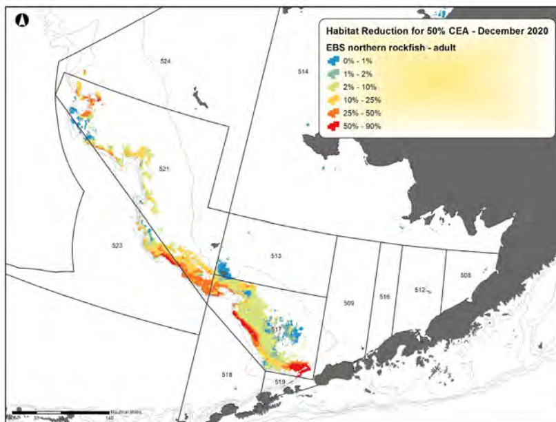
Figure 33. Proportion of habitat disturbance, December 2020 - EBS Northern rockfish.
