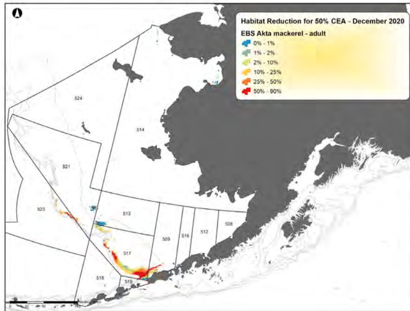
Figure 14. Proportion of habitat disturbance, December 2020 - EBS Atka mackerel.
