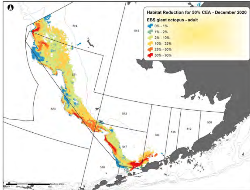
Figure 20. Proportion of habitat disturbance, December 2020 - EBS Giant octopus.
