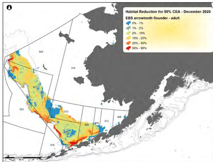
Figure 9. Proportion of habitat disturbance, December 2020 - EBS adult arrowtooth flounder.
