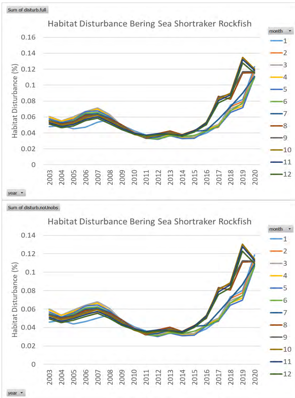
Figure 47. Habitat disturbance by month and year for shortraker rockfish in the Bering Sea for the observed plus unobserved model (top graph, sum of disturb.full) and observed only model (bottom graph, sum of disturb.noUnobs).
