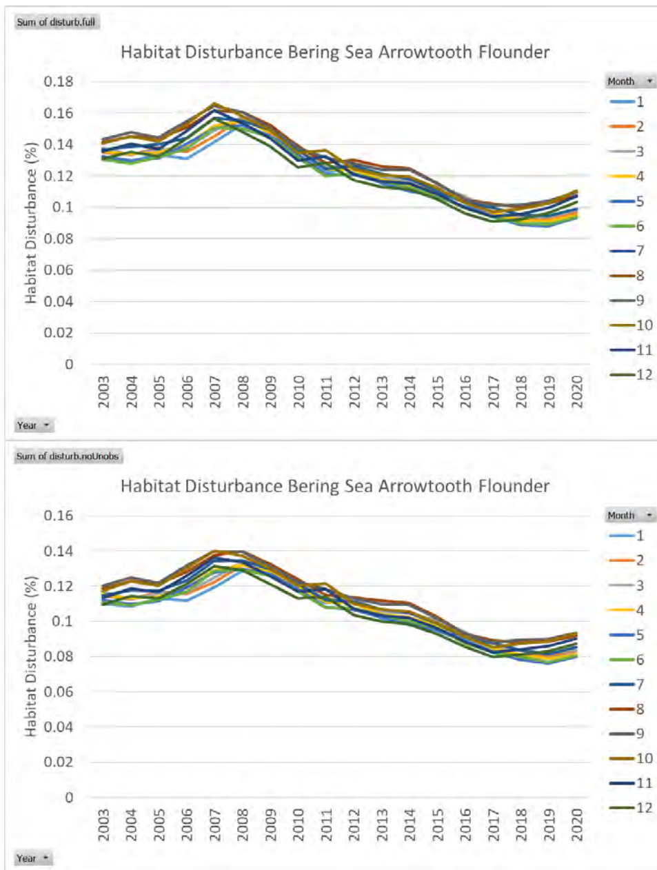
Figure 12. Habitat disturbance by month and year for arrowtooth flounder in the Bering Sea for the observed plus unobserved model (top graph, sum of disturb.full) and observed only model (bottom graph, sum of disturb.noUnobs).
