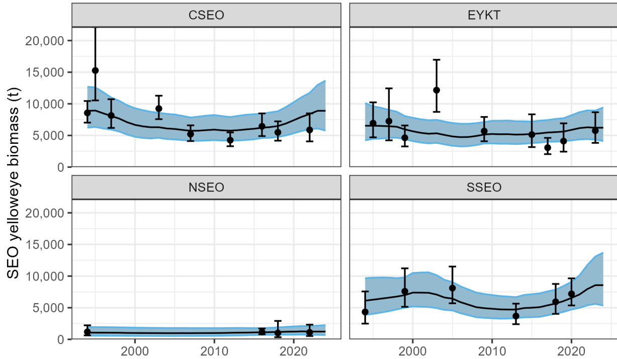
Figure 14.17: Model 22.2 fits to the Alaska Department of Fish and Game (ADFG) submersible and remotely operated vehicle (ROV) survey yelloweye rockfish biomass estimates by management unit.
