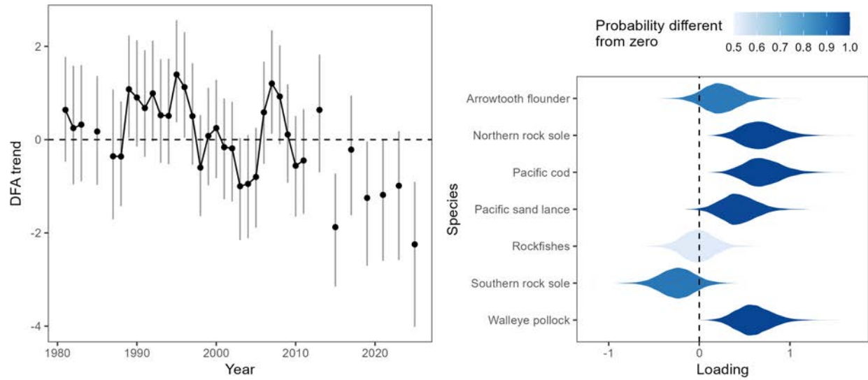
Figure 48: Estimated shared trend of the multispecies larval DFA and loadings of the 7 larval fish taxa on the time trend.
