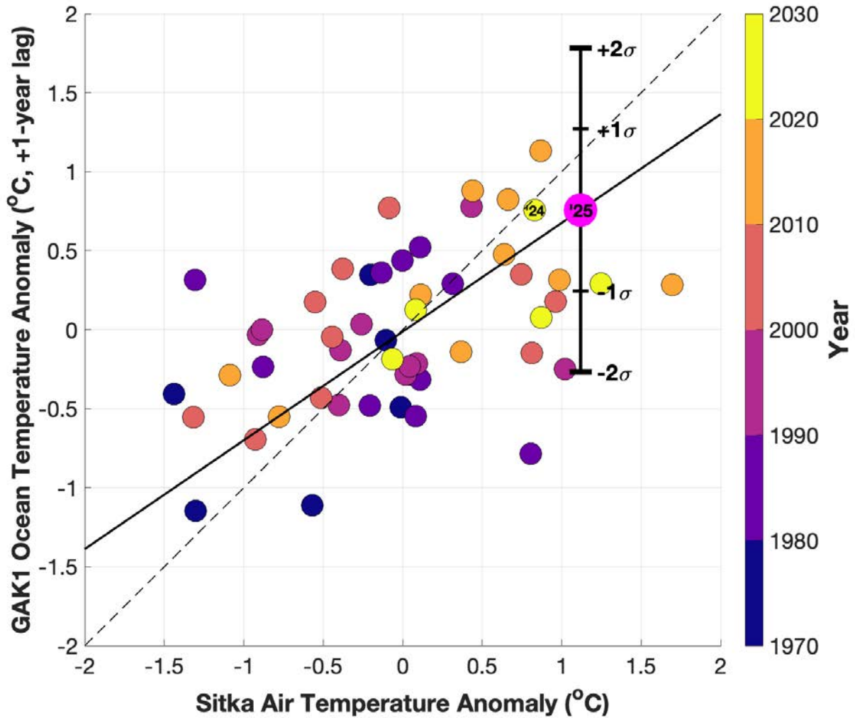
Figure 9: Relationship between the detrended annual Sitka air temperature anomaly (x axis) and the following-year whole water column ocean average temperature anomaly measured at station GAK1 (y axis), with a +1 year lag compared to Sitka. Dashed black line shows a 1:1 slope and the solid black line is the least squares best fit line between the two records. Both anomalies are referenced to the average temperature from the early 1970s to present (1971 for GAK1, 1973 for Sitka air). The blue to yellow dots show each yearly comparison between Sitka air anomaly and the next year's GAK1 anomaly. The pink dot shows the 2025 air temperature anomaly (through August 12th, 2025). The error bars show one and two standard deviations of variability from the trend line (solid black line, the dashed line is 1:1), for bounds on the expected water temperature at GAK1 in 2026.
