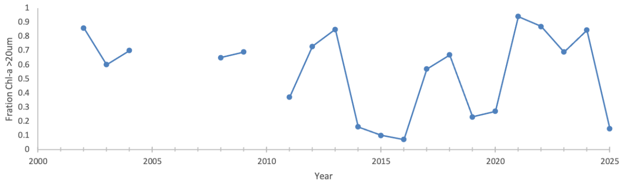
Figure 33: May 2001–2025 time series of phytoplankton size index (fraction of total chl-a present in cells >20\ \mu\text{m} ) for the Seward Line shelf stations.
