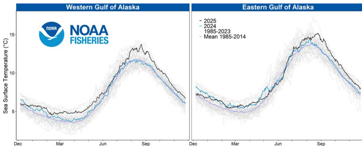
Figure 12: Daily sea surface temperatures (SST) for the western GOA and eastern GOA. Lines illustrate the daily SST for 2025 through December 2 (black), the daily SST for 2024 (blue), the 30-year (1985 – 2014) mean SST for each day (purple), and daily SST for each year of the time series (1985 – 2023; gray). Details are in the “Methods” section at the end of this contribution.
