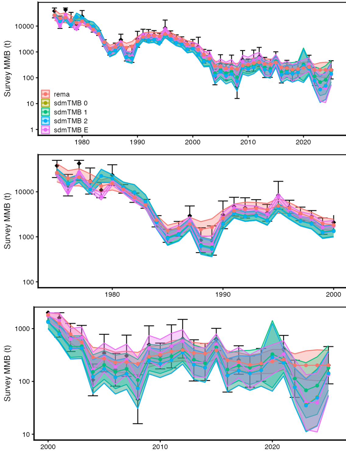
Figure 48. Comparison of sdmTMB and rema model-based indices (colored points, lines, and regions) and design-based indices (black dots and error bars). The last character of the “ sdmTMB ”-labelled indices indicates the fine scale prediction grid (0, 1, or 2) or the original haul locations (“E”) used to obtain the area-expanded survey MMB. The shaded areas represent 80% confidence intervals, as do the error bars. Upper plot: full time series; middle plot: 1975-2000; lower plot: 2000-current year.
