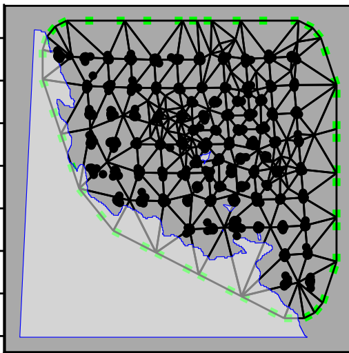
kmeans 80
