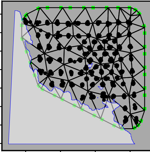
kmeans 60
