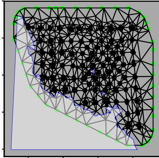
CT 10km
