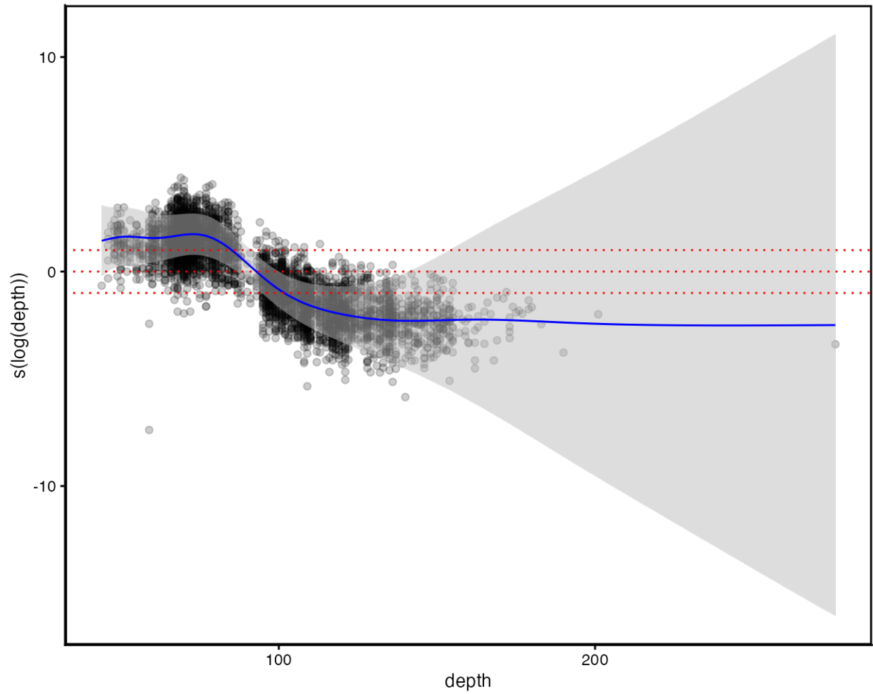
Figure 44. Estimated smooth function of \ln(\text{bottom depth}) as a main effect covariate, on the link ( \ln ) scale. Line: estimated effect; shading: 95% confidence intervals; points: residuals; horizontal dotted lines are plotted at link-scale values of -1, 0, and 1.
