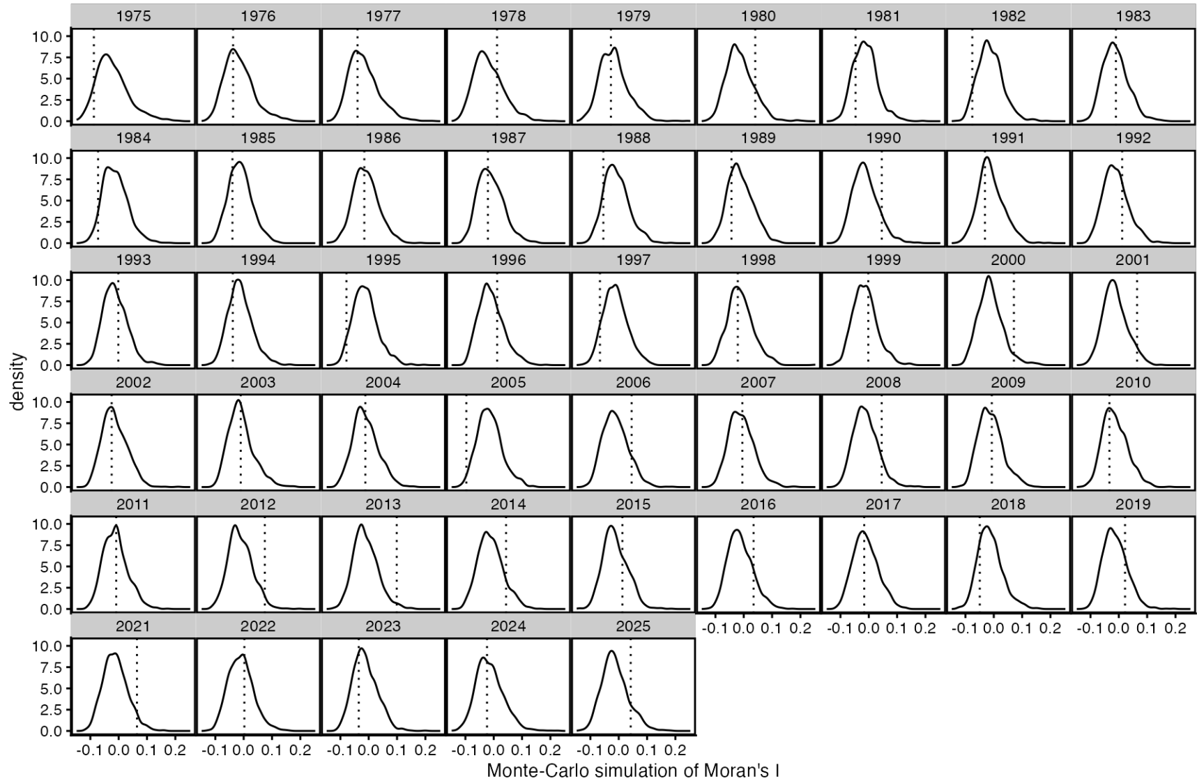
Figure 47. Monte-Carlo (permutation) simulation results for Moran's I, which tests for spatial autocorrelation, by year. Solid line: distribution of statistic under null hypothesis of no spatial autocorrelation. Dotted vertical line: value of realized statistic.
