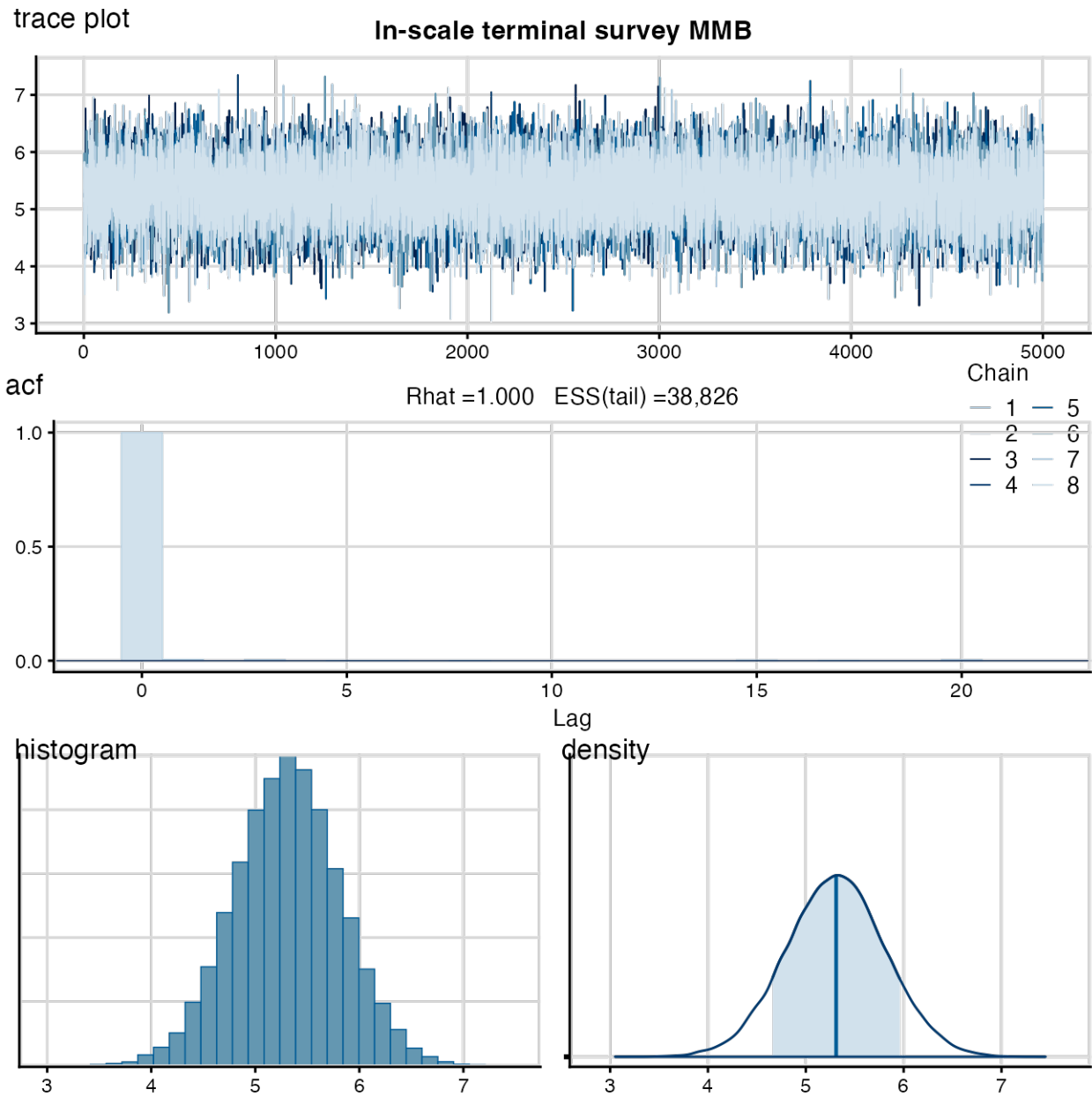
Figure 34. MCMC diagnostics for the In-scale terminal year survey MMB from the “zeros as NAs” model. Top row: trace plot; center row: autocorrelation plot; bottom row: histogram (left) and estimated posterior density with median (vertical line) and 80 percent confidence interval (shading). \hat{r} ( <1.05 ) and ESS ( >100 ) are measures of acceptable MCMC mixing.
