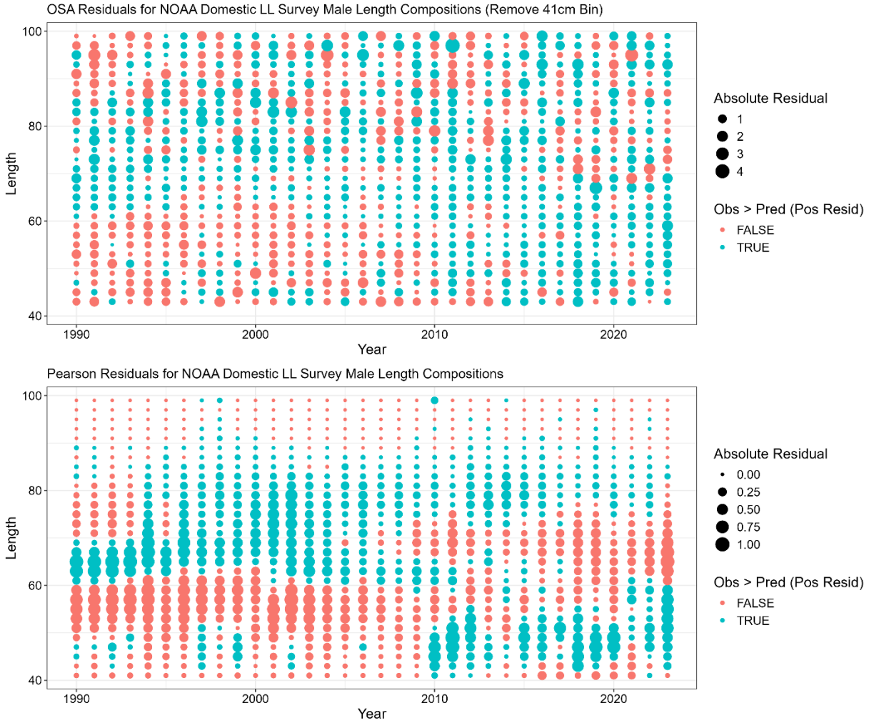
Figure 3C.6. NOAA domestic longline survey male length composition one step ahead (OSA; top row) and Pearson residuals (bottom row). Color denotes negative (red) or positive (blue) residuals. For OSA residuals the first size class was removed.
