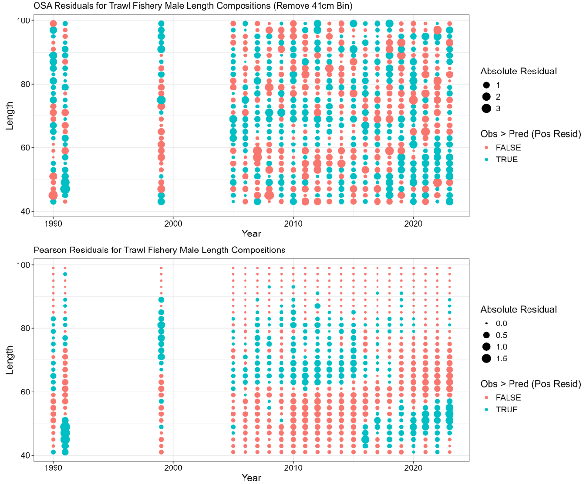
Figure 3C.12. Domestic trawl gear fishery male length composition one step ahead (OSA; top row) and Pearson residuals (bottom row). Color denotes negative (red) or positive (blue) residuals. For OSA residuals the first size class was removed.
