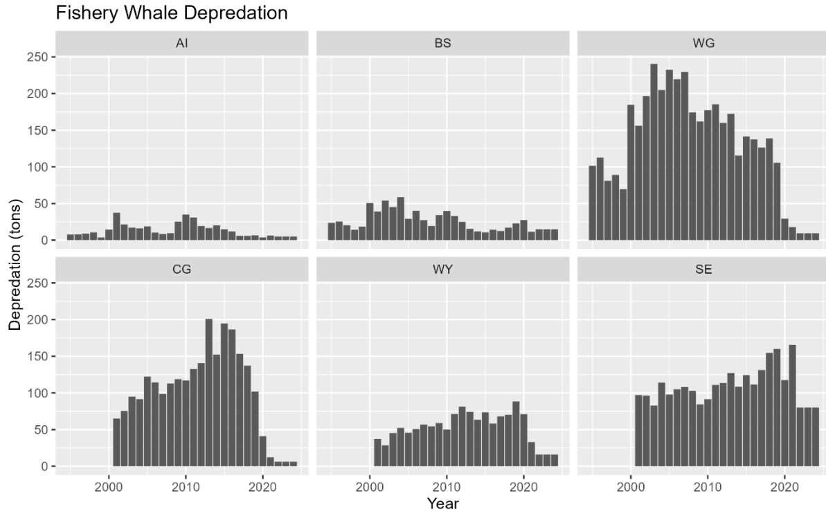
Figure 3.7. Estimated whale depredation in the sablefish fixed gear fishery. Depredation estimates reflect catch removals (tons) by region (panel) due to orcas (top row) and sperm whales (bottom row). Starting in 2023 estimates were held constant at 2022 values.
