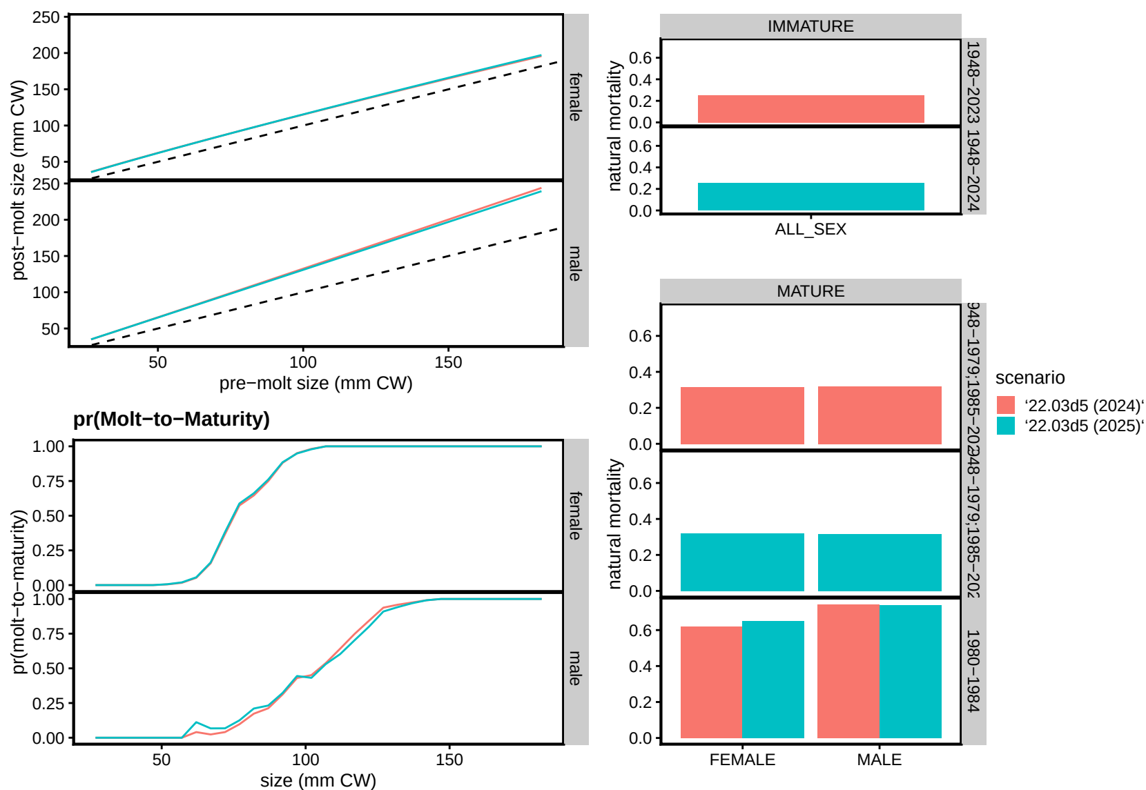
Figure 62. Estimated population processes. Plots in upper lefthand quadrant: sex-specific mean growth; plots in lower lefthand quadrant: sex-specific probability of the molt-to-maturity (i.e., terminal molt); plots in righthand column: natural mortality rates, by maturity state and sex. Preferred model is 22.03d5 (2025).
