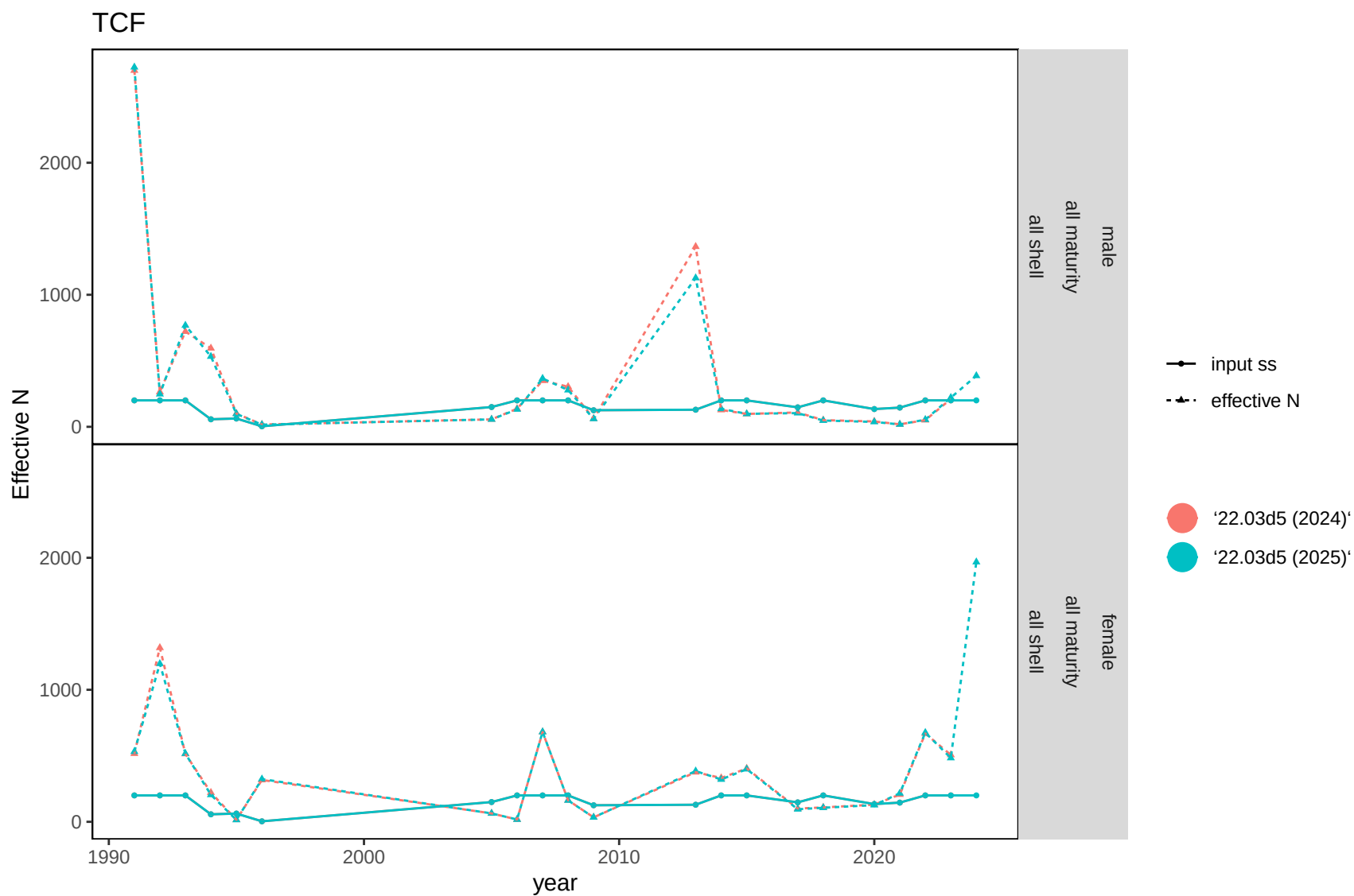
Figure 156. Effective sample sizes compared with input sample sizes for total catch data from the TCF fishery. Dotted lines are effective N's, solid lines are input sample sizes. Input sample sizes are scaled to sum to 200 in each year across categories. Model 22.03d5 (2025) is the preferred model.
