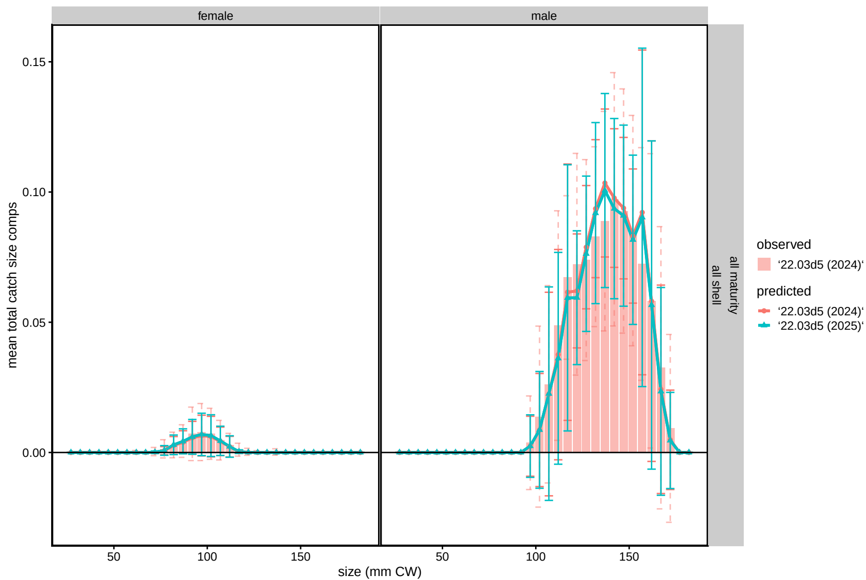
Figure 152. TCSAM02 models fits to mean bycatch size compositions from the BBRKC fishery. Model 22.03d5 (2025) is the preferred model.
