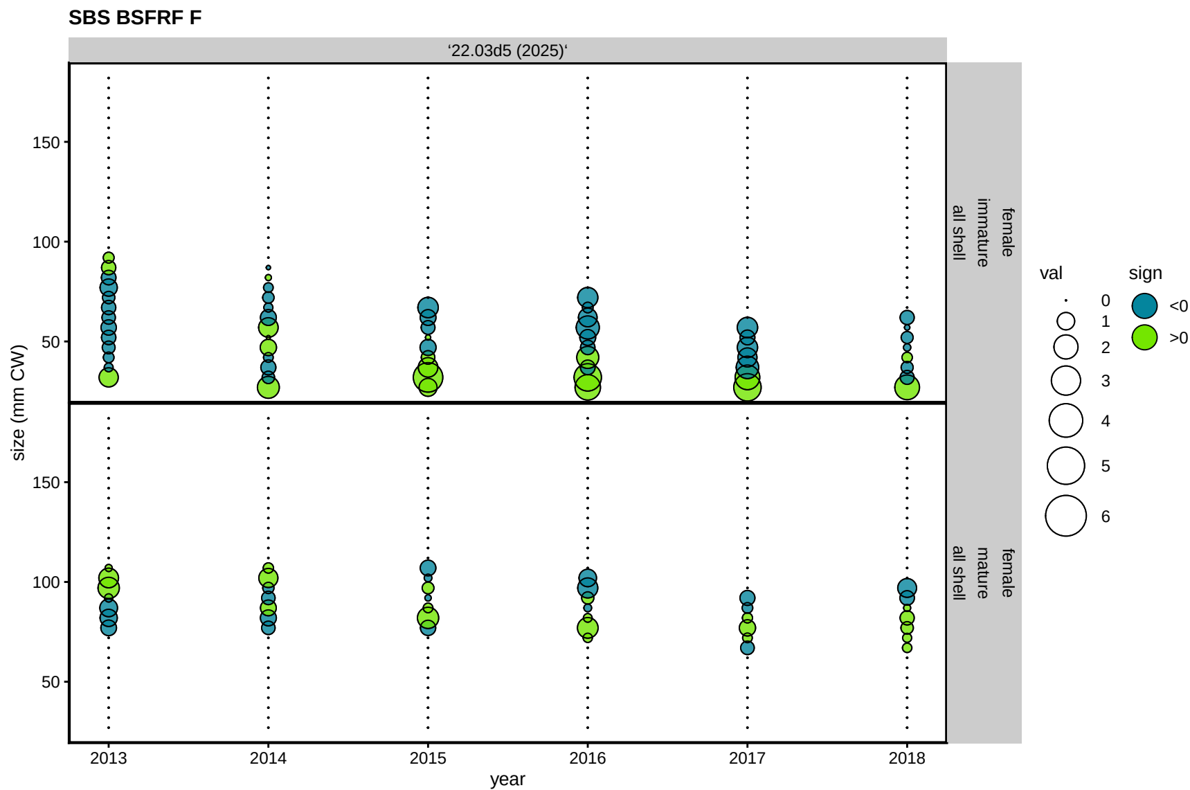
Figure 149. Pearson's residuals for fits to survey size composition in the BSFRF_F survey. Symbol areas reflect the size of each residual, extreme values (residuals larger than 4 in scale) are indicated with a red 'X' to facilitate identification.
