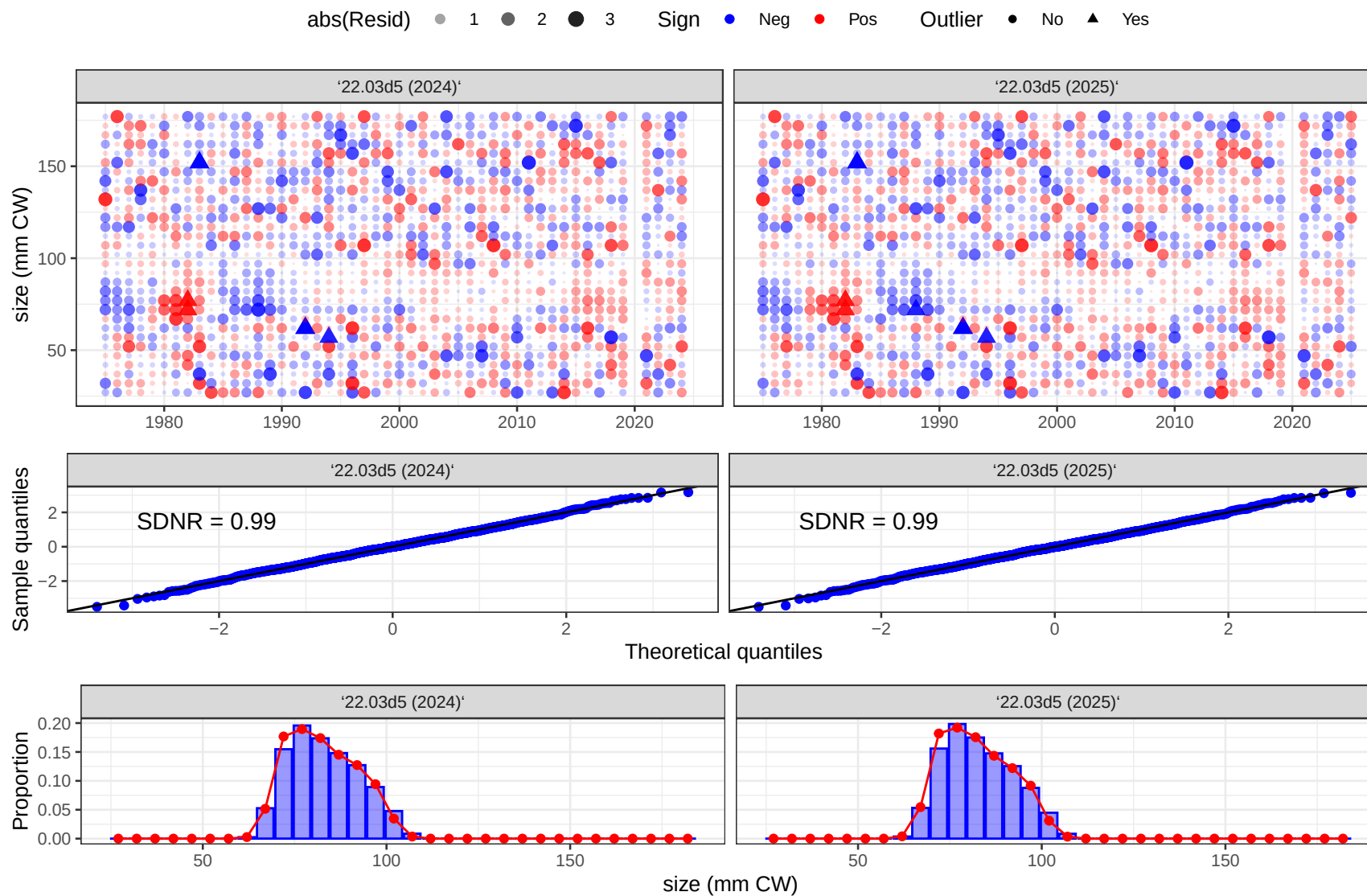
Figure 142. OSA residuals for fits to size compositions from the NMFS_F survey. The base/preferred model is 22.03d5.
