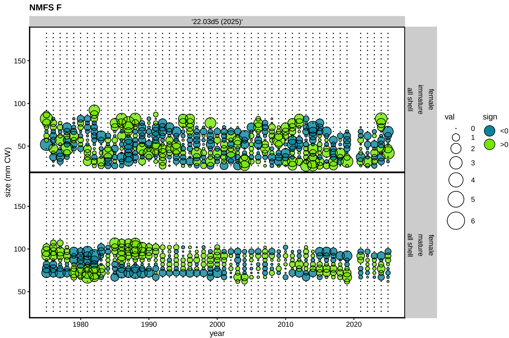
Figure 140. Pearson's residuals for fits to survey size composition data in the TCSAM02 models. Symbol areas reflect the size of each residual, extreme values (residuals larger than 4 in scale) are indicated with a red 'X' to facilitate identification. Preferred model is 22.03d5 (2025).
