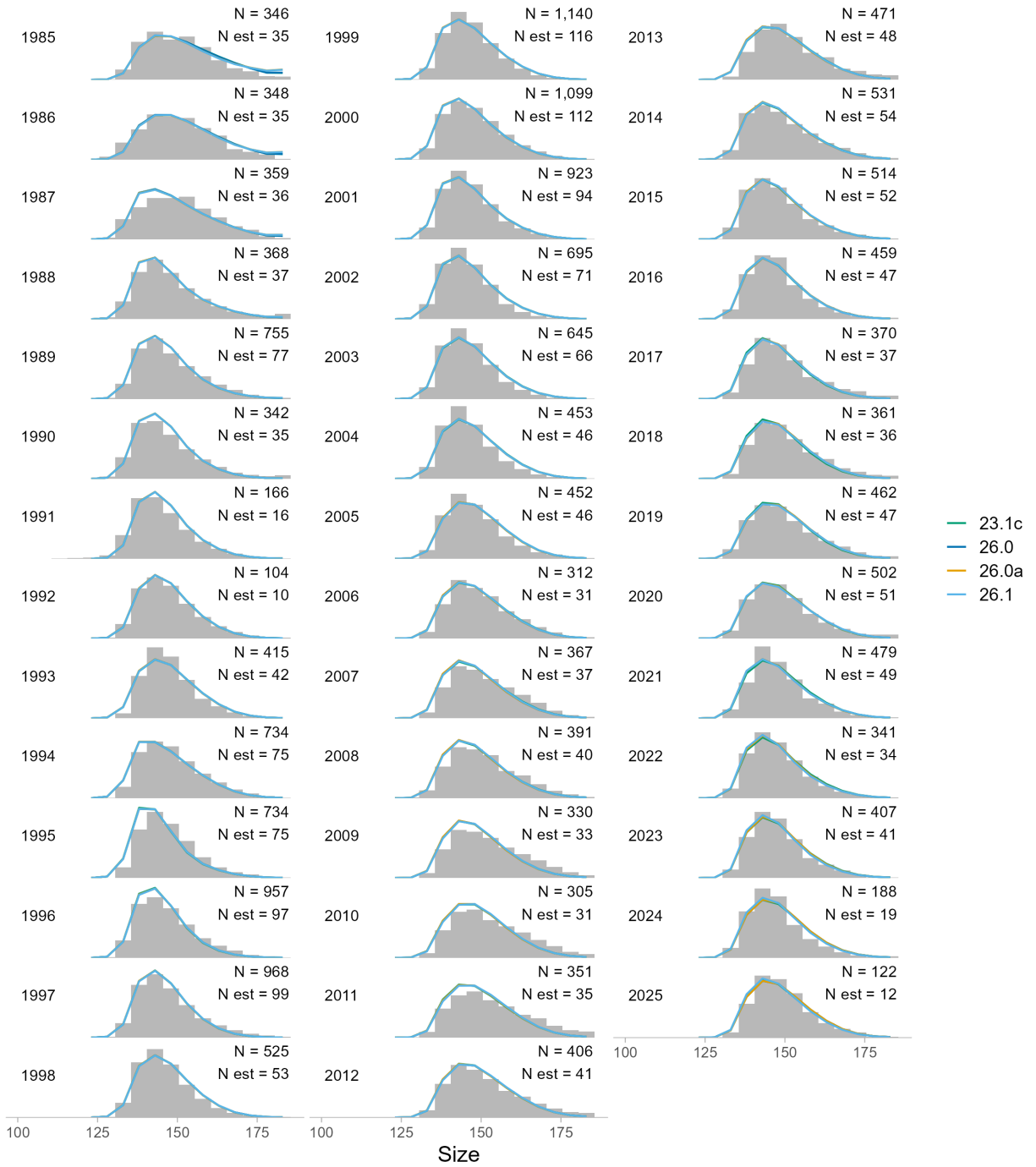
Figure 14: Comparison of model fit to retained catch size composition in the WAG.
