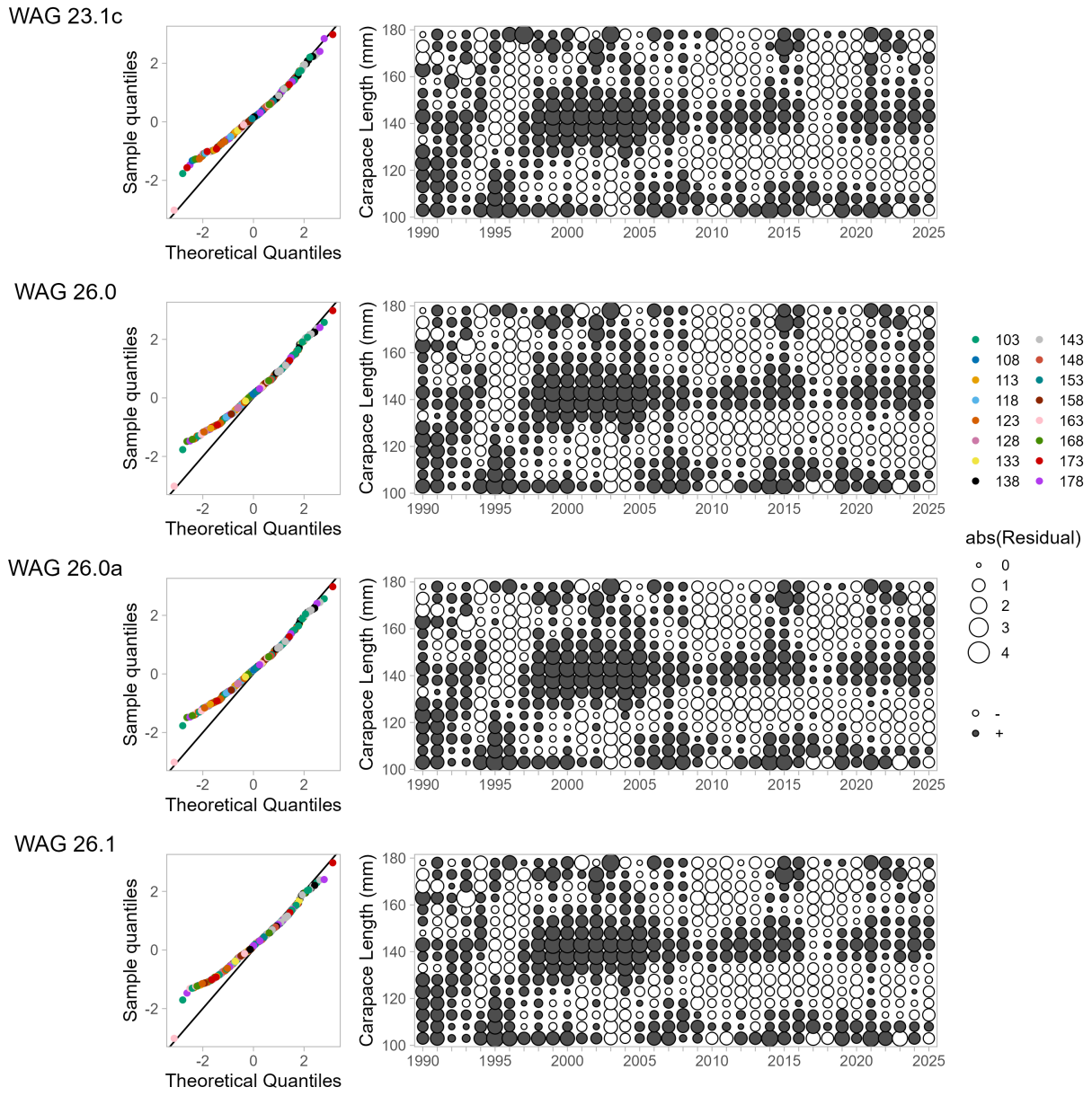
Figure 17: QQ plots and bubble plots for one step ahead residuals for fits to total size composition data among WAG models
