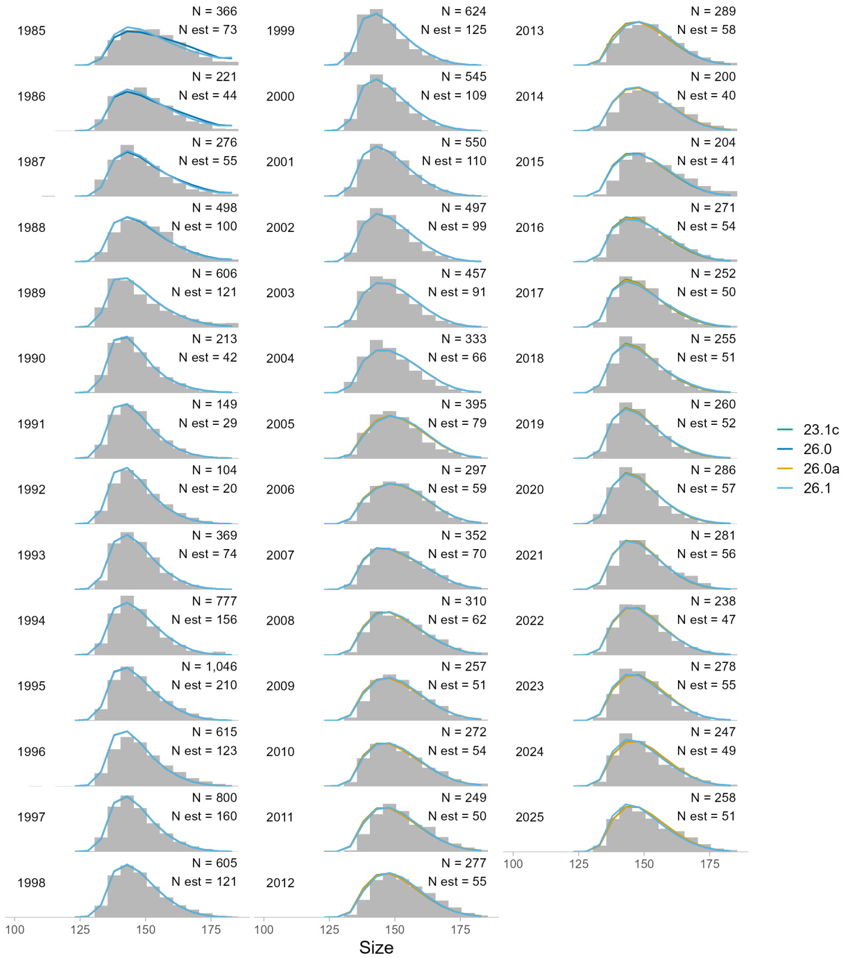
Figure 10: Comparison of model fit to retained catch size composition in the EAG.
