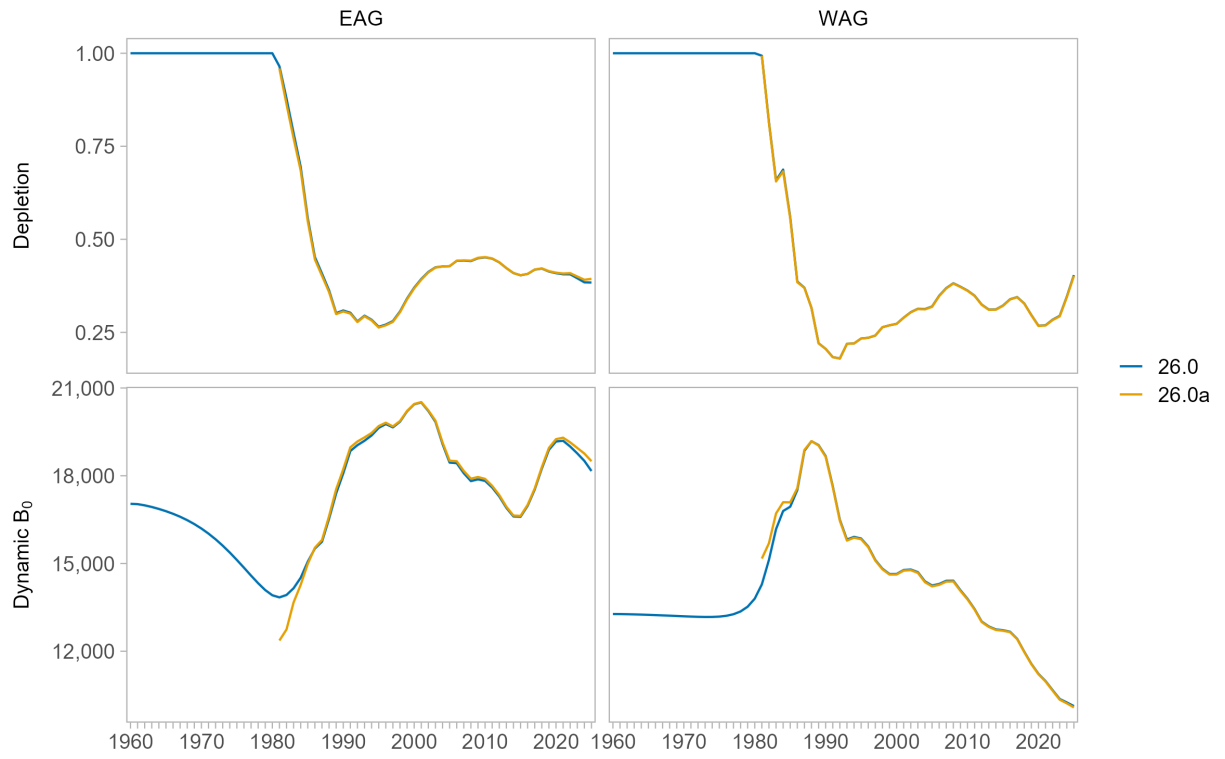
Figure 28: Dynamic B_0 and depletion from models with equilibrium (26.0) and fished (26.0a) initial conditions.
