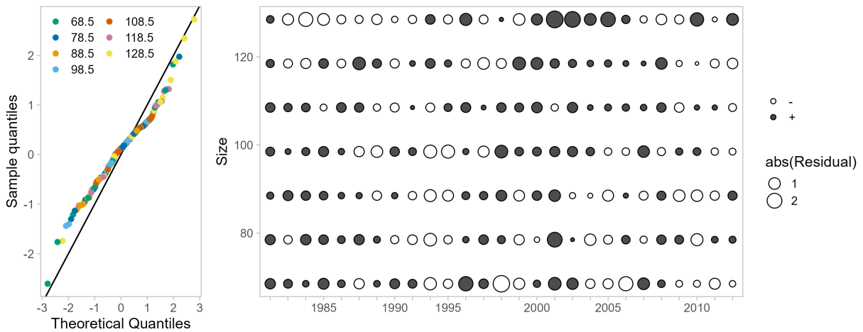
Figure 55: One-Step-Ahead residuals for model 26.1.nd fits to size composition data from the Alaska Department of Fish and Game (ADFG) winter pot survey.
