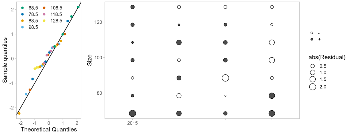
Figure 64: One-Step-Ahead residuals for model 26.2.nd fits to size composition data from the winter commercial fishery retained catch.
