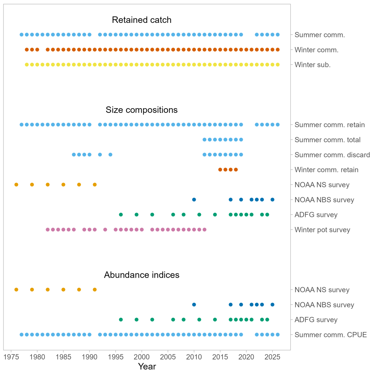
Figure 5: Data sources available for the Norton Sound red king crab stock assessment. Acronyms and abbreviations: National Oceanic and Atmospheric Administration, NOAA; Norton Sound, NS; Northern Bering Sea, NBS; Alaska Department of Fish and Game, ADFG; catch per unit effort, CPUE; comm., commercial; sub., subsistence.
