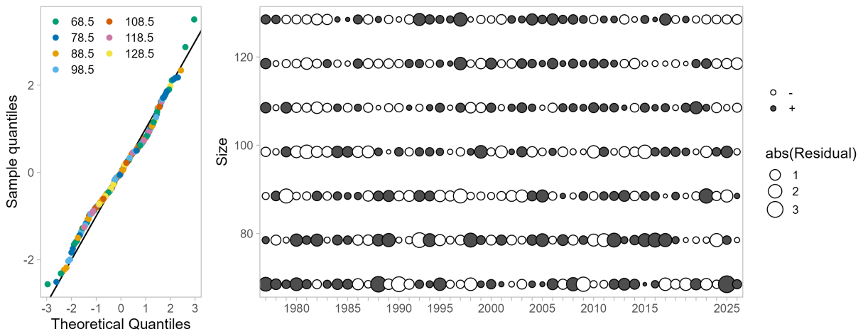
Figure 73: One-Step-Ahead residuals for model 26.2.d fits to size composition data from the summer commercial fishery retained catch.
