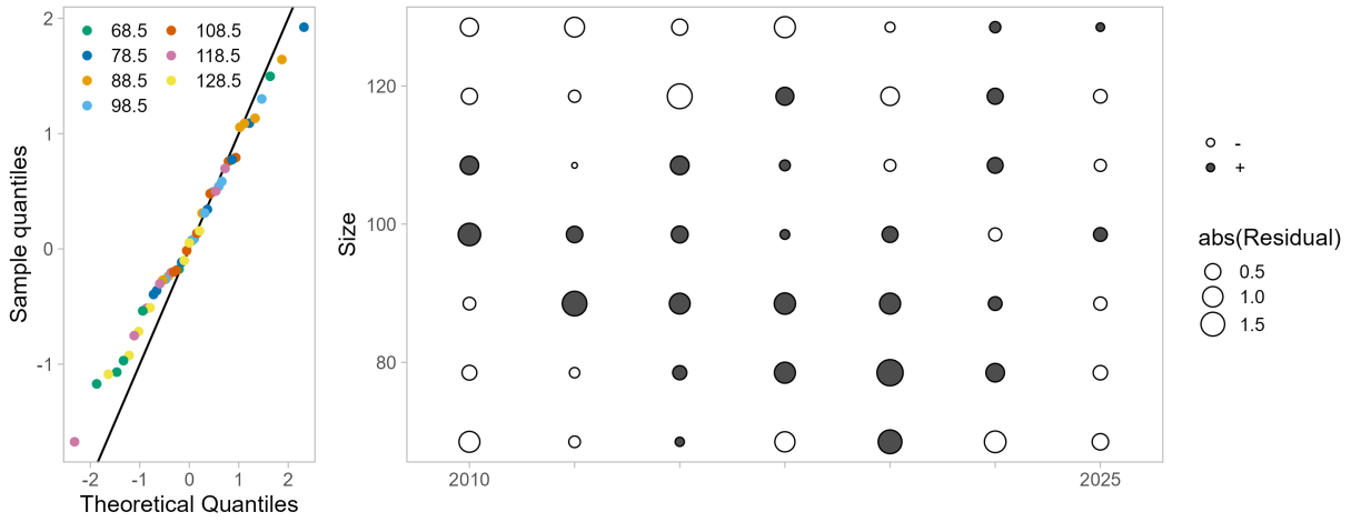
Figure 46: One-Step-Ahead residuals for model 26.0 fits to size composition data from the National Oceanic and Atmospheric Administration (NOAA) Northern Bering Sea (NBS) trawl survey.
