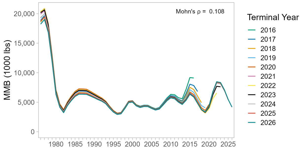
Figure 86: Retrospective patterns in estimated mature male biomass (MMB) for the model using a model-based index of abundance that does not take into account depth (26.1.nd).
