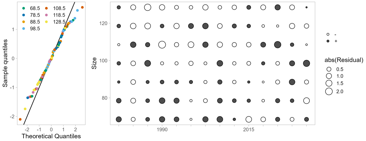
Figure 58: One-Step-Ahead residuals for model 26.1.d fits to size composition data from the summer commercial fishery discarded catch.
