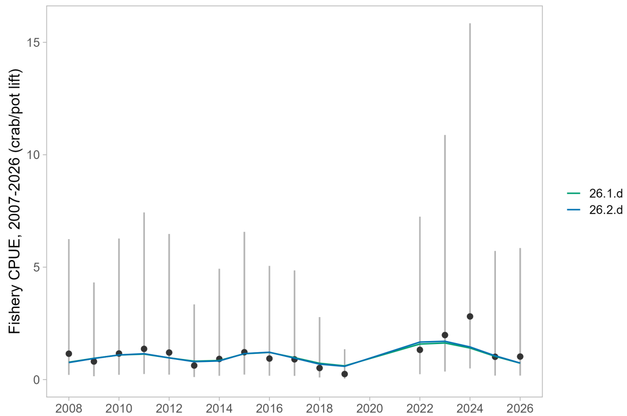
Figure 27: Model fits to the summer commercial fishery standardized catch per unit effort (CPUE) index (2007-2026) for the models including the model-based index of abundance that accounted for depth.
