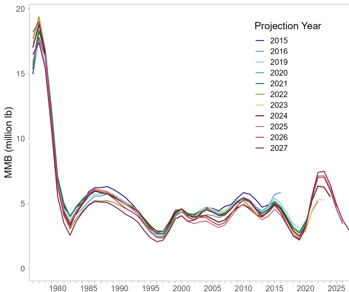
Figure 11: Comparison of historical estimates of mature male biomass of Norton Sound red king crab using the model selected in each year. Data were compiled from reported MMB values for the chosen model in the published SAFE document from the assessment year. The legend shows the year for which model projections were made.
