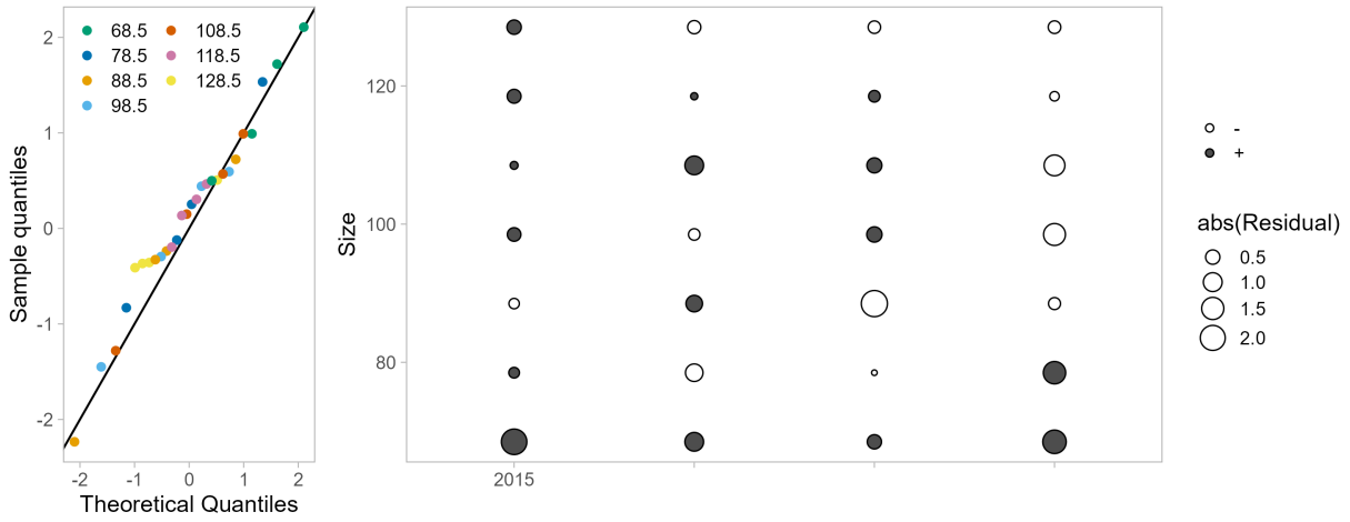
Figure 72: One-Step-Ahead residuals for model 26.2.d fits to size composition data from the winter commercial fishery retained catch.
