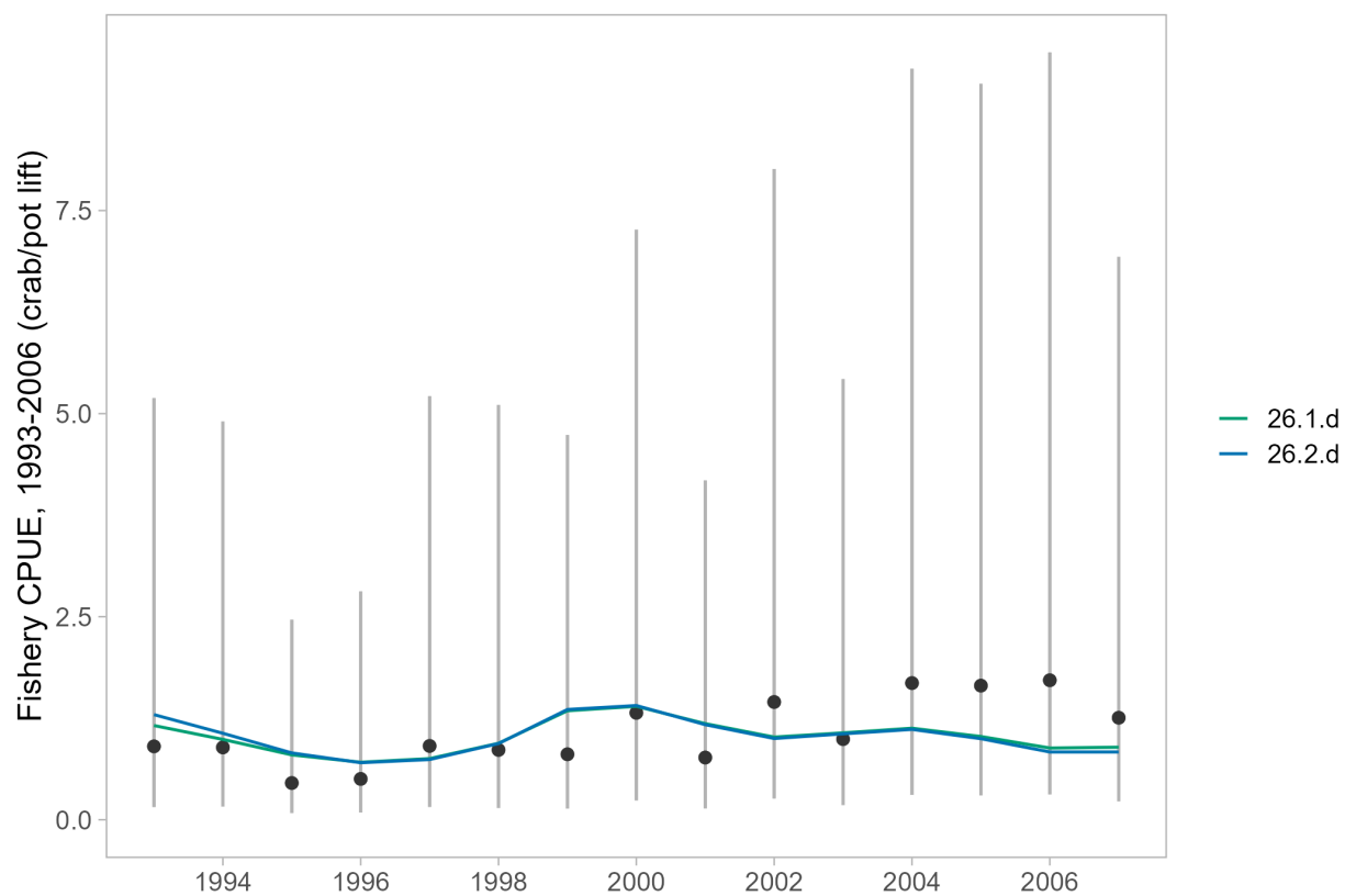
Figure 26: Model fits to the summer commercial fishery standardized catch per unit effort (CPUE) index (1993-2006) for the models including the model-based index of abundance that accounted for depth.
