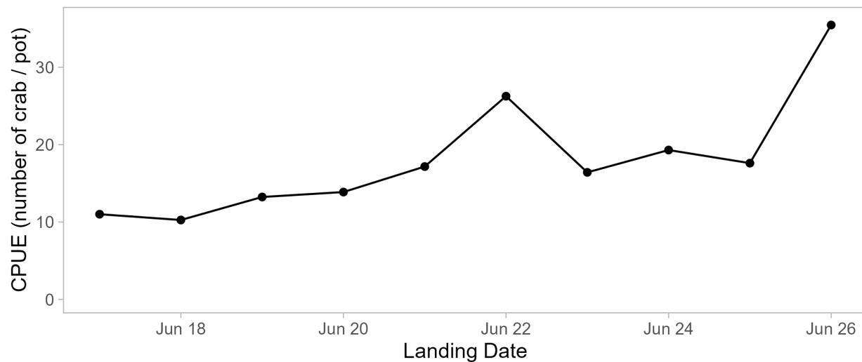
Figure 2: Norton Sound red king crab summer commercial fishery daily average catch per unit effort (CPUE) during the 2026 fishery.
