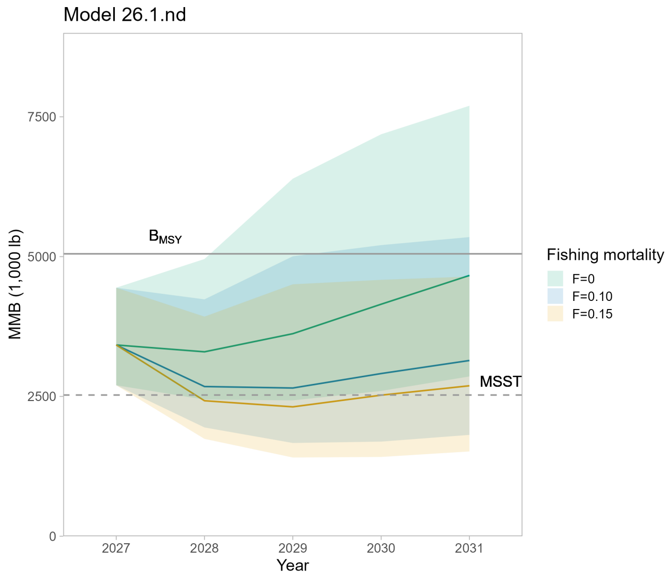
Figure 91: Mature male biomass (MMB) projections from the model using a model-based index of abundance that does not take into account depth (26.1.nd) for the next five years. Solid colored lines represent mean projected MMB for each fishing mortality rate while shaded regions represent 0.05 to 0.95 quantiles. The solid horizontal line shows B_{MSY} , which is equal to time series mean MMB for this Tier 4 stock, while the dashed horizontal line shows MSST (the minimum stock size threshold, 0.5 * B_{MSY} ).
