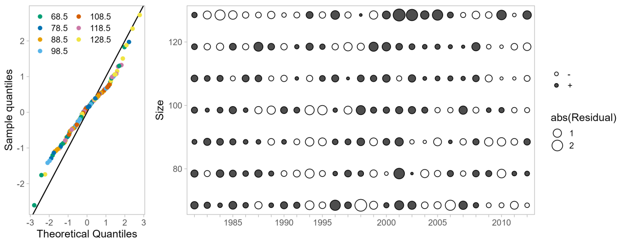
Figure 79: One-Step-Ahead residuals for model 26.2.d fits to size composition data from the Alaska Department of Fish and Game (ADFG) winter pot survey.
