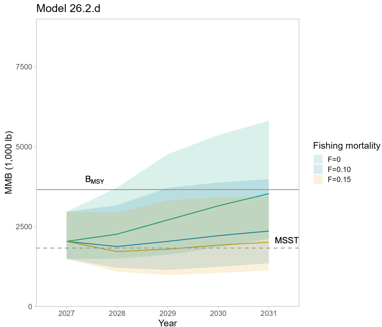
Figure 94: Mature male biomass (MMB) projections from the model using a model-based index of abundance that takes into account depth (26.2.d) for the next five years. Solid colored lines represent mean projected MMB for each fishing mortality rate while shaded regions represent 0.05 to 0.95 quantiles. The solid horizontal line shows B_{MSY} , which is equal to time series mean MMB for this Tier 4 stock, while the dashed horizontal line shows MSST (the minimum stock size threshold, 0.5 * B_{MSY} ).
