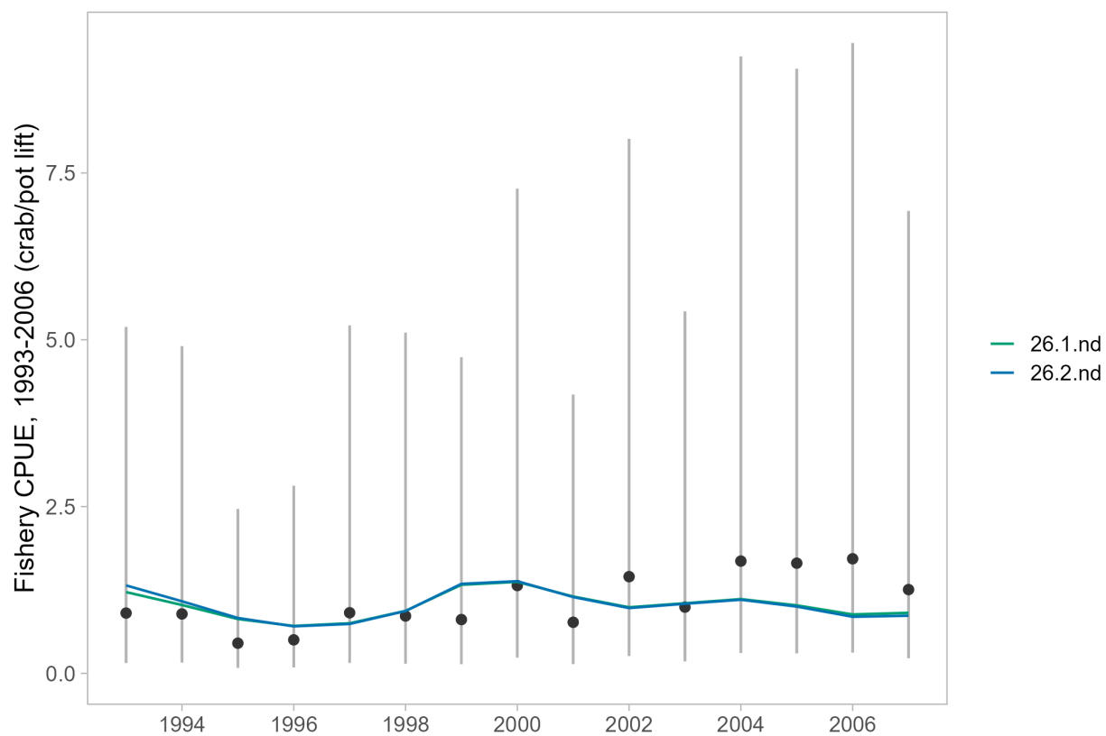
Figure 23: Model fits to the summer commercial fishery standardized catch per unit effort (CPUE) index (1993-2006) for the models including the model-based index of abundance that did not account for depth.
