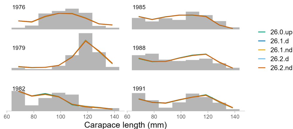
Figure 36: Annual observed and model-estimated size frequencies of all male red king crab caught in the National Oceanic and Atmospheric Administration (NOAA) Norton Sound trawl survey for the updated base model (26.0.up) and the models including a model-based index of abundance with depth excluded (nd) or included (d) and catchability for the model-based index fixed (26.1 models) or estimated (26.2 models).
