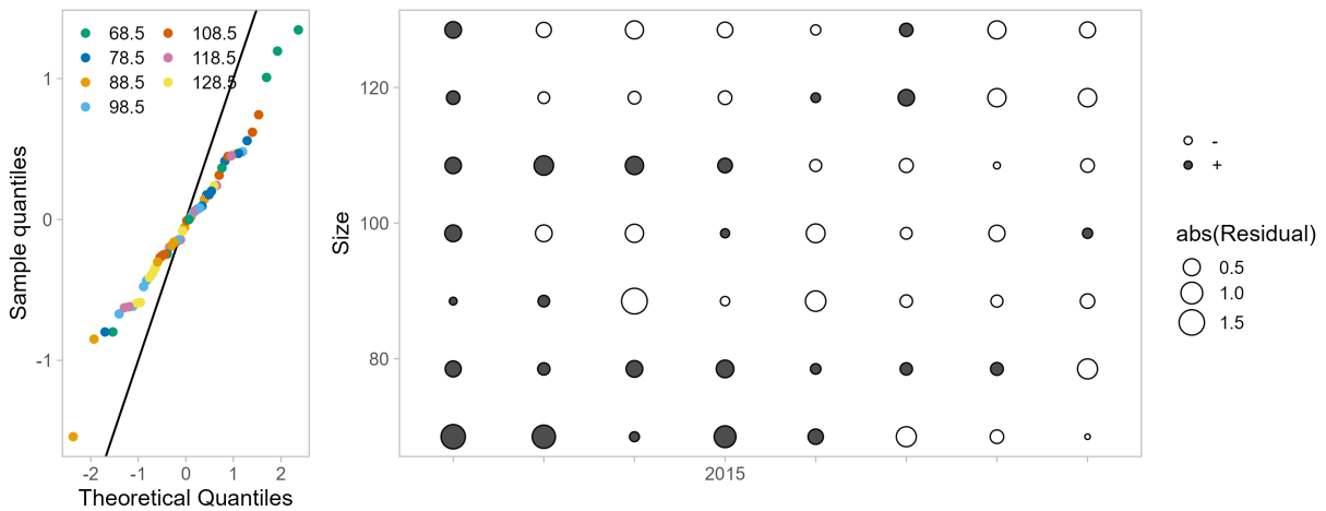
Figure 51: One-Step-Ahead residuals for model 26.1.nd fits to size composition data from the summer commercial fishery total catch.
