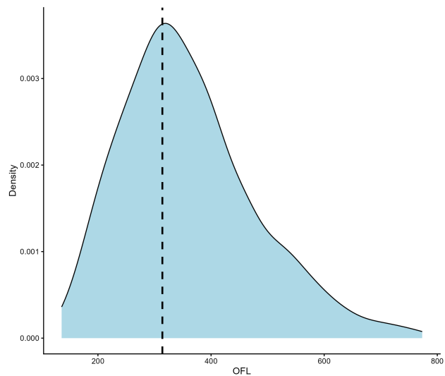
Figure 7: The probability density function of the OFL for model 26.0, based on 1,000 Markov chain Monte Carlo (MCMC) draws. The vertical dashed line represents the OFL from the original model run.
