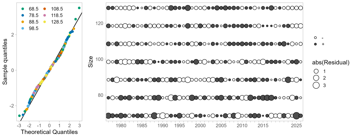
Figure 41: One-Step-Ahead residuals for model 26.0 fits to size composition data from the summer commercial fishery retained catch.
