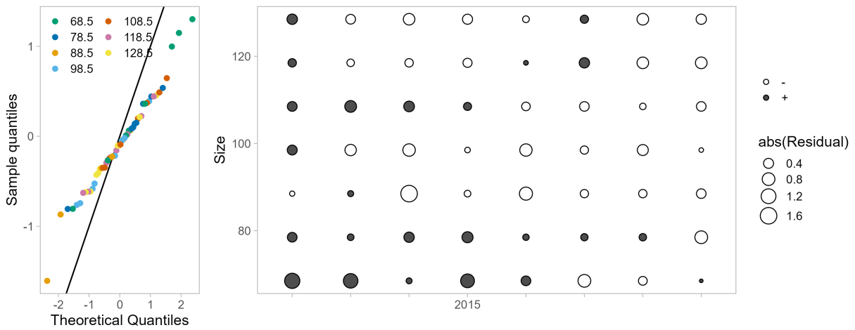
Figure 75: One-Step-Ahead residuals for model 26.2.d fits to size composition data from the summer commercial fishery total catch.
