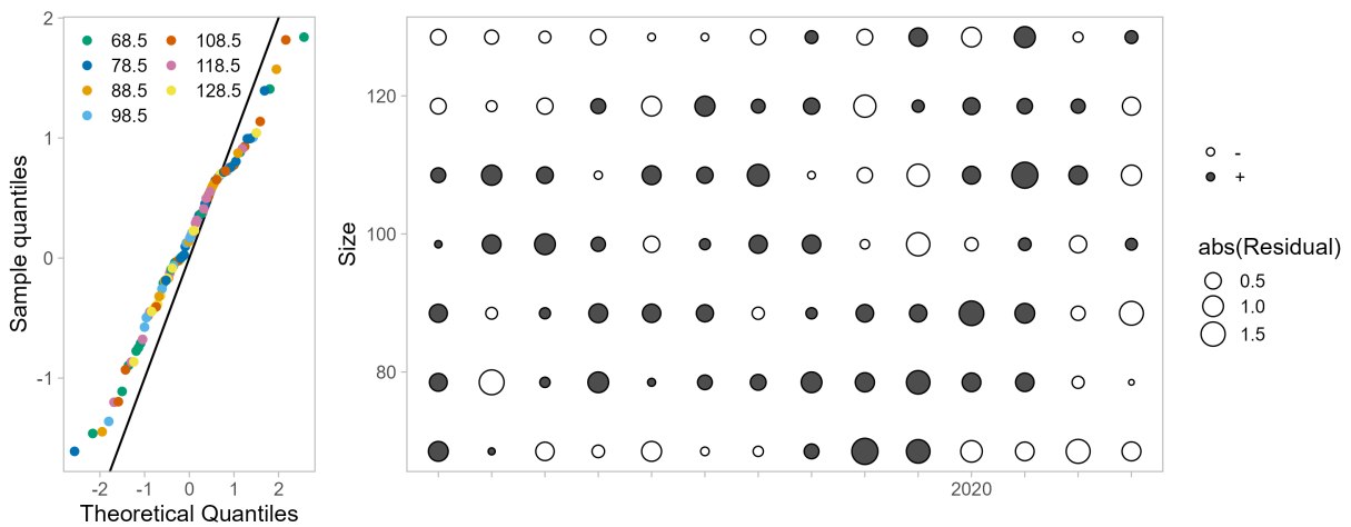
Figure 53: One-Step-Ahead residuals for model 26.1.nd fits to size composition data from the Alaska Department of Fish and Game (ADFG) trawl survey.
