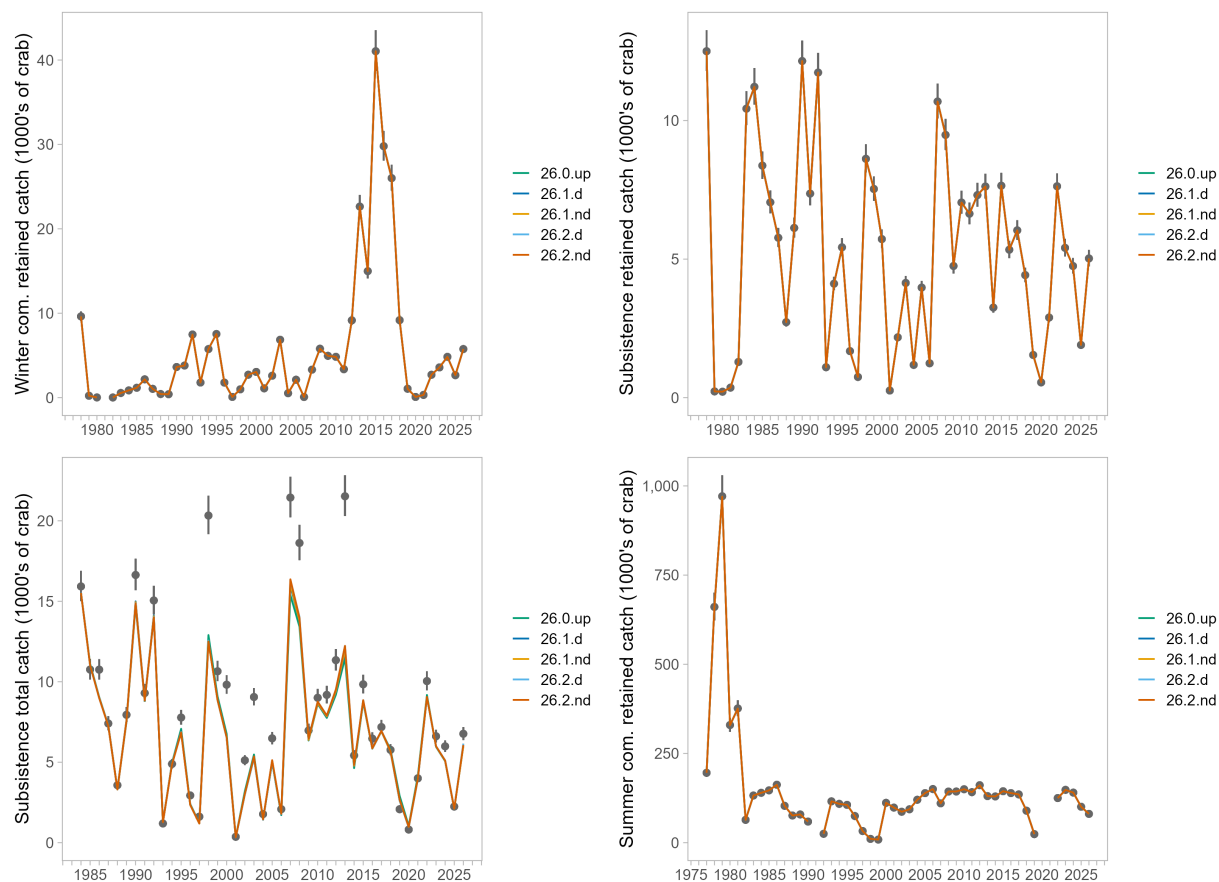
Figure 15: Observed and model-estimated catch of male red king crab caught in the winter commercial, summer commercial, and subsistence fisheries for the updated base model (26.0.up) and the models including the model-based index of abundance. Note that subsistence total catch was not fitted in these models (emphasis set to 0).
