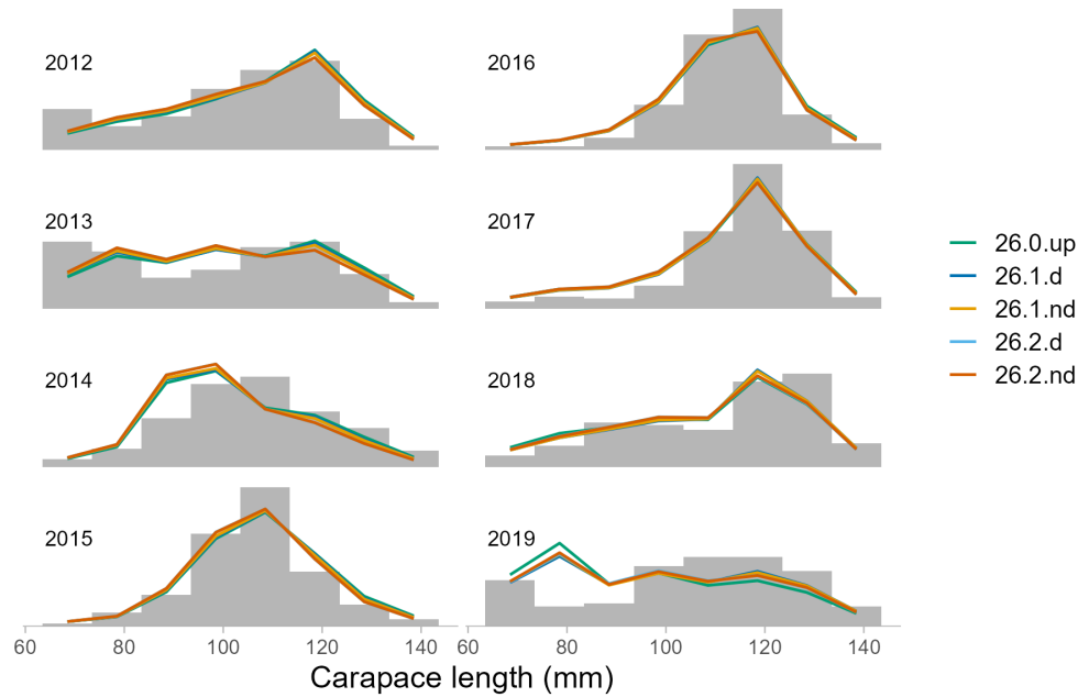
Figure 35: Annual observed and model-estimated size frequencies of all male red king crab caught in the directed summer commercial fishery for the updated base model (26.0.up) and the models including a model-based index of abundance with depth excluded (nd) or included (d) and catchability for the model-based index fixed (26.1 models) or estimated (26.2 models).
