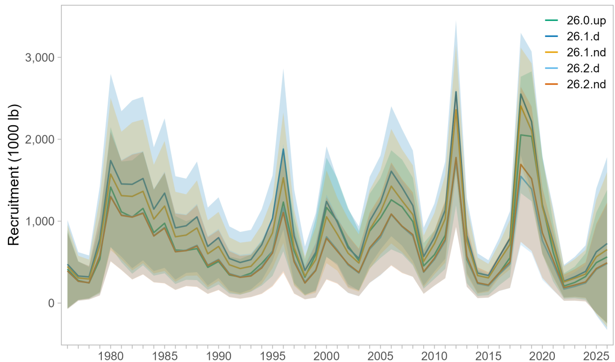
Figure 80: Estimated recruitment (1000 lb) over 1976-2025 for the updated base model (26.0.up) and the models including a model-based index of abundance with depth excluded (nd) or included (d) and catchability for the model-based index fixed (26.1 models) or estimated (26.2 models).
