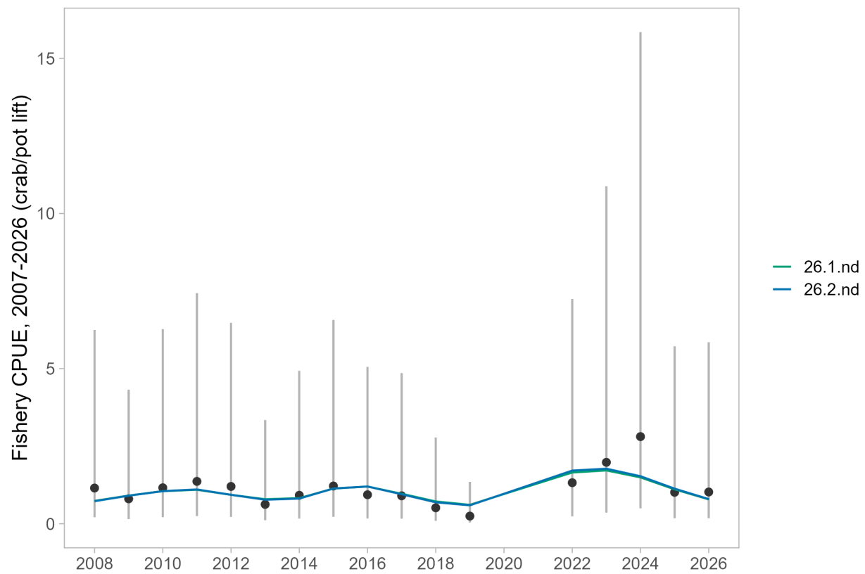
Figure 24: Model fits to the summer commercial fishery standardized catch per unit effort (CPUE) index (2007-2026) for the models including the model-based index of abundance that did not account for depth.
