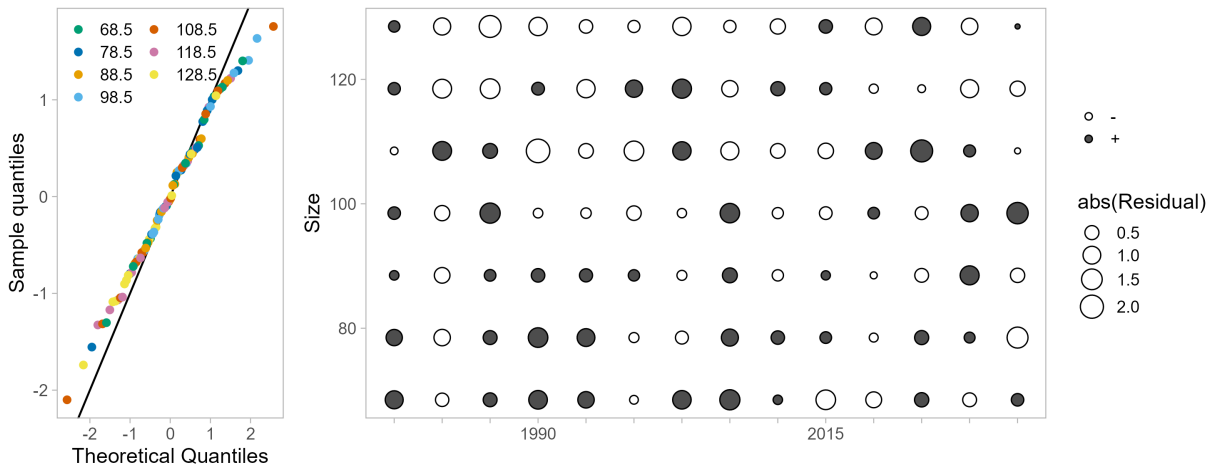
Figure 42: One-Step-Ahead residuals for model 26.0 fits to size composition data from the summer commercial fishery discarded catch.
