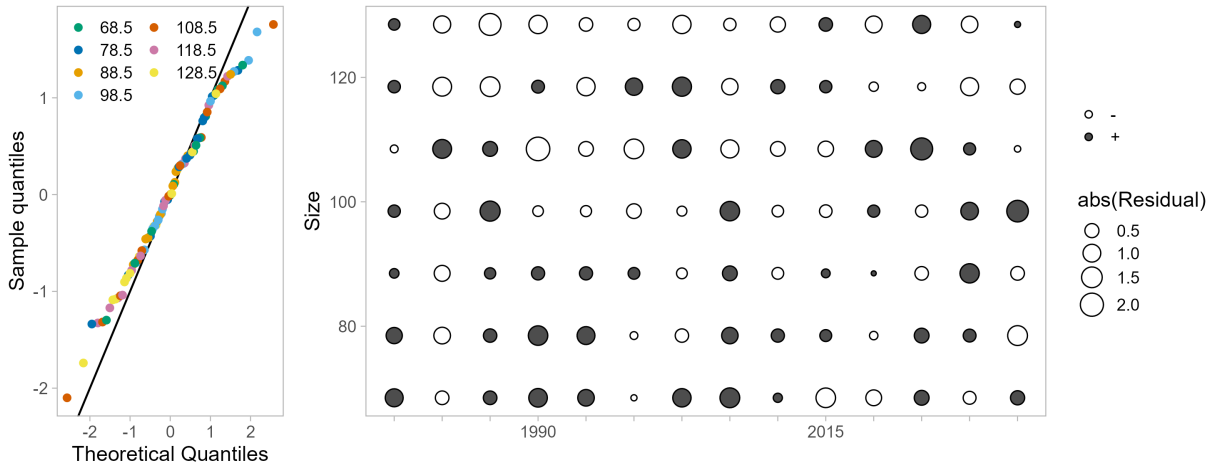
Figure 74: One-Step-Ahead residuals for model 26.2.d fits to size composition data from the summer commercial fishery discarded catch.
