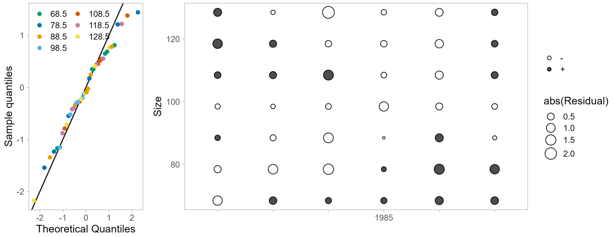
Figure 44: One-Step-Ahead residuals for model 26.0 fits to size composition data from the National Oceanic and Atmospheric Administration (NOAA) Norton Sound trawl survey.
