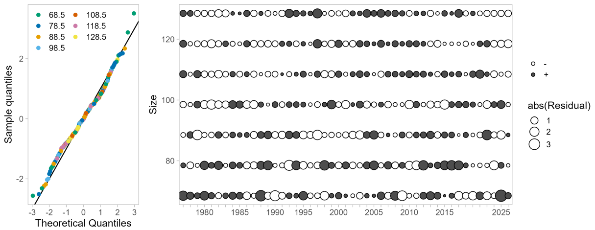
Figure 49: One-Step-Ahead residuals for model 26.1.nd fits to size composition data from the summer commercial fishery retained catch.
