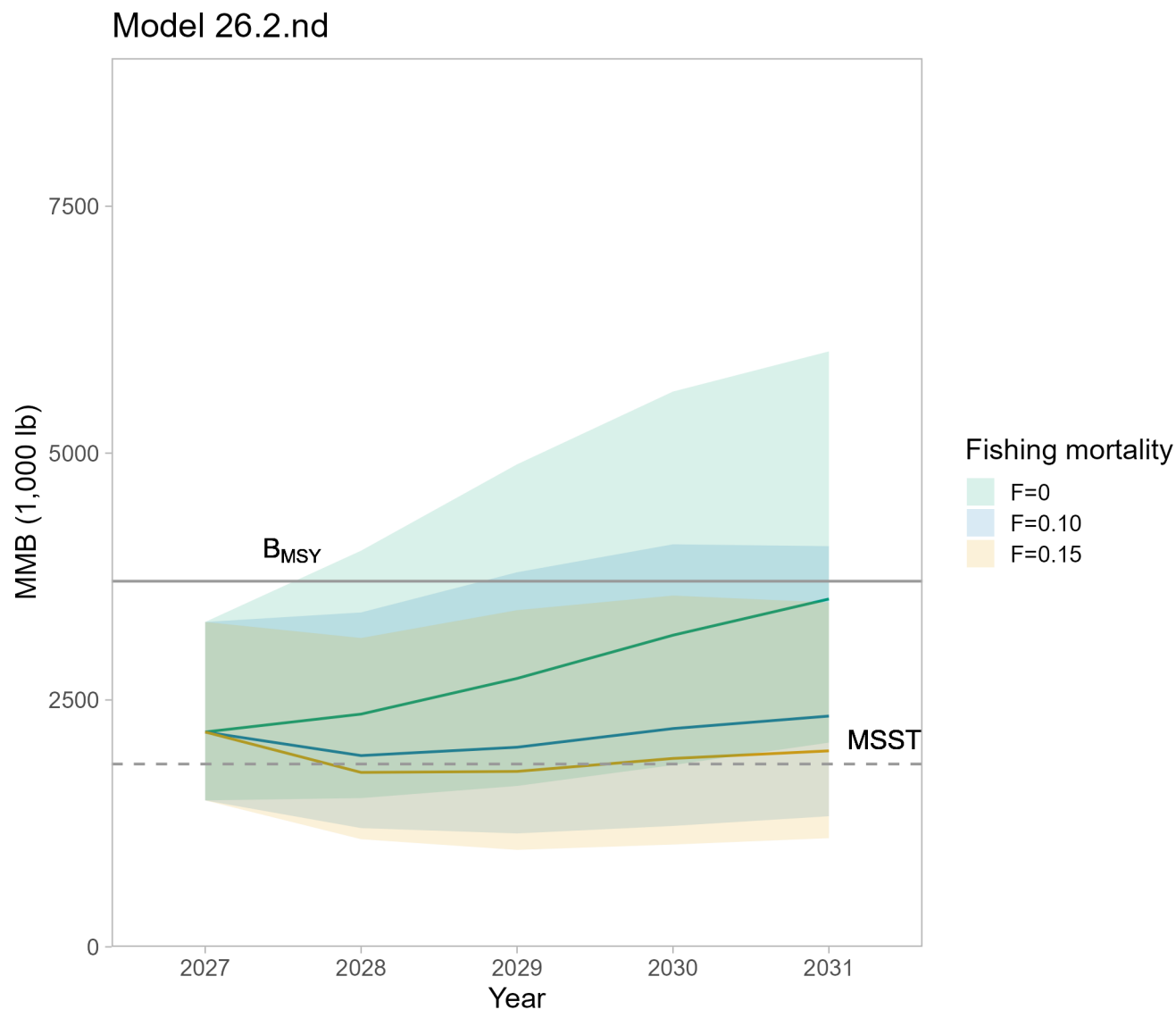
Figure 93: Mature male biomass (MMB) projections from the model using a model-based index of abundance that does not take into account depth (26.2.nd) for the next five years. Solid colored lines represent mean projected MMB for each fishing mortality rate while shaded regions represent 0.05 to 0.95 quantiles. The solid horizontal line shows B_{MSY} , which is equal to time series mean MMB for this Tier 4 stock, while the dashed horizontal line shows MSST (the minimum stock size threshold, 0.5 * B_{MSY} ).
