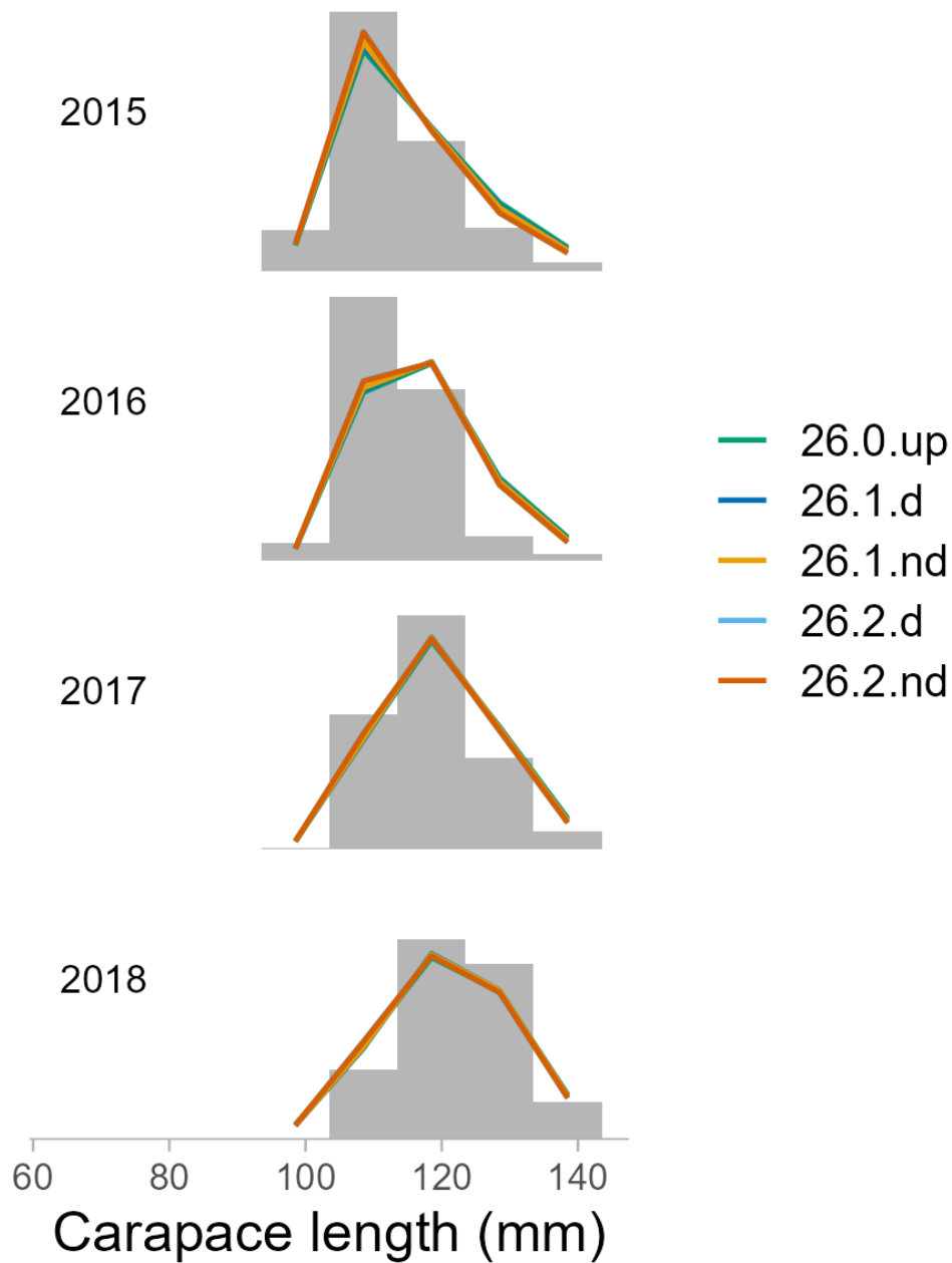
Figure 32: Annual observed and model-estimated size frequencies of male red king crab retained in the directed winter commercial fishery for the updated base model (26.0.up) and the models including a model-based index of abundance with depth excluded (nd) or included (d) and catchability for the model-based index fixed (26.1 models) or estimated (26.2 models).
