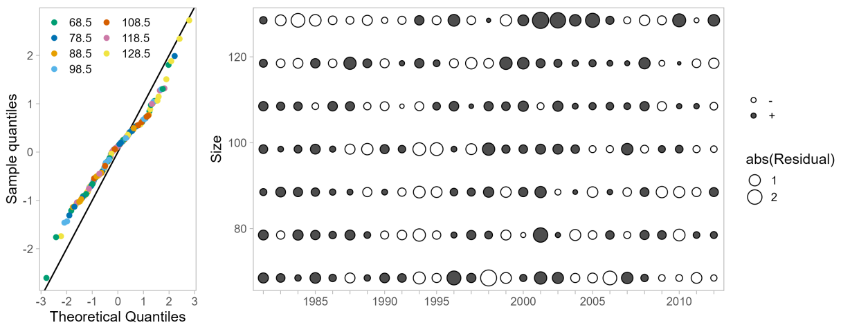
Figure 63: One-Step-Ahead residuals for model 26.1.d fits to size composition data from the Alaska Department of Fish and Game (ADFG) winter pot survey.
