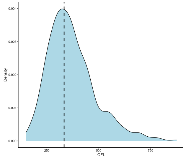
Figure 8: The probability density function of the OFL for model 26.1.nd, based on 1,000 Markov chain Monte Carlo (MCMC) draws. The vertical dashed line represents the OFL from the original model run.
