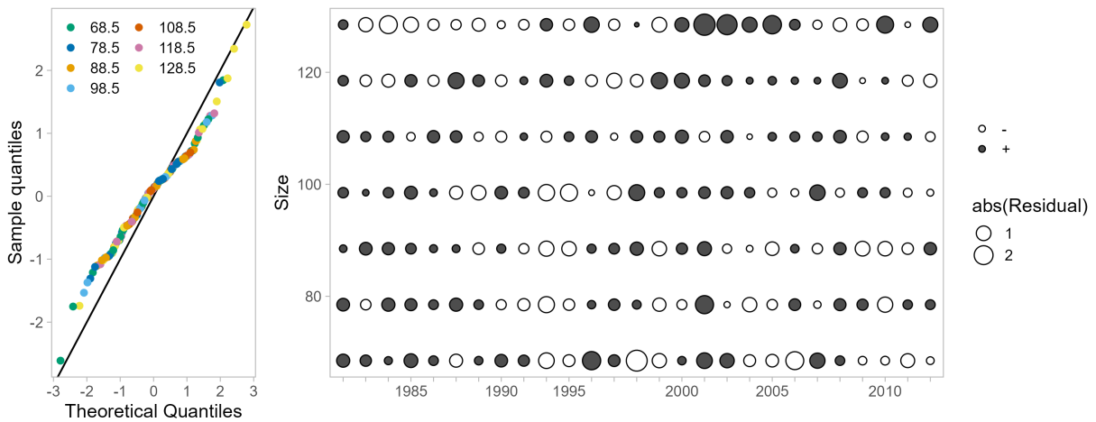
Figure 47: One-Step-Ahead residuals for model 26.0 fits to size composition data from the Alaska Department of Fish and Game (ADFG) winter pot survey.
