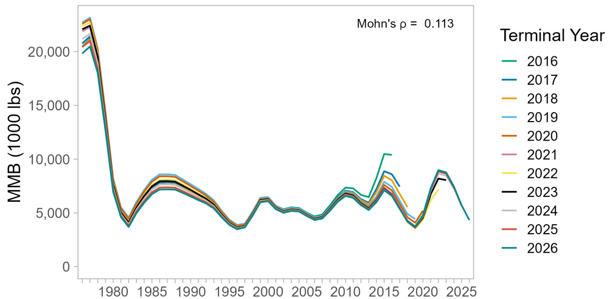
Figure 87: Retrospective patterns in estimated mature male biomass (MMB) for the model using a model-based index of abundance that takes into account depth (26.1.d).
