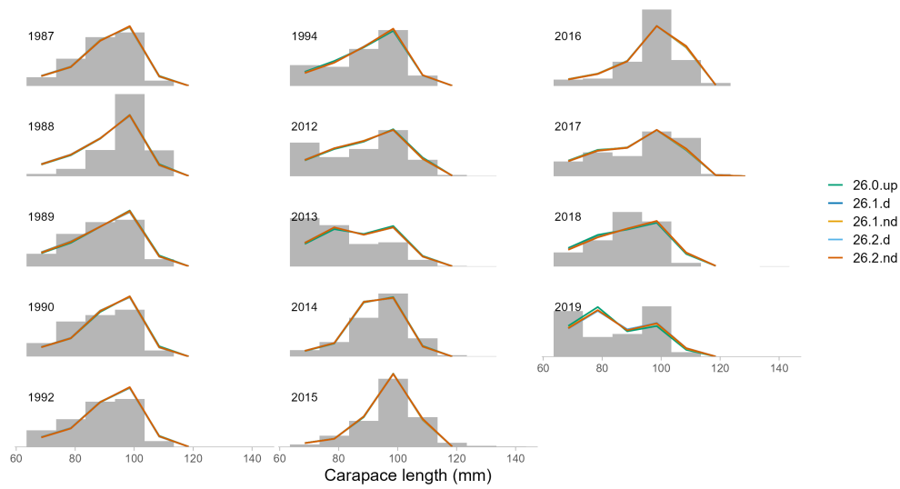
Figure 34: Annual observed and model-estimated size frequencies of male red king crab discarded in the directed summer commercial fishery for the updated base model (26.0.up) and the models including a model-based index of abundance with depth excluded (nd) or included (d) and catchability for the model-based index fixed (26.1 models) or estimated (26.2 models).
