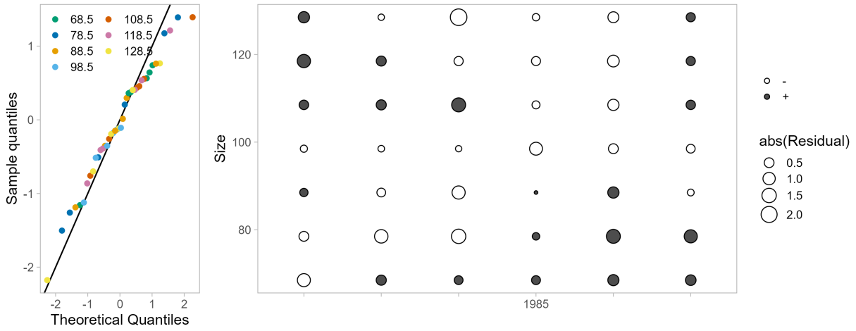
Figure 52: One-Step-Ahead residuals for model 26.1.nd fits to size composition data from the National Oceanic and Atmospheric Administration (NOAA) Norton Sound trawl survey.
