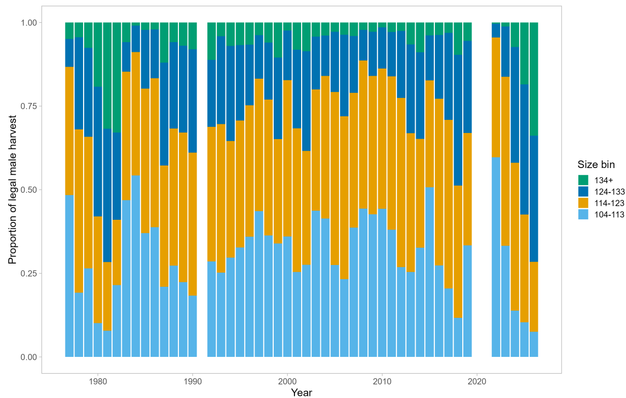
Figure 4: Proportion of Norton Sound red king crab summer commercial fishery legal male retained catch in each size bin over 1977-2026. Size bins are defined in male carapace length (mm).
