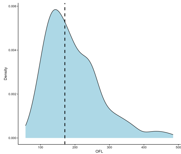
Figure 10: The probability density function of the OFL for model 26.2.d, based on 1,000 Markov chain Monte Carlo (MCMC) draws. The vertical dashed line represents the OFL from the original model run.
