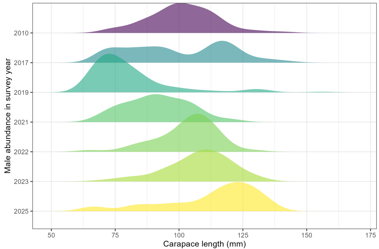
Figure 6: National Oceanic and Atmospheric Administration Northern Bering Sea trawl survey abundances by carapace length for male Norton Sound red king crab from 2010 to 2025.
