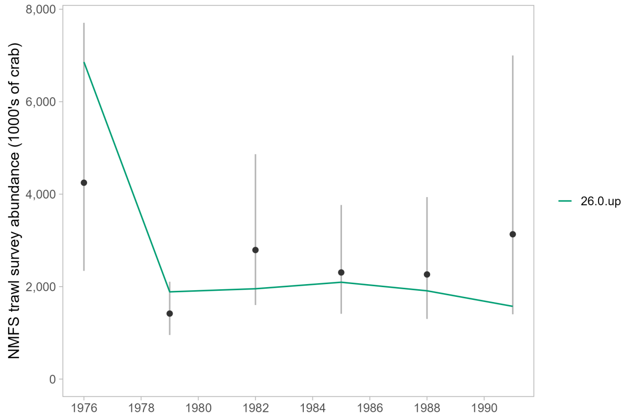
Figure 16: Model fits to the design-based index of abundance from the historical National Oceanic and Atmospheric Administration (NOAA) Norton Sound trawl survey for the updated base model. Note that this design-based index of abundance for the historical survey was used in all models in this document, while the design-based indices of abundance for the ADFG and NBS trawl surveys were only included in the base model.
