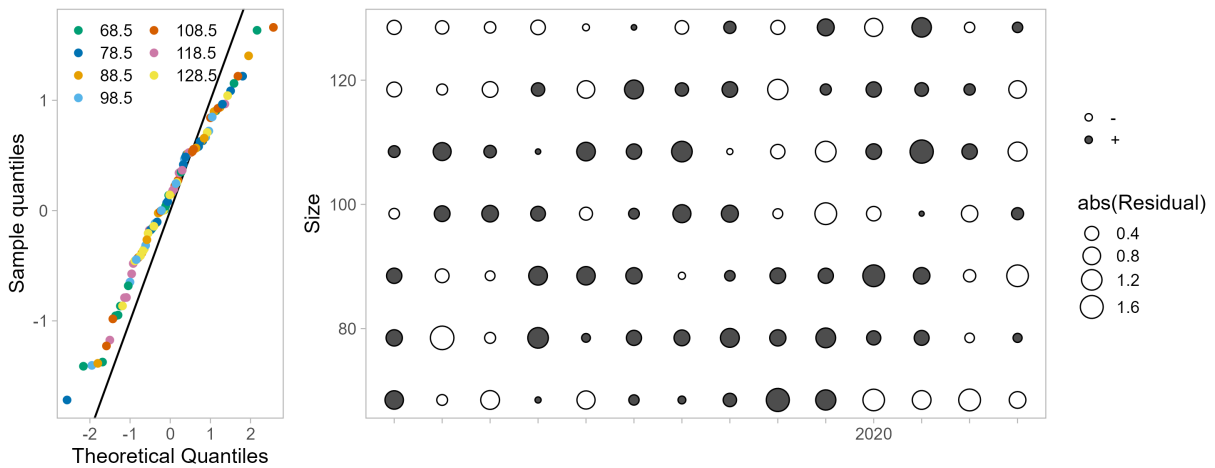
Figure 45: One-Step-Ahead residuals for model 26.0 fits to size composition data from the Alaska Department of Fish and Game (ADFG) trawl survey.
