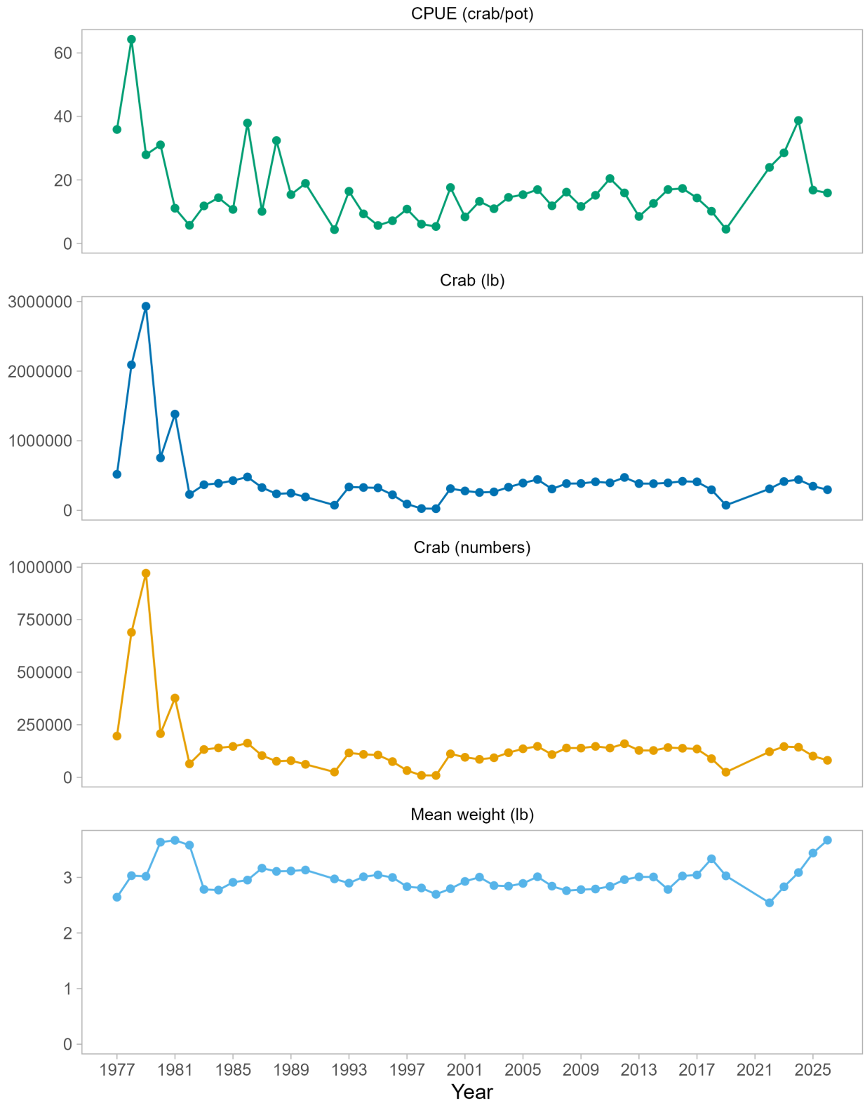
Figure 1: Norton Sound red king crab summer commercial fishery catch per unit effort (CPUE), retained catch in lb, retained catch in number of crab, and mean weight in lb during 1977-2026.
