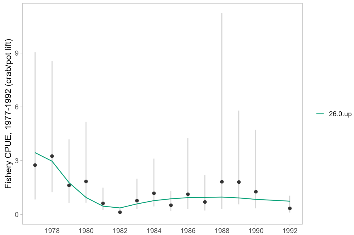
Figure 19: Model fits to the summer commercial fishery standardized catch per unit effort (CPUE) index (1977-1992) for the updated base model.
