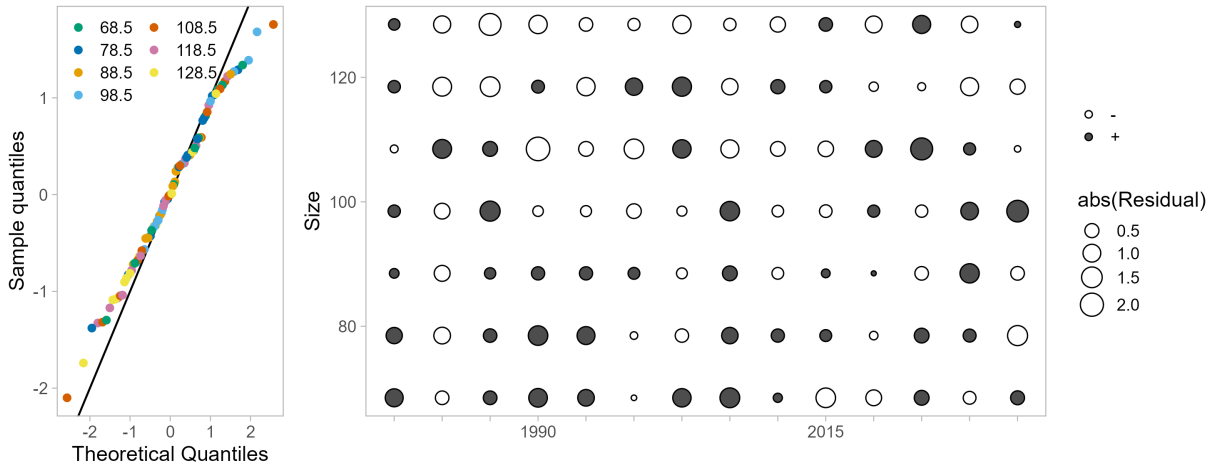
Figure 66: One-Step-Ahead residuals for model 26.2.nd fits to size composition data from the summer commercial fishery discarded catch.
