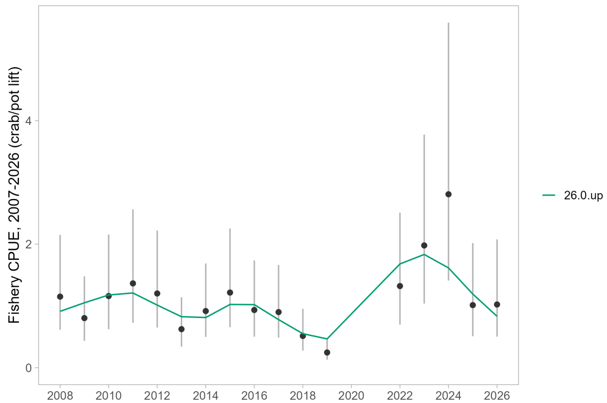
Figure 21: Model fits to the summer commercial fishery standardized catch per unit effort (CPUE) index (2007-2026) for the updated base model.
