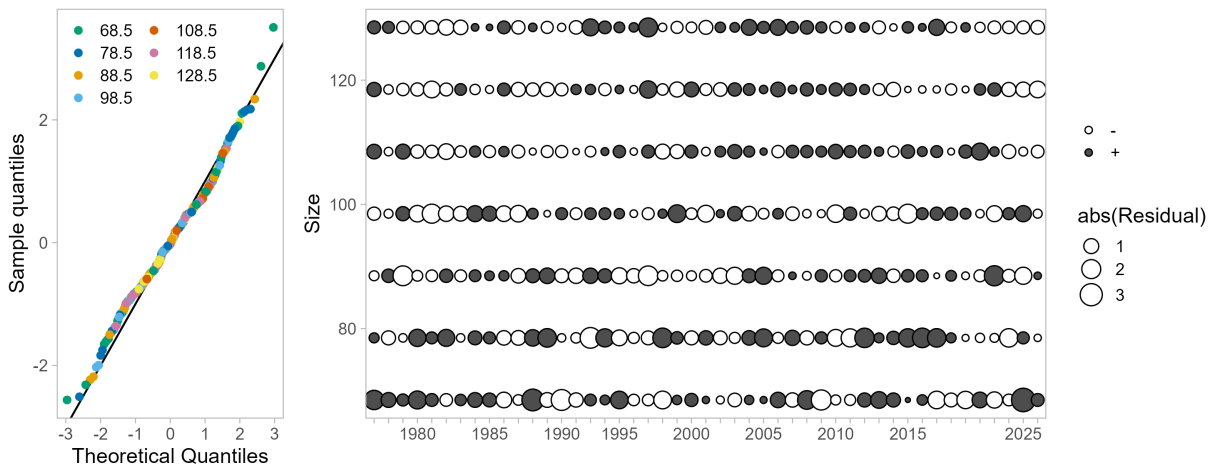
Figure 57: One-Step-Ahead residuals for model 26.1.d fits to size composition data from the summer commercial fishery retained catch.
