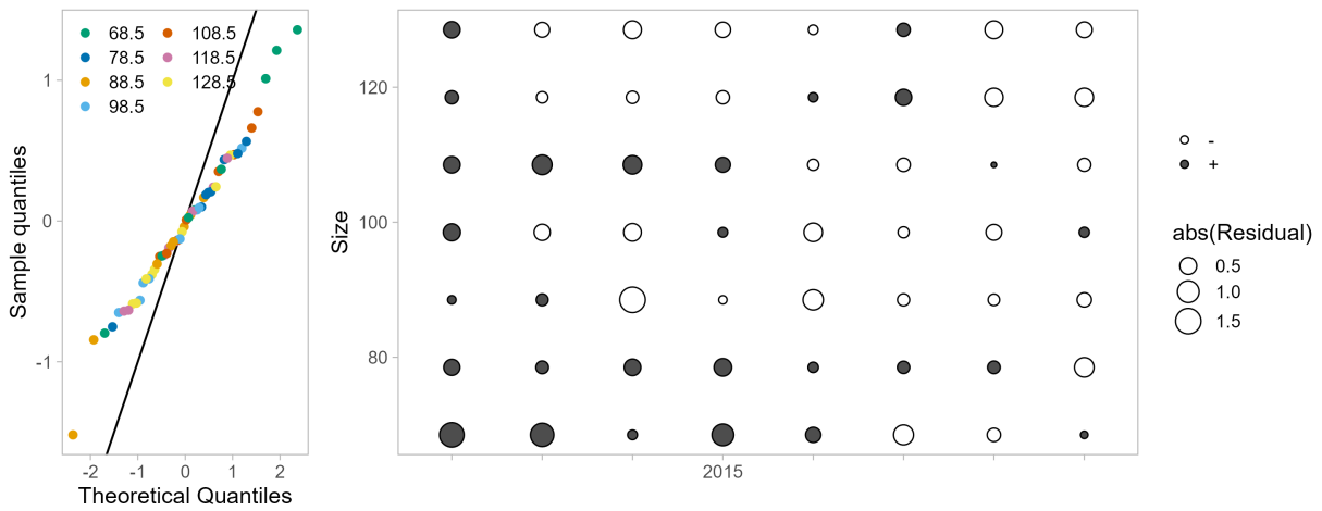
Figure 59: One-Step-Ahead residuals for model 26.1.d fits to size composition data from the summer commercial fishery total catch.
