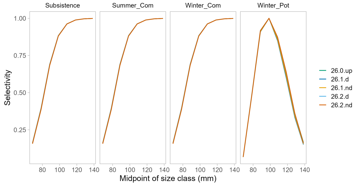
Figure 82: Comparisons of estimated capture selectivities in the summer commercial, winter commercial, and winter subsistence fisheries, as well as the winter pot survey, for the updated base model (26.0) and the models including a model-based index of abundance.
