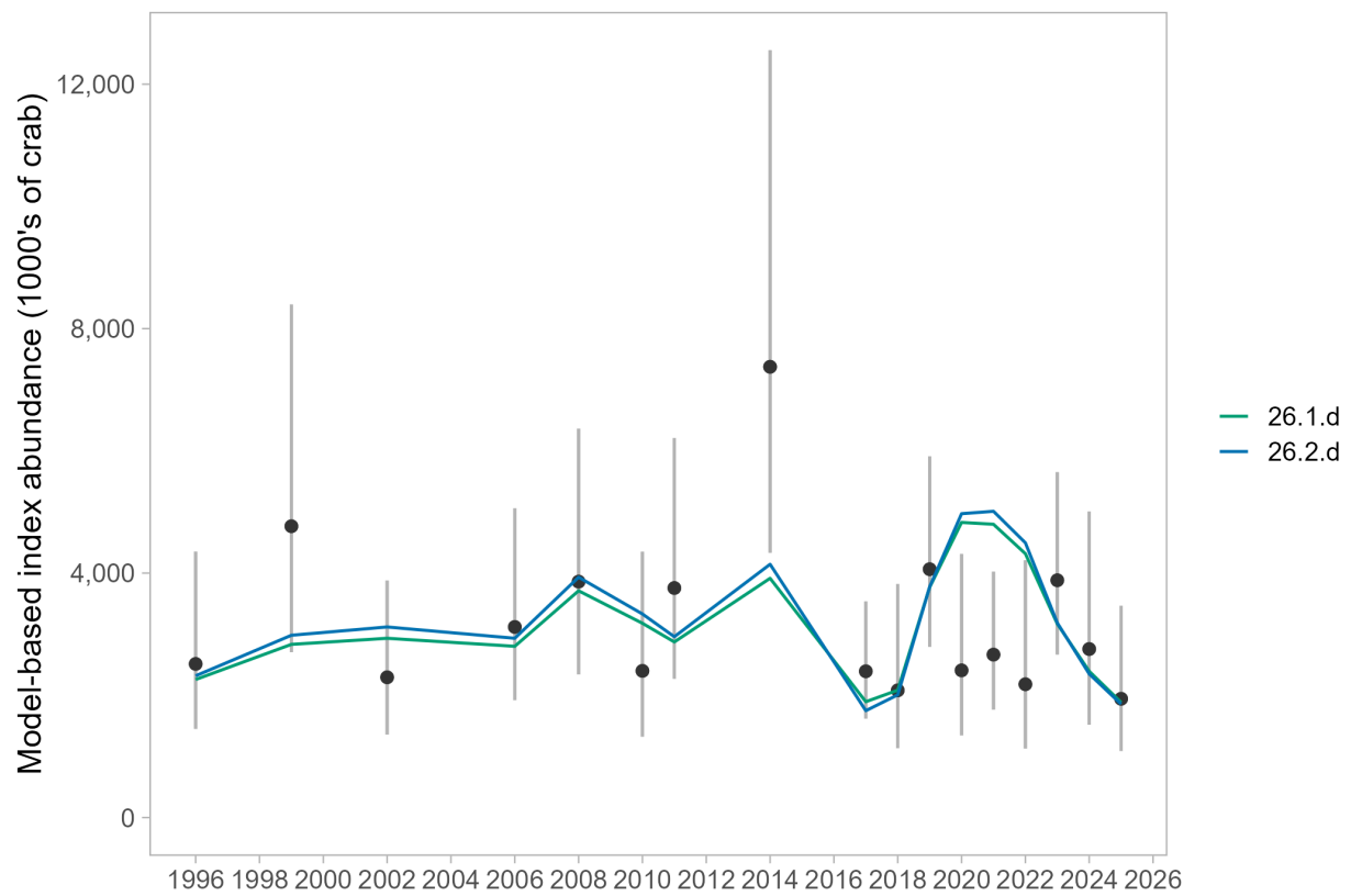
Figure 31: Model fits to the model-based index of abundance that accounted for depth for the models that included this index.
