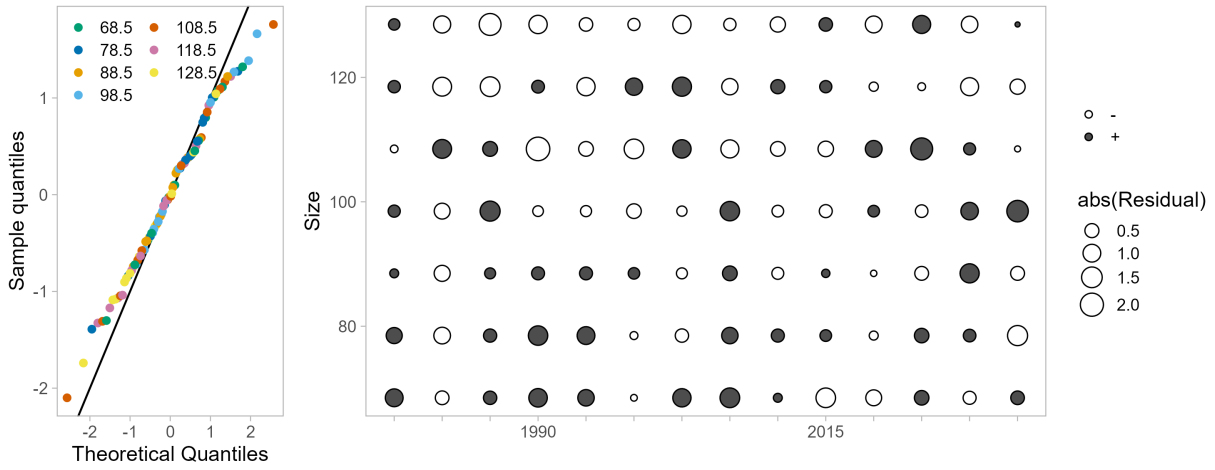
Figure 50: One-Step-Ahead residuals for model 26.1.nd fits to size composition data from the summer commercial fishery discarded catch.
