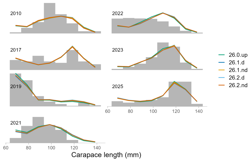
Figure 38: Annual observed and model-estimated size frequencies of all male red king crab caught in the National Oceanic and Atmospheric Administration (NOAA) Northern Bering Sea (NBS) trawl survey for the updated base model (26.0.up) and the models including a model-based index of abundance with depth excluded (nd) or included (d) and catchability for the model-based index fixed (26.1 models) or estimated (26.2 models).
