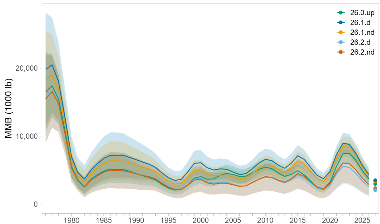
Figure 81: Comparisons of estimated mature male biomass (MMB) time series over 1976-2026 for the updated base model (26.0.up) and the models including a model-based index of abundance with depth excluded (nd) or included (d) and catchability for the model-based index fixed (26.1 models) or estimated (26.2 models). Points represent projected values for 2027.
