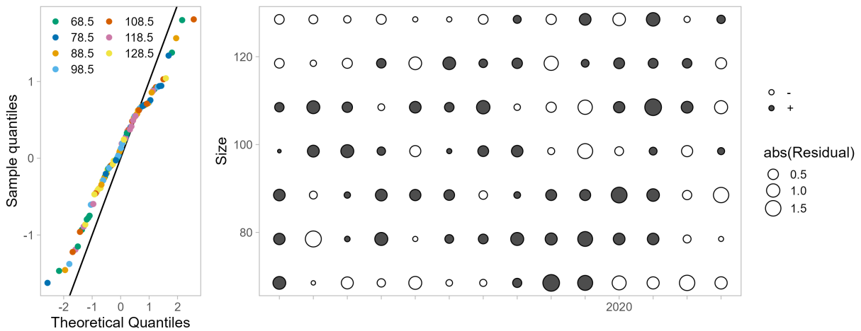
Figure 69: One-Step-Ahead residuals for model 26.2.nd fits to size composition data from the Alaska Department of Fish and Game (ADFG) trawl survey.
