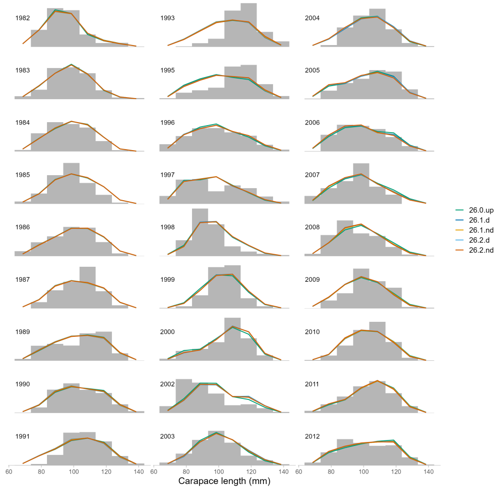
Figure 39: Annual observed and model-estimated size frequencies of all male red king crab caught in the Alaska Department of Fish and Game (ADFG) winter pot survey for the updated base model (26.0.up) and the models including a model-based index of abundance with depth excluded (nd) or included (d) and catchability for the model-based index fixed (26.1 models) or estimated (26.2 models).
