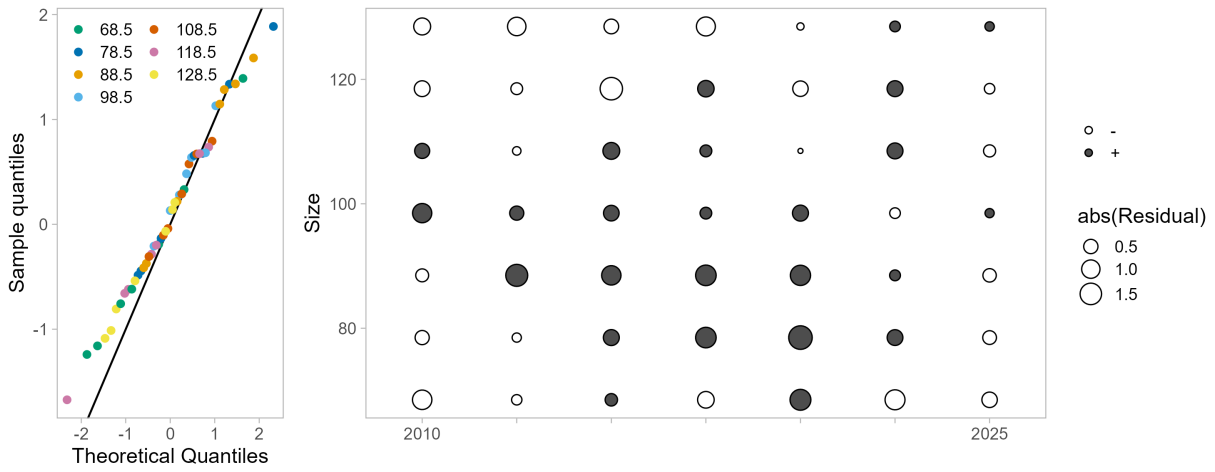
Figure 78: One-Step-Ahead residuals for model 26.2.d fits to size composition data from the National Oceanic and Atmospheric Administration (NOAA) Northern Bering Sea (NBS) trawl survey.
