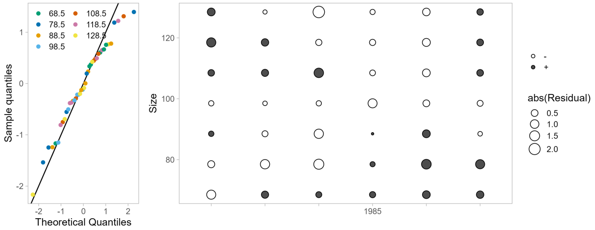
Figure 68: One-Step-Ahead residuals for model 26.2.nd fits to size composition data from the National Oceanic and Atmospheric Administration (NOAA) Norton Sound trawl survey.
