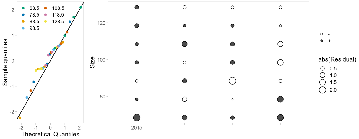
Figure 56: One-Step-Ahead residuals for model 26.1.d fits to size composition data from the winter commercial fishery retained catch.
