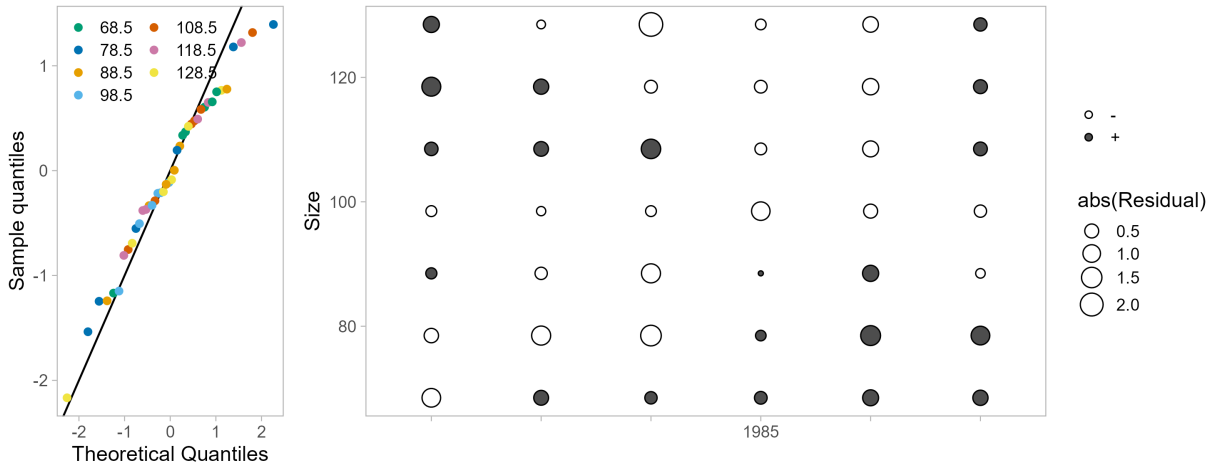
Figure 76: One-Step-Ahead residuals for model 26.2.d fits to size composition data from the National Oceanic and Atmospheric Administration (NOAA) Norton Sound trawl survey.
