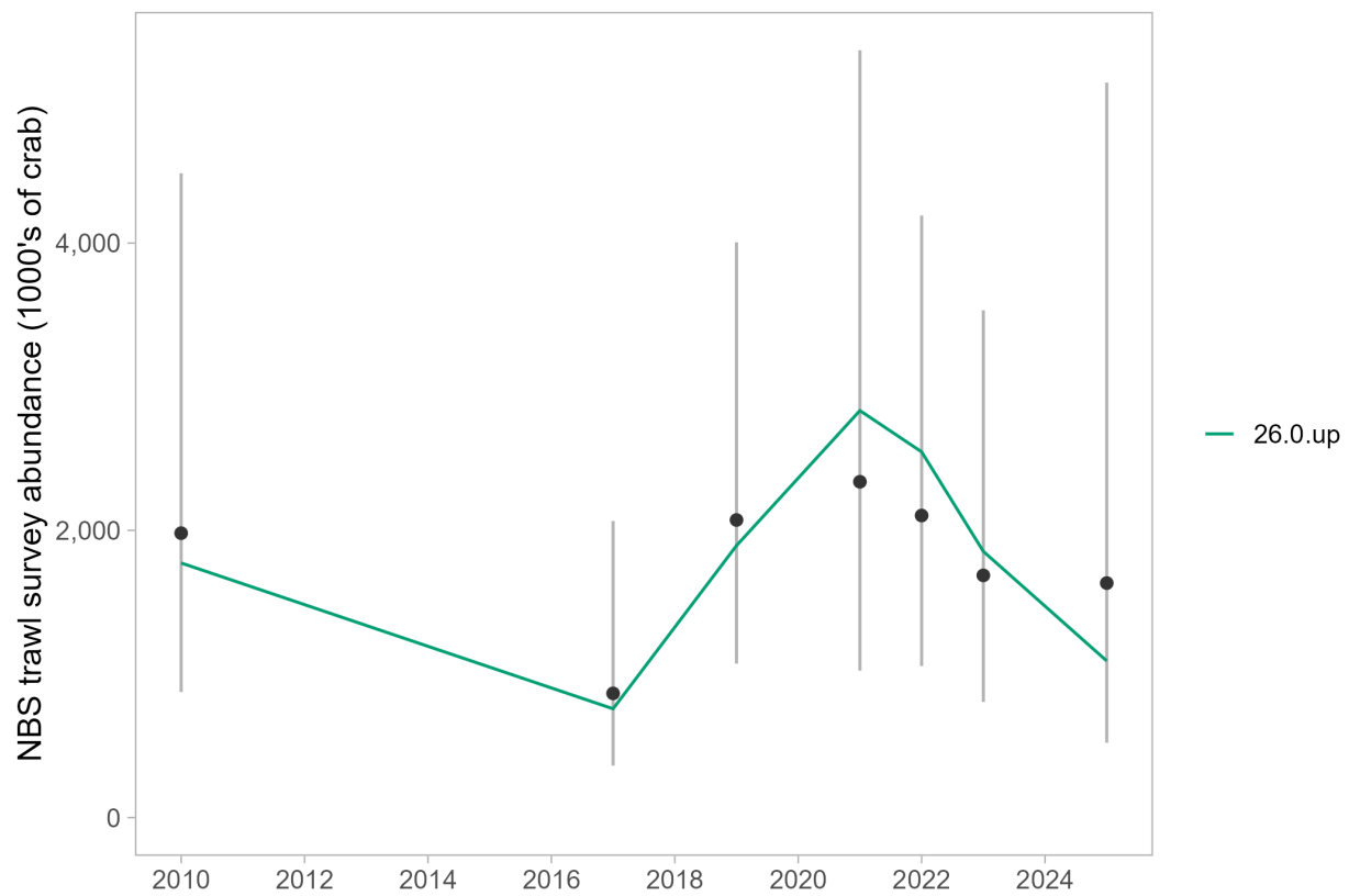
Figure 29: Model fits to the design-based index of abundance from the National Oceanic and Atmospheric Administration (NOAA) Northern Bering Sea (NBS) trawl survey for the base model.
