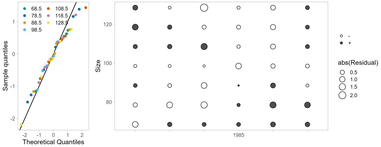
Figure 60: One-Step-Ahead residuals for model 26.1.d fits to size composition data from the National Oceanic and Atmospheric Administration (NOAA) Norton Sound trawl survey.
