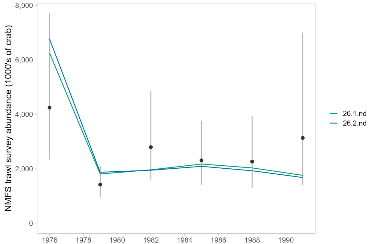
Figure 17: Model fits to the design-based index of abundance from the historical National Oceanic and Atmospheric Administration (NOAA) Norton Sound trawl survey for the models that included a model-based index of abundance that did not account for depth in place of the design-based indices for the ADFG and NBS trawl surveys. These models still included the design-based index of abundance from the historical survey shown here, as the data from the historical survey was not included in the model-based index.
