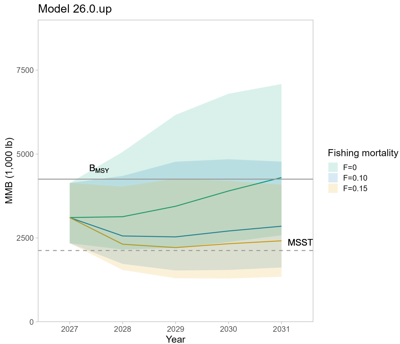
Figure 90: Mature male biomass (MMB) projections from the base model with updated data and GMACS version (26.0.up) for the next five years. Solid colored lines represent mean projected MMB for each fishing mortality rate while shaded regions represent 0.05 to 0.95 quantiles. The solid horizontal line shows B_{MSY} , which is equal to time series mean MMB for this Tier 4 stock, while the dashed horizontal line shows MSST (the minimum stock size threshold, 0.5 * B_{MSY} ).
