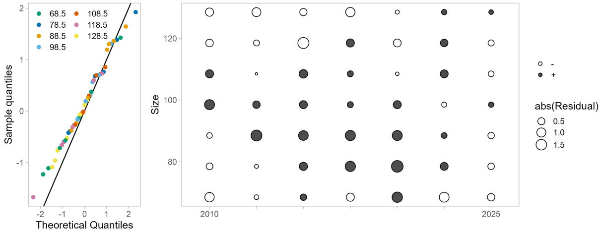
Figure 62: One-Step-Ahead residuals for model 26.1.d fits to size composition data from the National Oceanic and Atmospheric Administration (NOAA) Northern Bering Sea (NBS) trawl survey.
