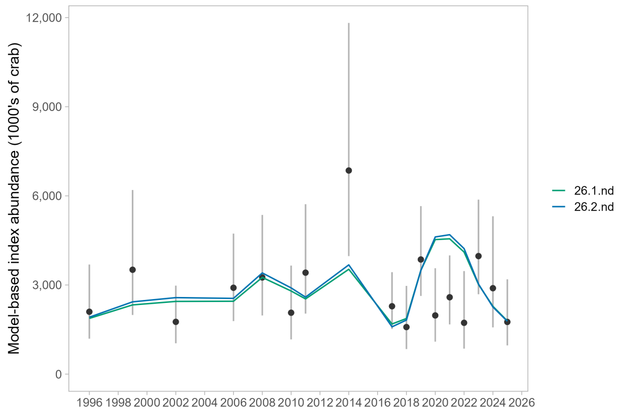
Figure 30: Model fits to the model-based index of abundance that did not account for depth for the models that included this index.
