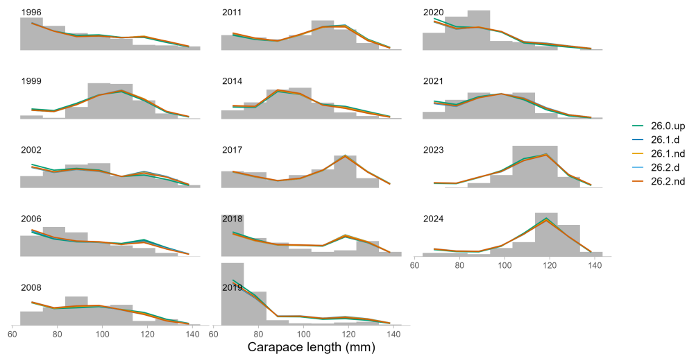
Figure 37: Annual observed and model-estimated size frequencies of all male red king crab caught in the Alaska Department of Fish and Game (ADFG) trawl survey for the updated base model (26.0.up) and the models including a model-based index of abundance with depth excluded (nd) or included (d) and catchability for the model-based index fixed (26.1 models) or estimated (26.2 models).
