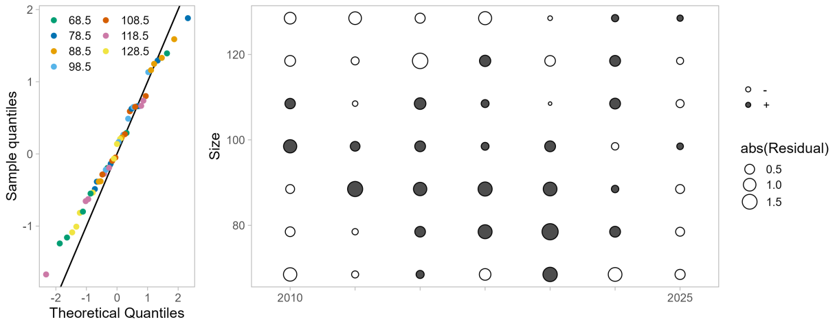
Figure 70: One-Step-Ahead residuals for model 26.2.nd fits to size composition data from the National Oceanic and Atmospheric Administration (NOAA) Northern Bering Sea (NBS) trawl survey.
