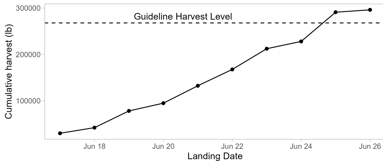
Figure 3: Norton Sound red king crab summer commercial fishery daily cumulative retained catch (lb) during the 2026 fishery.
