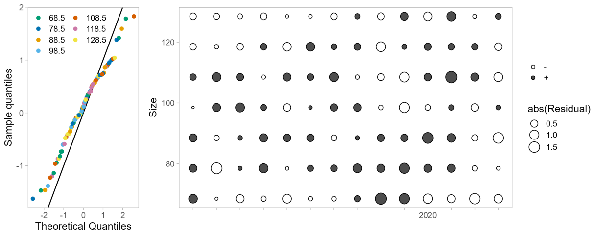
Figure 77: One-Step-Ahead residuals for model 26.2.d fits to size composition data from the Alaska Department of Fish and Game (ADFG) trawl survey.
