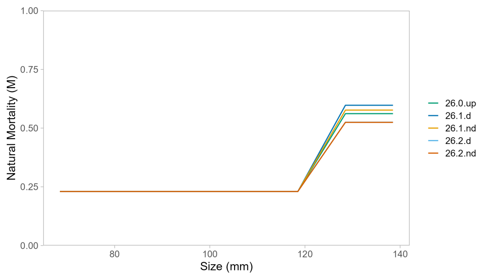
Figure 84: Natural mortality estimates for the updated base model (26.0.up) and the models including a model-based index of abundance (26.1.nd, 26.1.d, 26.2.nd, 26.2.d).
