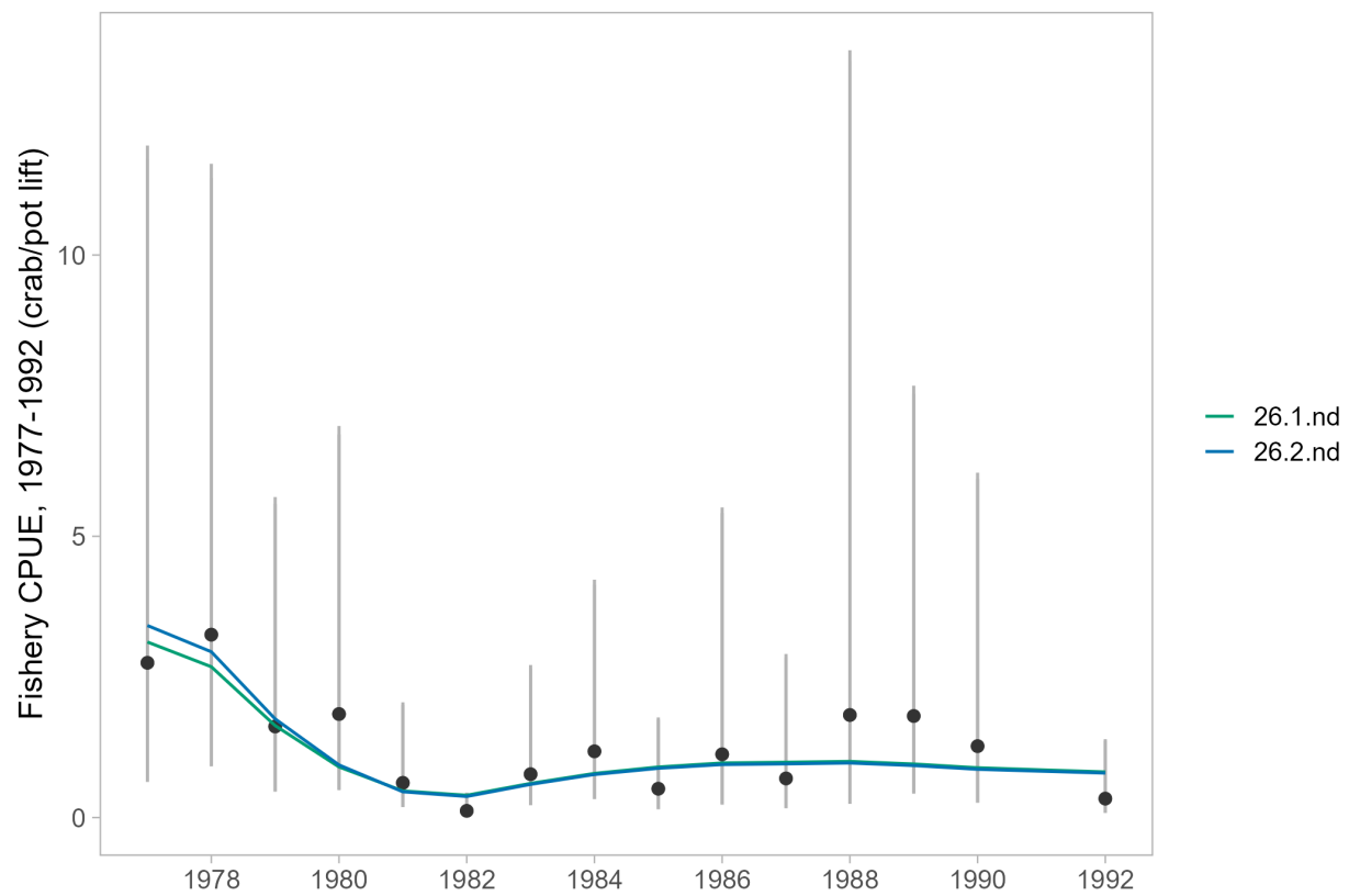
Figure 22: Model fits to the summer commercial fishery standardized catch per unit effort (CPUE) index (1977-1992) for the models including the model-based index of abundance that did not account for depth.
