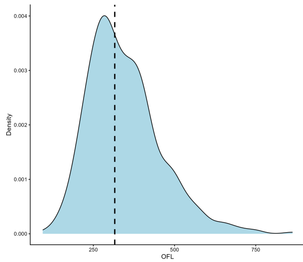
Figure 9: The probability density function of the OFL for model 26.1.d, based on 1,000 Markov chain Monte Carlo (MCMC) draws. The vertical dashed line represents the OFL from the original model run.
