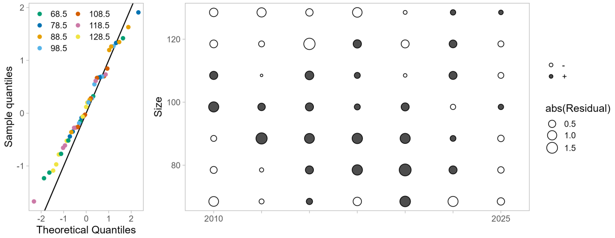
Figure 54: One-Step-Ahead residuals for model 26.1.nd fits to size composition data from the National Oceanic and Atmospheric Administration (NOAA) Northern Bering Sea (NBS) trawl survey.
