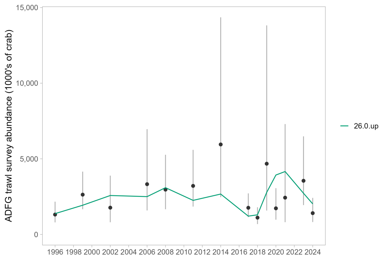
Figure 28: Model fits to the design-based index of abundance from the Alaska Department of Fish and Game (ADFG) trawl survey for the base model.
