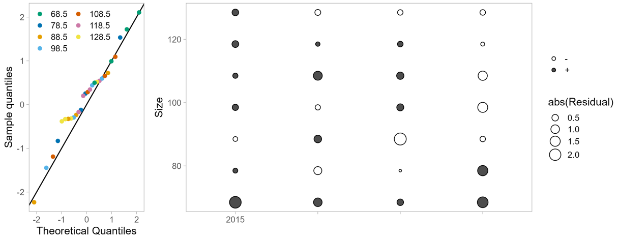
Figure 48: One-Step-Ahead residuals for model 26.1.nd fits to size composition data from the winter commercial fishery retained catch.
