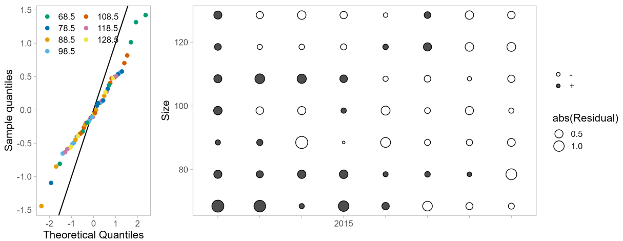
Figure 43: One-Step-Ahead residuals for model 26.0 fits to size composition data from the summer commercial fishery total catch.
