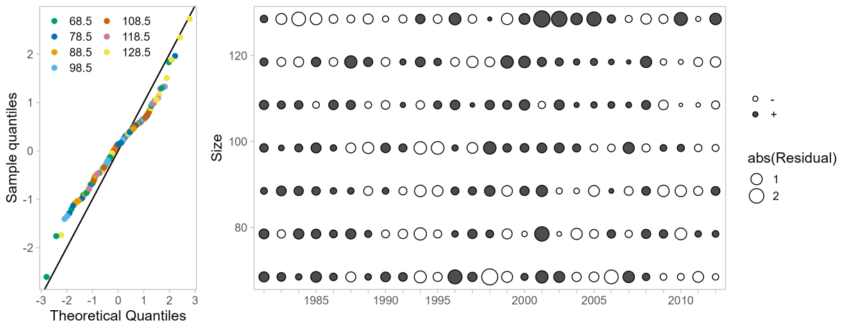
Figure 71: One-Step-Ahead residuals for model 26.2.nd fits to size composition data from the Alaska Department of Fish and Game (ADFG) winter pot survey.
