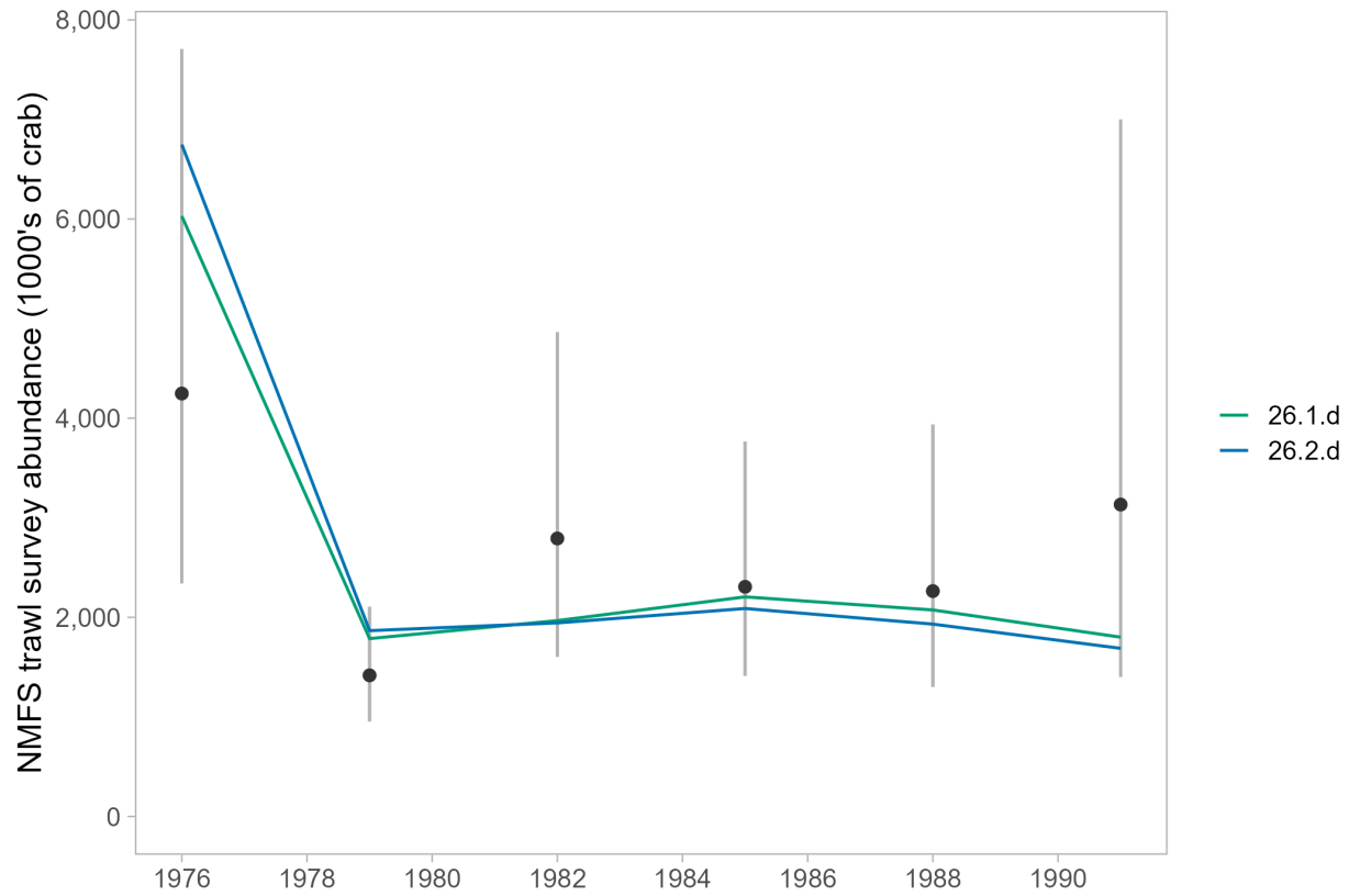
Figure 18: Model fits to the design-based index of abundance from the historical National Oceanic and Atmospheric Administration (NOAA) Norton Sound trawl survey for the models that included a model-based index of abundance that accounted for depth in place of the design-based indices for the ADFG and NBS trawl surveys. These models still included the design-based index of abundance from the historical survey shown here, as the data from the historical survey was not included in the model-based index.
