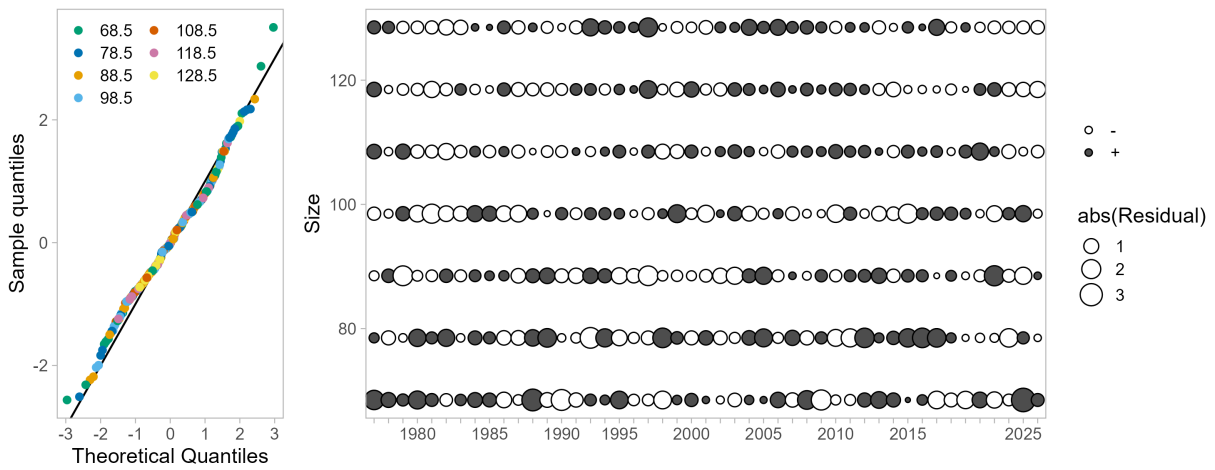
Figure 65: One-Step-Ahead residuals for model 26.2.nd fits to size composition data from the summer commercial fishery retained catch.
