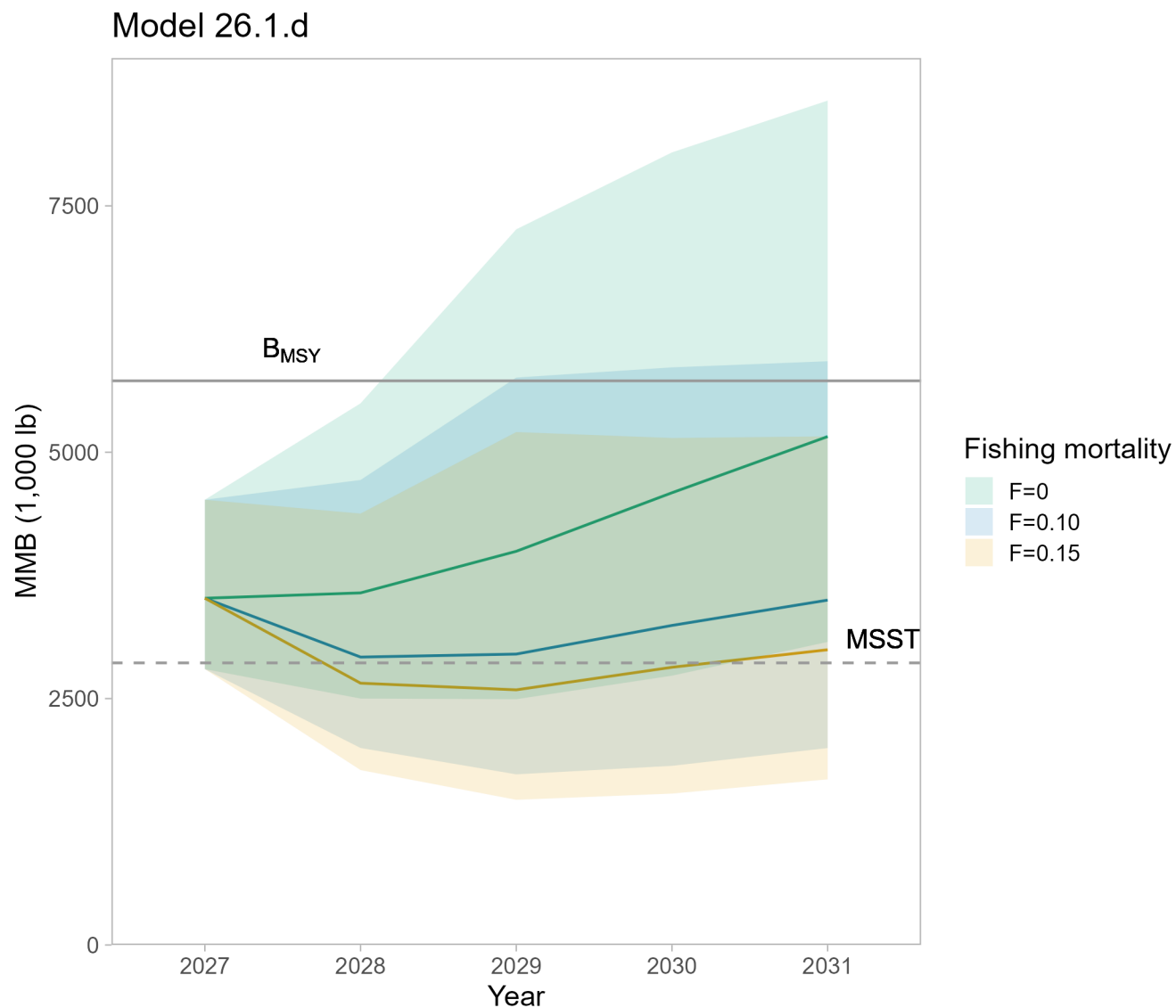
Figure 92: Mature male biomass (MMB) projections from the model using a model-based index of abundance that takes into account depth (26.1.d) for the next five years. Solid colored lines represent mean projected MMB for each fishing mortality rate while shaded regions represent 0.05 to 0.95 quantiles. The solid horizontal line shows B_{MSY} , which is equal to time series mean MMB for this Tier 4 stock, while the dashed horizontal line shows MSST (the minimum stock size threshold, 0.5 * B_{MSY} ).
