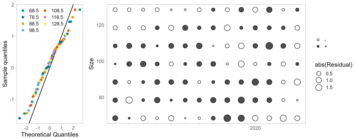
Figure 61: One-Step-Ahead residuals for model 26.1.d fits to size composition data from the Alaska Department of Fish and Game (ADFG) trawl survey.
