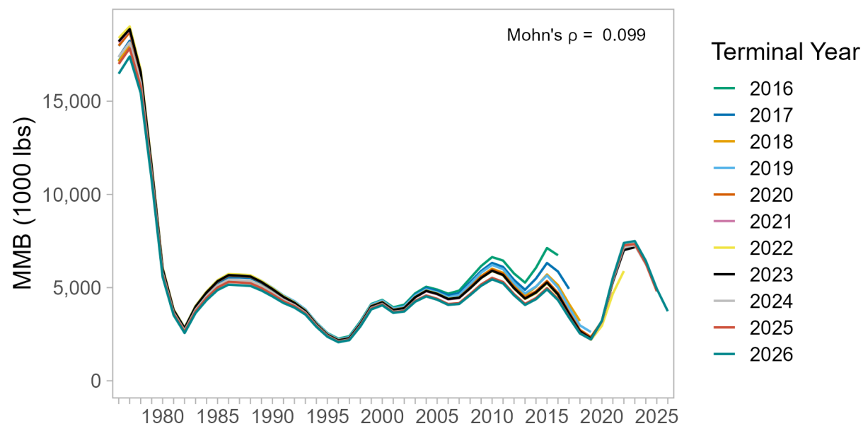
Figure 85: Retrospective patterns in estimated mature male biomass (MMB) for the base model with updated data and GMACS version (26.0.up).
