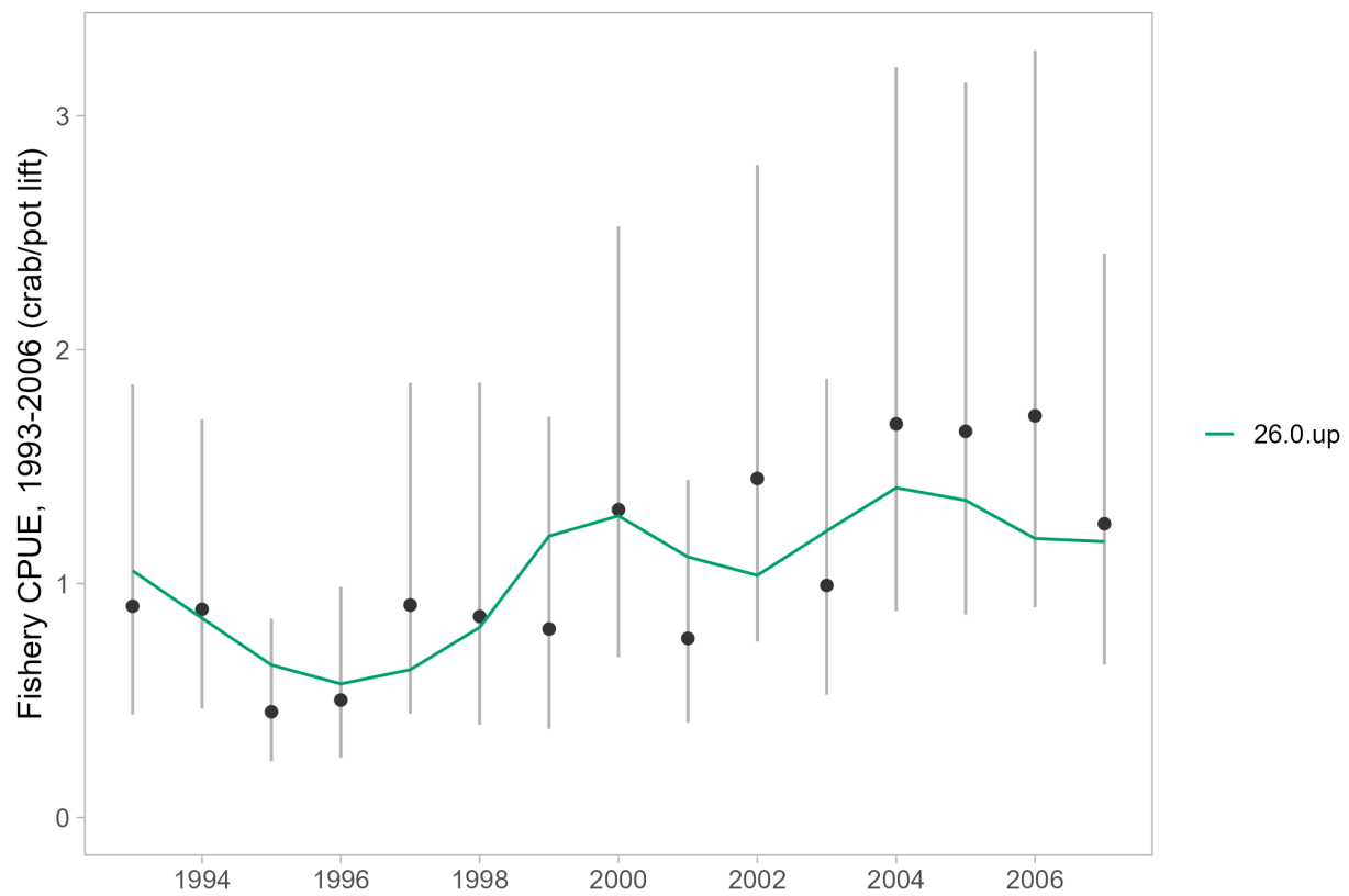
Figure 20: Model fits to the summer commercial fishery standardized catch per unit effort (CPUE) index (1993-2006) for the updated base model.
