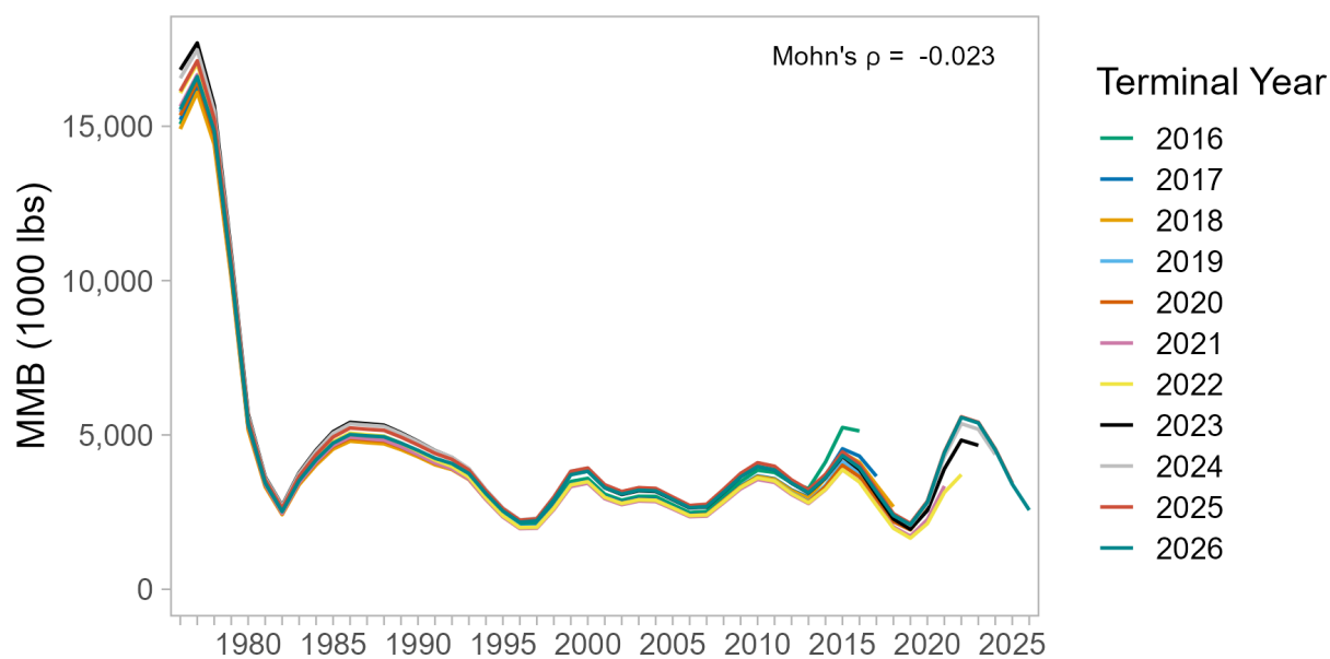
Figure 89: Retrospective patterns in estimated mature male biomass (MMB) for model 26.2.d, which uses a model-based index of abundance that takes into account depth, and also estimates catchability for that index.
