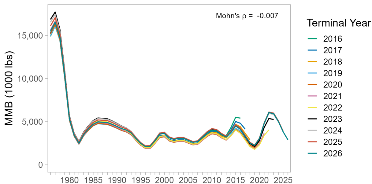
Figure 88: Retrospective patterns in estimated mature male biomass (MMB) for model 26.2.nd, which uses a model-based index of abundance that does not take into account depth, and also estimates catchability for that index.
