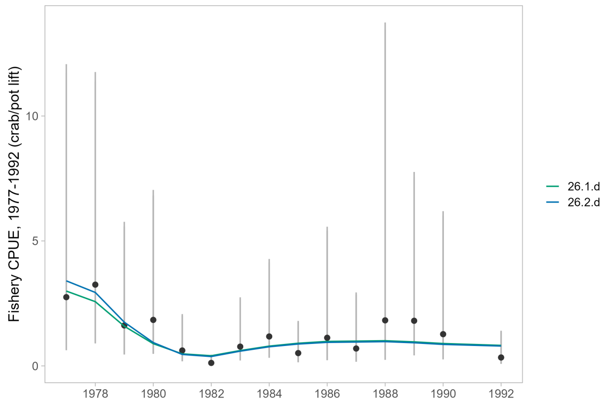
Figure 25: Model fits to the summer commercial fishery standardized catch per unit effort (CPUE) index (1977-1992) for the models including the model-based index of abundance that accounted for depth.
