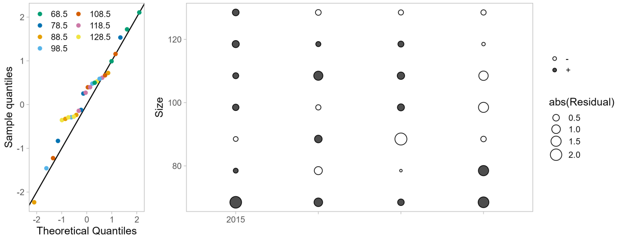
Figure 40: One-Step-Ahead residuals for model 26.0 fits to size composition data from the winter commercial fishery retained catch.
