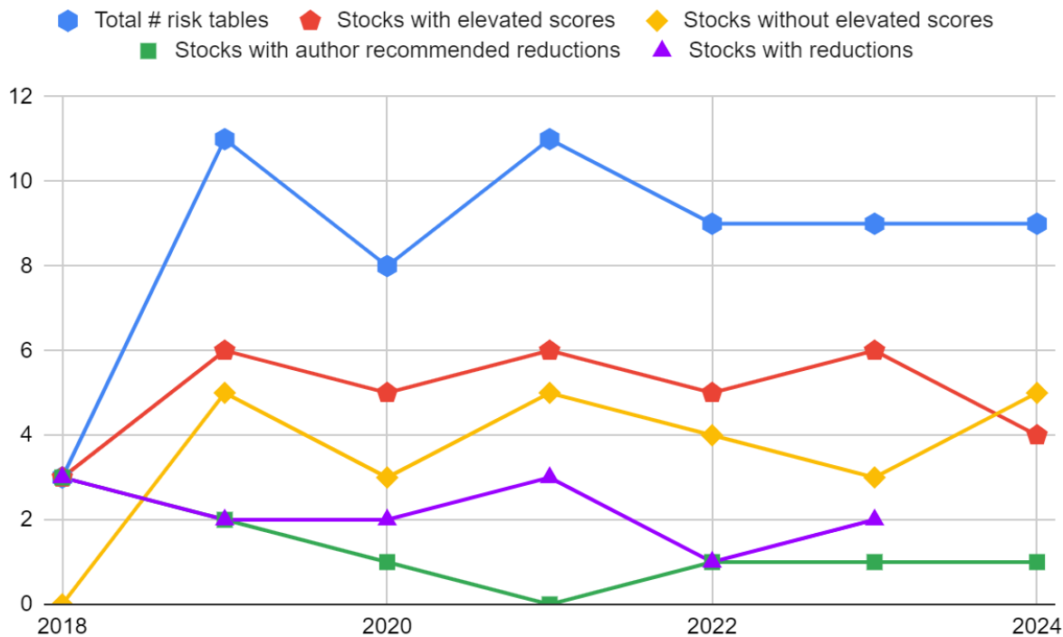
Figure 3: Summary counts of risk tables for the Gulf of Alaska (GOA) groundfish over the years 2018 to present based on Table 1. Blue line is the total number of risk tables completed for all stocks. Red line is the count of stocks with risk tables that had at least one elevated score ( \geq 2 ). Yellow line is the count of stocks without any elevated scores. Green line is the count of stocks with an author recommended reduction from maximum ABC. Purple line is the final count of risk tables with a reduction following review from Plan Team and SSC.
