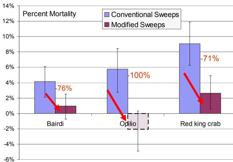
Figure 28 Estimated mortalities of Chionoecetes opilio , C. bairdi , and red king crab after contact with conventional and modified sweeps. Rates have been adjusted for handling mortality based on mortality estimates from a control net. (Apparent negative mortality is a non-significant artifact of the control adjustment).
